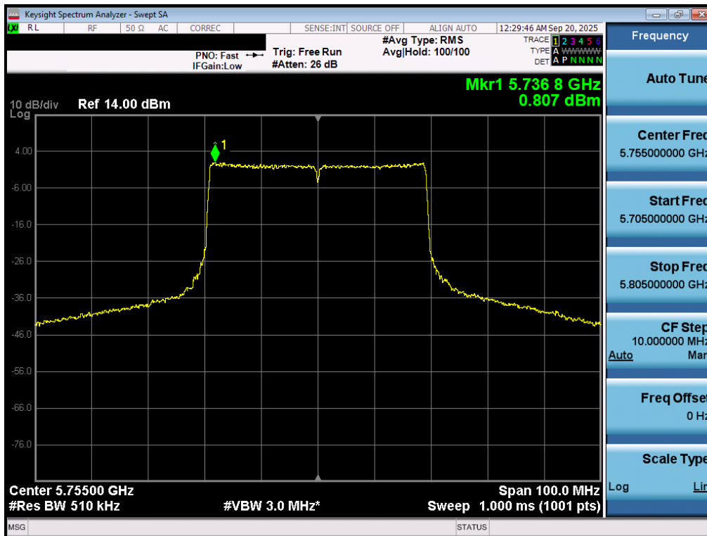
Plot 7-76. Power Spectral Density Plot MIMO ANT1 (40MHz BW 802.11be (UNII Band 3) – Ch. 151)
