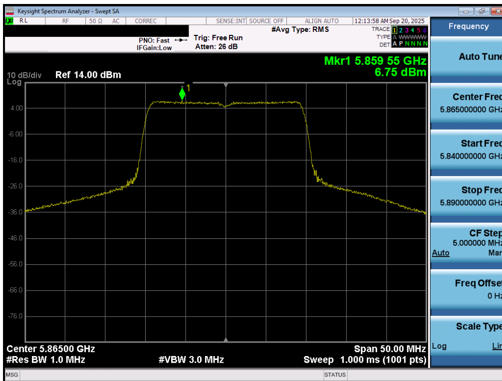
Plot 7-82. Power Spectral Density Plot MIMO ANT1 (20MHz BW 802.11be (UNII Band 4) – Ch. 173)
