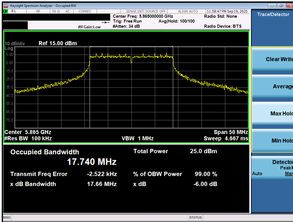
Plot 7-31. 6dB Bandwidth Plot MIMO ANT1 (20MHz BW 802.11n (UNII Band 4) – Ch. 173)
