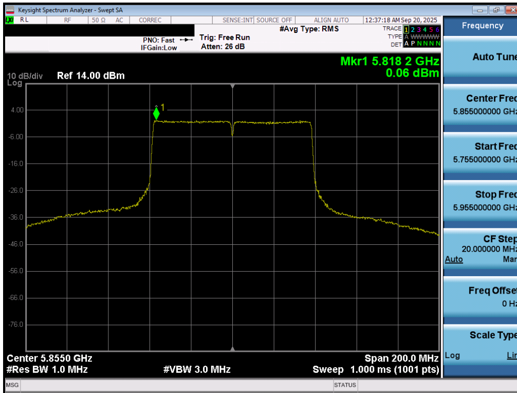
Plot 7-85. Power Spectral Density Plot MIMO ANT1 (80MHz BW 802.11ac (UNII Band 3/4) – Ch. 171)
