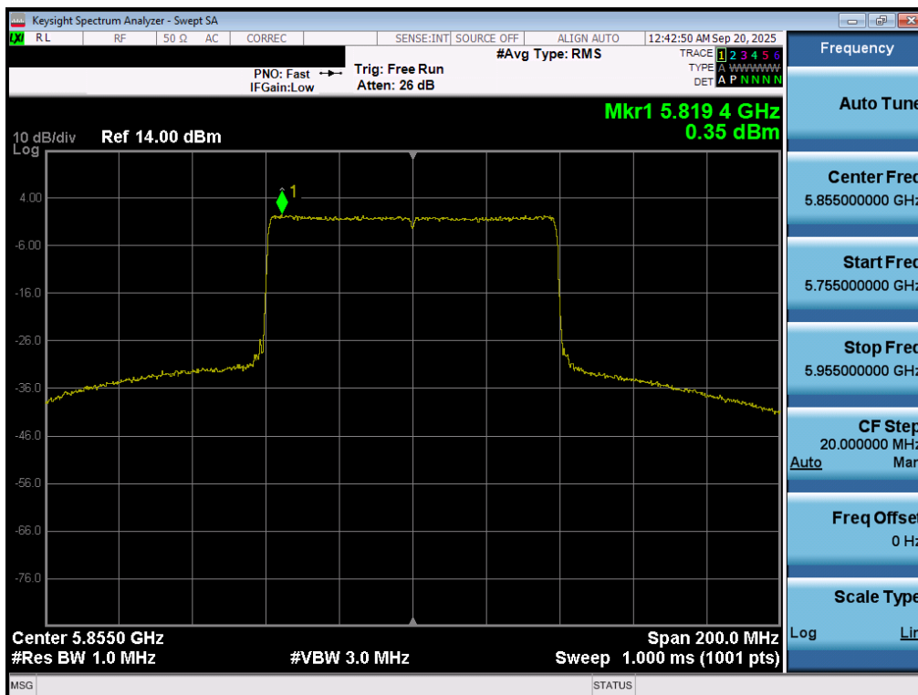
Plot 7-86. Power Spectral Density Plot MIMO ANT1 (80MHz BW 802.11be (UNII Band 3/4) – Ch. 171)
