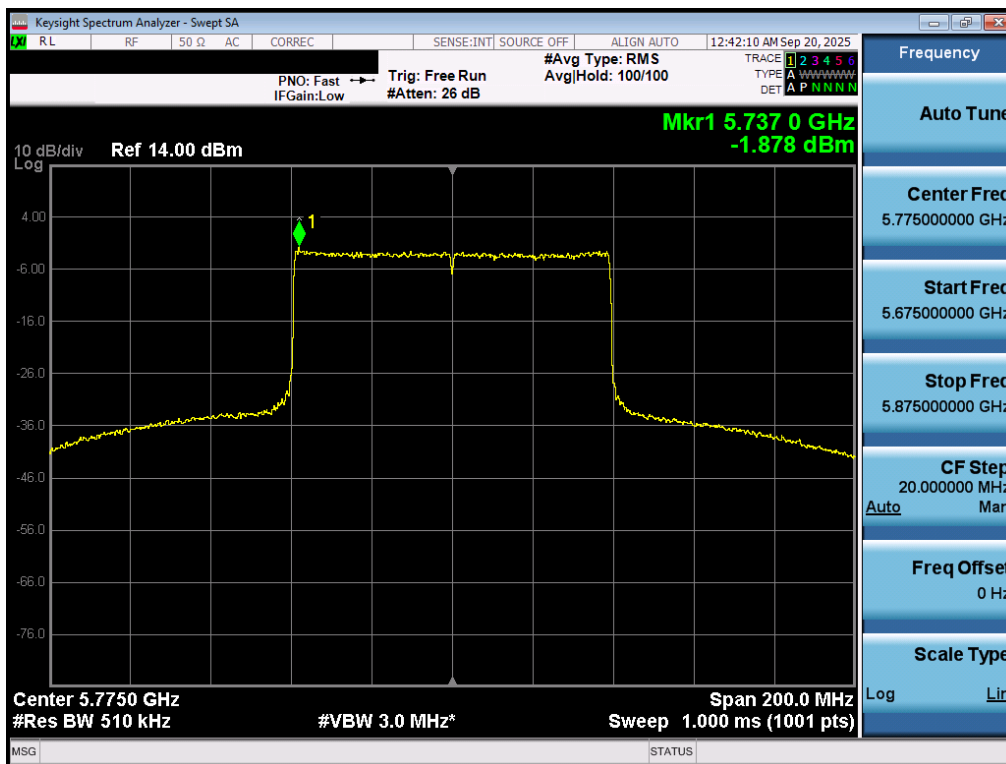
Plot 7-78. Power Spectral Density Plot MIMO ANT1 (80MHz BW 802.11be (UNII Band 3) – Ch. 155)
