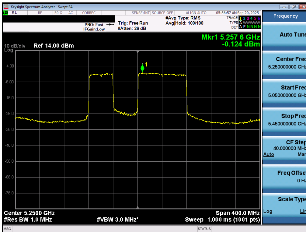
Plot 7-78. Power Spectral Density Plot MIMO ANT1 (160MHz BW 802.11be – 996+484 Tones (UNII Band 1/2A) – Ch. 50)
