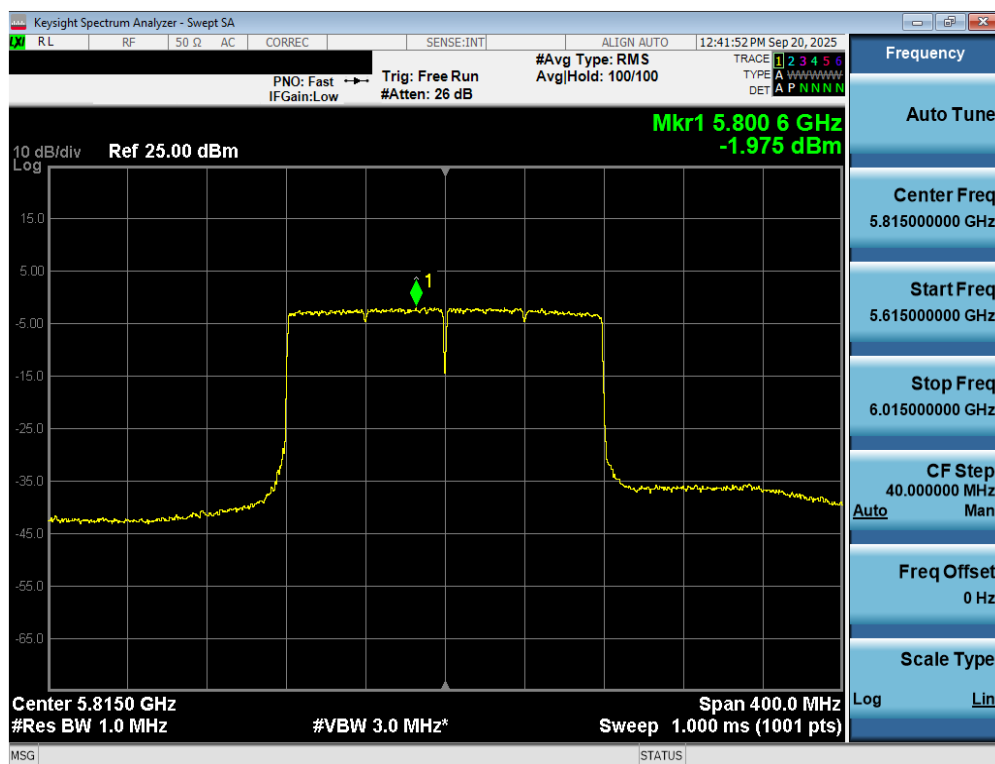
Plot 7-103. Power Spectral Density Plot MIMO ANT2 (160MHz BW 802.11be – 996*2 Tones (UNII Band 3/4) – Ch. 163)
