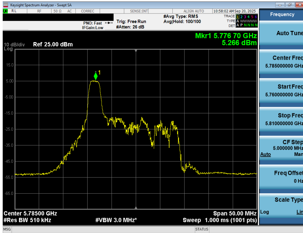
Plot 7-86. Power Spectral Density Plot MIMO ANT2 (20MHz BW 802.11be – 26 Tones (UNII Band 3) – Ch. 157)
