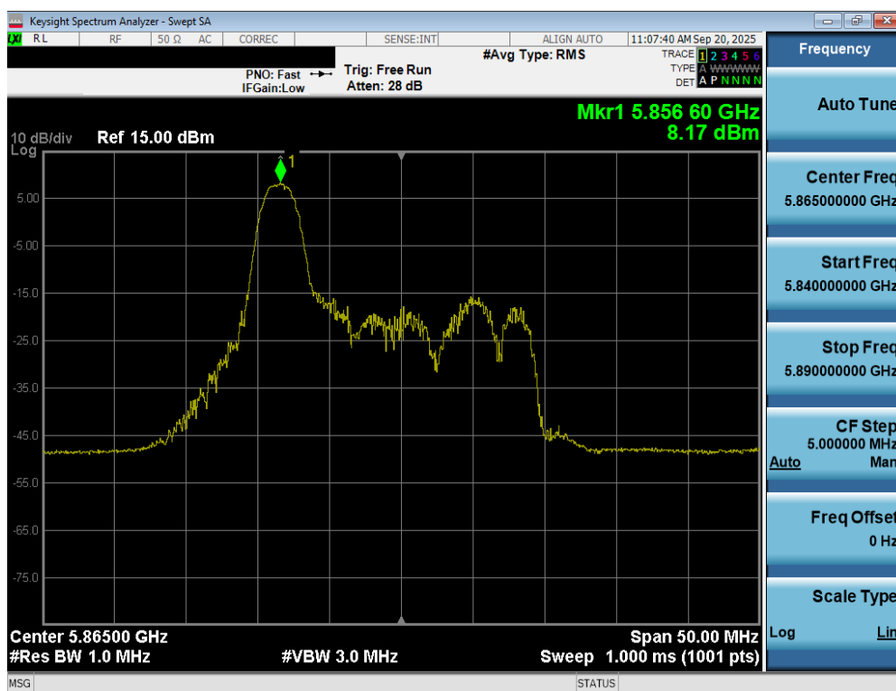
Plot 7-89. Power Spectral Density Plot MIMO ANT2 (20MHz BW 802.11be – 26 Tones (UNII Band 4) – Ch. 173)
