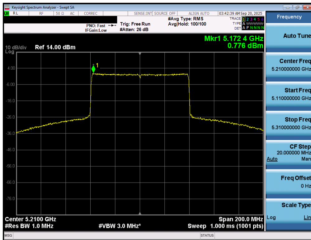
Plot 7-68. Power Spectral Density Plot MIMO ANT1 (80MHz BW 802.11be – 996 Tones (UNII Band 1) – Ch. 42)
