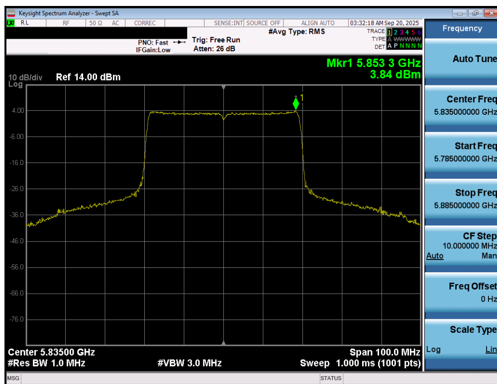
Plot 7-74. Power Spectral Density Plot MIMO ANT1 (40MHz BW 802.11be – 484 Tones (UNII Band 3/4) – Ch. 167)
