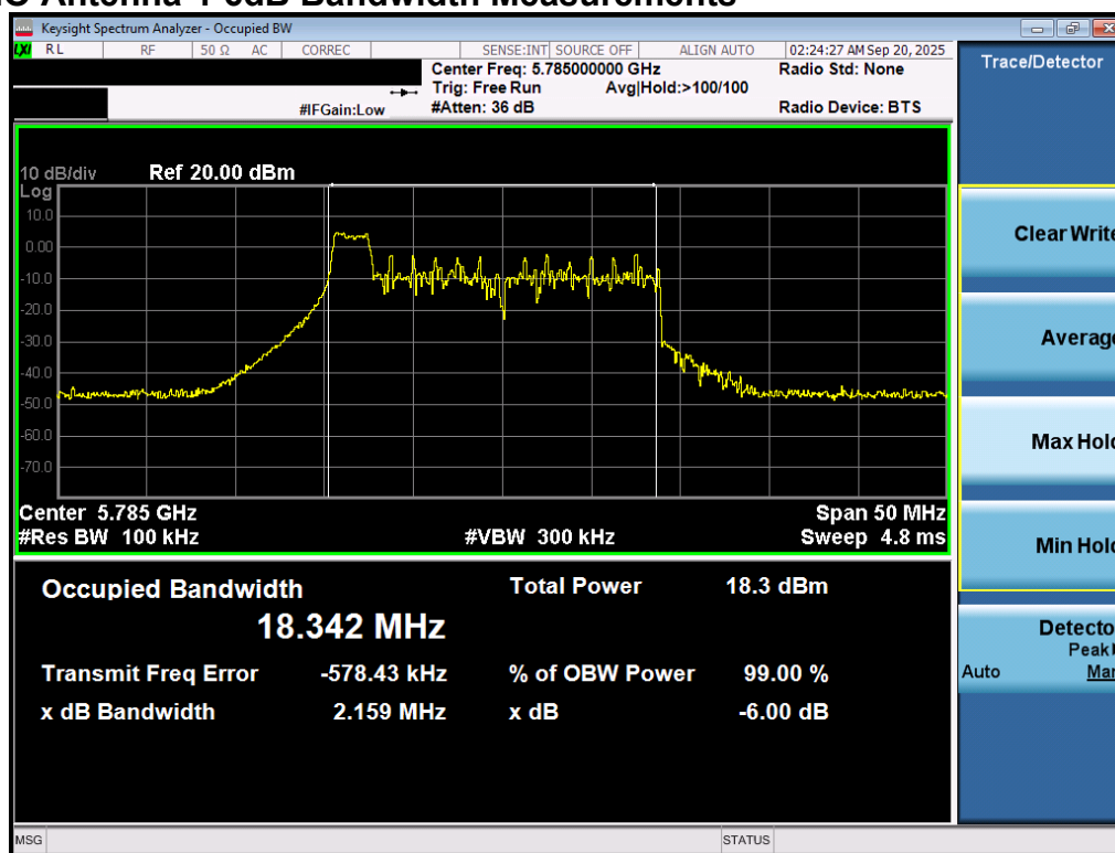
Plot 7-21. 6dB Bandwidth Plot MIMO ANT1 (20MHz BW 802.11be – 26 Tones (UNII Band 3) – Ch. 157)
