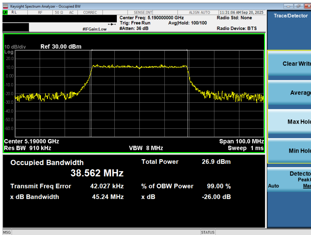
Plot 7-16. 26dB Bandwidth Plot MIMO ANT2 (40MHz BW 802.11be – 484 Tones (UNII Band 1) – Ch. 38)
