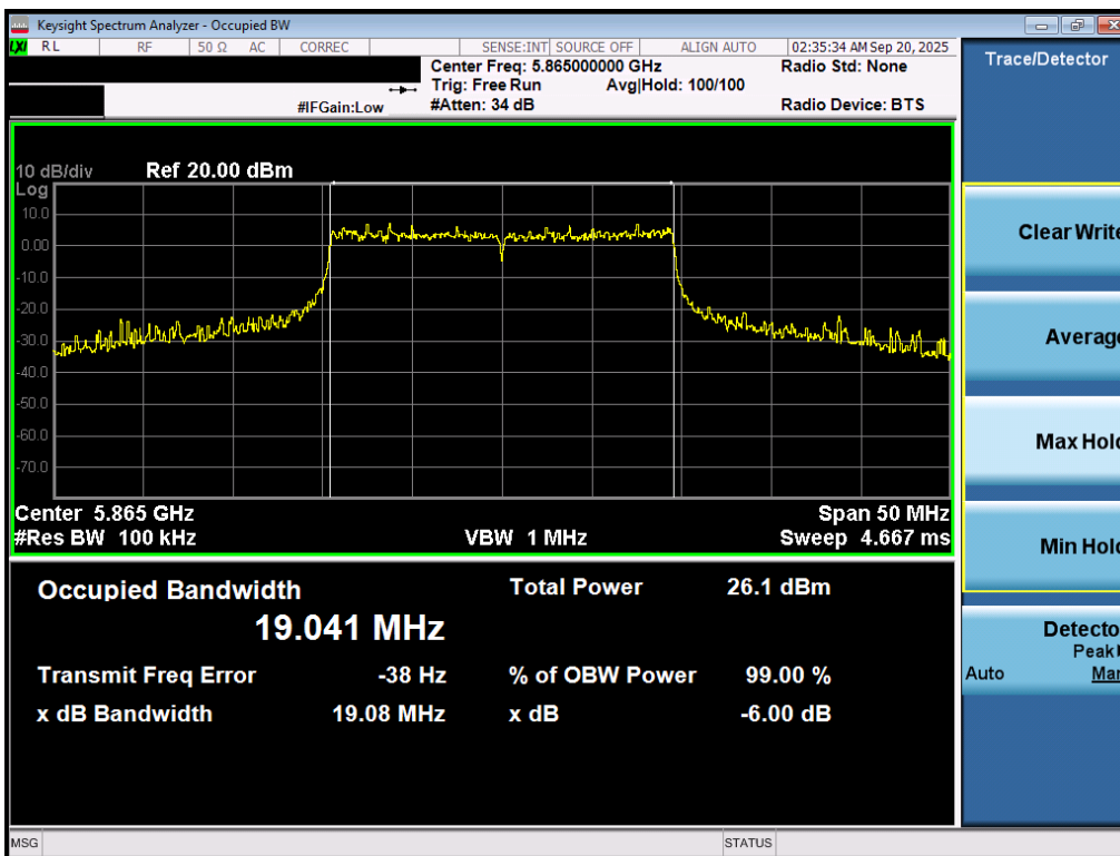
Plot 7-32. 6dB Bandwidth Plot MIMO ANT1 (20MHz BW 802.11be – 242 Tones (UNII Band 4) – Ch. 173)
