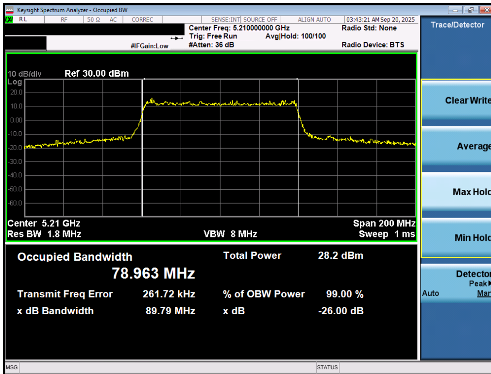
Plot 7-7. 26dB Bandwidth Plot MIMO ANT1 (80MHz BW 802.11be – 996 Tones (UNII Band 1) – Ch. 42)
