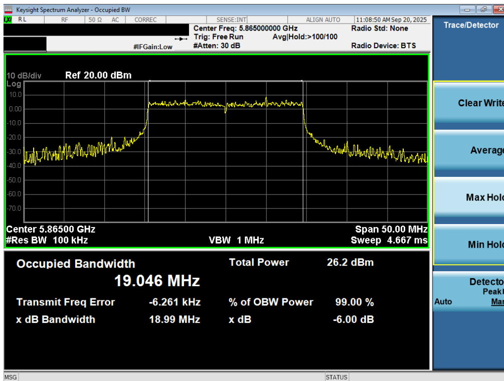
Plot 7-49. 6dB Bandwidth Plot MIMO ANT2 (20MHz BW 802.11be – 242 Tones (UNII Band 4) – Ch. 173)
