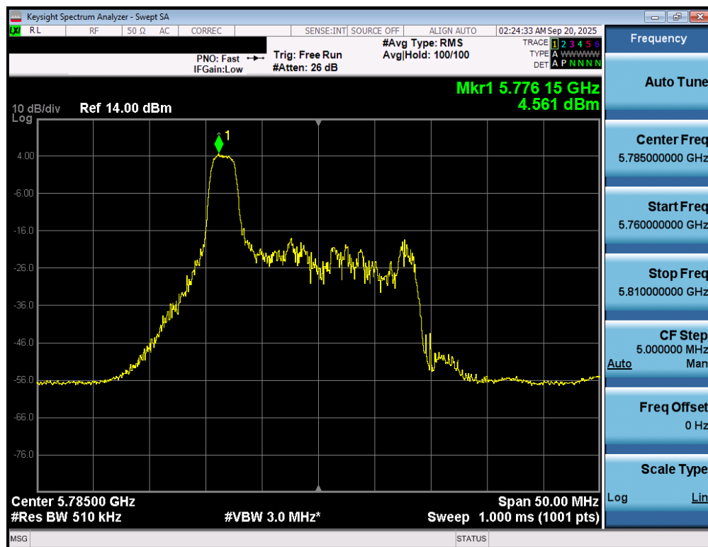
Plot 7-59. Power Spectral Density Plot MIMO ANT1 (20MHz BW 802.11be – 26 Tones (UNII Band 3) – Ch. 157)
