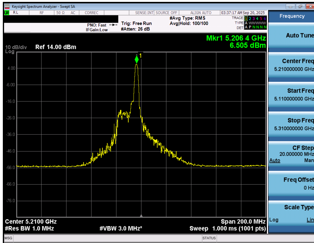
Plot 7-57. Power Spectral Density Plot MIMO ANT1 (80MHz BW 802.11be – 26 Tones (UNII Band 1) – Ch. 42)
