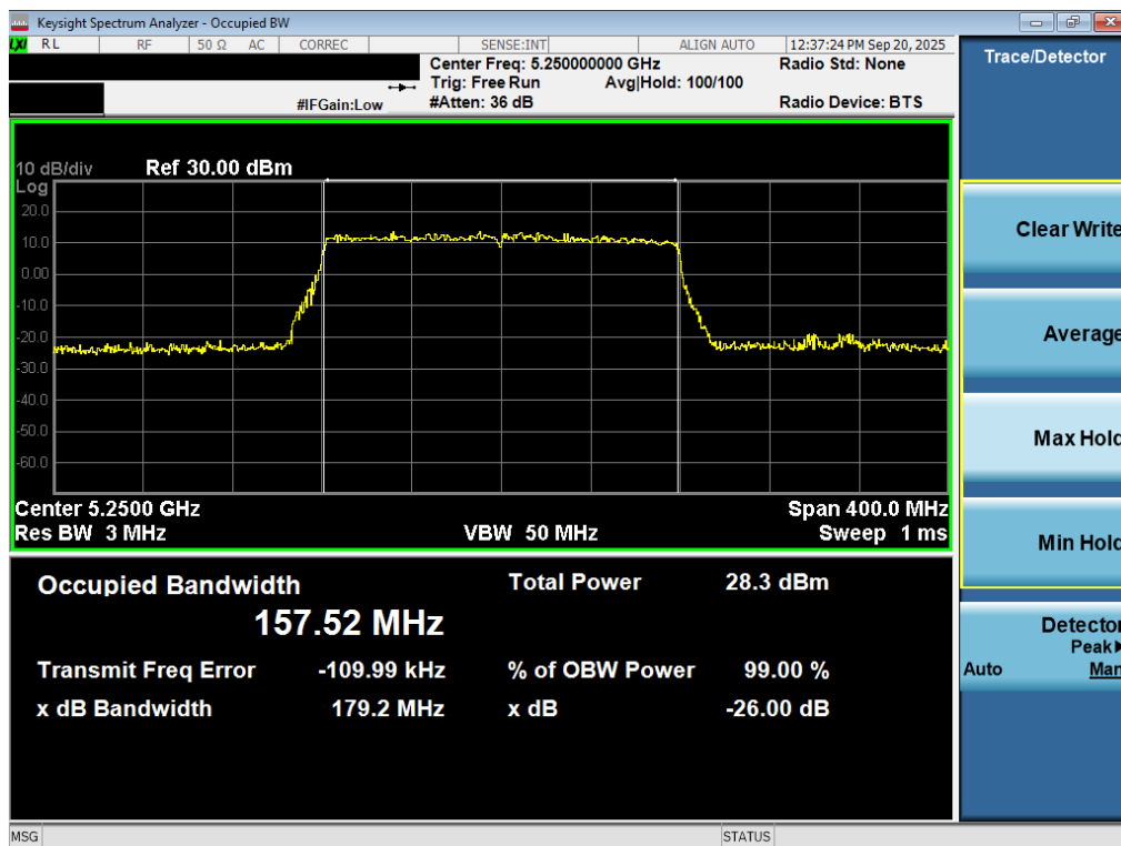
Plot 7-18. 26dB Bandwidth Plot MIMO ANT2 (160MHz BW 802.11be – 2x996 Tones (UNII Band 1/2A) – Ch. 50)
