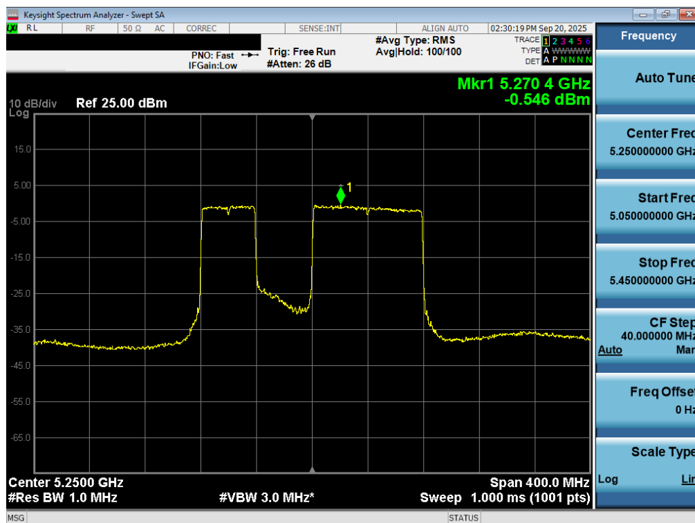
Plot 7-105. Power Spectral Density Plot MIMO ANT2 (160MHz BW 802.11be – 996+484 Tones (UNII Band 1/2A) – Ch. 50)
