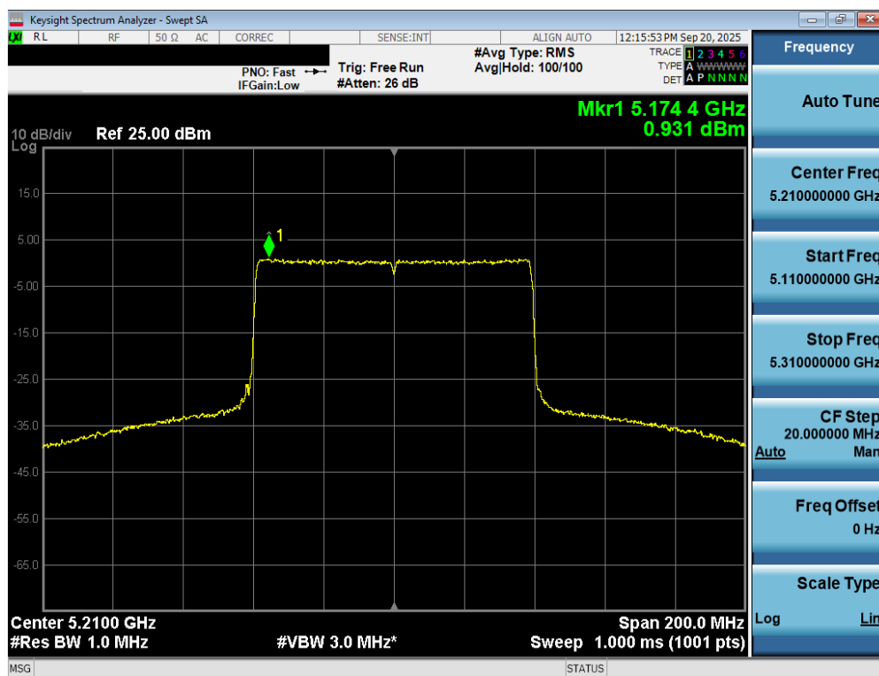
Plot 7-95. Power Spectral Density Plot MIMO ANT2 (80MHz BW 802.11be – 996 Tones (UNII Band 1) – Ch. 42)
