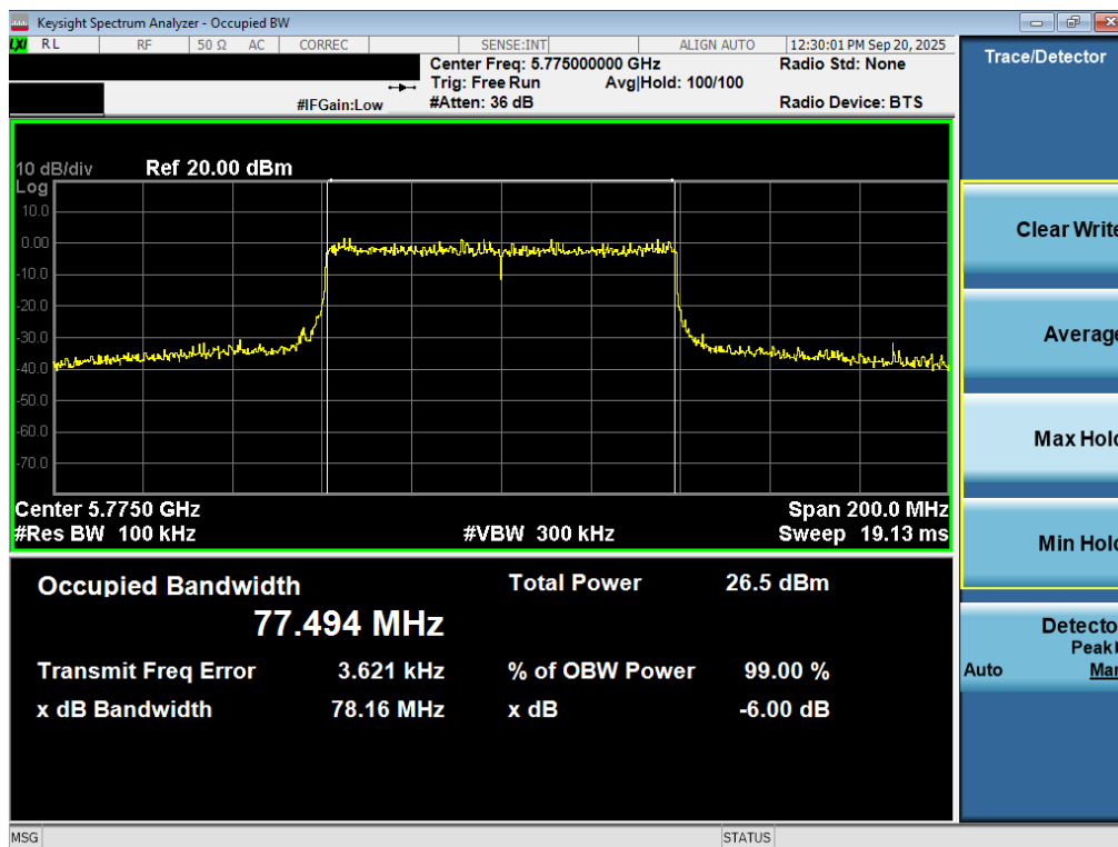
Plot 7-47. 6dB Bandwidth Plot MIMO ANT2 (80MHz BW 802.11be – 996 Tones (UNII Band 3) – Ch. 155)
