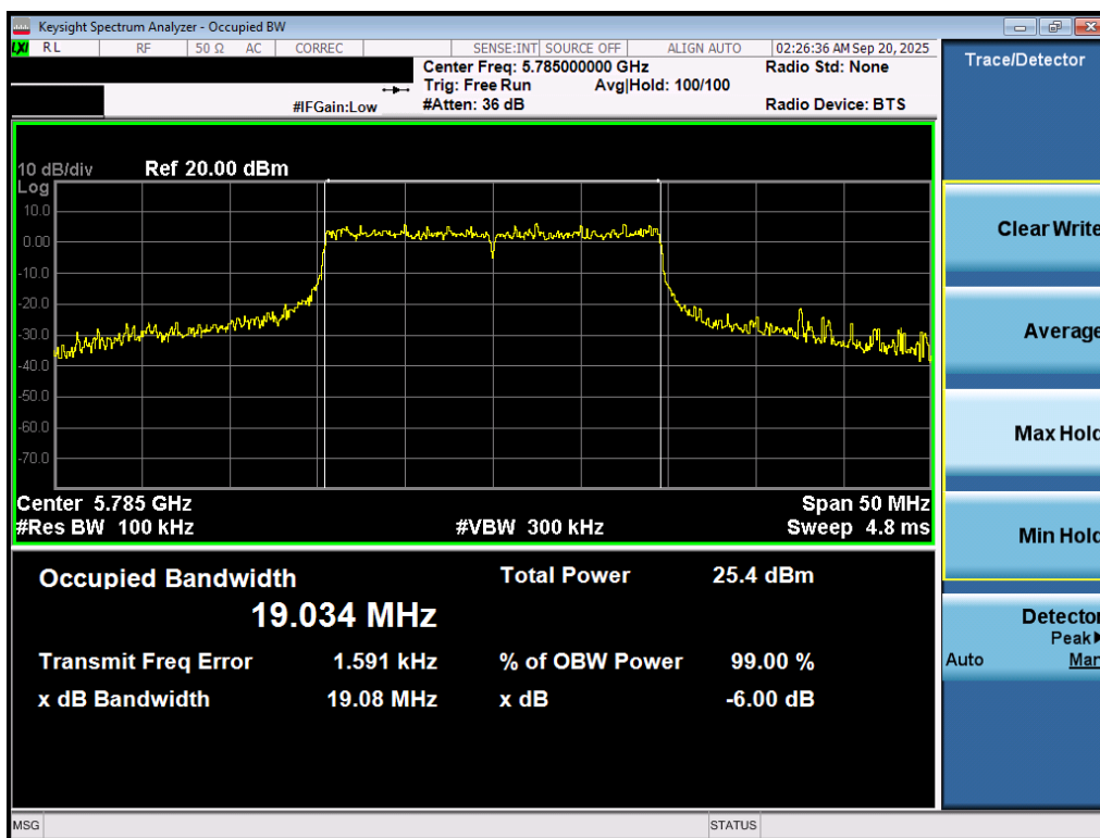
Plot 7-28. 6dB Bandwidth Plot MIMO ANT1 (20MHz BW 802.11be – 242 Tones (UNII Band 3) – Ch. 157)
