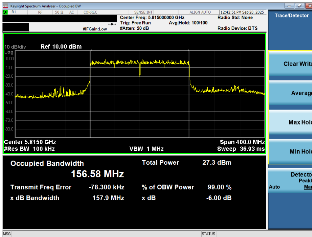
Plot 7-52. 6dB Bandwidth Plot MIMO ANT2 (160MHz BW 802.11be – 996*2 Tones (UNII Band 3/4) – Ch. 163)
