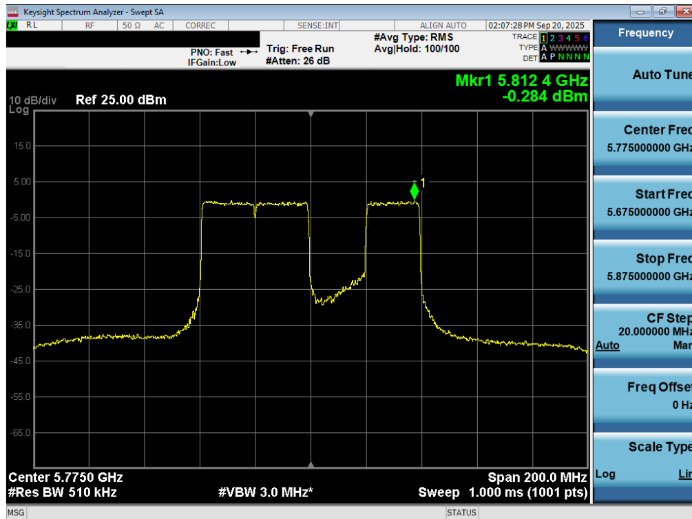
Plot 7-106. Power Spectral Density Plot MIMO ANT2 (80MHz BW 802.11be – 484+242 Tones (UNII Band 3) – Ch. 155)
