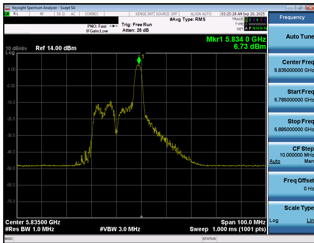
Plot 7-63. Power Spectral Density Plot MIMO ANT1 (40MHz BW 802.11be – 26 Tones (UNII Band 3/4) – Ch. 167)
