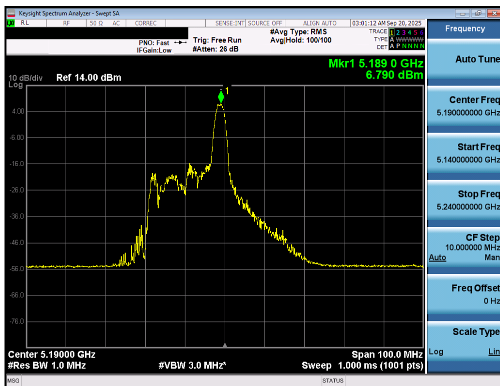
Plot 7-56. Power Spectral Density Plot MIMO ANT1 (40MHz BW 802.11be – 26 Tones (UNII Band 1) – Ch. 38)
