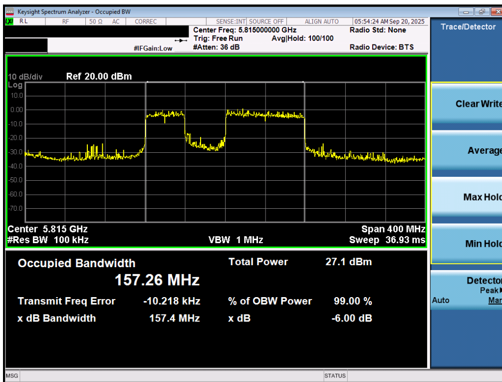
Plot 7-37. 6dB Bandwidth Plot MIMO ANT1 (160MHz BW 802.11be – 996+484 Tones (UNII Band 3/4) – Ch. 163)
