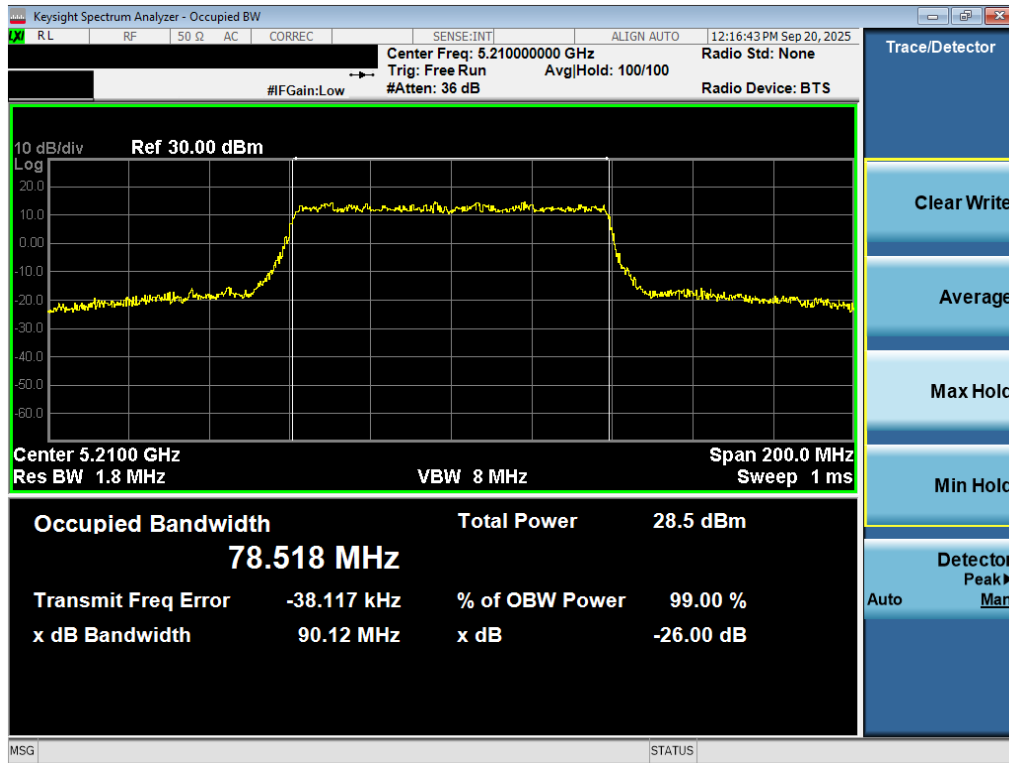
Plot 7-17. 26dB Bandwidth Plot MIMO ANT2 (80MHz BW 802.11be – 996 Tones (UNII Band 1) – Ch. 42)
