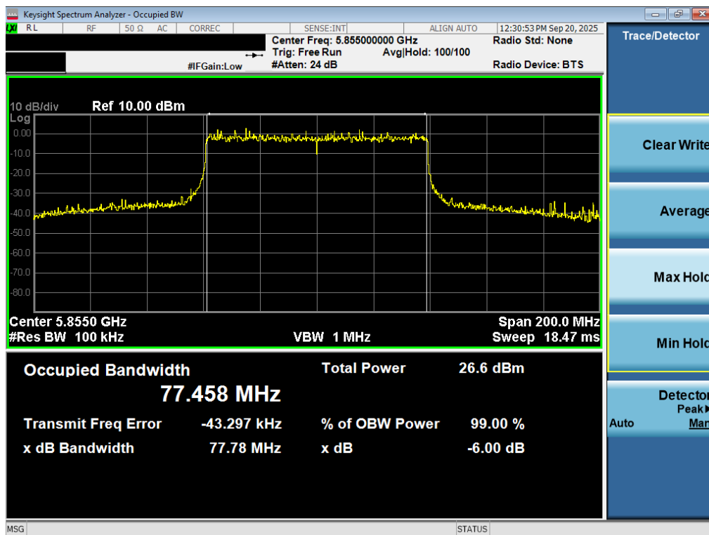
Plot 7-51. 6dB Bandwidth Plot MIMO ANT2 (80MHz BW 802.11be – 996 Tones (UNII Band 3/4) – Ch. 171)
