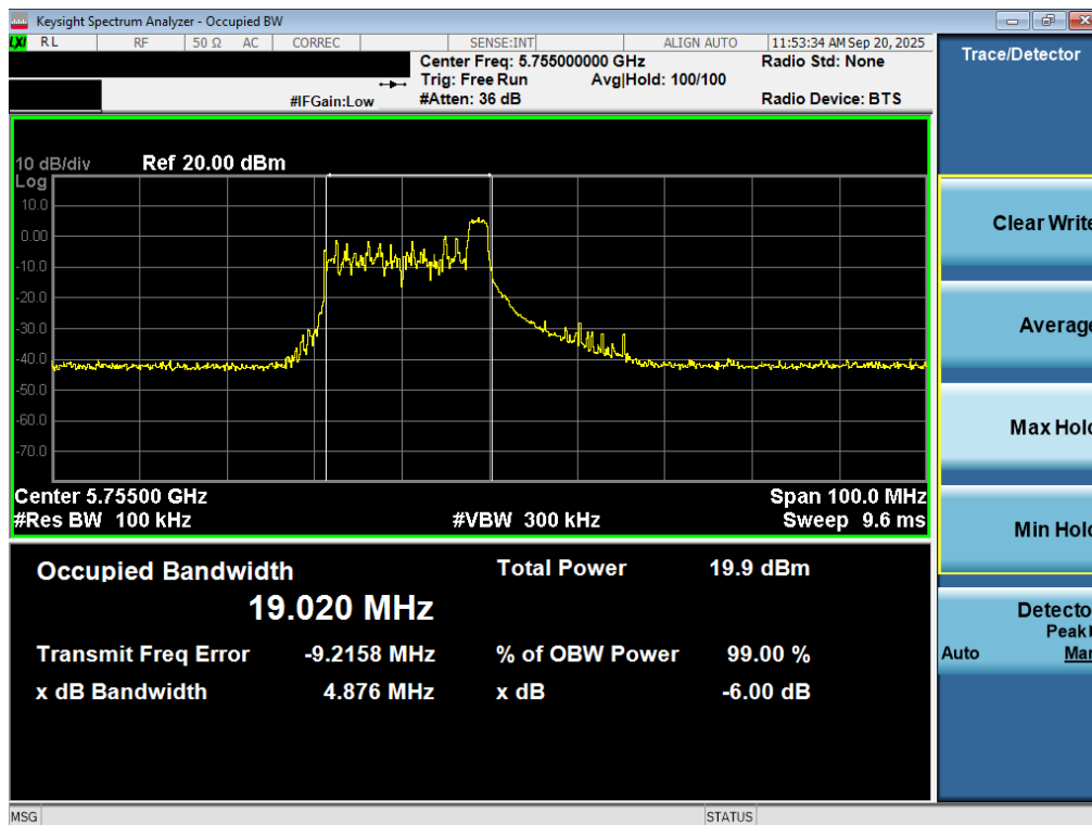
Plot 7-39. 6dB Bandwidth Plot MIMO ANT2 (40MHz BW 802.11be – 26 Tones (UNII Band 3) – Ch. 151)
