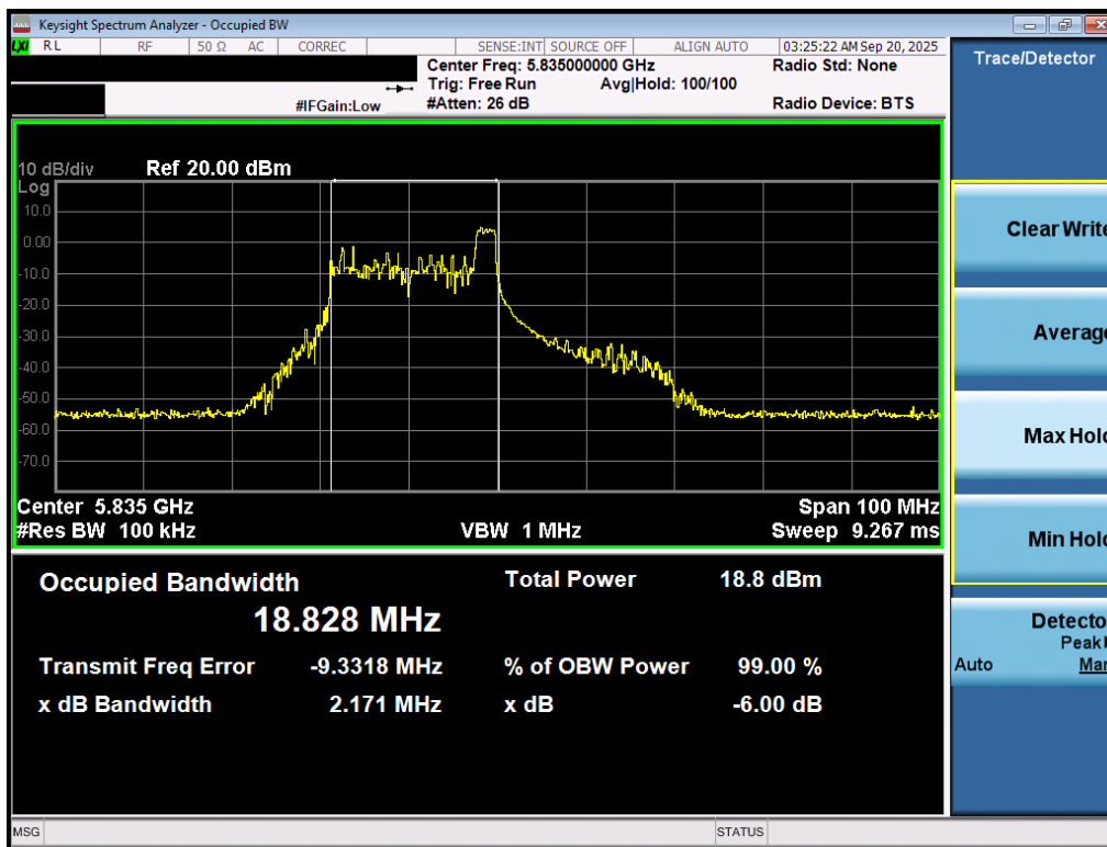
Plot 7-25. 6dB Bandwidth Plot MIMO ANT1 (40MHz BW 802.11be – 26 Tones (UNII Band 3/4) – Ch. 167)
