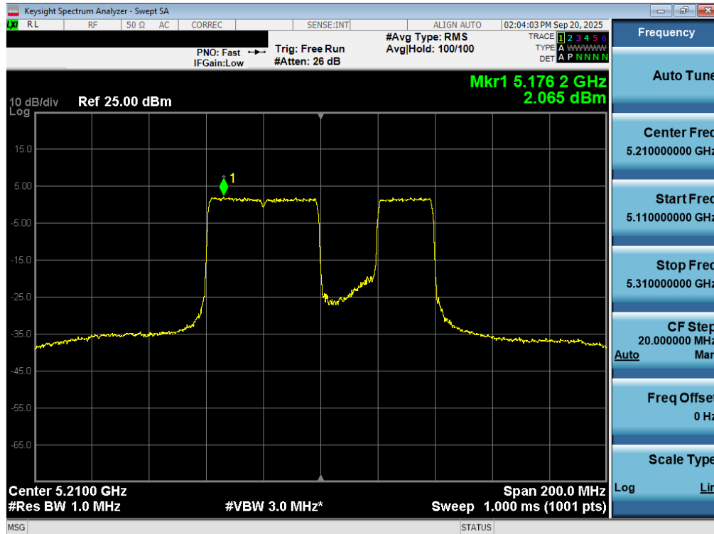
Plot 7-104. Power Spectral Density Plot MIMO ANT2 (80MHz BW 802.11be – 484+242 Tones (UNII Band 1) – Ch. 42)
