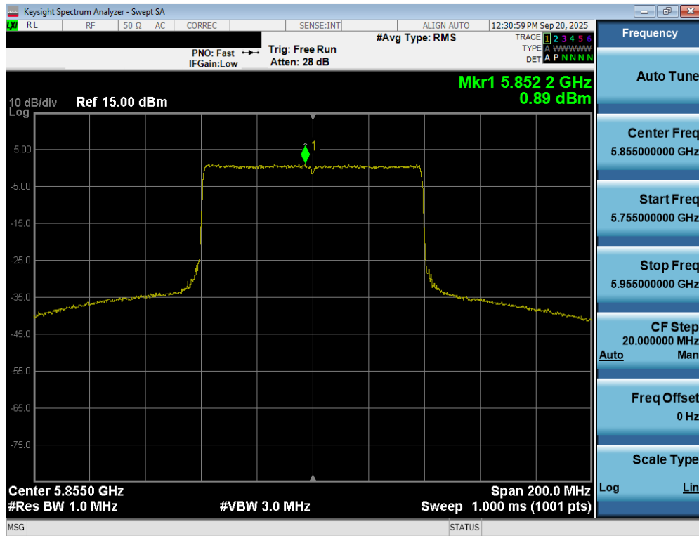
Plot 7-102. Power Spectral Density Plot MIMO ANT2 (80MHz BW 802.11be – 996 Tones (UNII Band 3/4) – Ch. 171)
