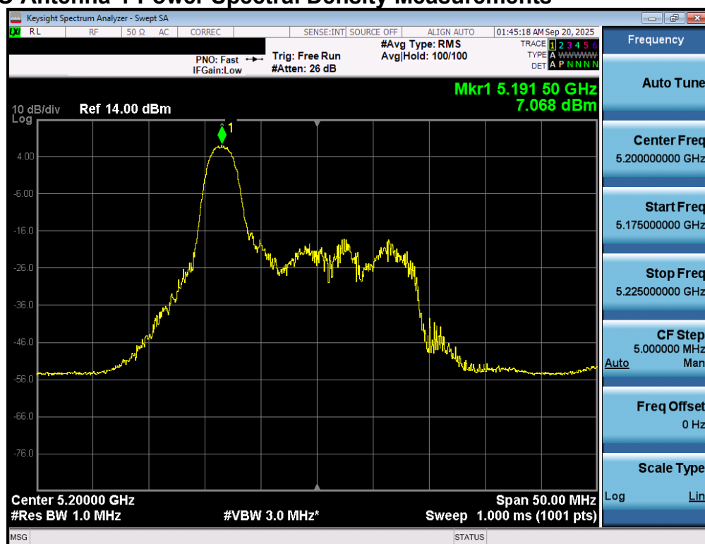
Plot 7-55. Power Spectral Density Plot MIMO ANT1 (20MHz BW 802.11be – 26 Tones (UNII Band 1) – Ch. 40)
