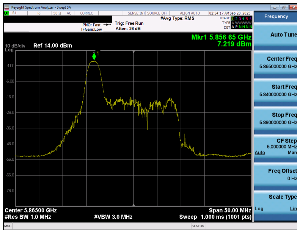
Plot 7-62. Power Spectral Density Plot MIMO ANT1 (20MHz BW 802.11be – 26 Tones (UNII Band 4) – Ch. 173)
