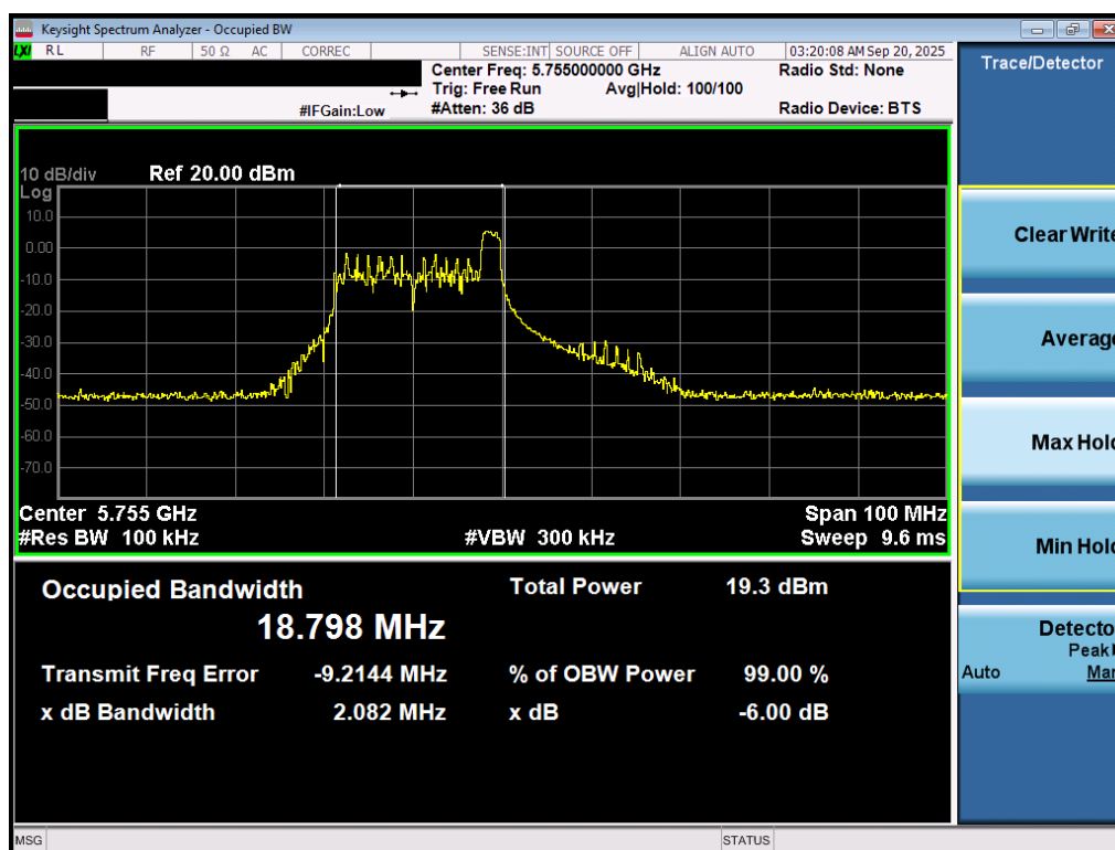
Plot 7-22. 6dB Bandwidth Plot MIMO ANT1 (40MHz BW 802.11be – 26 Tones (UNII Band 3) – Ch. 151)
