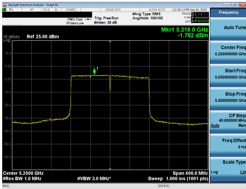
Plot 7-96. Power Spectral Density Plot MIMO ANT2 (160MHz BW 802.11be – 2x996 Tones (UNII Band 1/2A) – Ch. 50)
