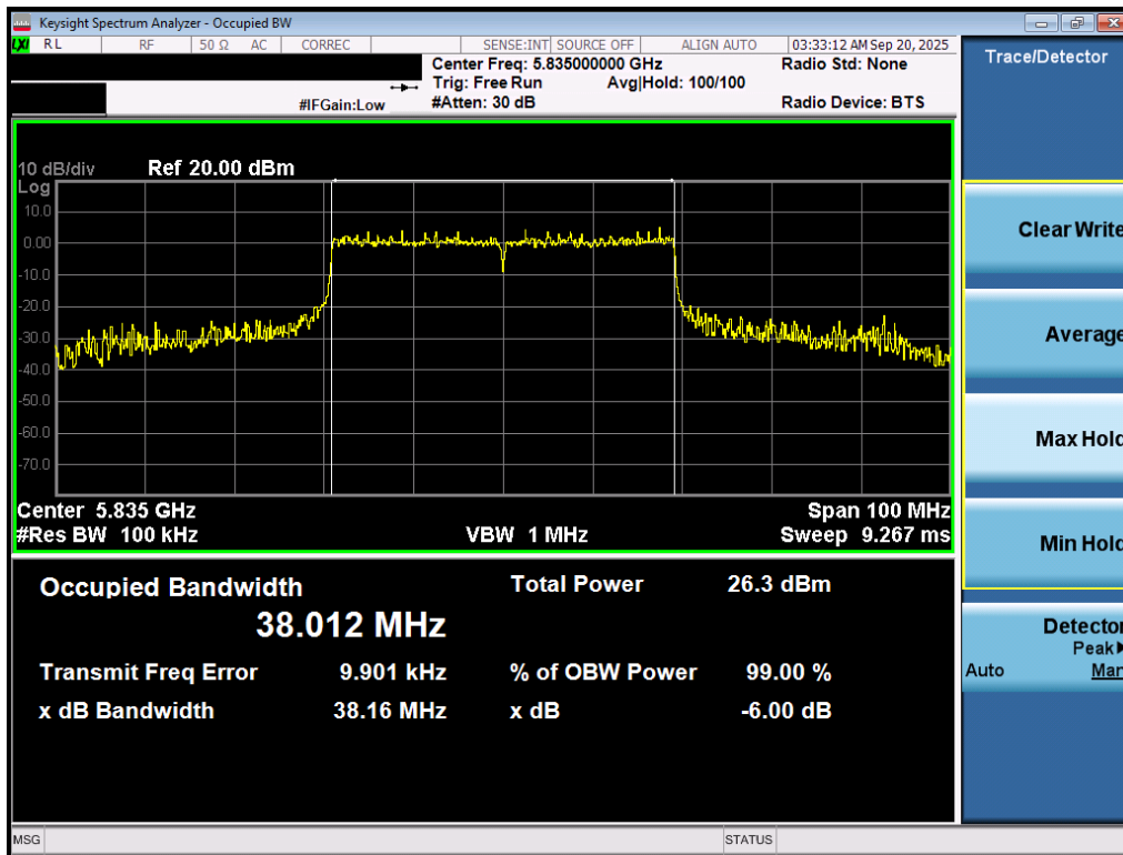
Plot 7-33. 6dB Bandwidth Plot MIMO ANT1 (40MHz BW 802.11be – 484 Tones (UNII Band 3/4) – Ch. 167)
