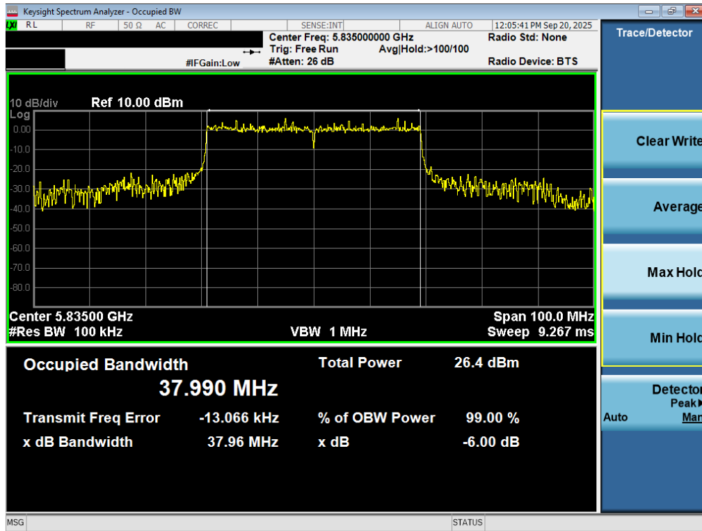
Plot 7-50. 6dB Bandwidth Plot MIMO ANT2 (40MHz BW 802.11be – 484 Tones (UNII Band 3/4) – Ch. 167)
