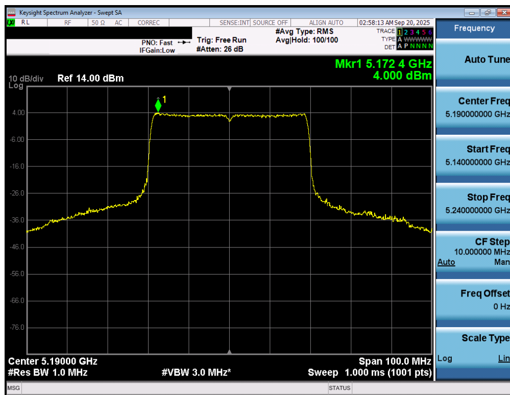
Plot 7-67. Power Spectral Density Plot MIMO ANT1 (40MHz BW 802.11be – 484 Tones (UNII Band 1) – Ch. 38)
