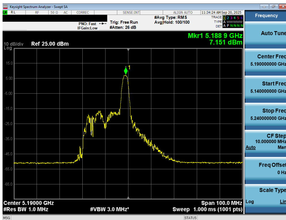
Plot 7-83. Power Spectral Density Plot MIMO ANT2 (40MHz BW 802.11be – 26 Tones (UNII Band 1) – Ch. 38)
