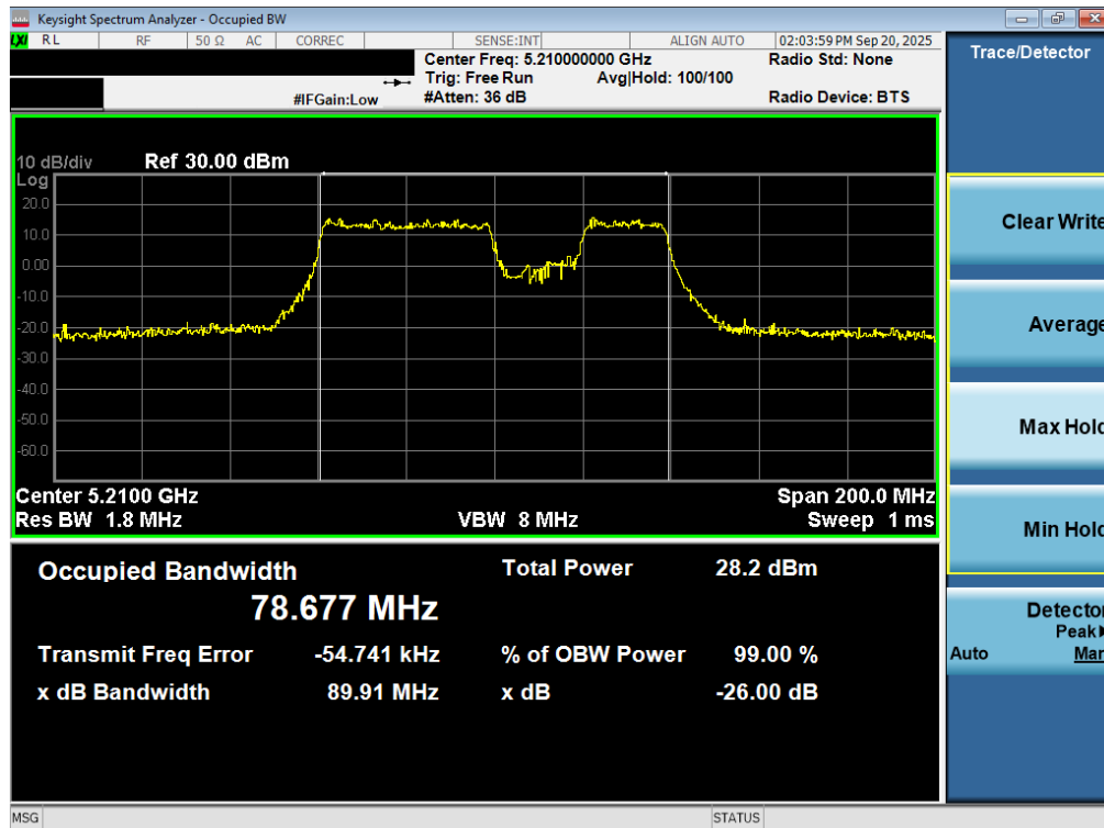
Plot 7-19. 26dB Bandwidth Plot MIMO ANT2 (80MHz BW 802.11be – 484+242 Tones (UNII Band 1) – Ch. 42)
