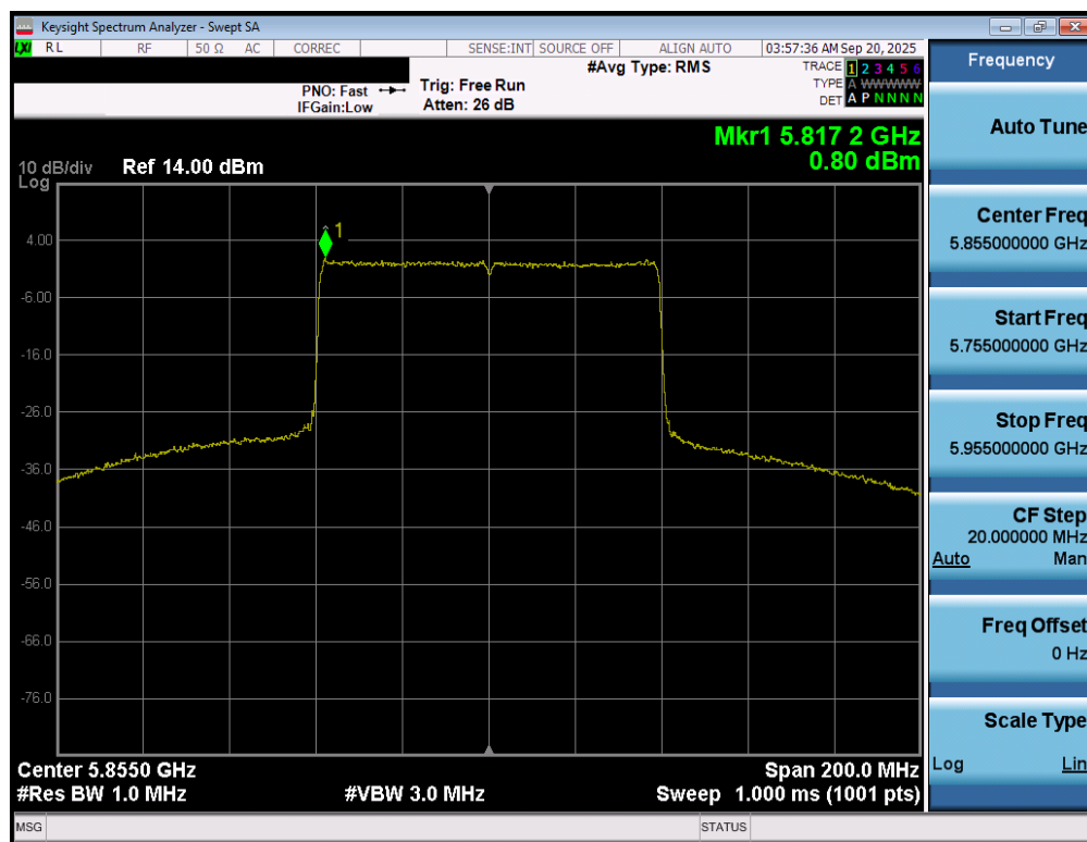
Plot 7-75. Power Spectral Density Plot MIMO ANT1 (80MHz BW 802.11be – 996 Tones (UNII Band 3/4) – Ch. 171)
