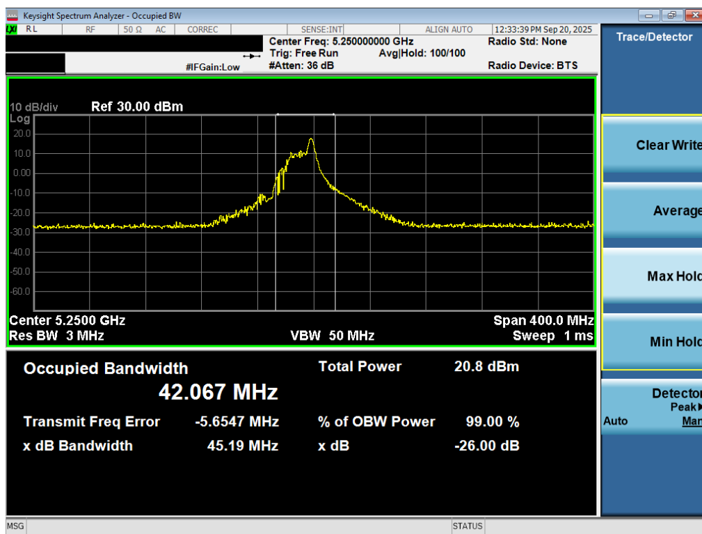
Plot 7-14. 26dB Bandwidth Plot MIMO ANT2 (160MHz(U) BW 802.11be – 26 Tones (UNII Band 1/2A) – Ch. 50)
