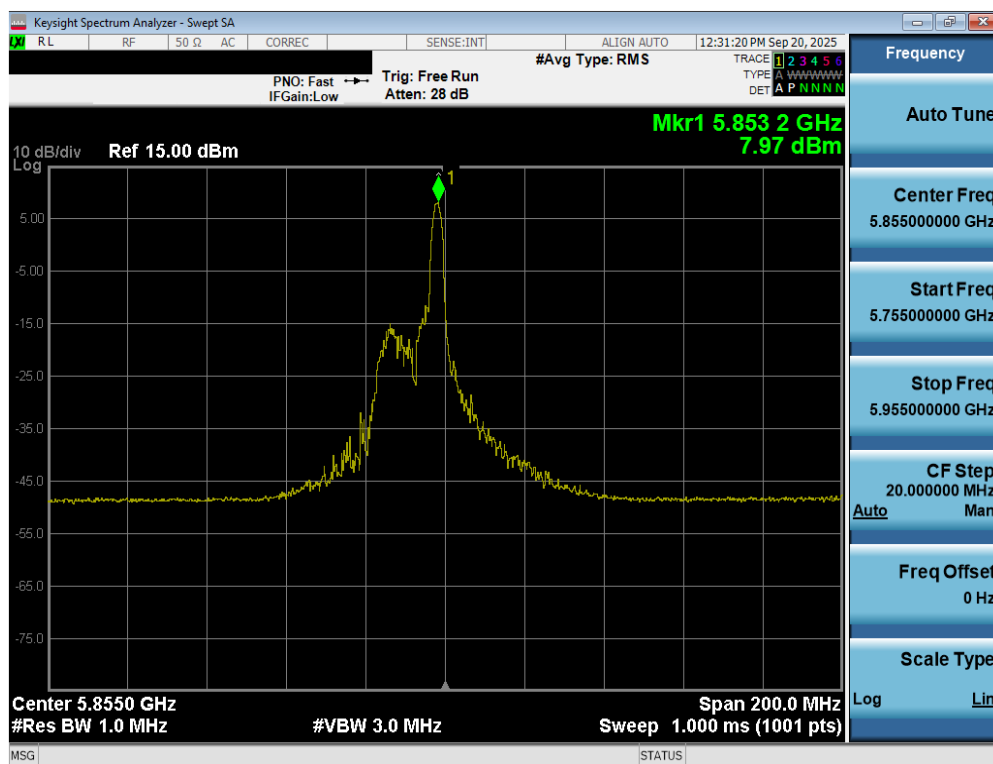
Plot 7-91. Power Spectral Density Plot MIMO ANT2 (80MHz BW 802.11be – 26 Tones (UNII Band 3/4) – Ch. 171)
