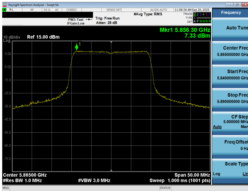
Plot 7-100. Power Spectral Density Plot MIMO ANT2 (20MHz BW 802.11be – 242 Tones (UNII Band 4) – Ch. 173)
