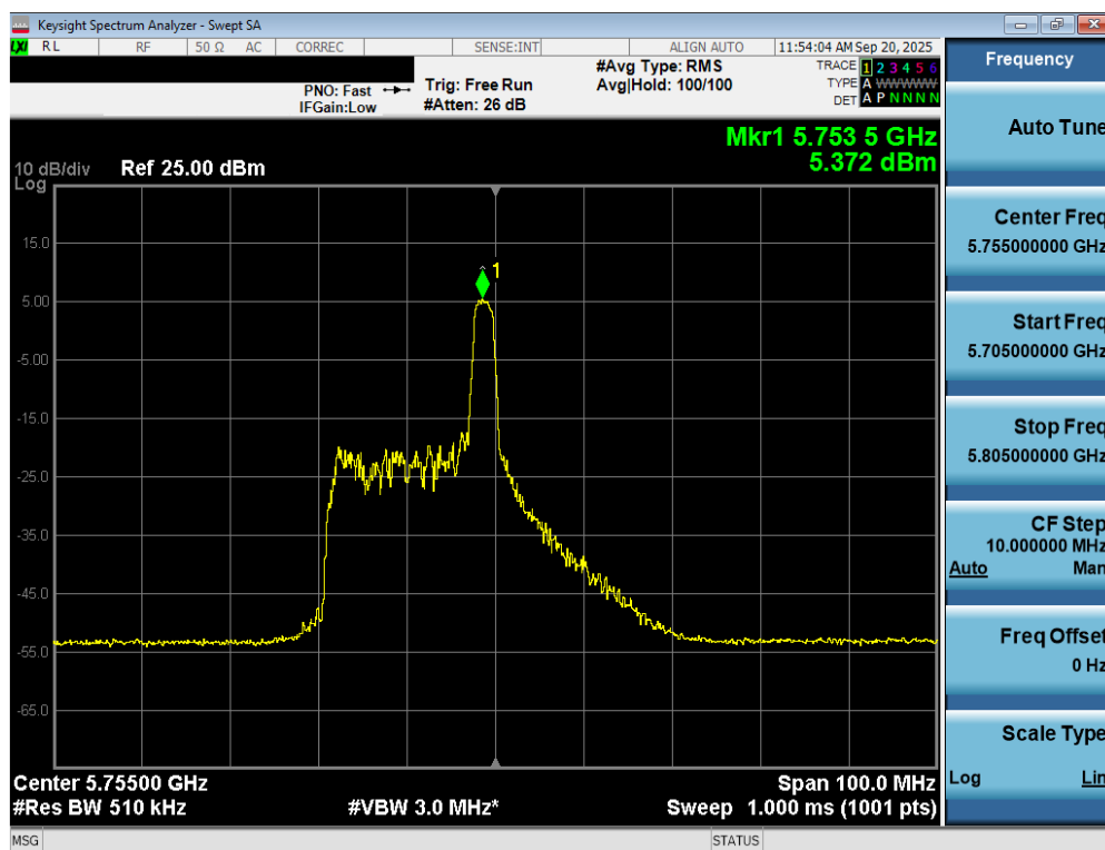
Plot 7-87. Power Spectral Density Plot MIMO ANT2 (40MHz BW 802.11be – 26 Tones (UNII Band 3) – Ch. 151)
