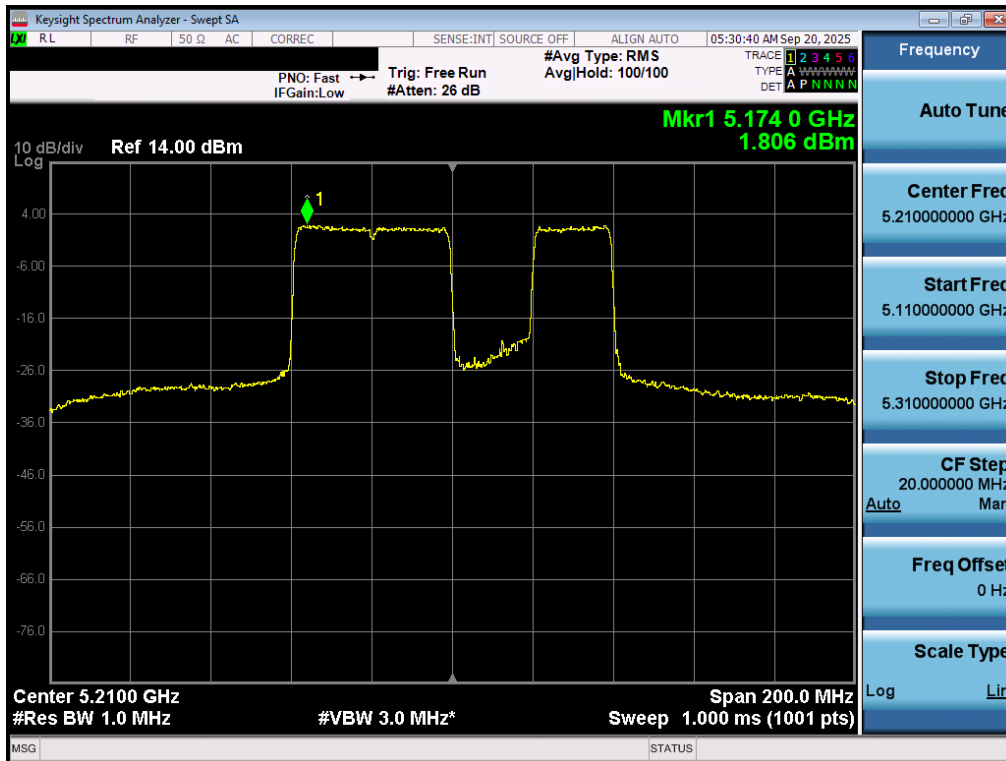
Plot 7-77. Power Spectral Density Plot MIMO ANT1 (80MHz BW 802.11be – 484+242 Tones (UNII Band 1) – Ch. 42)
