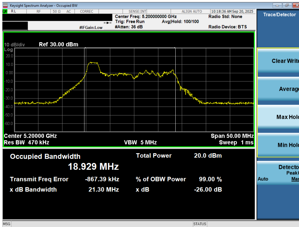
Plot 7-11. 26dB Bandwidth Plot MIMO ANT2 (20MHz BW 802.11be – 26 Tones (UNII Band 1) – Ch. 40)
