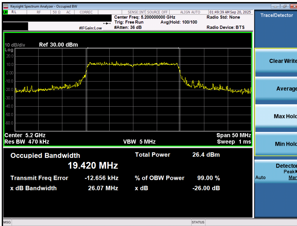
Plot 7-5. 26dB Bandwidth Plot MIMO ANT1 (20MHz BW 802.11be – 242 Tones (UNII Band 1) – Ch. 40)
