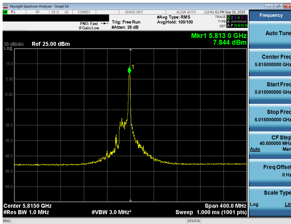
Plot 7-92. Power Spectral Density Plot MIMO ANT2 (160MHz BW 802.11be – 26 Tones (UNII Band 3/4) – Ch. 163)
