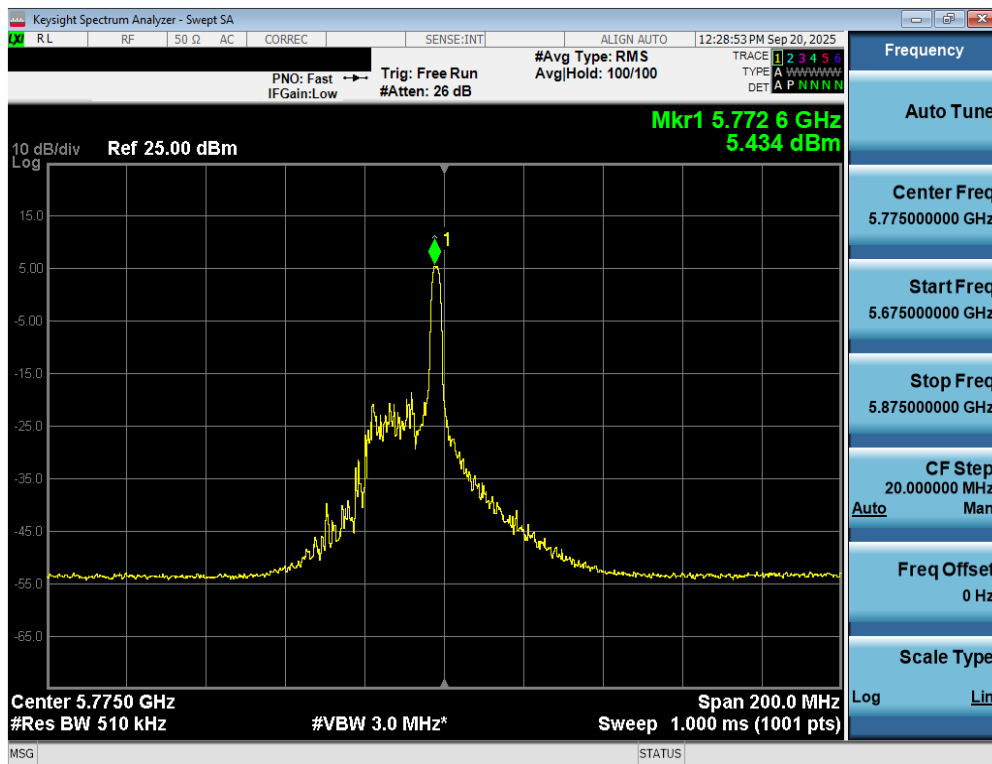
Plot 7-88. Power Spectral Density Plot MIMO ANT2 (80MHz BW 802.11be – 26 Tones (UNII Band 3) – Ch. 155)
