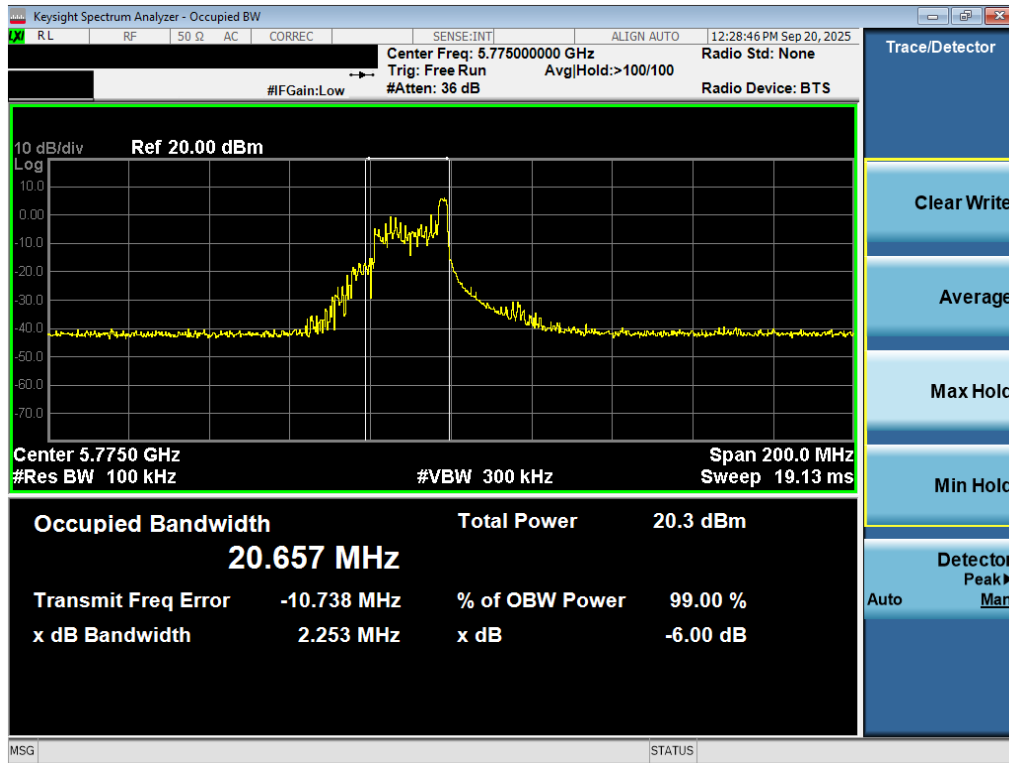
Plot 7-40. 6dB Bandwidth Plot MIMO ANT2 (80MHz BW 802.11be – 26 Tones (UNII Band 3) – Ch. 155)
