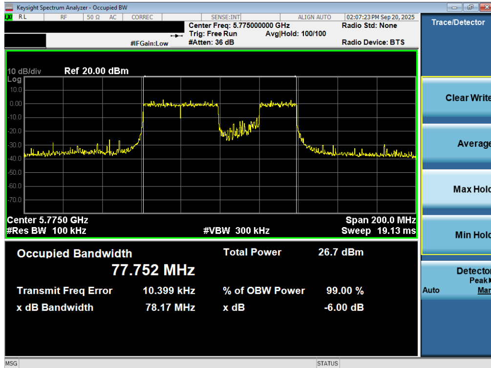
Plot 7-48. 6dB Bandwidth Plot MIMO ANT2 (80MHz BW 802.11be – 484/242 Tones (UNII Band 3) – Ch. 155)
