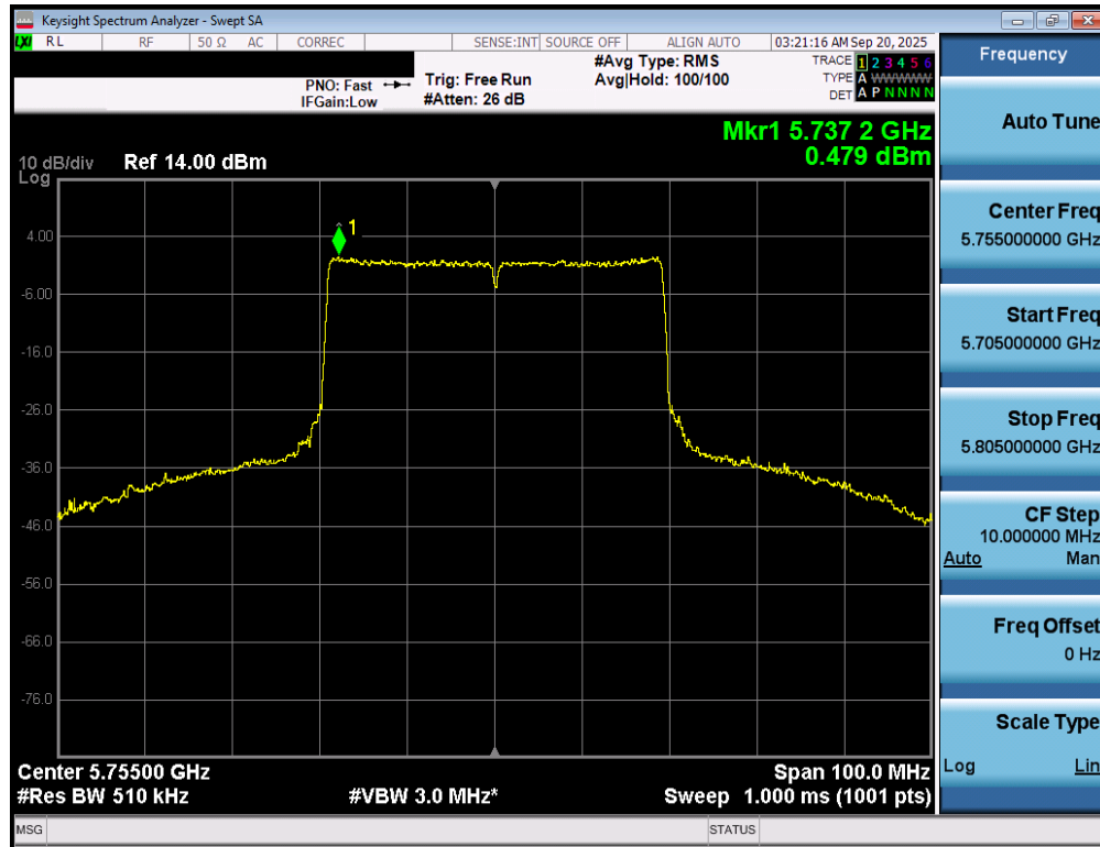
Plot 7-71. Power Spectral Density Plot MIMO ANT1 (40MHz BW 802.11be – 484 Tones (UNII Band 3) – Ch. 151)
