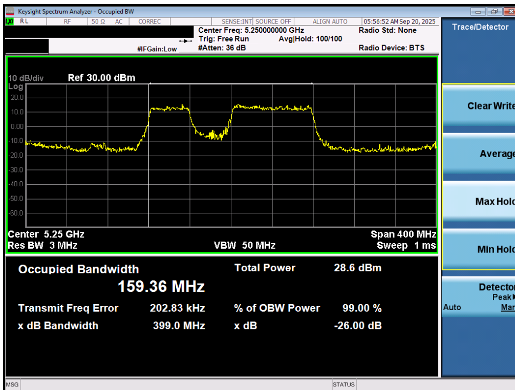
Plot 7-10. 26dB Bandwidth Plot MIMO ANT1 (160MHz BW 802.11be – 996+484 Tones (UNII Band 1/2A) – Ch. 50)
