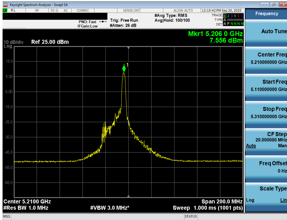
Plot 7-84. Power Spectral Density Plot MIMO ANT2 (80MHz BW 802.11be – 26 Tones (UNII Band 1) – Ch. 42)
