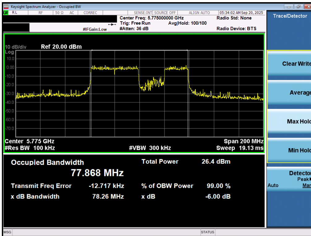
Plot 7-31. 6dB Bandwidth Plot MIMO ANT1 (80MHz BW 802.11be – 484+242 Tones (UNII Band 3) – Ch. 155)
