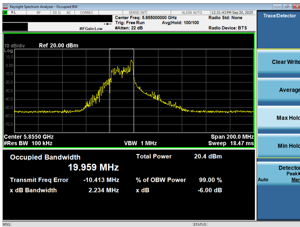
Plot 7-43. 6dB Bandwidth Plot MIMO ANT2 (80MHz BW 802.11be – 26 Tones (UNII Band 3/4) – Ch. 171)
