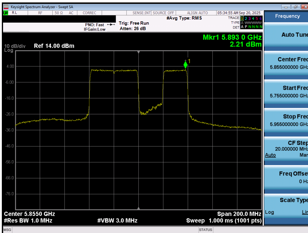
Plot 7-80. Power Spectral Density Plot MIMO ANT1 (80MHz BW 802.11be – 484+242Tones (UNII Band 3/4) – Ch. 171)
