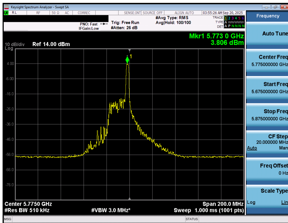
Plot 7-61. Power Spectral Density Plot MIMO ANT1 (80MHz BW 802.11be – 26 Tones (UNII Band 3) – Ch. 155)
