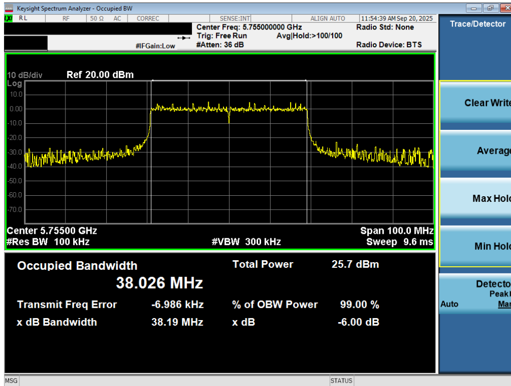
Plot 7-46. 6dB Bandwidth Plot MIMO ANT2 (40MHz BW 802.11be – 484 Tones (UNII Band 3) – Ch. 151)
