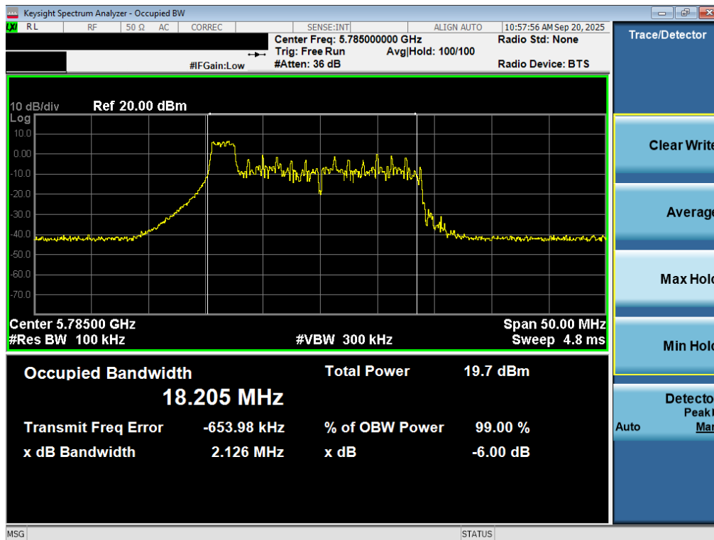
Plot 7-38. 6dB Bandwidth Plot MIMO ANT2 (20MHz BW 802.11be – 26 Tones (UNII Band 3) – Ch. 157)
