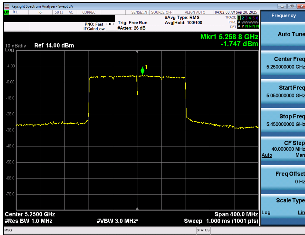
Plot 7-69. Power Spectral Density Plot MIMO ANT1 (160MHz BW 802.11be – 2x996 Tones (UNII Band 1/2A) – Ch. 50)
