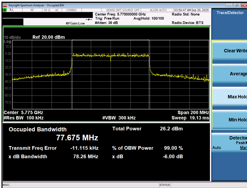
Plot 7-30. 6dB Bandwidth Plot MIMO ANT1 (80MHz BW 802.11be – 996 Tones (UNII Band 3) – Ch. 155)
