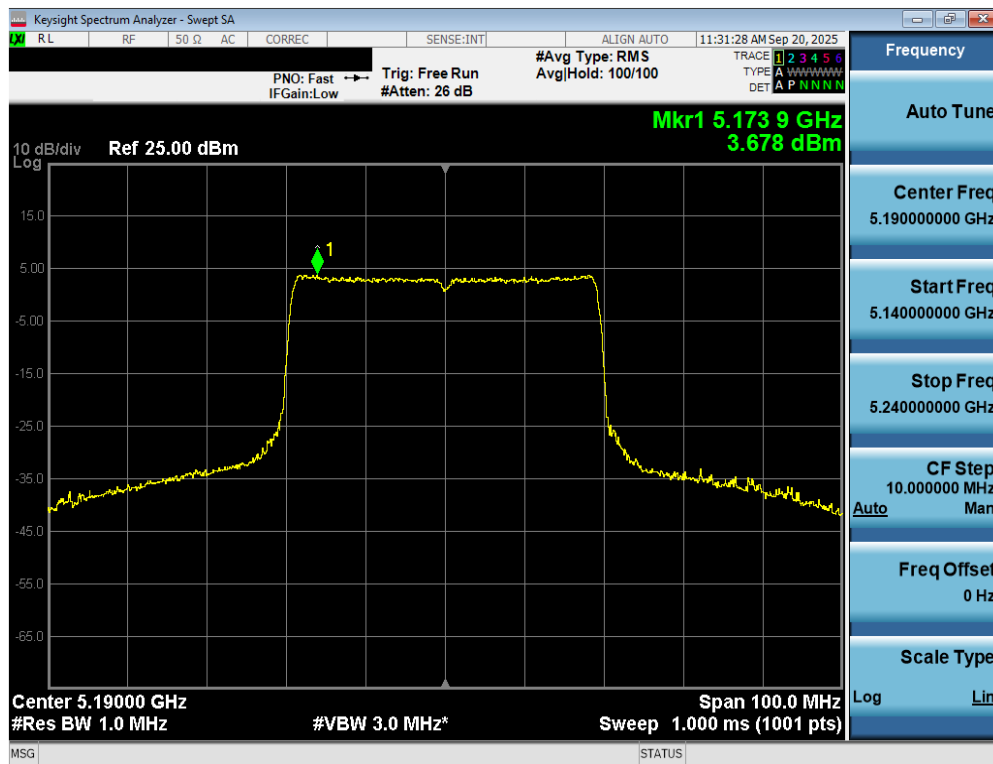
Plot 7-94. Power Spectral Density Plot MIMO ANT2 (40MHz BW 802.11be – 484 Tones (UNII Band 1) – Ch. 38)
