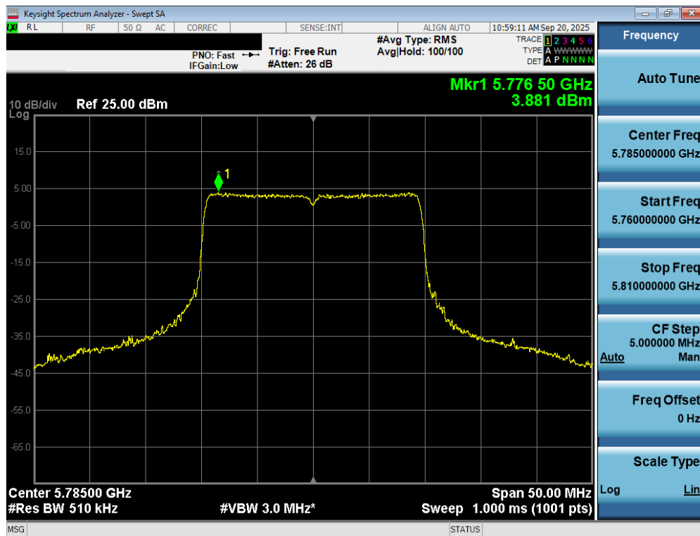
Plot 7-97. Power Spectral Density Plot MIMO ANT2 (20MHz BW 802.11be – 242 Tones (UNII Band 3) – Ch. 157)
