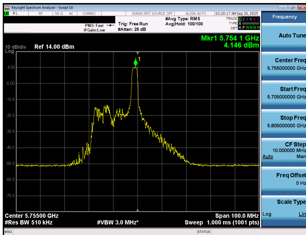
Plot 7-60. Power Spectral Density Plot MIMO ANT1 (40MHz BW 802.11be – 26 Tones (UNII Band 3) – Ch. 151)
