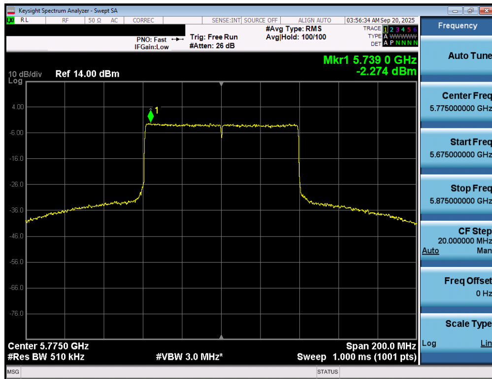
Plot 7-72. Power Spectral Density Plot MIMO ANT1 (80MHz BW 802.11be – 996 Tones (UNII Band 3) – Ch. 155)
