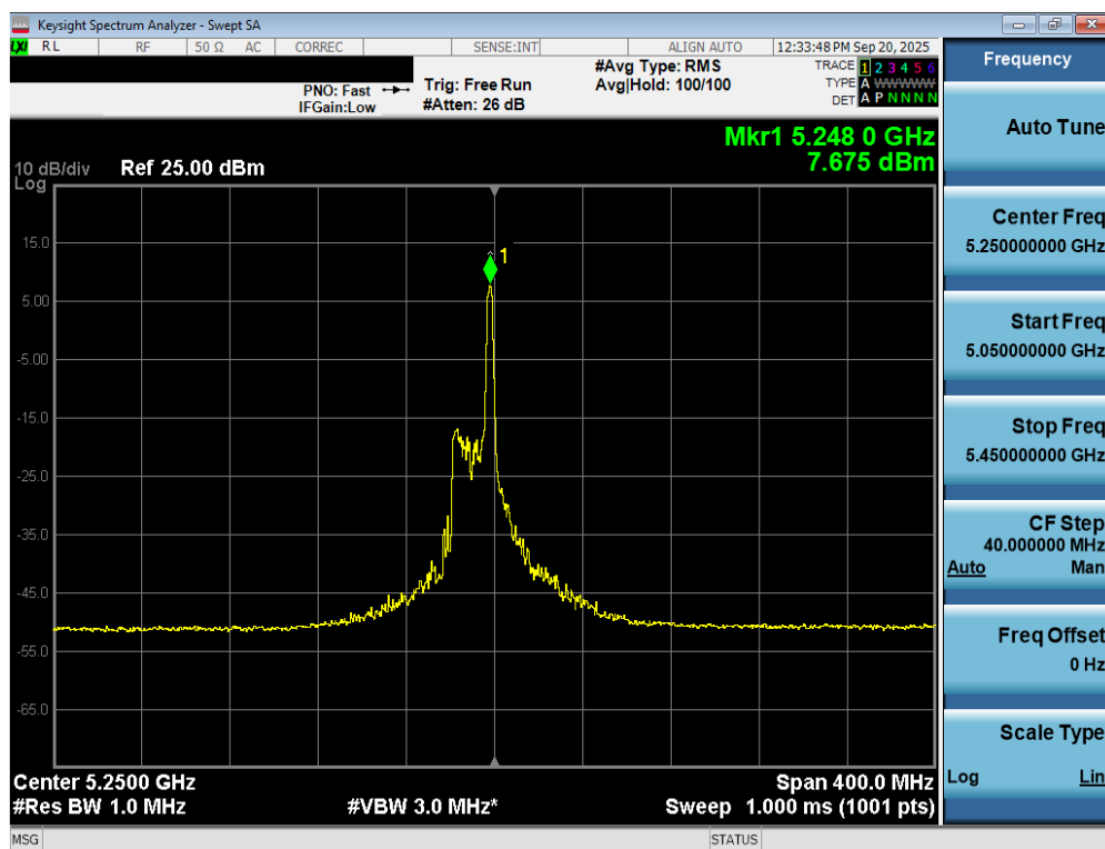
Plot 7-85. Power Spectral Density Plot MIMO ANT2 (160MHz BW 802.11be – 26 Tones (UNII Band 1/2A) – Ch. 50)
