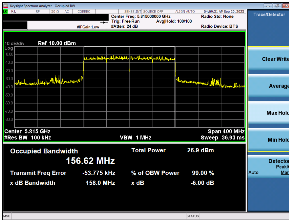
Plot 7-35. 6dB Bandwidth Plot MIMO ANT1 (160MHz BW 802.11be – 996*2 Tones (UNII Band 3/4) – Ch. 163)
