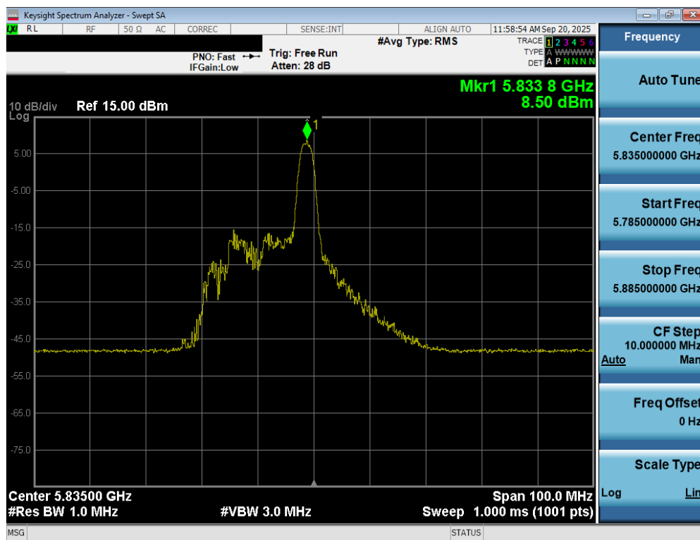
Plot 7-90. Power Spectral Density Plot MIMO ANT2 (40MHz BW 802.11be – 26 Tones (UNII Band 3/4) – Ch. 167)
