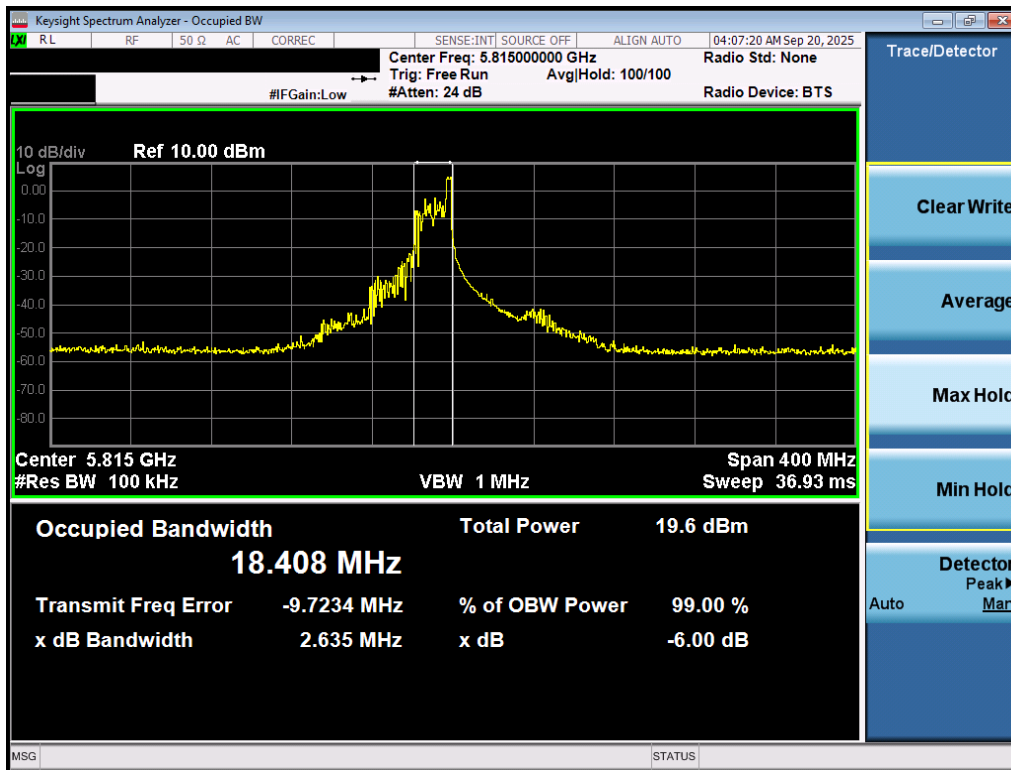
Plot 7-27. 6dB Bandwidth Plot MIMO ANT1 (160MHz BW 802.11be – 26 Tones (UNII Band 3/4) – Ch. 163)
