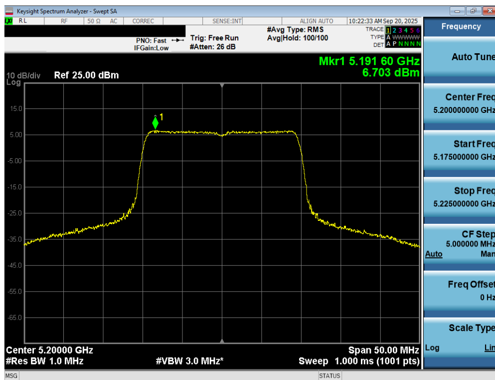
Plot 7-93. Power Spectral Density Plot MIMO ANT2 (20MHz BW 802.11be – 242 Tones (UNII Band 1) – Ch. 40)
