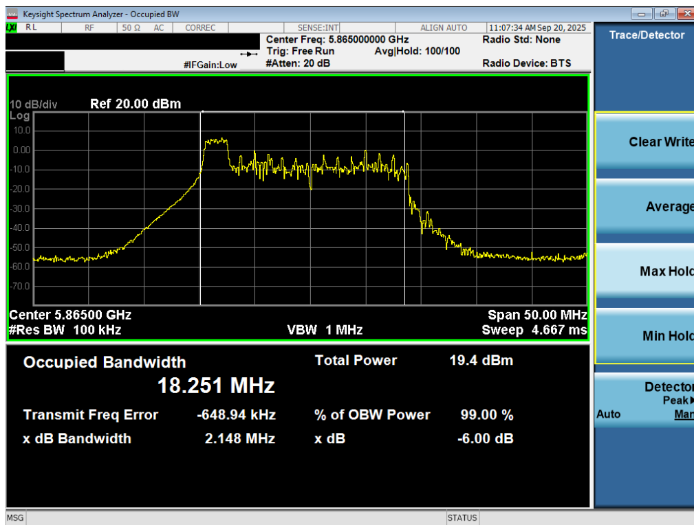
Plot 7-41. 6dB Bandwidth Plot MIMO ANT2 (20MHz BW 802.11be – 26 Tones (UNII Band 4) – Ch. 173)
