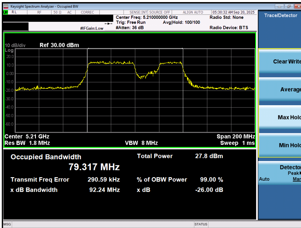
Plot 7-9. 26dB Bandwidth Plot MIMO ANT1 (80MHz BW 802.11be – 484+242 Tones (UNII Band 1) – Ch. 42)
