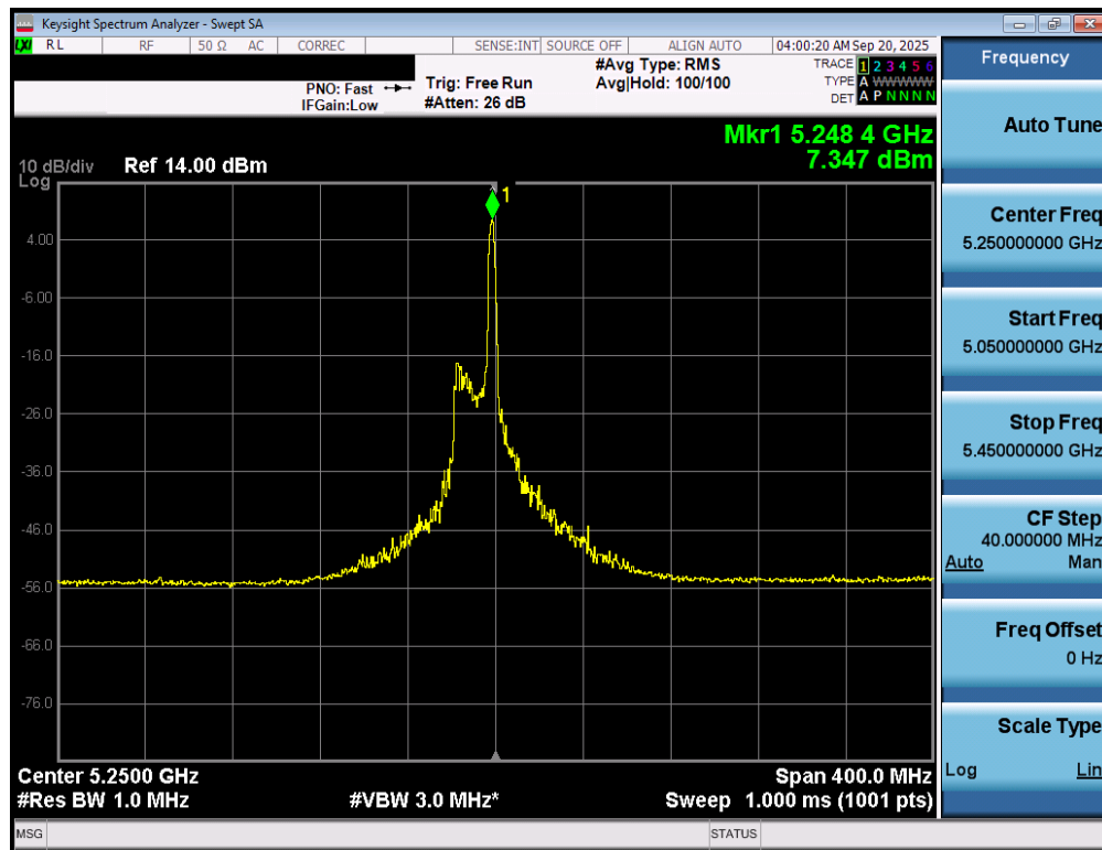
Plot 7-58. Power Spectral Density Plot MIMO ANT1 (160MHz BW 802.11be – 26 Tones (UNII Band 1/2A) – Ch. 50)
