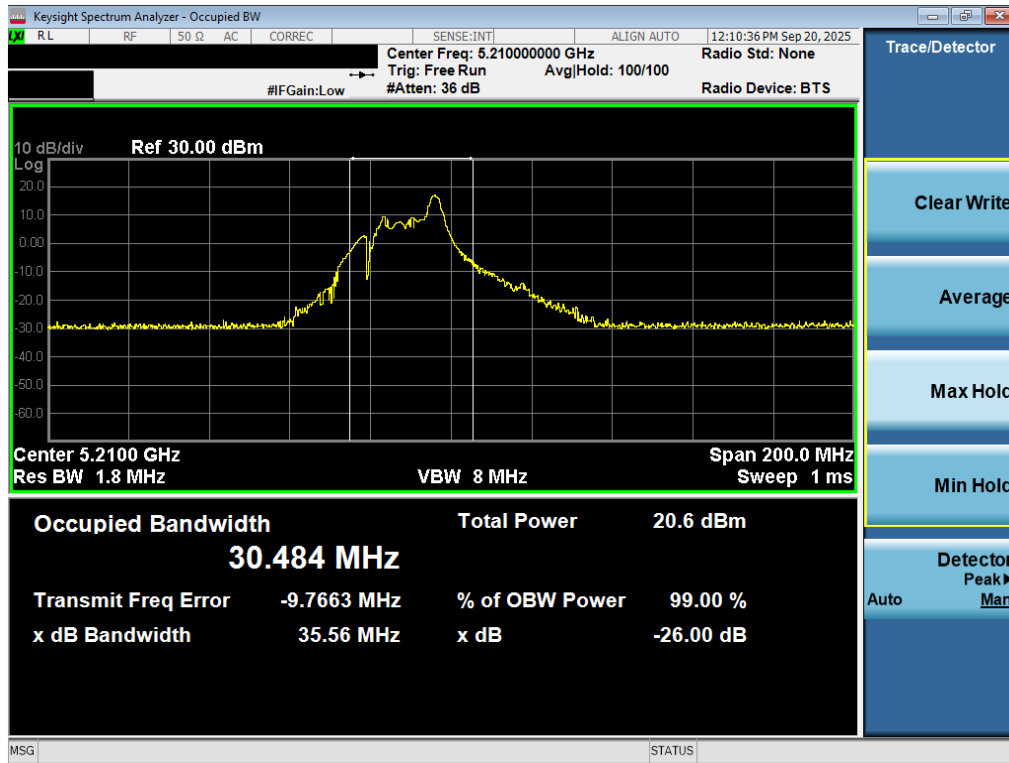
Plot 7-13. 26dB Bandwidth Plot MIMO ANT2 (80MHz BW 802.11be – 26 Tones (UNII Band 1) – Ch. 42)
