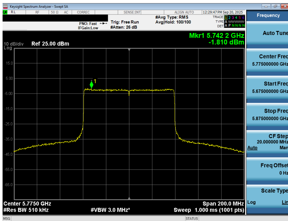
Plot 7-99. Power Spectral Density Plot MIMO ANT2 (80MHz BW 802.11be – 996 Tones (UNII Band 3) – Ch. 155)
