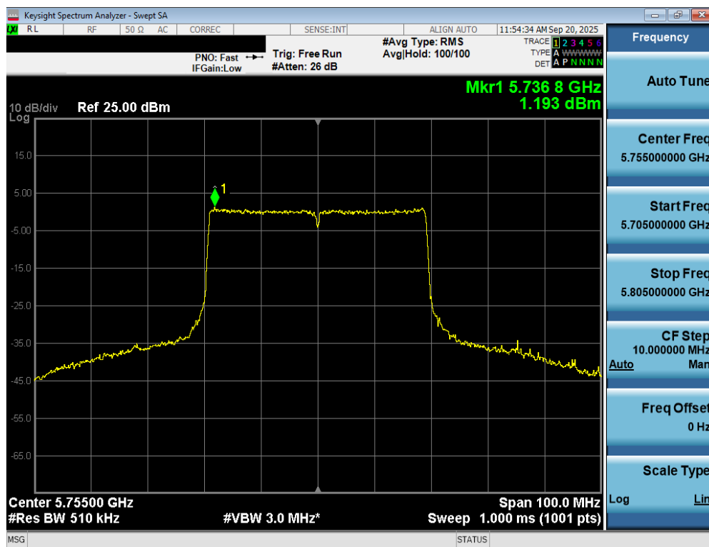
Plot 7-98. Power Spectral Density Plot MIMO ANT2 (40MHz BW 802.11be – 484 Tones (UNII Band 3) – Ch. 151)
