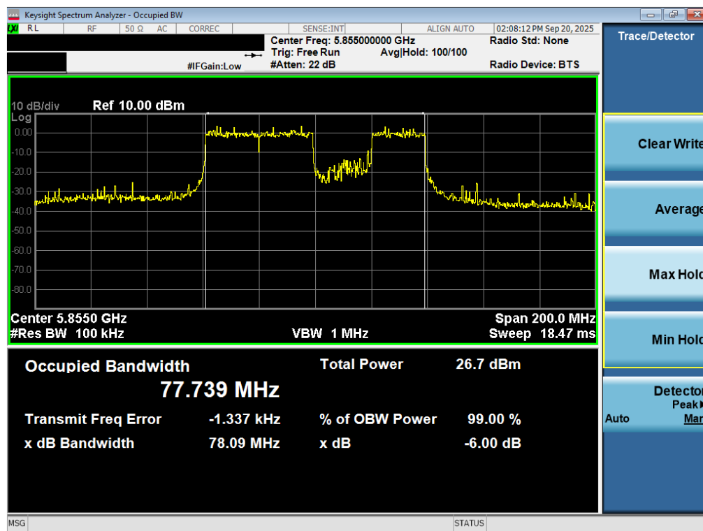
Plot 7-53. 6dB Bandwidth Plot MIMO ANT2 (80MHz BW 802.11be – 484+242 Tones (UNII Band 3/4) – Ch. 171)
