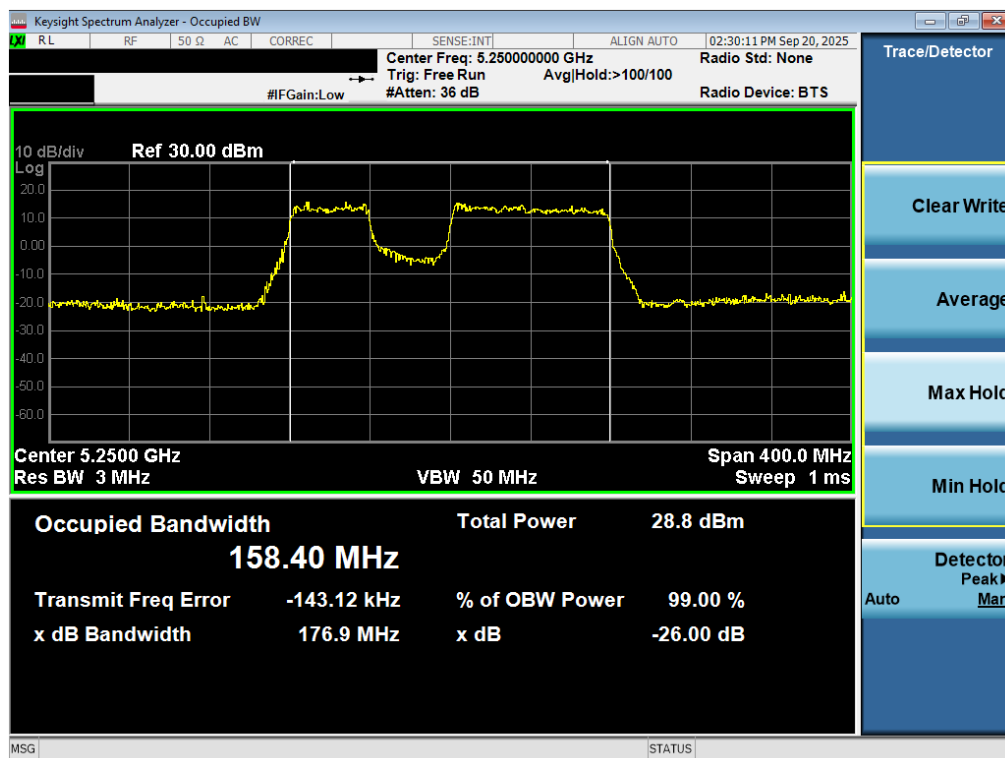
Plot 7-20. 26dB Bandwidth Plot MIMO ANT2 (160MHz BW 802.11be – 996+484 Tones (UNII Band 1/2A) – Ch. 50)
