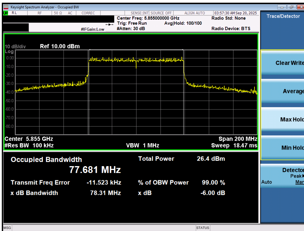
Plot 7-34. 6dB Bandwidth Plot MIMO ANT1 (80MHz BW 802.11be – 996 Tones (UNII Band 3/4) – Ch. 171)
