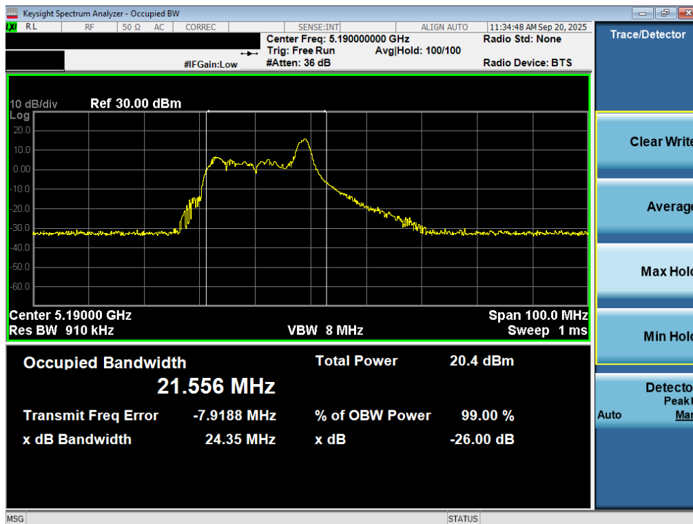
Plot 7-12. 26dB Bandwidth Plot MIMO ANT2 (40MHz BW 802.11be – 26 Tones (UNII Band 1) – Ch. 38)
