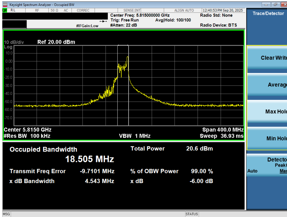
Plot 7-44. 6dB Bandwidth Plot MIMO ANT2 (160MHz BW 802.11be – 26 Tones (UNII Band 3/4) – Ch. 163)
