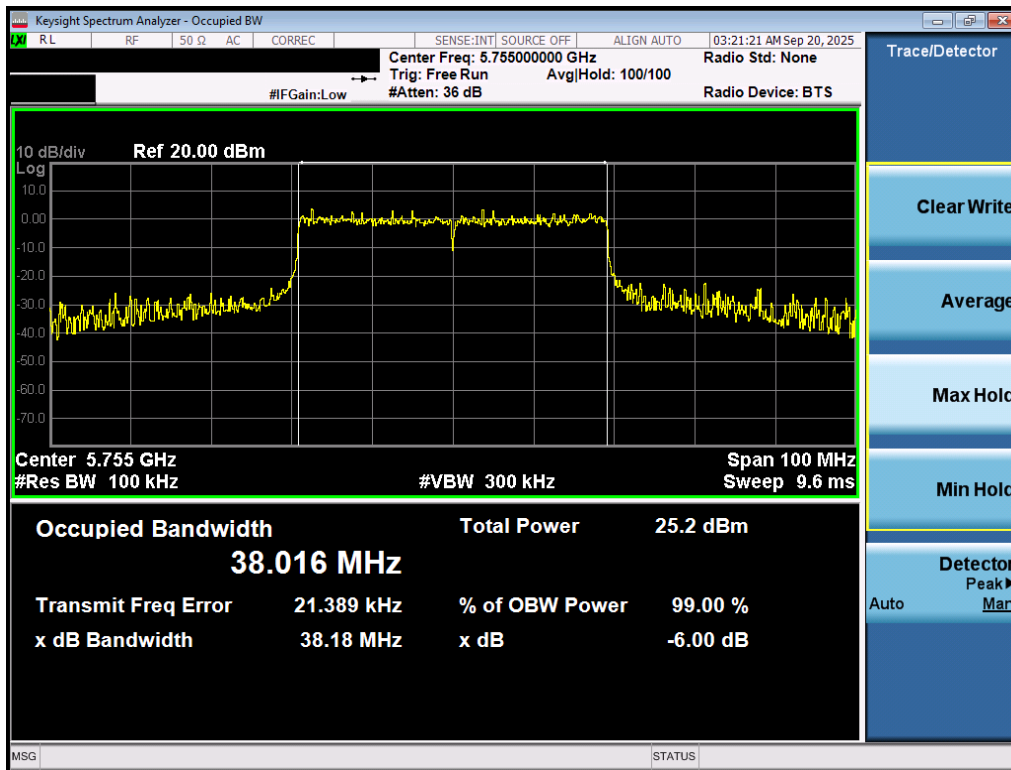
Plot 7-29. 6dB Bandwidth Plot MIMO ANT1 (40MHz BW 802.11be – 484 Tones (UNII Band 3) – Ch. 151)
