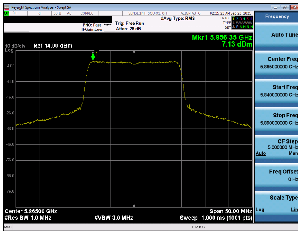
Plot 7-73. Power Spectral Density Plot MIMO ANT1 (20MHz BW 802.11be – 242 Tones (UNII Band 4) – Ch. 173)
