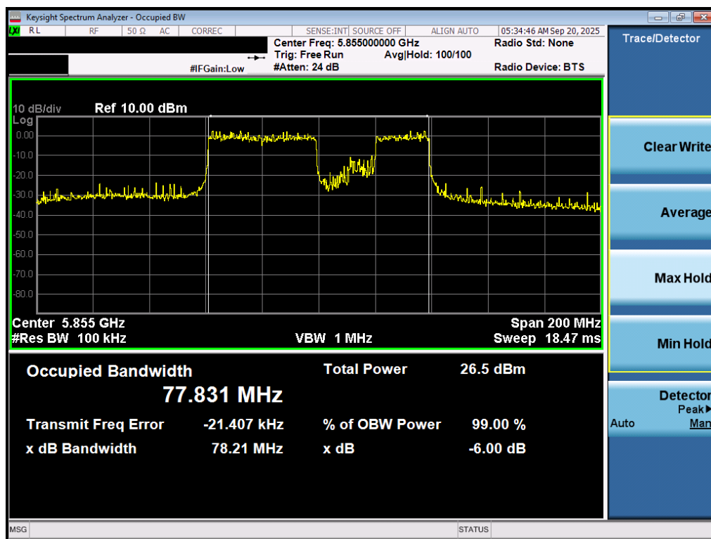
Plot 7-36. 6dB Bandwidth Plot MIMO ANT1 (80MHz BW 802.11be – 484+242 Tones (UNII Band 3/4) – Ch. 171)
