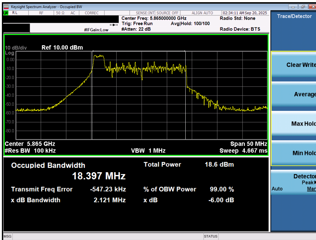
Plot 7-24. 6dB Bandwidth Plot MIMO ANT1 (20MHz BW 802.11be – 26 Tones (UNII Band 4) – Ch. 173)
