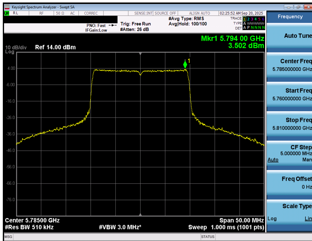
Plot 7-70. Power Spectral Density Plot MIMO ANT1 (20MHz BW 802.11be – 242 Tones (UNII Band 3) – Ch. 157)
