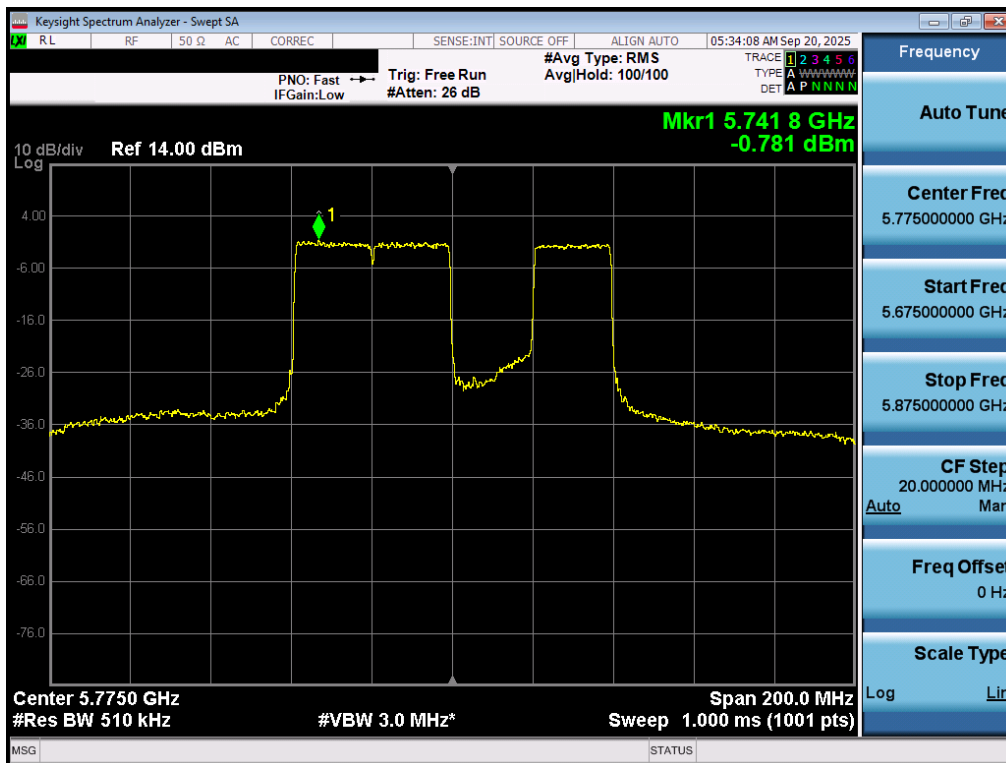
Plot 7-79. Power Spectral Density Plot MIMO ANT1 (80MHz BW 802.11be – 484+242 Tones (UNII Band 3) – Ch. 155)
