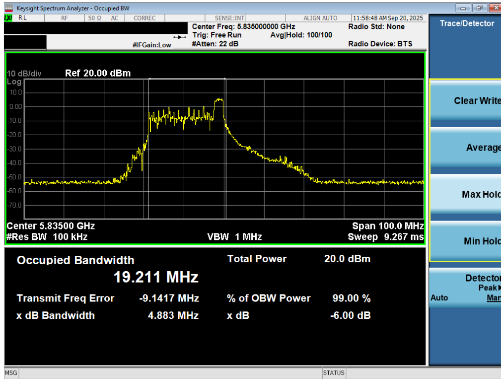
Plot 7-42. 6dB Bandwidth Plot MIMO ANT2 (40MHz BW 802.11be – 26 Tones (UNII Band 3/4) – Ch. 167)
