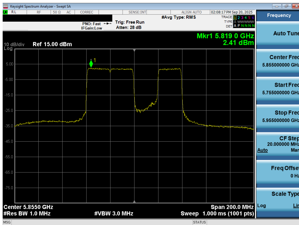
Plot 7-107. Power Spectral Density Plot MIMO ANT2 (80MHz BW 802.11be – 484+242Tones (UNII Band 3/4) – Ch. 171)
