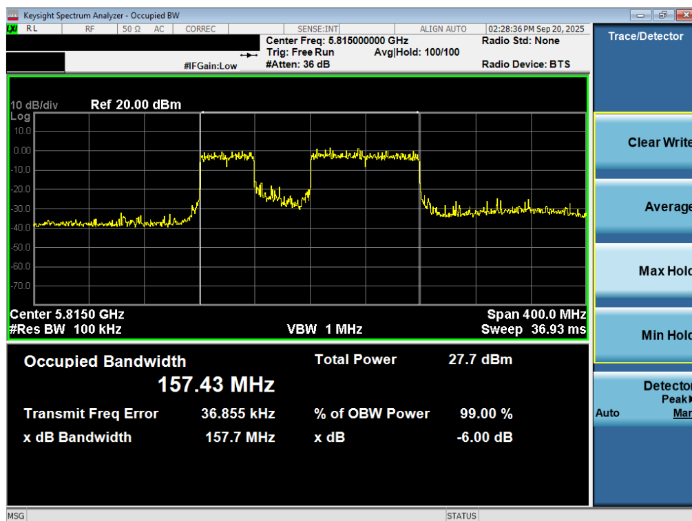
Plot 7-54. 6dB Bandwidth Plot MIMO ANT2 (160MHz BW 802.11be – 996+484 Tones (UNII Band 3/4) – Ch. 163)
