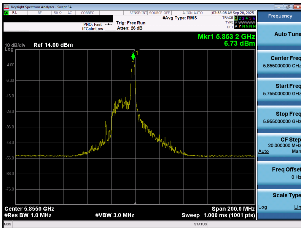
Plot 7-64. Power Spectral Density Plot MIMO ANT1 (80MHz BW 802.11be – 26 Tones (UNII Band 3/4) – Ch. 171)
