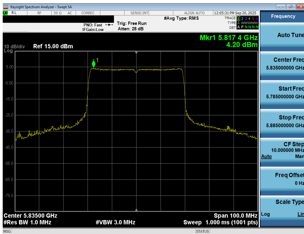
Plot 7-101. Power Spectral Density Plot MIMO ANT2 (40MHz BW 802.11be – 484 Tones (UNII Band 3/4) – Ch. 167)
