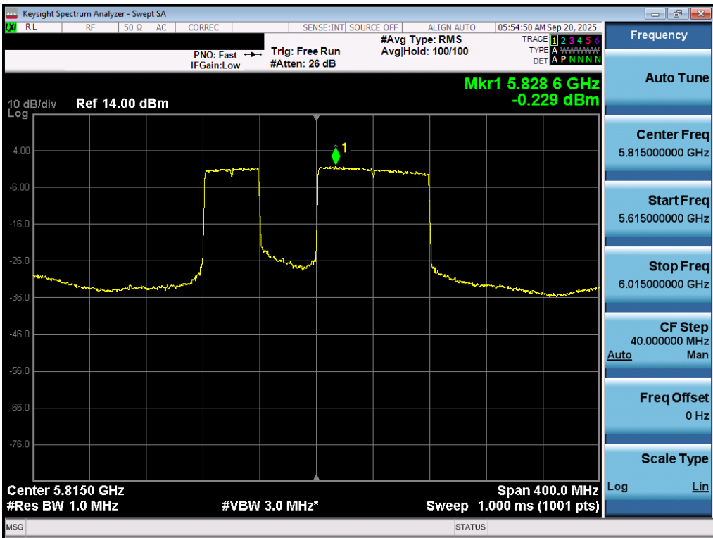
Plot 7-81. Power Spectral Density Plot MIMO ANT1 (160MHz BW 802.11be – 996+484 Tones (UNII Band 3/4) – Ch. 163)
