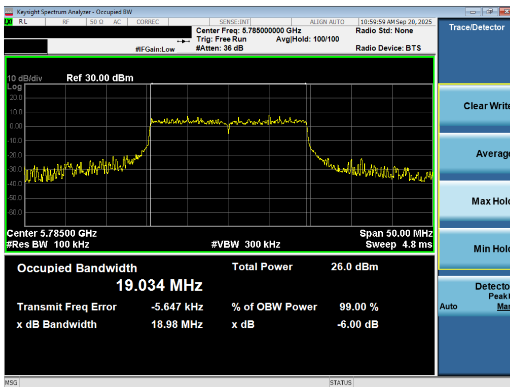
Plot 7-45. 6dB Bandwidth Plot MIMO ANT2 (20MHz BW 802.11be – 242 Tones (UNII Band 3) – Ch. 157)
