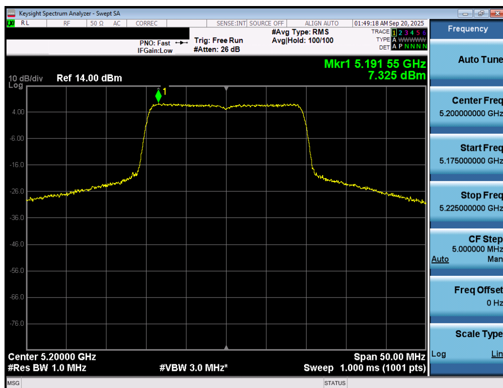
Plot 7-66. Power Spectral Density Plot MIMO ANT1 (20MHz BW 802.11be – 242 Tones (UNII Band 1) – Ch. 40)
