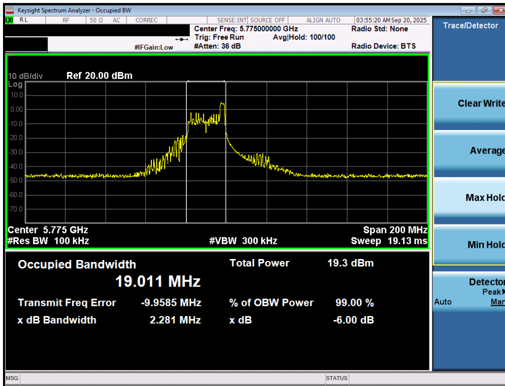
Plot 7-23. 6dB Bandwidth Plot MIMO ANT1 (80MHz BW 802.11be – 26 Tones (UNII Band 3) – Ch. 155)
