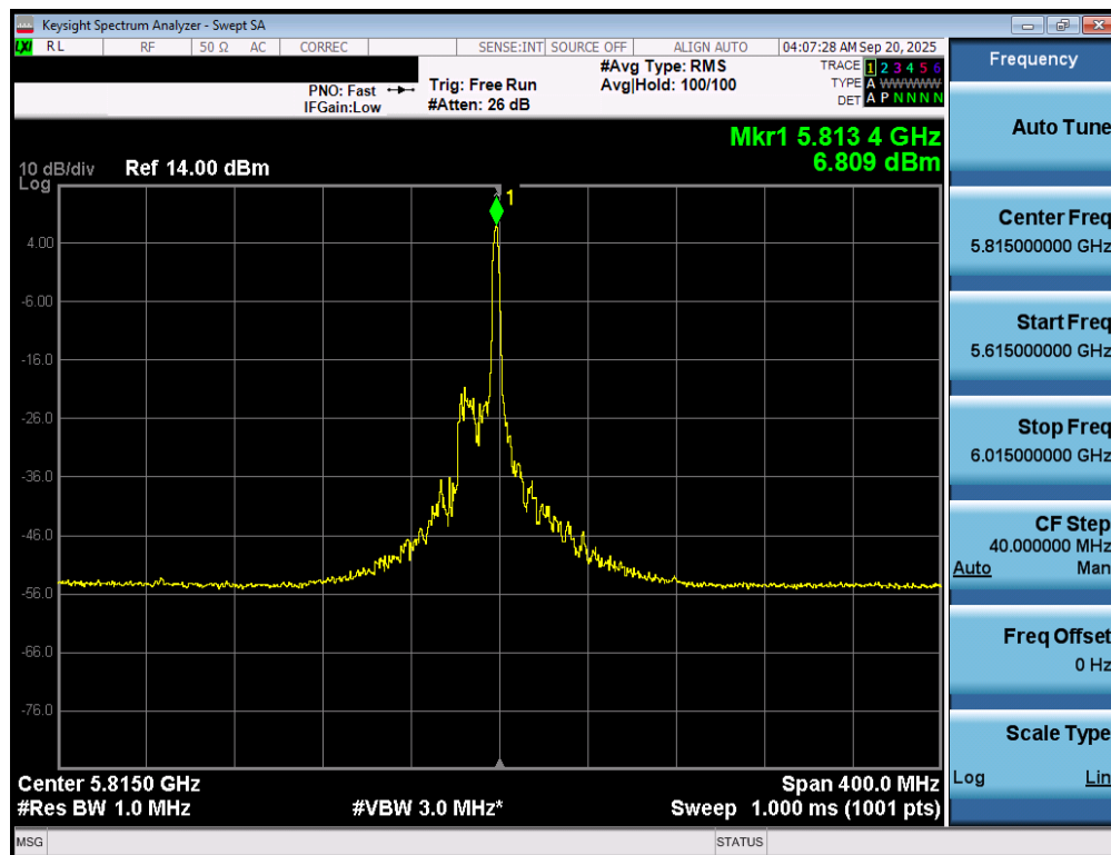
Plot 7-65. Power Spectral Density Plot MIMO ANT1 (160MHz BW 802.11be – 26 Tones (UNII Band 3/4) – Ch. 163)
