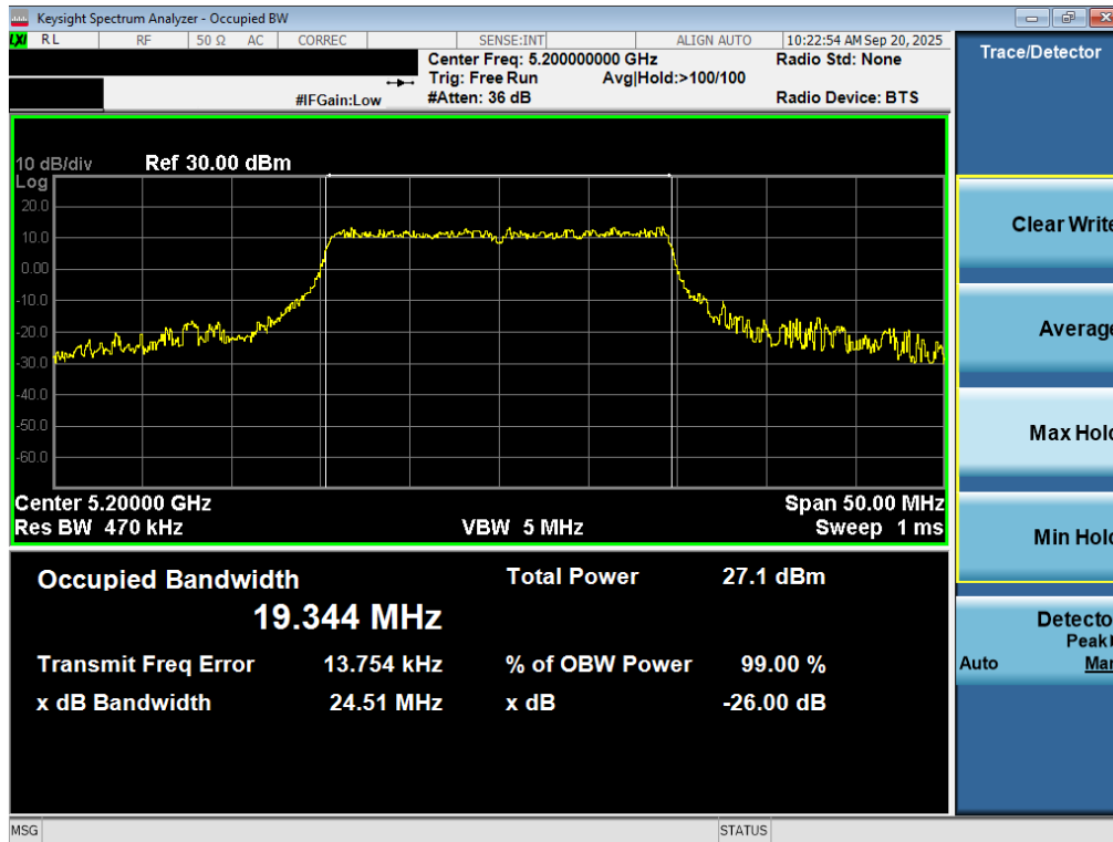
Plot 7-15. 26dB Bandwidth Plot MIMO ANT2 (20MHz BW 802.11be – 242 Tones (UNII Band 1) – Ch. 40)
