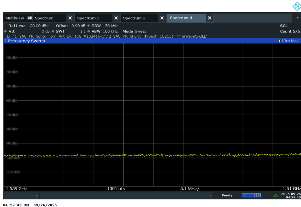
Plot 7-43. Radiated Spurious Pre-Scan 1559 - 1610 MHz - CH.5 – GPS band
