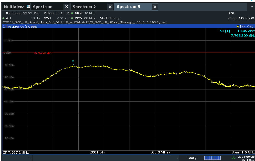
Plot 7-37. UWB Peak Power Measurement - CH.9 – HPRF
