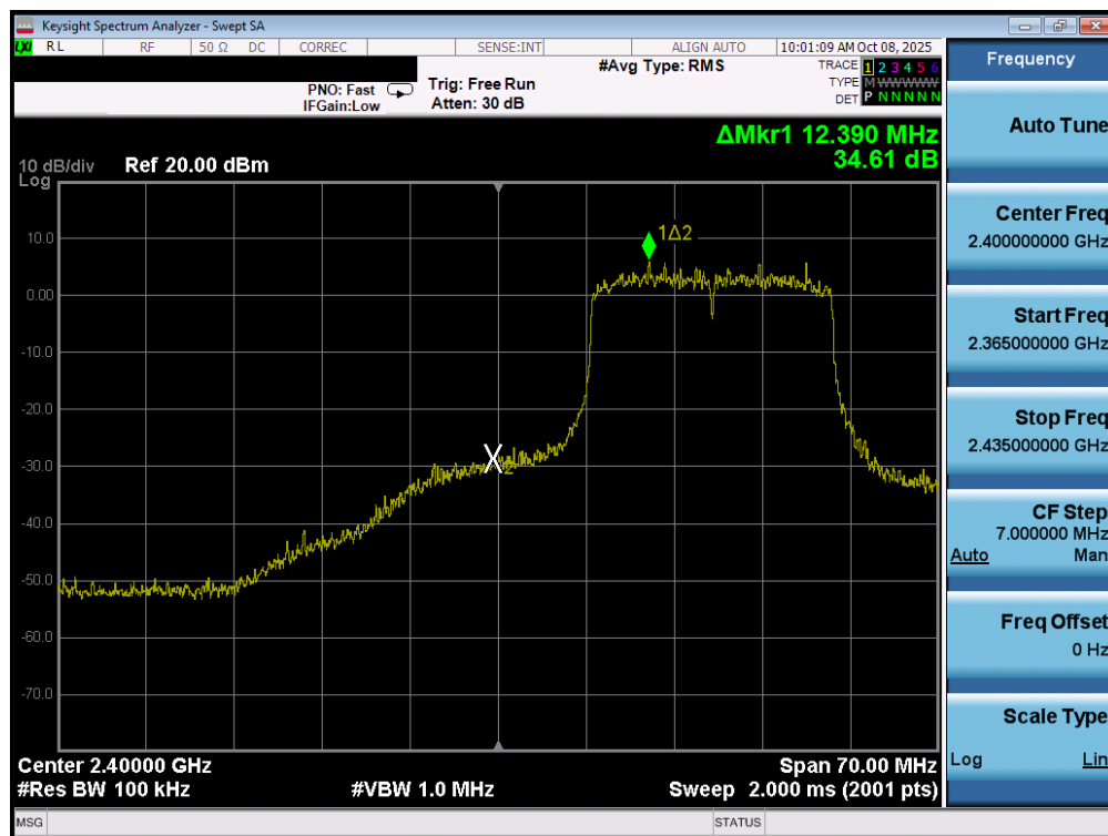
Plot 7-72. Band Edge Plot MIMO ANT2 (802.11ax/be (2.4GHz) – Ch. 2)
