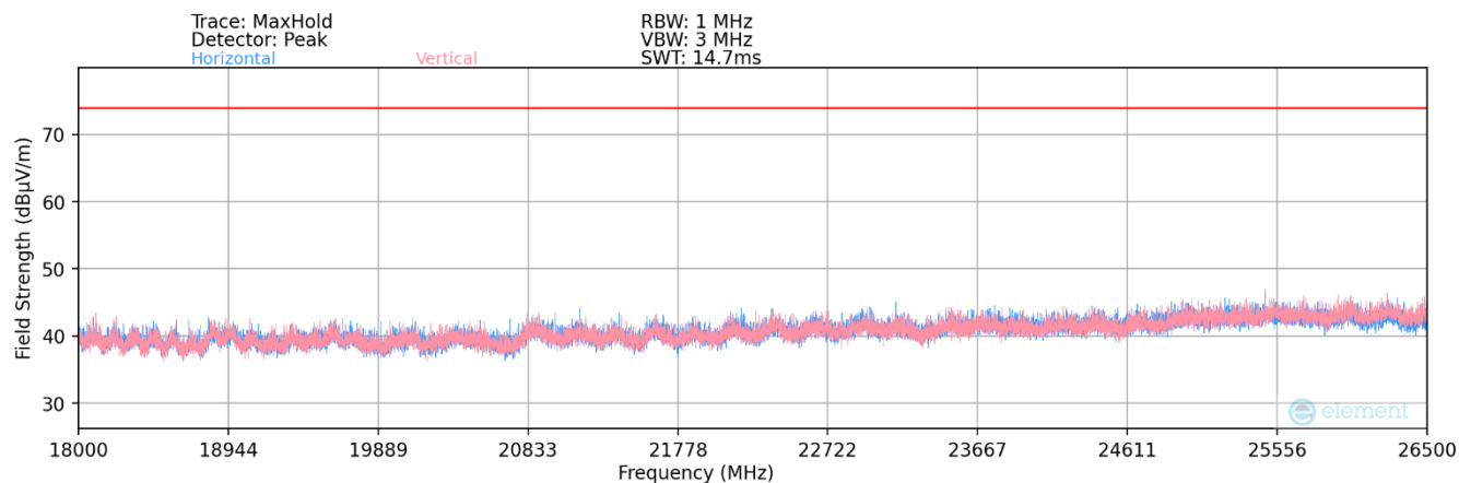
Plot 7-91. Radiated Spurious Plot above 18GHz MIMO
