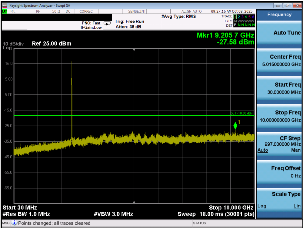
Plot 7-83. Conducted Spurious Plot SISO ANT2 (802.11b – Ch. 6)
