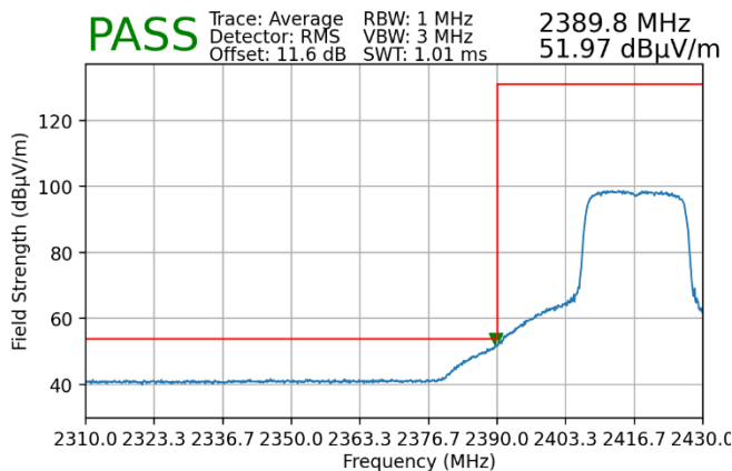
Plot 7-94. Radiated Restricted Lower Band Edge Measurement MIMO (Average)
