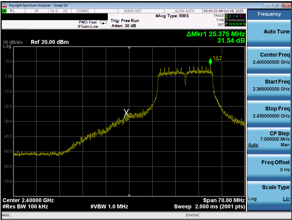
Plot 7-52. Band Edge Plot MIMO ANT1 (802.11g- Ch. 2)
