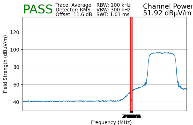
Plot 7-92. Radiated Restricted Lower Band Edge Measurement MIMO (Average)
