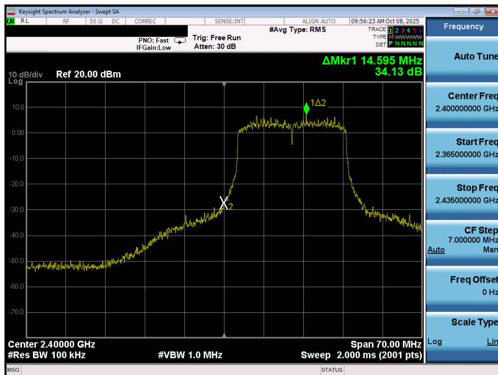
Plot 7-58. Band Edge Plot MIMO ANT1 (802.11ax/be (2.4GHz) – Ch. 1)
