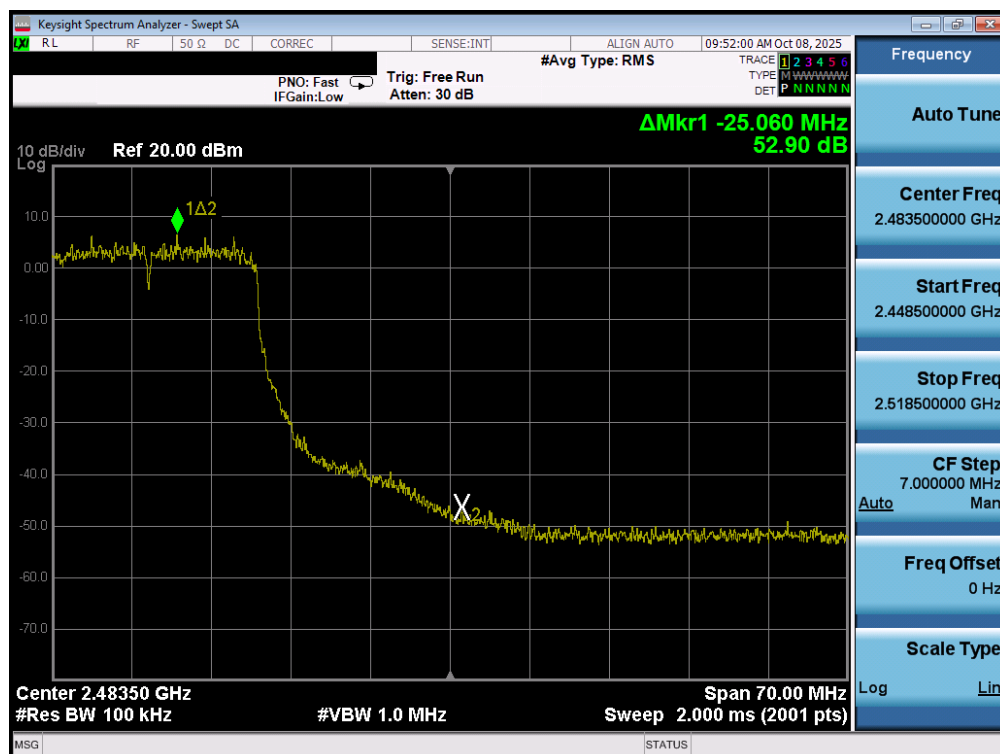
Plot 7-60. Band Edge Plot MIMO ANT1 (802.11ax/be (2.4GHz) – Ch. 10)
