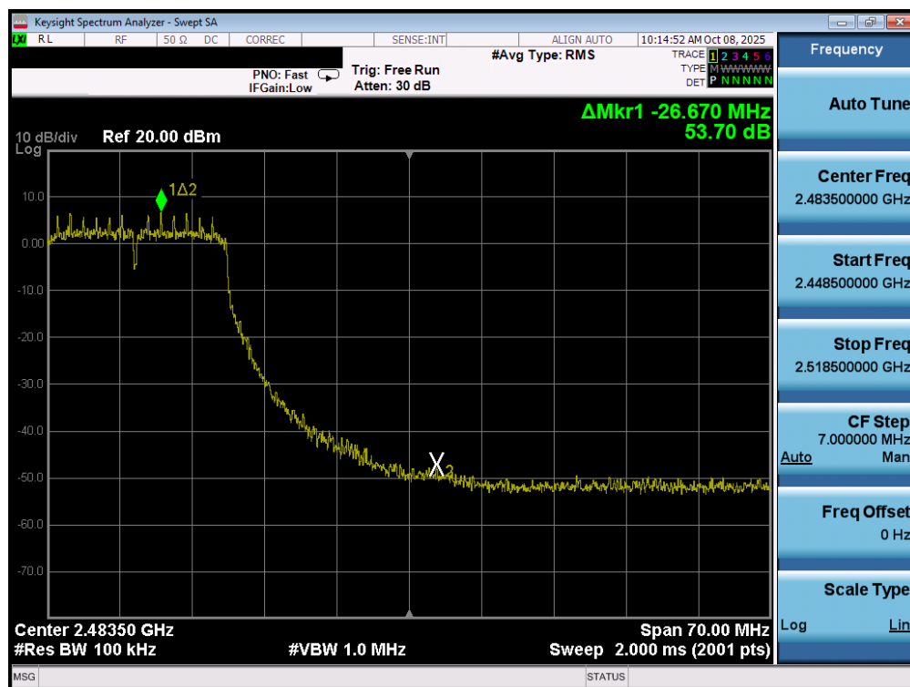
Plot 7-56. Band Edge Plot MIMO ANT1 (802.11n/ac (2.4GHz) – Ch. 10)
