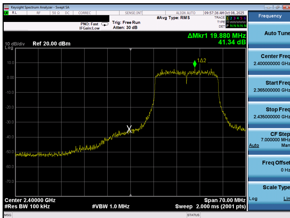
Plot 7-59. Band Edge Plot MIMO ANT1 (802.11ax/be (2.4GHz) – Ch. 2)
