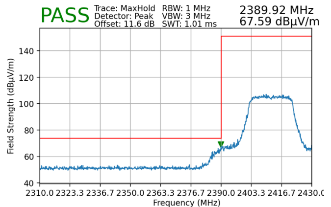
Plot 7-93. Radiated Restricted Lower Band Edge Measurement MIMO (Peak)
