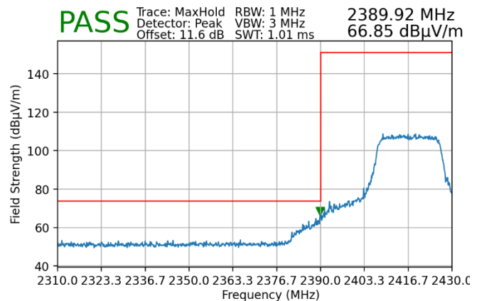
Plot 7-95. Radiated Restricted Lower Band Edge Measurement MIMO (Peak)
