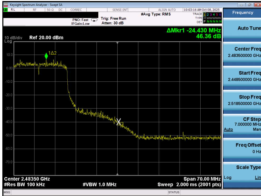
Plot 7-73. Band Edge Plot MIMO ANT2 (802.11ax/be (2.4GHz) – Ch. 10)
