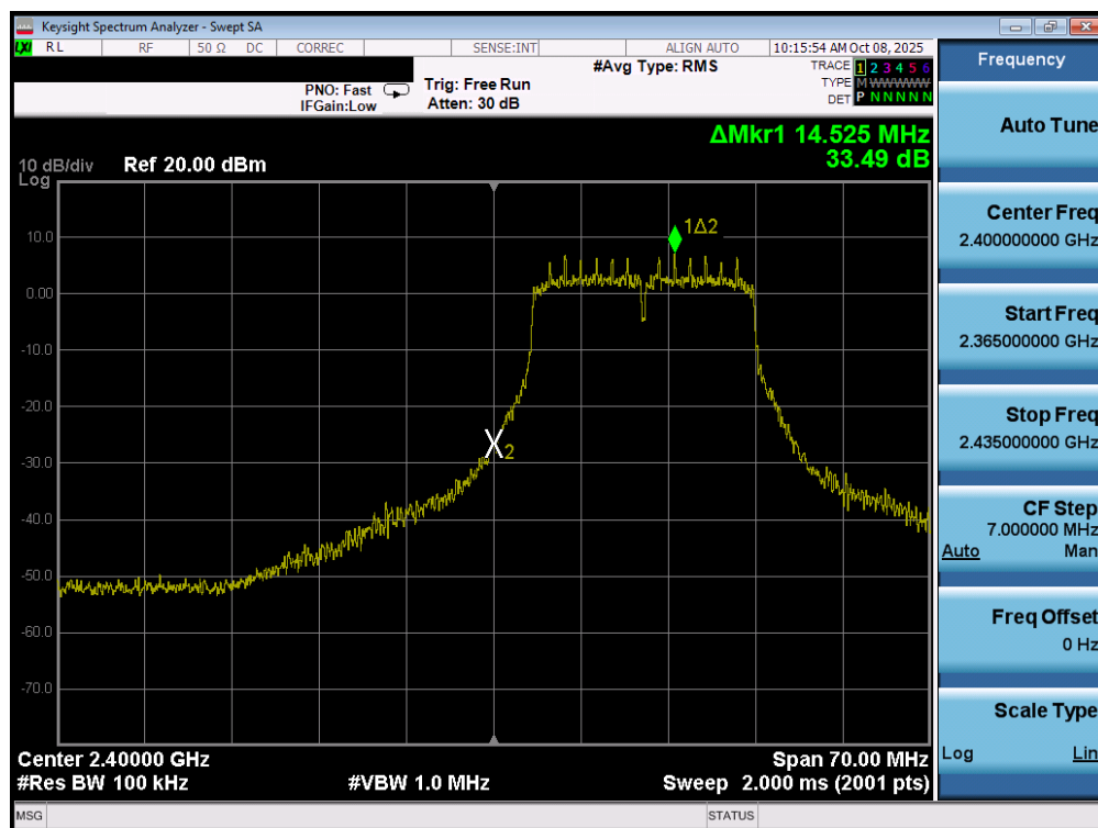
Plot 7-54. Band Edge Plot MIMO ANT1 (802.11n/ac (2.4GHz) – Ch. 1)
