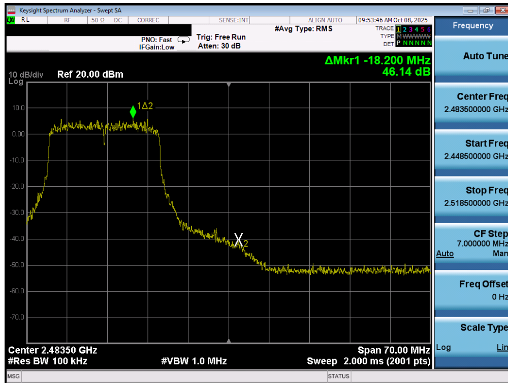
Plot 7-61. Band Edge Plot MIMO ANT1 (802.11ax/be (2.4GHz) – Ch. 11)
