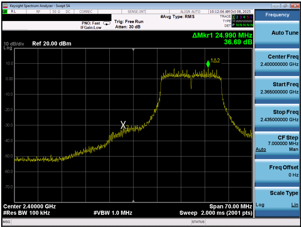
Plot 7-68. Band Edge Plot MIMO ANT2 (802.11n/ac (2.4GHz) – Ch. 2)
