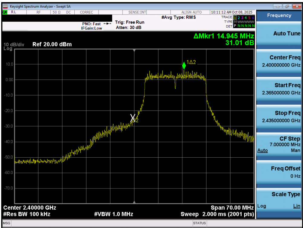
Plot 7-67. Band Edge Plot MIMO ANT2 (802.11n/ac (2.4GHz) – Ch. 1)
