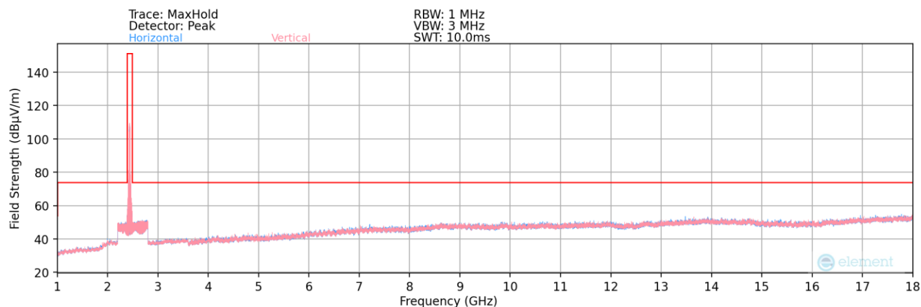
Plot 7-89. Radiated Spurious Plot above 1GHz MIMO (802.11n – Ch. 6)
