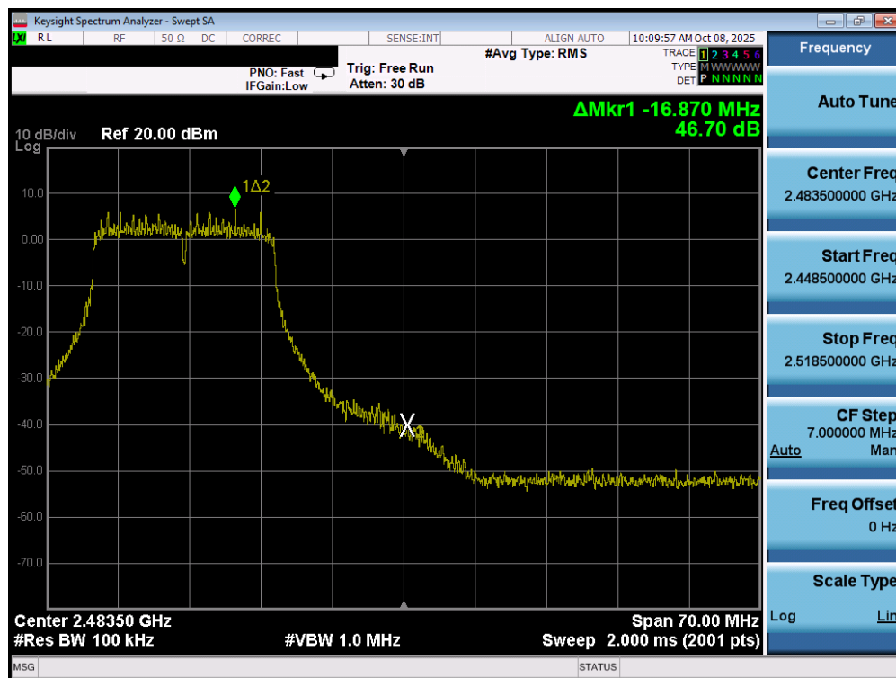
Plot 7-70. Band Edge Plot MIMO ANT2 (802.11n/ac (2.4GHz) – Ch. 11)
