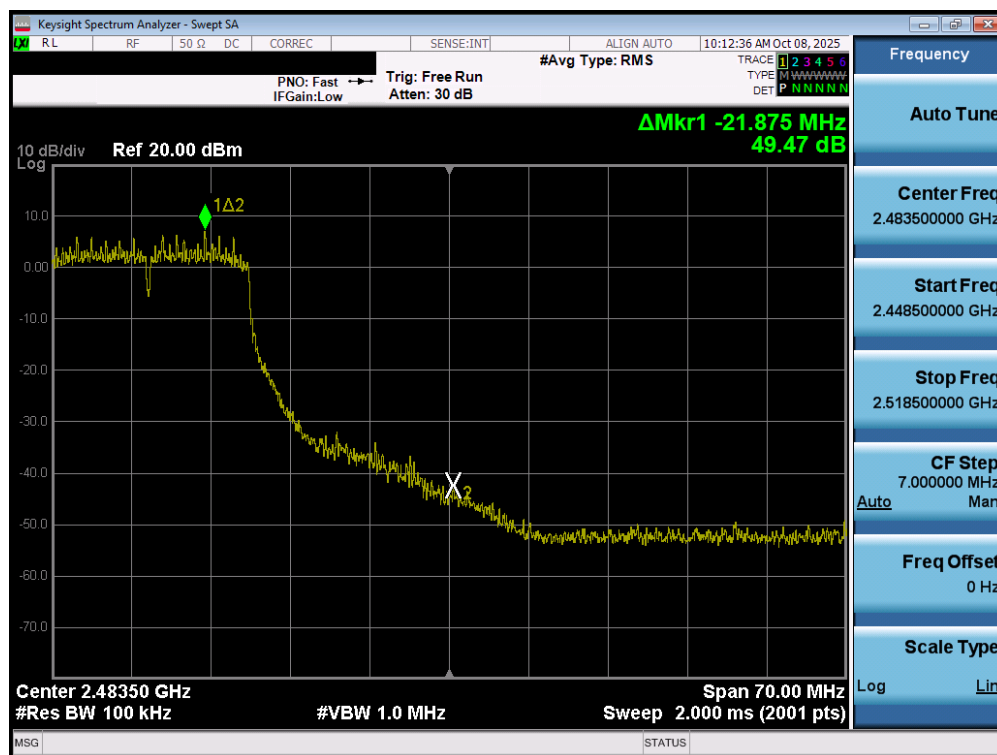
Plot 7-69. Band Edge Plot MIMO ANT2 (802.11n/ac (2.4GHz) – Ch. 10)
