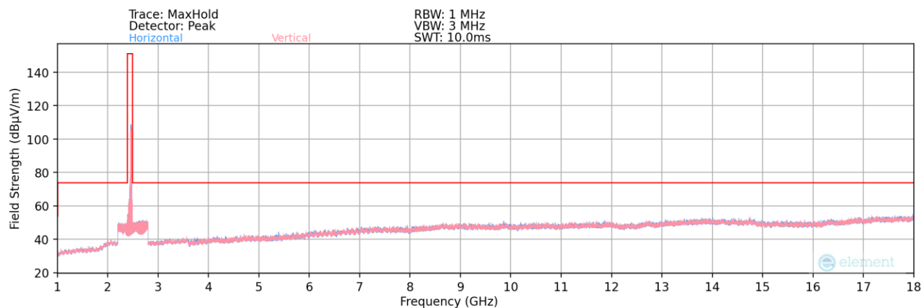
Plot 7-90. Radiated Spurious Plot above 1GHz MIMO (802.11n – Ch. 11)
