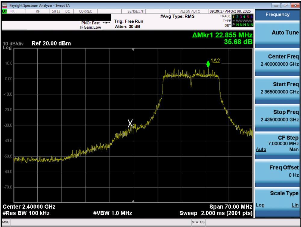
Plot 7-65. Band Edge Plot MIMO ANT2 (802.11g– Ch. 2)
