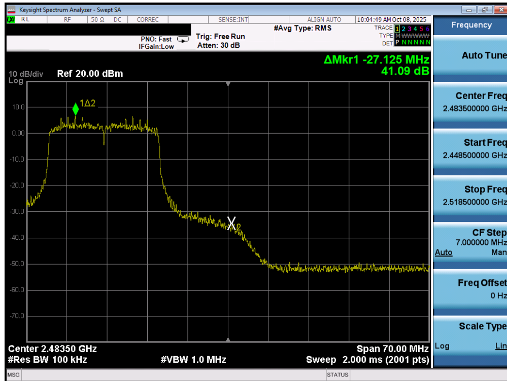
Plot 7-74. Band Edge Plot MIMO ANT2 (802.11ax/be (2.4GHz) – Ch. 11)
