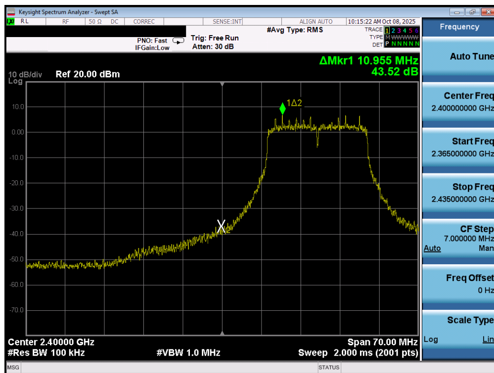
Plot 7-55. Band Edge Plot MIMO ANT1 (802.11n/ac (2.4GHz) – Ch. 2)
