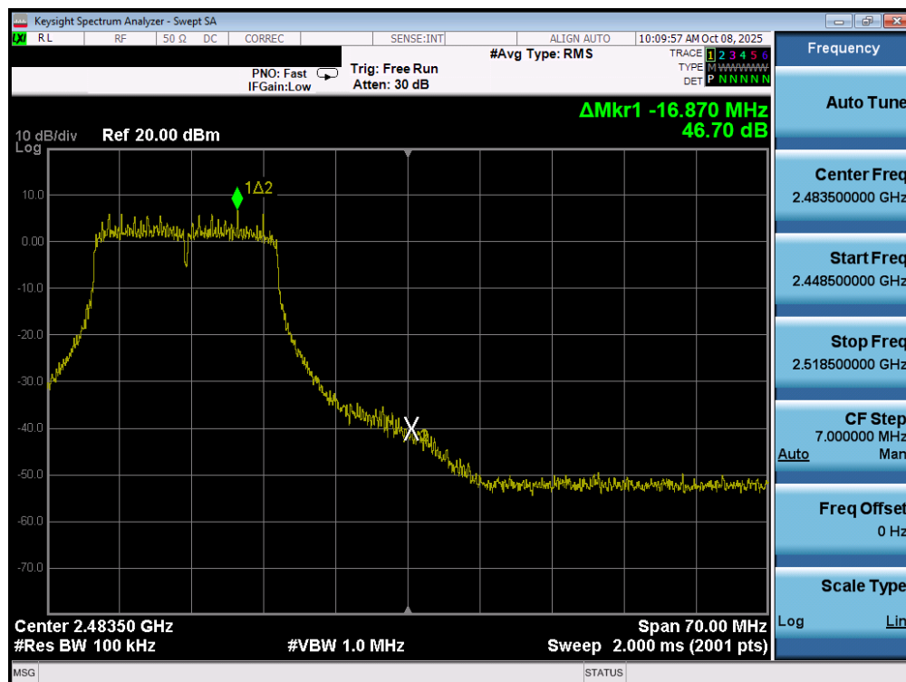
Plot 7-57. Band Edge Plot MIMO ANT1 (802.11n/ac (2.4GHz) – Ch. 11)
