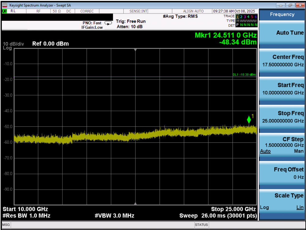
Plot 7-84. Conducted Spurious Plot SISO ANT2 (802.11b – Ch. 6)
