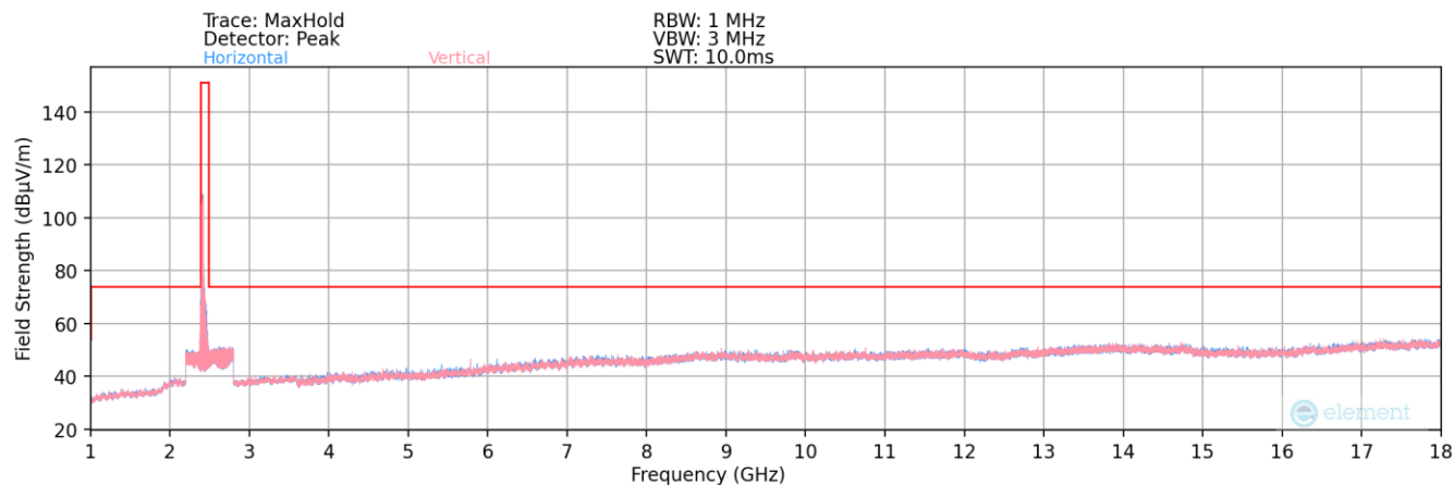
Plot 7-88. Radiated Spurious Plot above 1GHz MIMO (802.11n – Ch. 1)
