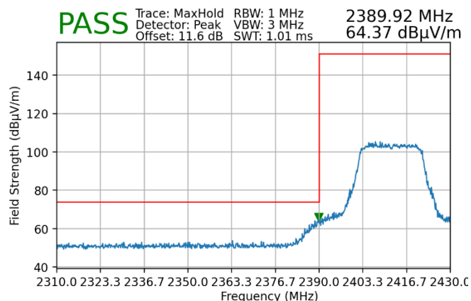
Plot 7-101. Radiated Restricted Lower Band Edge Measurement MIMO (Peak) – WCP
