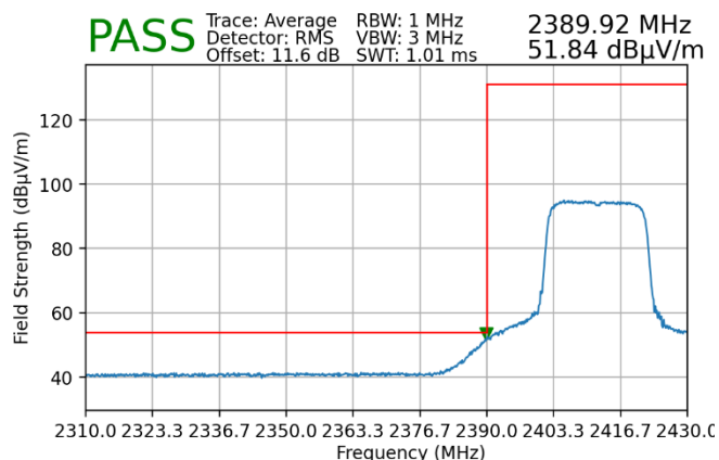
Plot 7-100. Radiated Restricted Lower Band Edge Measurement MIMO (Average) – WCP
