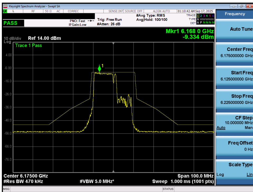
Plot 7-62. In Band Emissions Plot MIMO ANT1 (20MHz 802.11be (106+26 Tones) (UNII Band 5) – Ch. 45) - VLP
