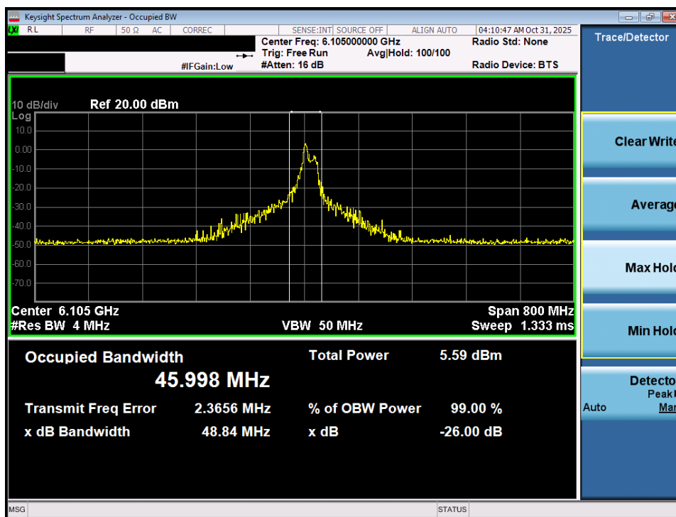
Plot 7-19. 26dB Bandwidth Plot MIMO ANT2 (320MHz 802.11be (26 Tones) (UNII Band 5) – Ch. 31) - VLP
