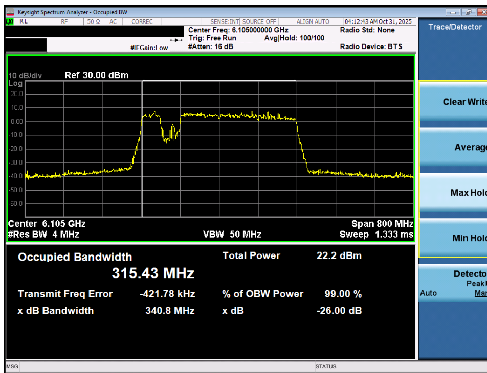
Plot 7-23. 26dB Bandwidth Plot MIMO ANT2 (320MHz 802.11be (3*996+484 Tones) (UNII Band 5) – Ch. 31) VLP
