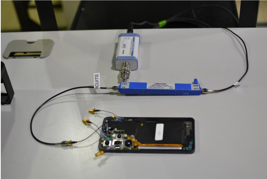
Test Setup Photo 3 – Conducted Test Setup (Figure 7-1a)
