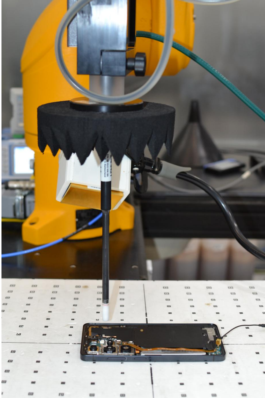
Test Setup Photo 14 – Conducted Test Setup (Figure 12-1)
