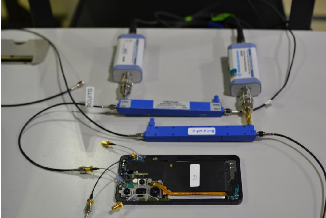
Test Setup Photo 9 – Conducted Test Setup (Figure 7-1c)
