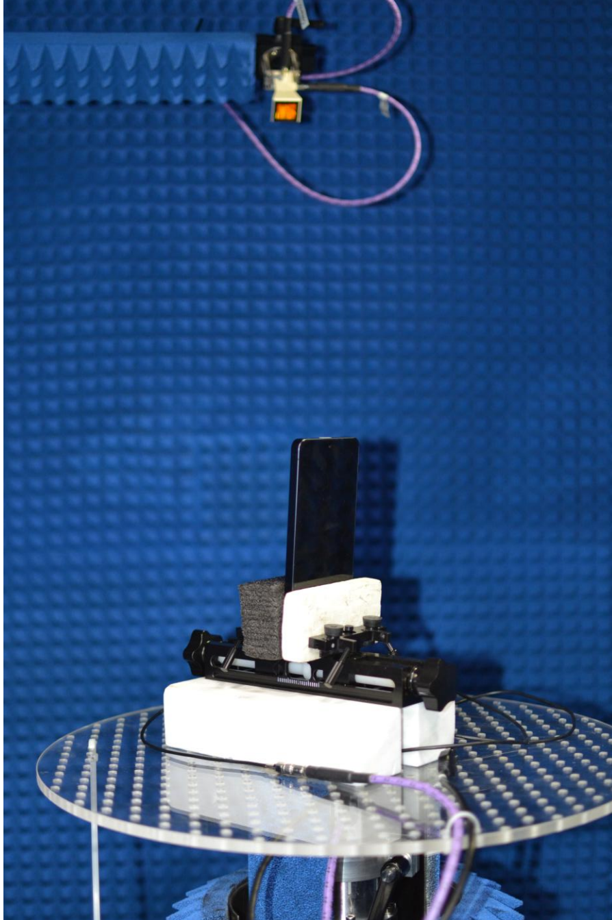
Test Setup Photo 13 – Conducted Test Setup (Figure 10-1)
