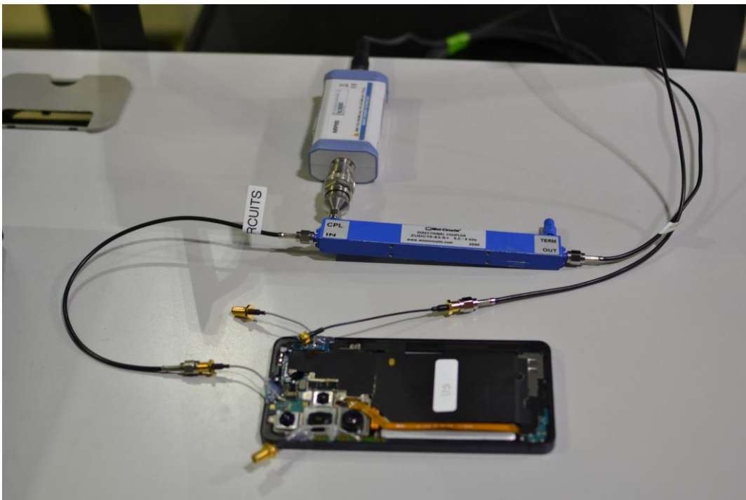
Test Setup Photo 6 – Conducted Test Setup (Figure 7-1d)
