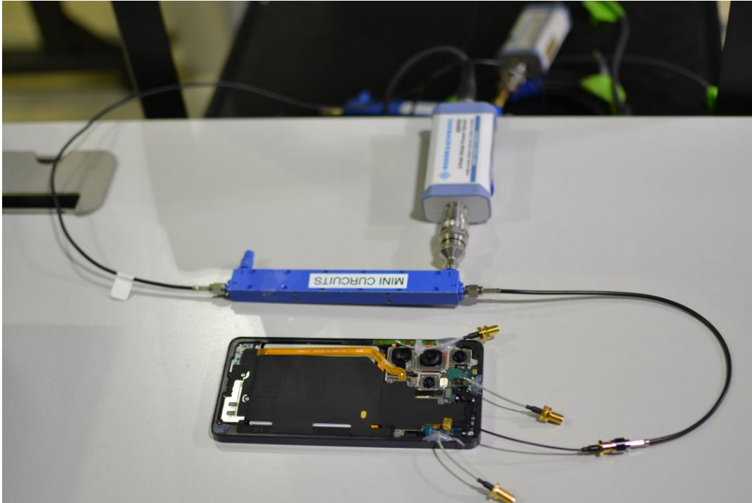
Test Setup Photo 5 – Conducted Test Setup (Figure 7-1a)
