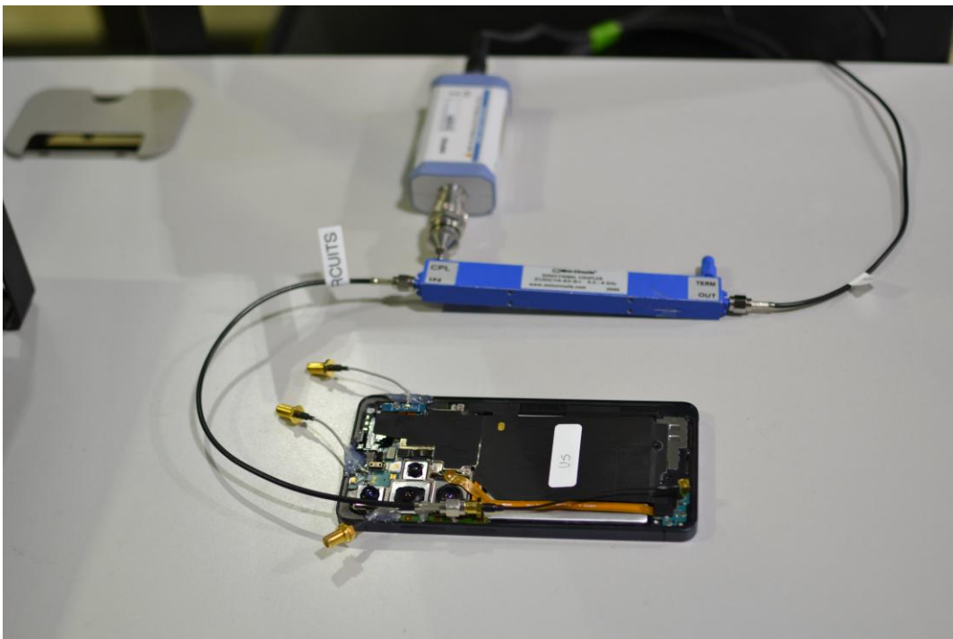
Test Setup Photo 2 – Conducted Test Setup (Figure 7-1a)
