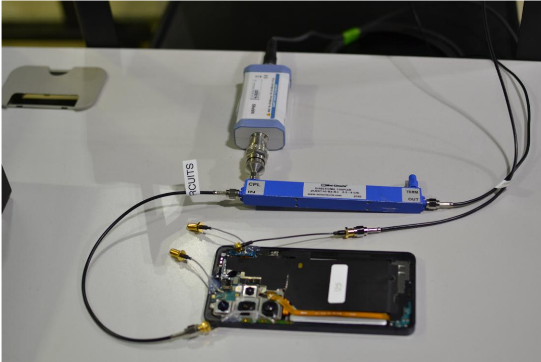
Test Setup Photo 7 – Conducted Test Setup (Figure 7-1d)
