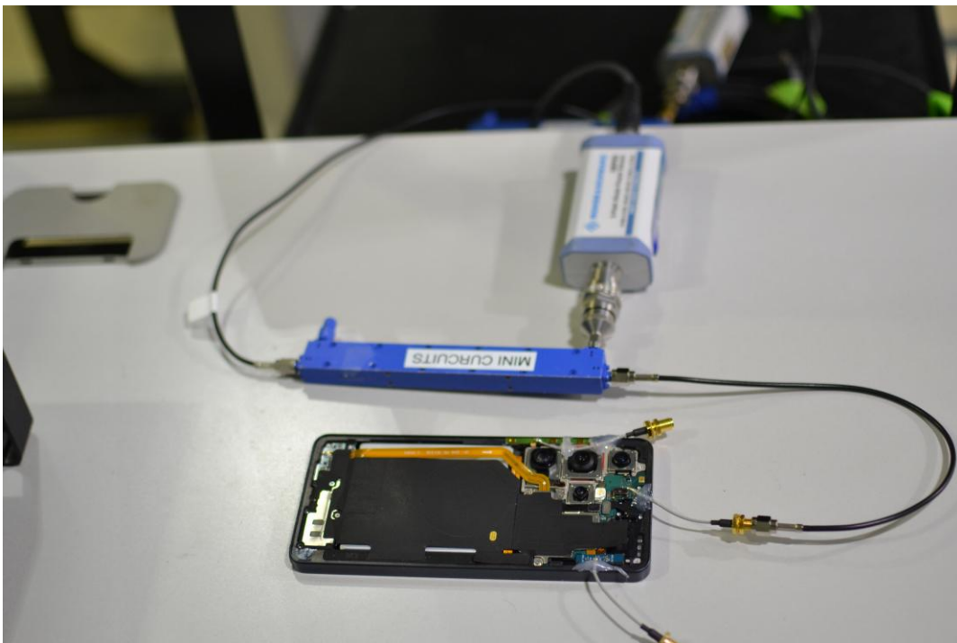
Test Setup Photo 4 – Conducted Test Setup (Figure 7-1a)
