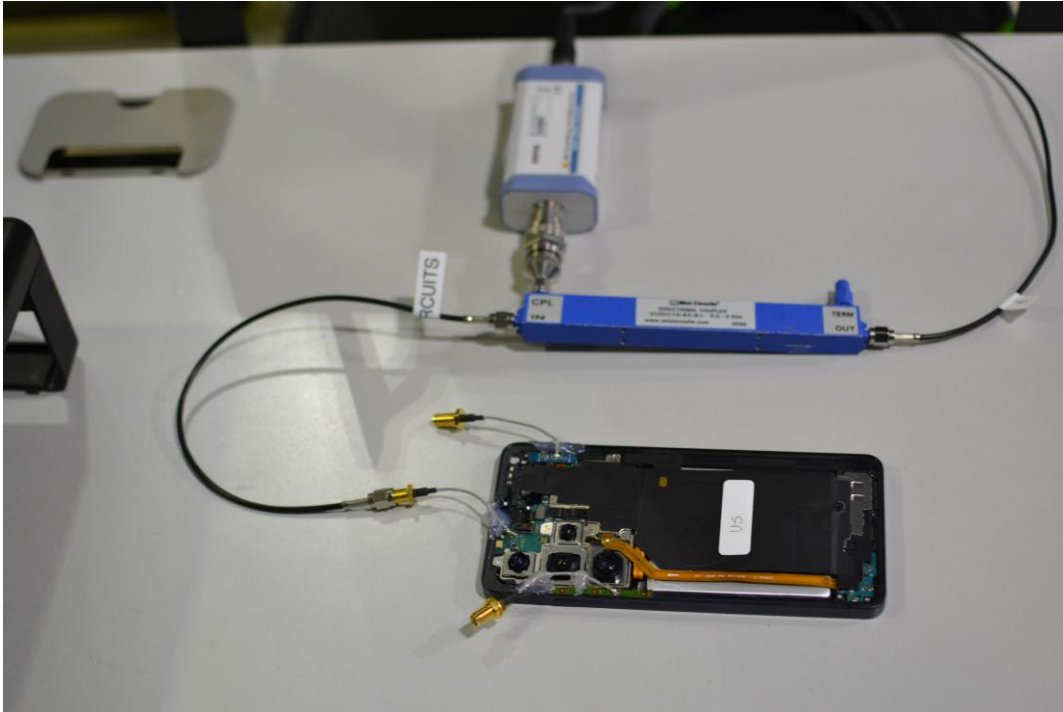
Test Setup Photo 1 – Conducted Test Setup (Figure 7-1a)
