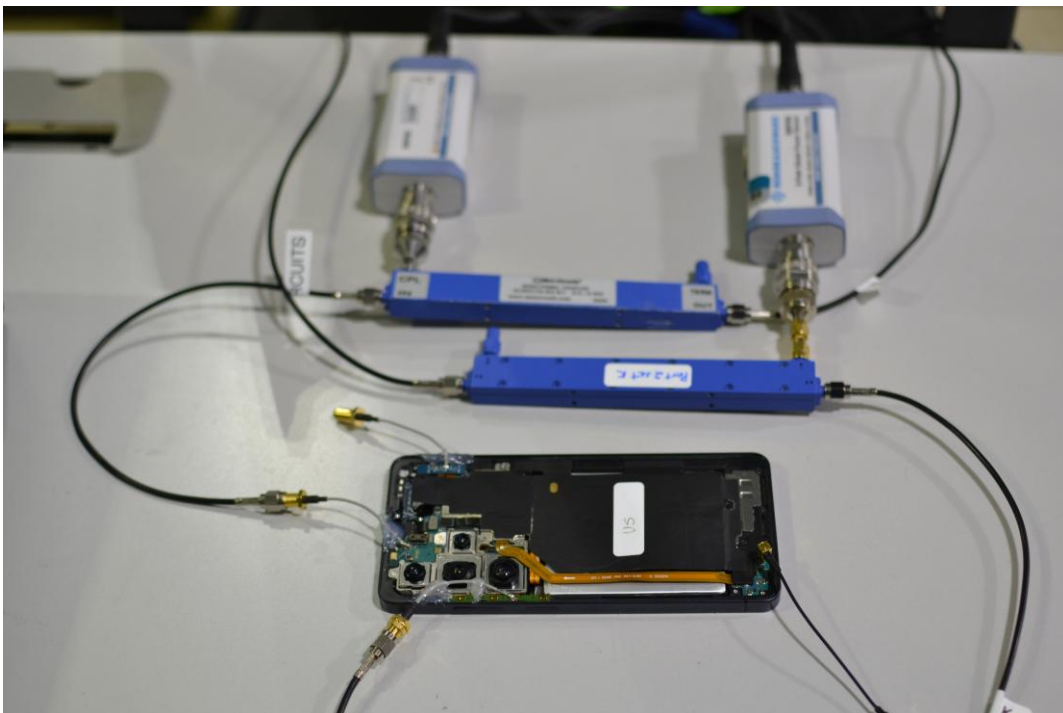
Test Setup Photo 10 – Conducted Test Setup (Figure 7-1e)
