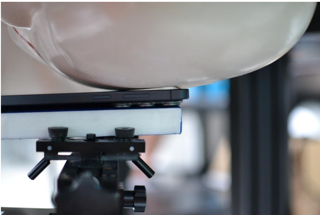
Test Setup Photo 16 – Radiated SAR, Left Cheek
