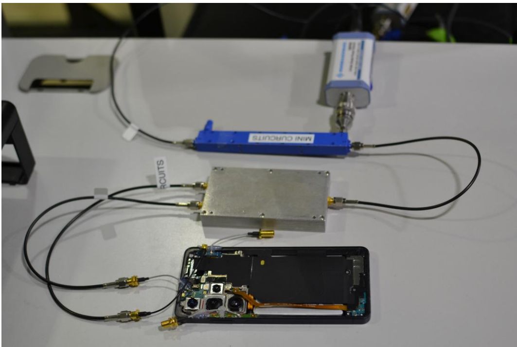
Test Setup Photo 8 – Conducted Test Setup (Figure 7-1b)
