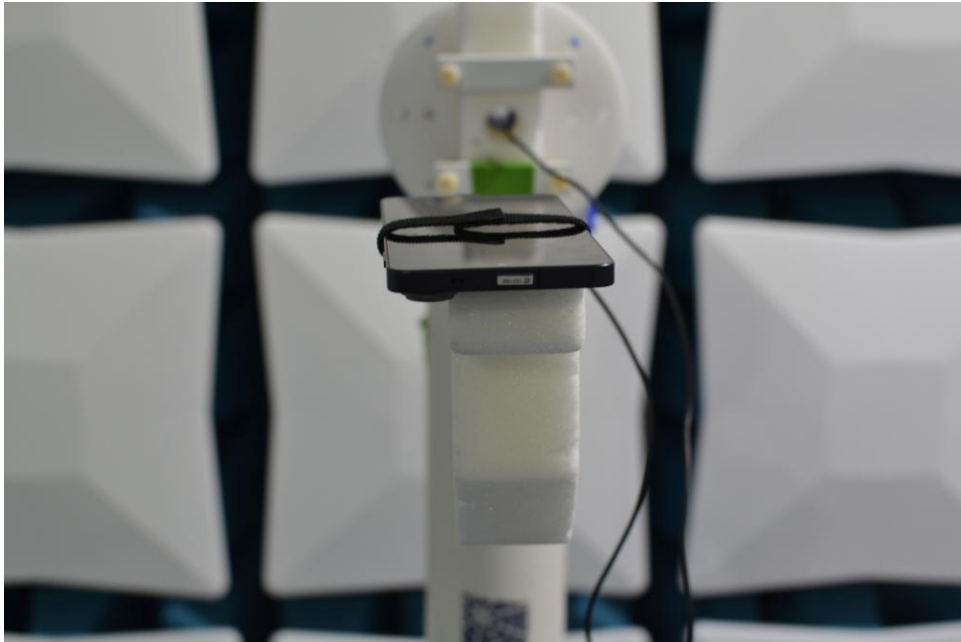
Figure 1. Test Setup – X-Up Position - >40GHz
