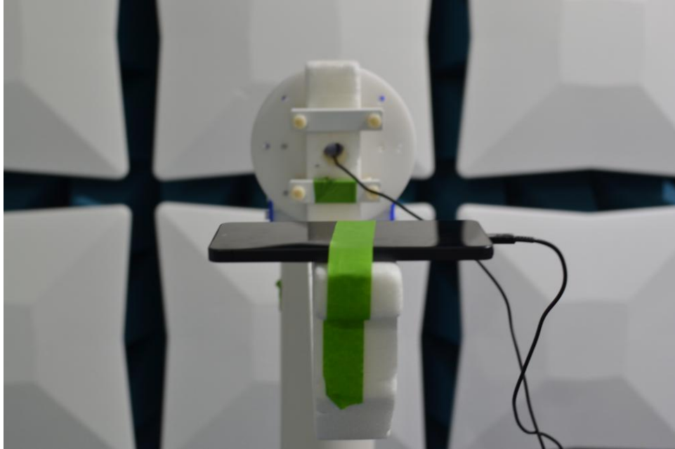
Figure 3. Test Setup – Y-Up Position - >40GHz
