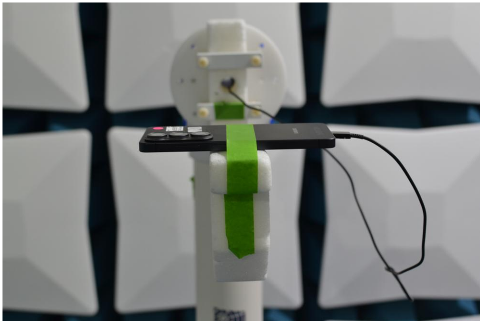
Figure 4. Test Setup – Y-Down Position - >40GHz
