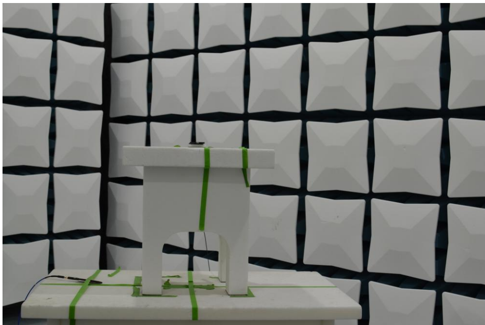
Figure 8. Test Setup – WCP
