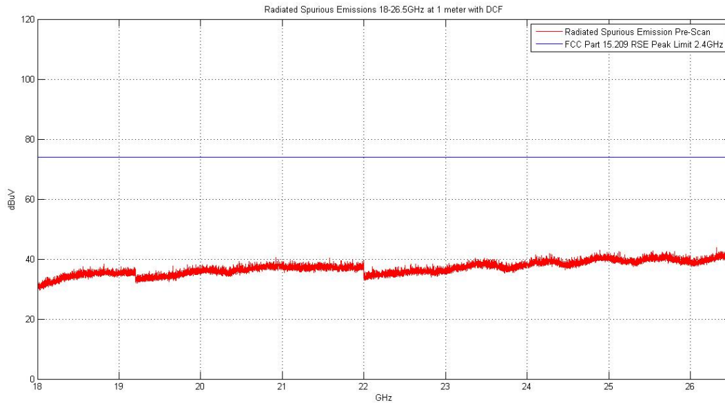
Plot 6-48. Radiated Spurious Plot above 18GHz (Pol. H)
