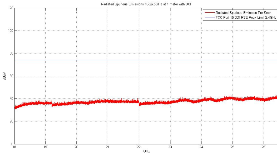
Plot 6-49. Radiated Spurious Plot above 18GHz (Pol. V)
