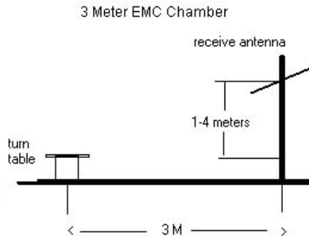
Figure 6-5. Test Instrument & Measurement Setup
