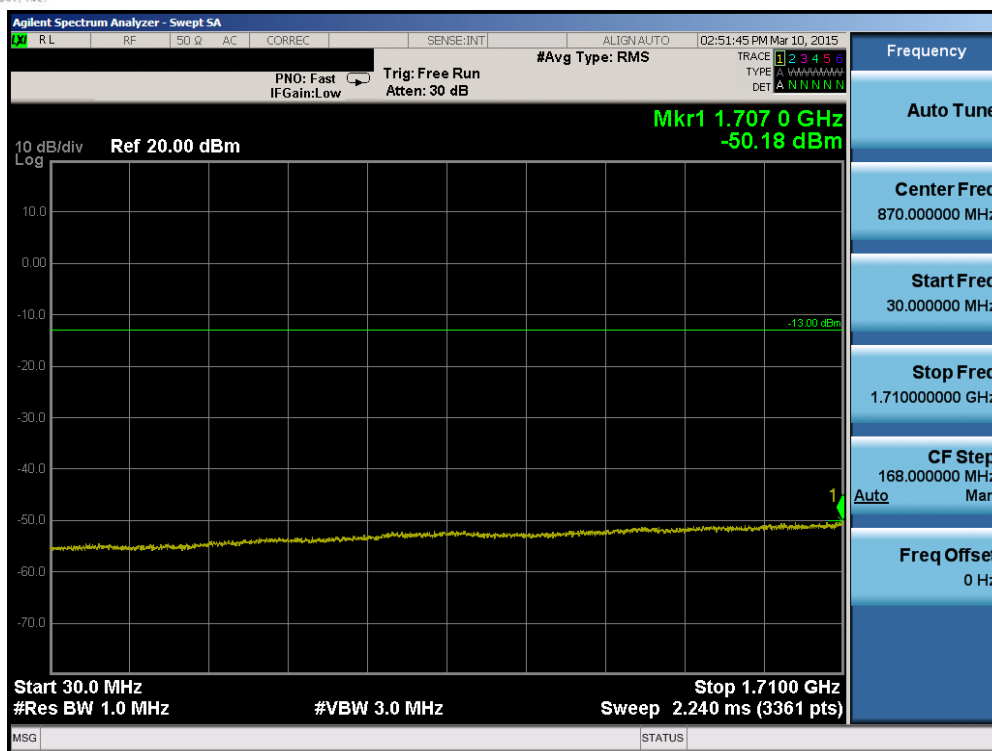
Plot 6-29. Conducted Spurious Plot (Band 4 – 15.0MHz QPSK – RB Size 1, RB Offset 0 – Mid Channel)
