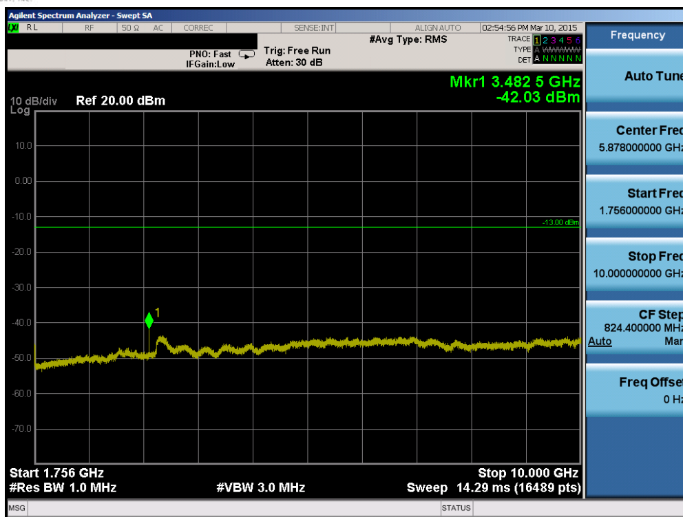
Plot 6-33. Conducted Spurious Plot (Band 4 – 15.0MHz QPSK – RB Size 1, RB Offset 0 – High Channel)
