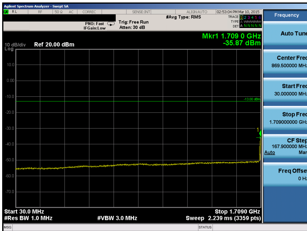
Plot 6-26. Conducted Spurious Plot (Band 4 – 15.0MHz QPSK – RB Size 1, RB Offset 0 – Low Channel)
