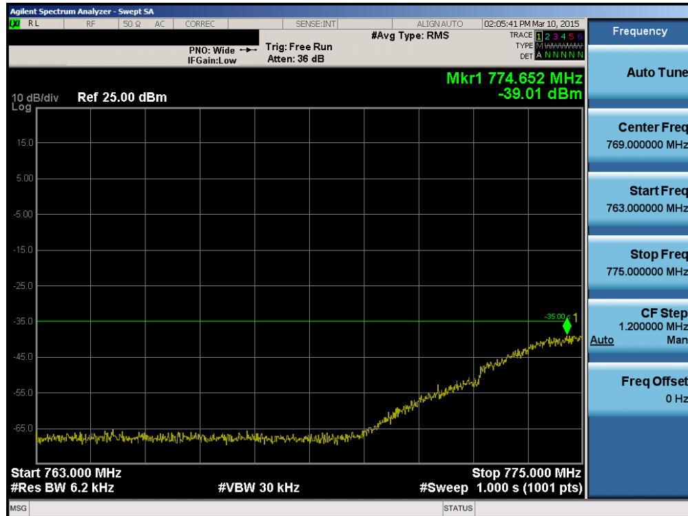
Plot 6-36. Lower Emission Mask Plot (Band 13 – 5.0MHz QPSK – RB Size 25)
