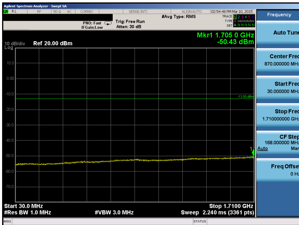
Plot 6-32. Conducted Spurious Plot (Band 4 – 15.0MHz QPSK – RB Size 1, RB Offset 0 – High Channel)
