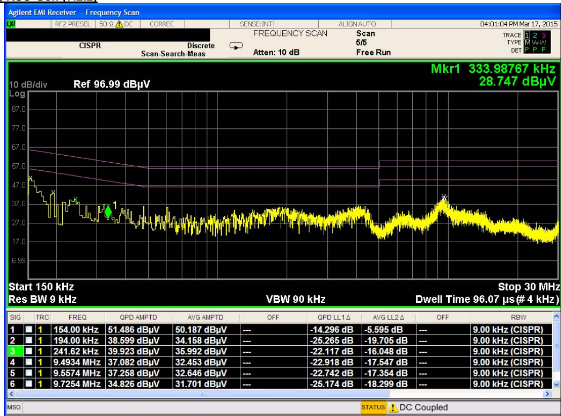
Plot 7-2. Line Conducted Plot (LN)
