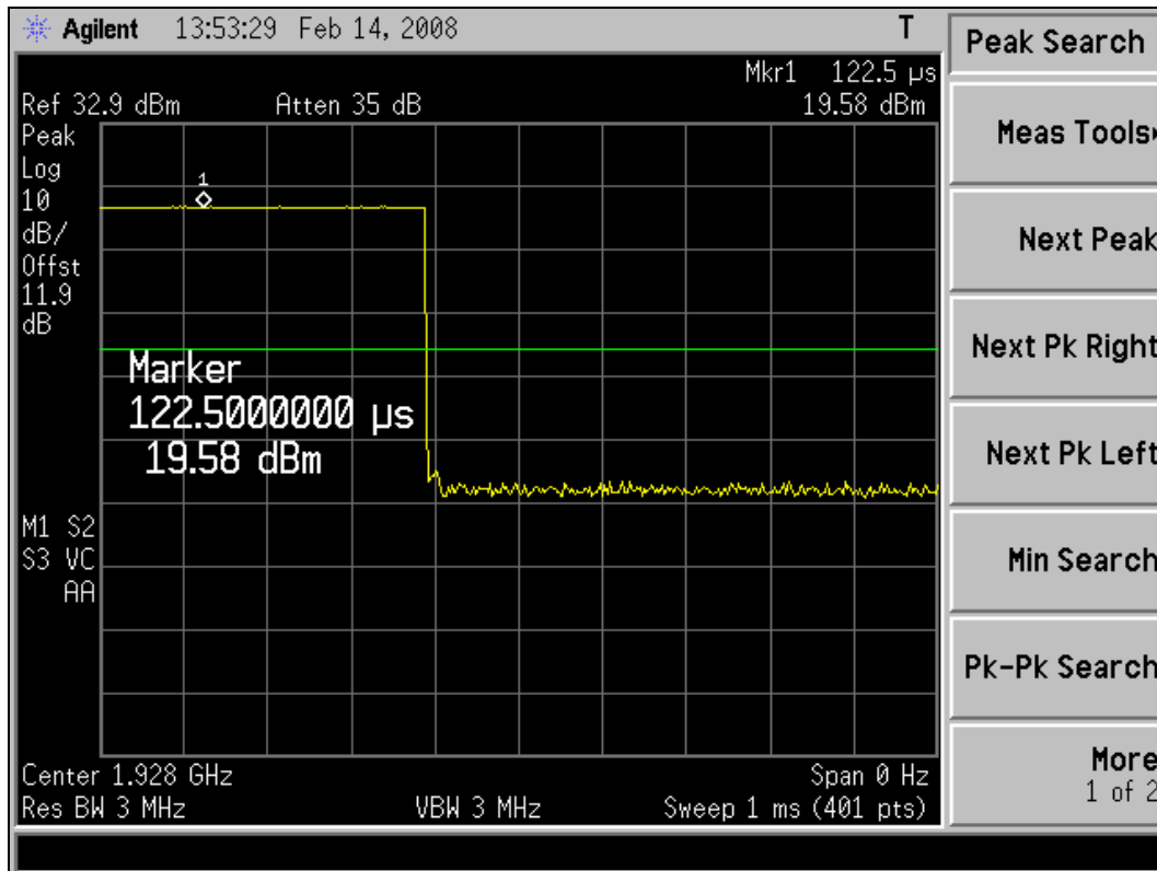
– Peak transmit power of Ch 5 –
