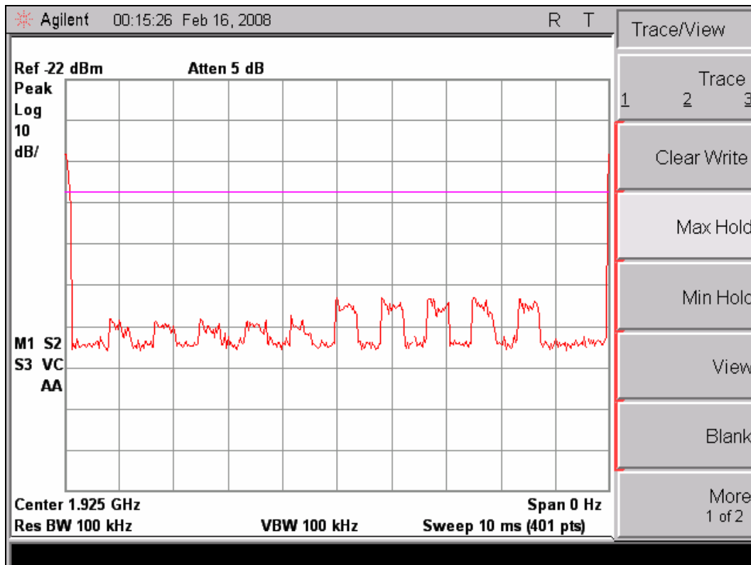
– Slot Occupancy for clause 8.3.2(e) –
