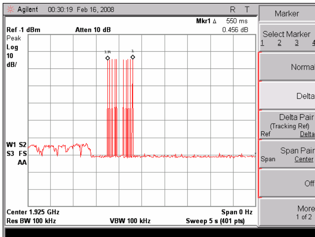
– Initial transmission without acknowledgements –
