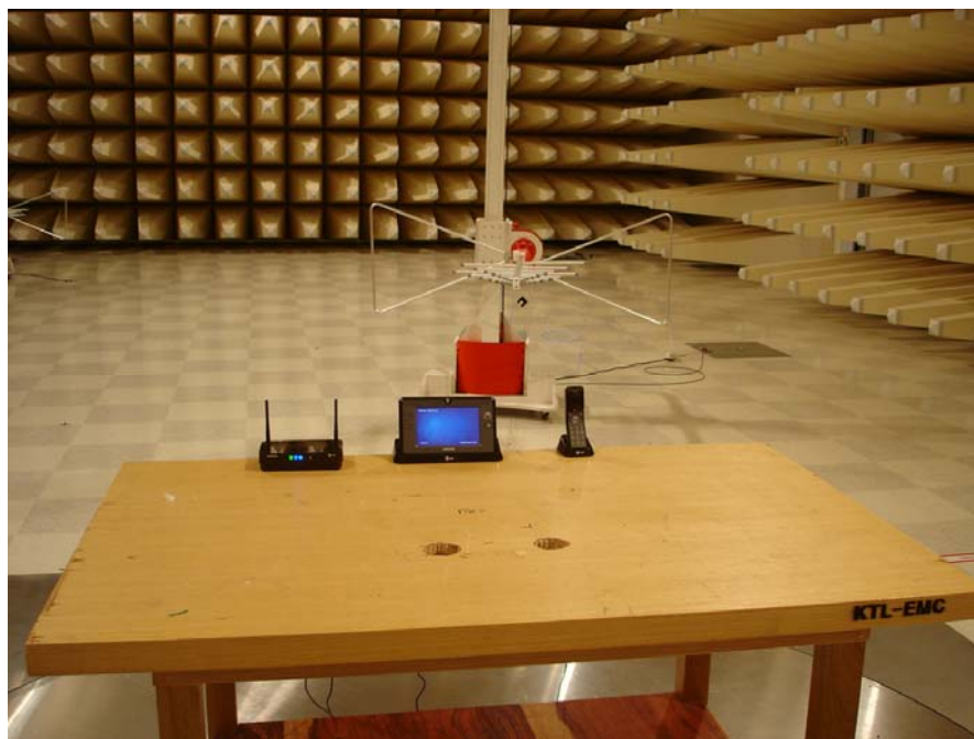
<Radiated Emission>
