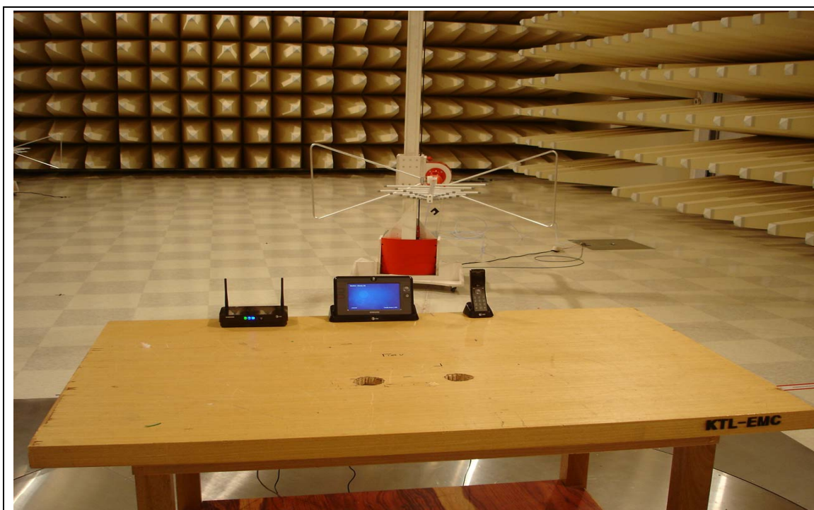
< Radiated emission Test >
