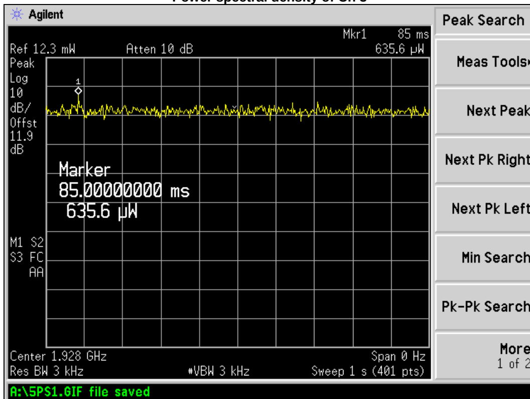
– Power spectral density of Ch 5 –
