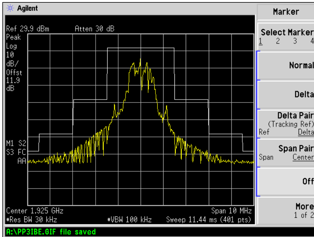
– In-band emission of Ch 3 –
