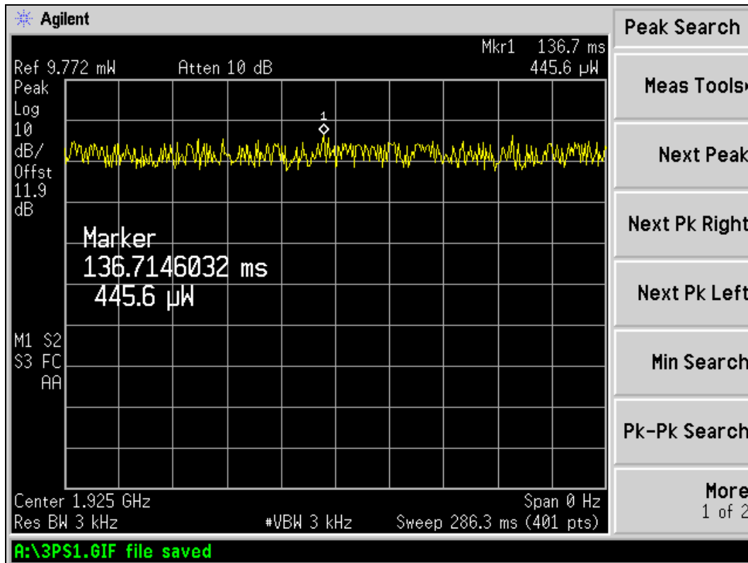
– Power spectral density of Ch 3 –
