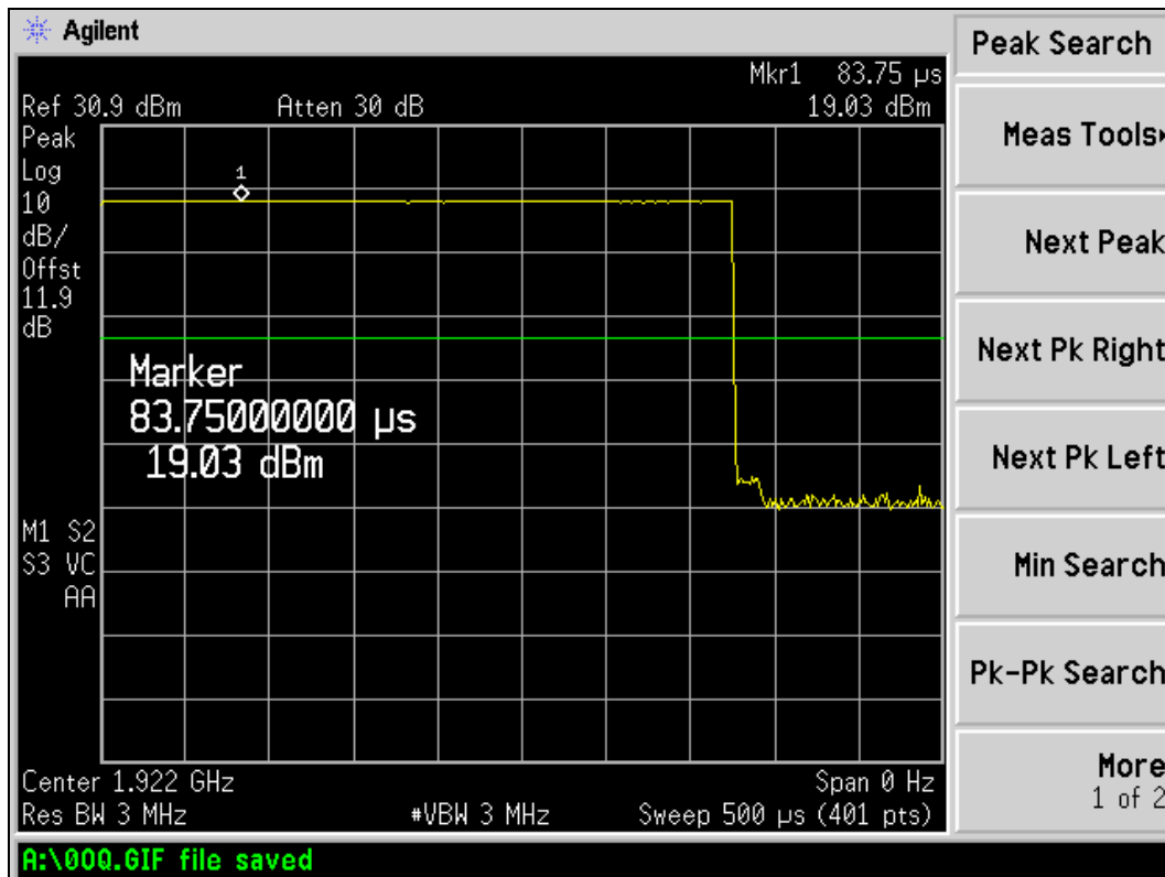
- Peak transmit power of Ch 1 -
