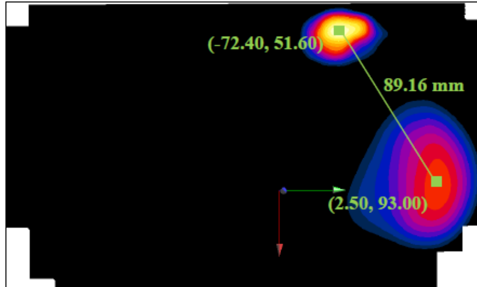
Figure 11-2 Peak SAR Locations of 2.4 GHz WLAN and GPRS 850 MHz
