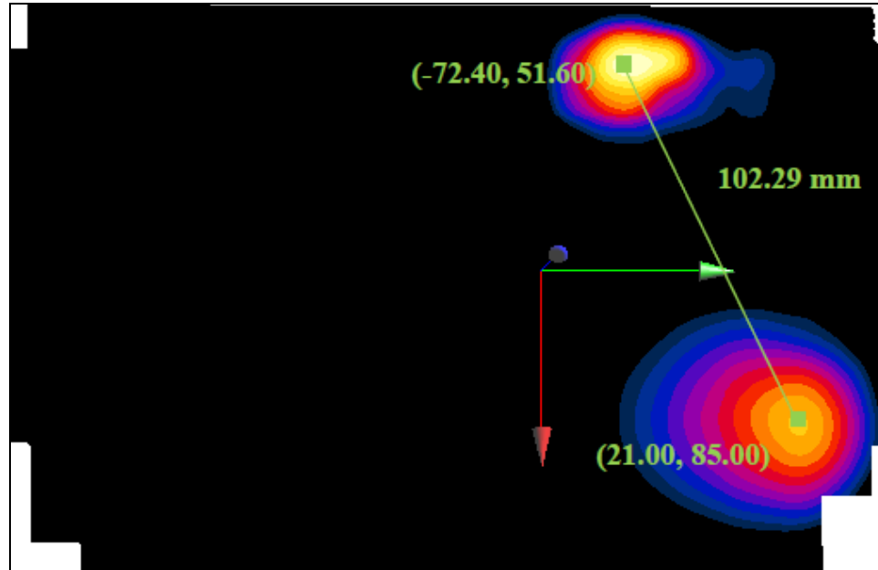
Figure 11-1 Peak SAR Locations of 2.4 GHz WLAN and GPRS 850 MHz
