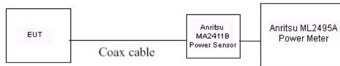
Figure 8-2 Power Measurement Setup
