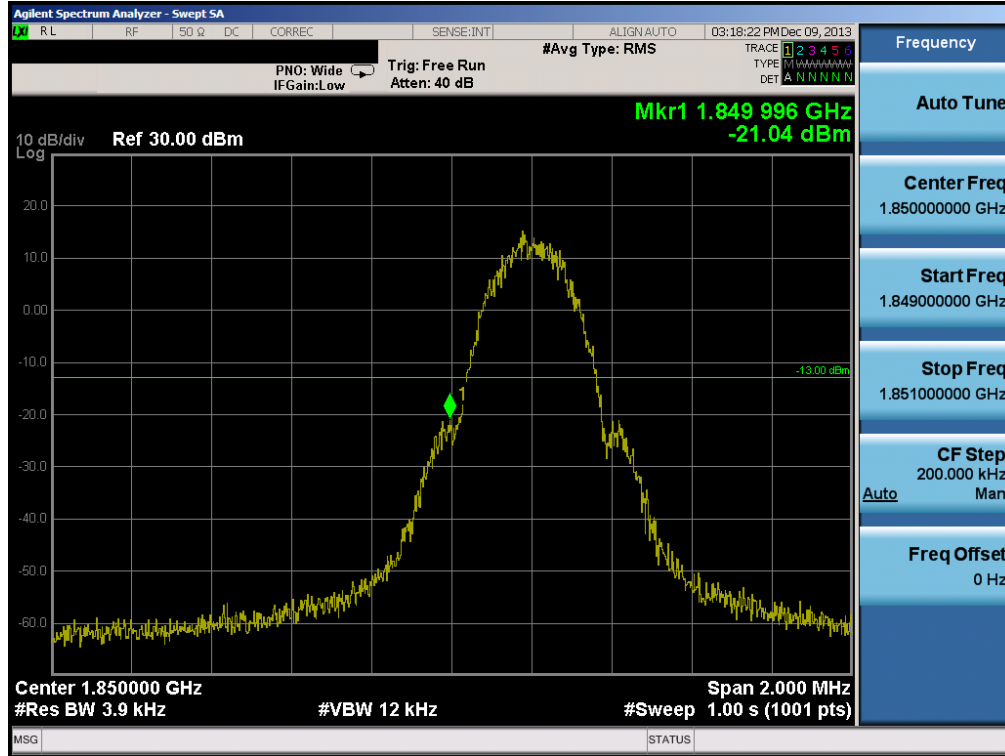
Plot 6-20. Band Edge Plot (PCS GSM Mode – Ch. 512)
