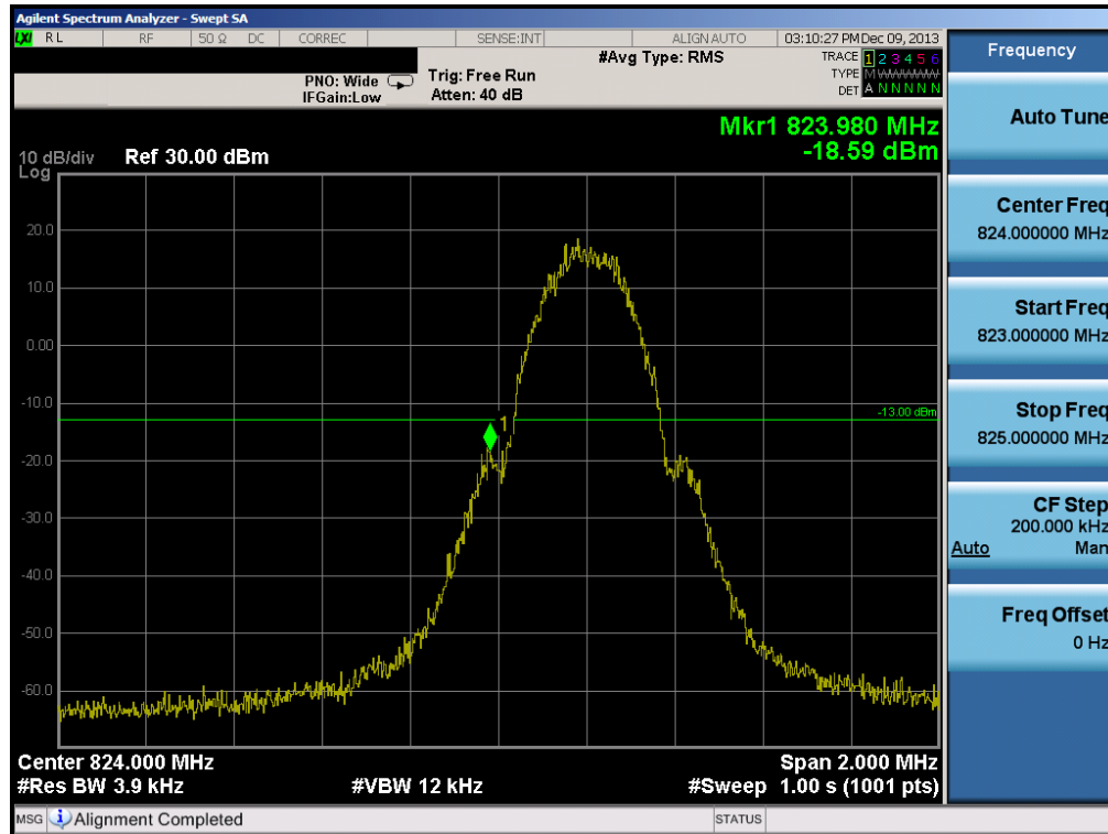
Plot 6-18. Band Edge Plot (Cellular GSM Mode – Ch. 128)
