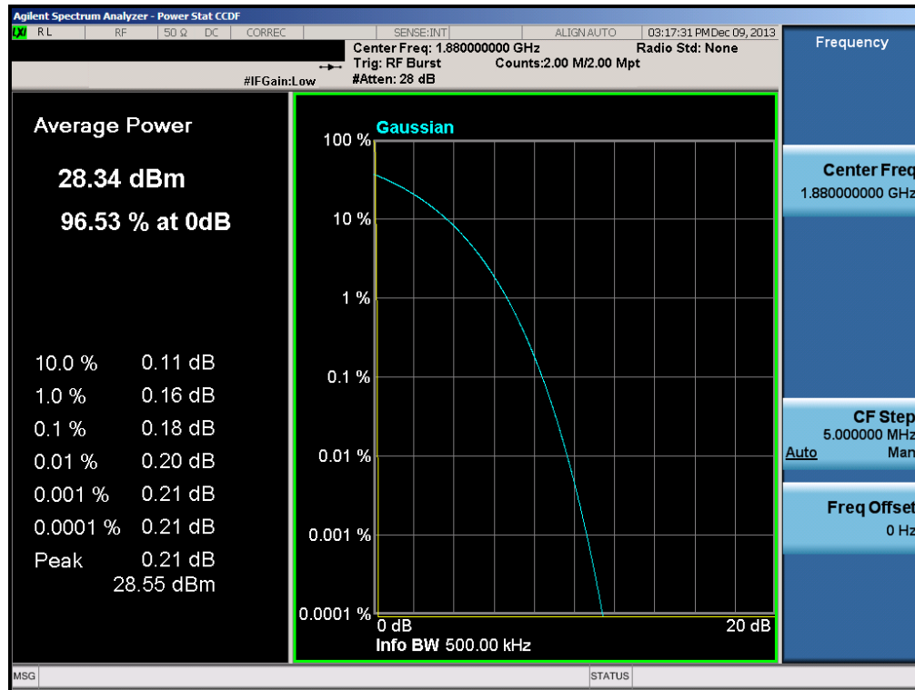
Plot 6-22. Peak-Average Ratio Plot (PCS GSM Mode – Ch. 661)
