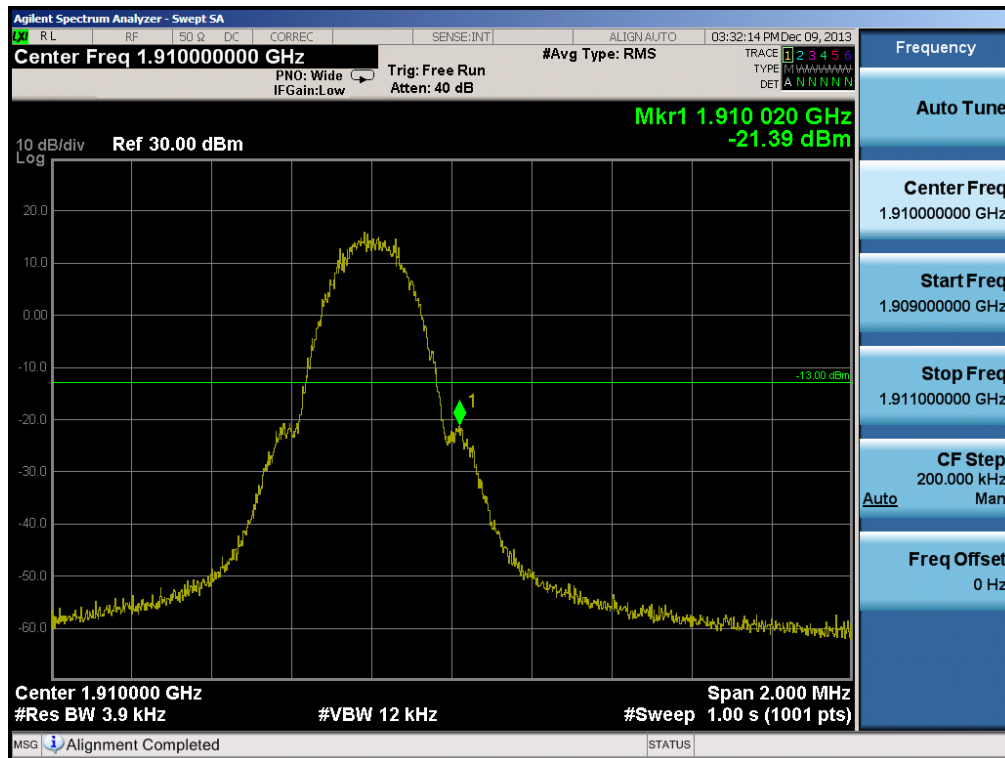
Plot 6-21. Band Edge Plot (PCS GSM Mode – Ch. 810)
