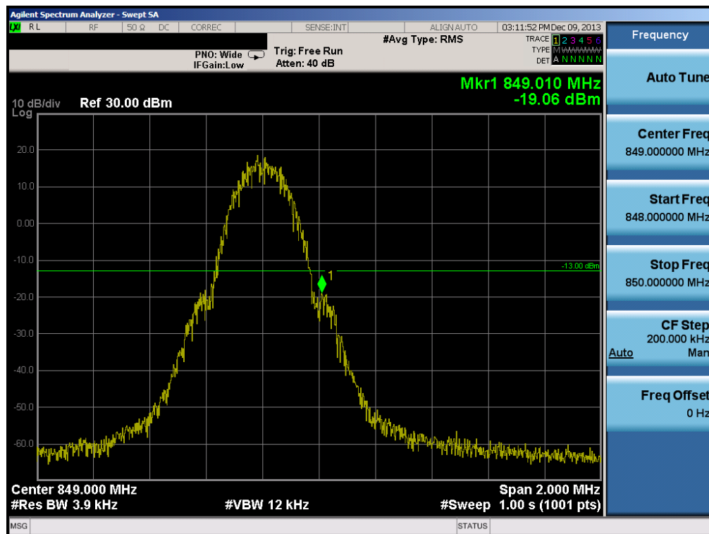
Plot 6-19. Band Edge Plot (Cellular GSM Mode – Ch. 251)
