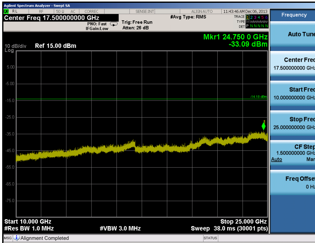
Plot 6-39. Conducted Spurious Plot (Bluetooth, 3Mbps – Ch. 39)
