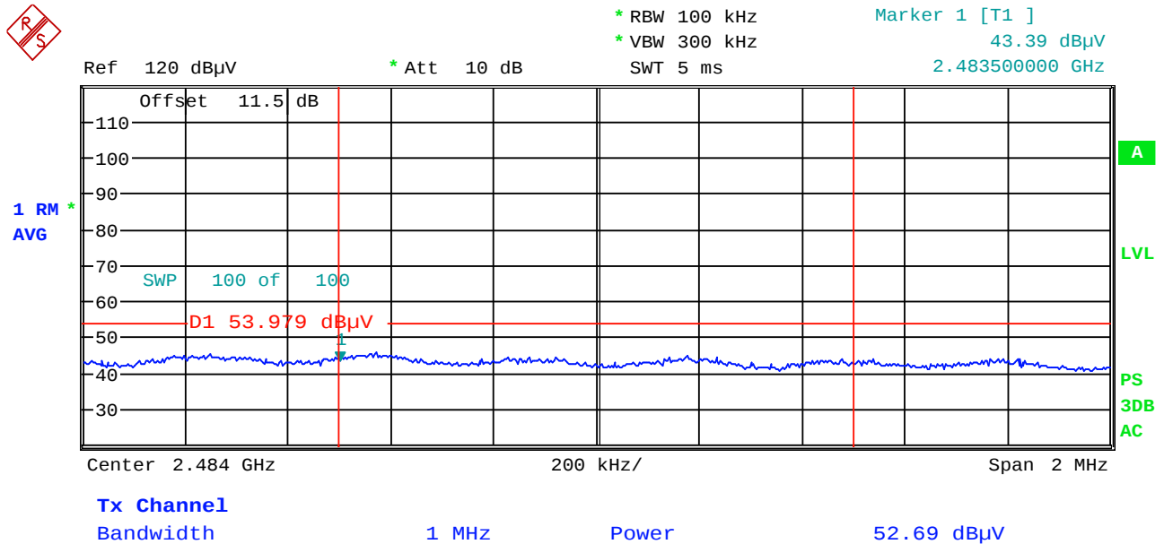
Plot 6-33. Radiated Restricted Upper Band Edge Measurement (Average)
