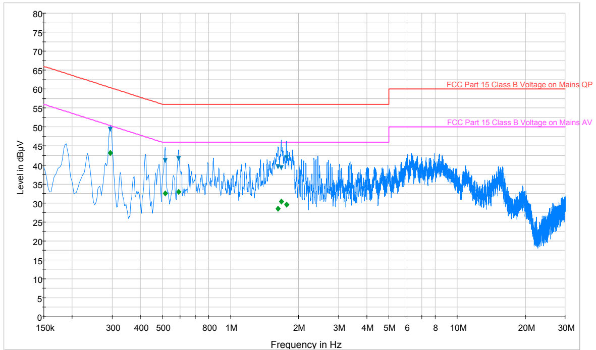
Plot 6-36. Line Conducted Plot with 802.11b (N)
