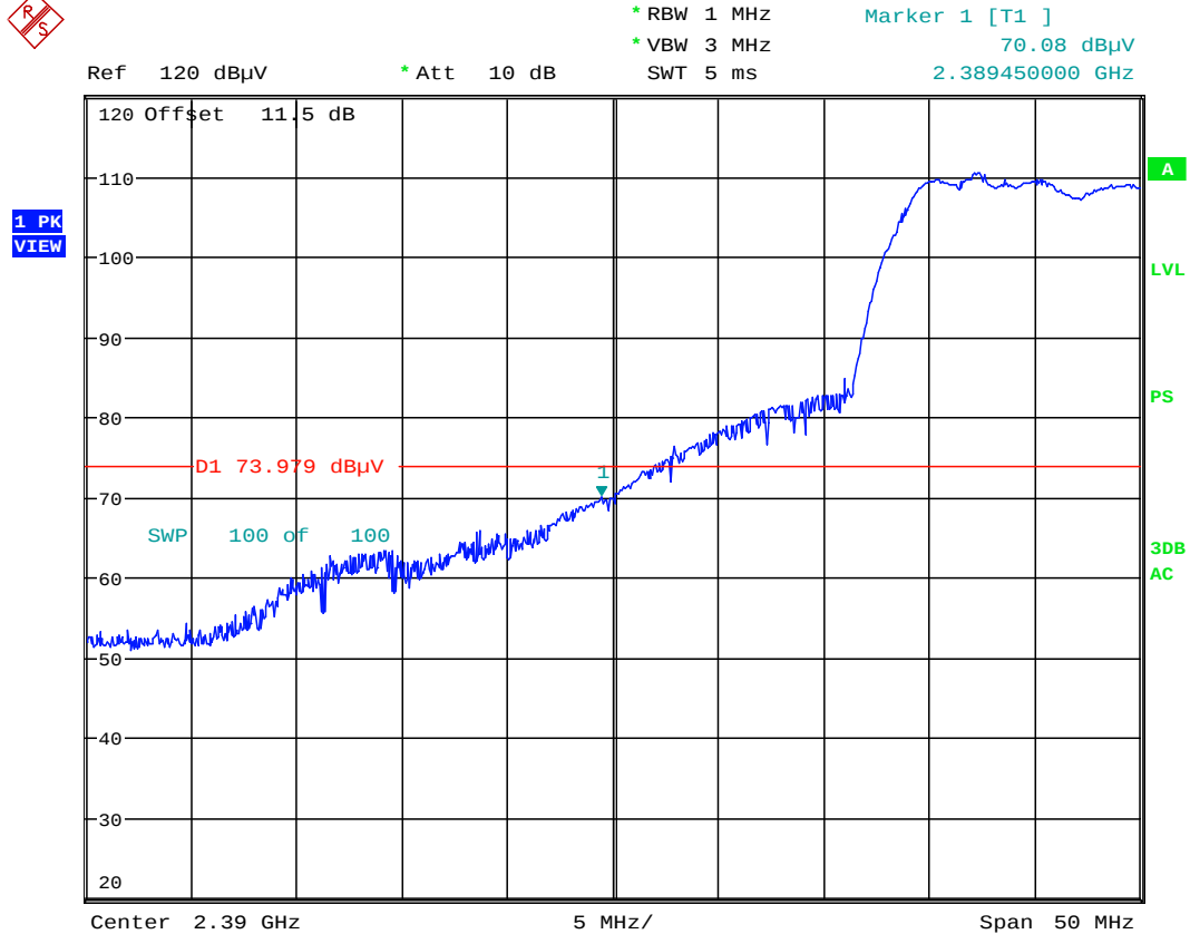
Plot 6-32. Radiated Restricted Lower Band Edge Measurement (Peak)
