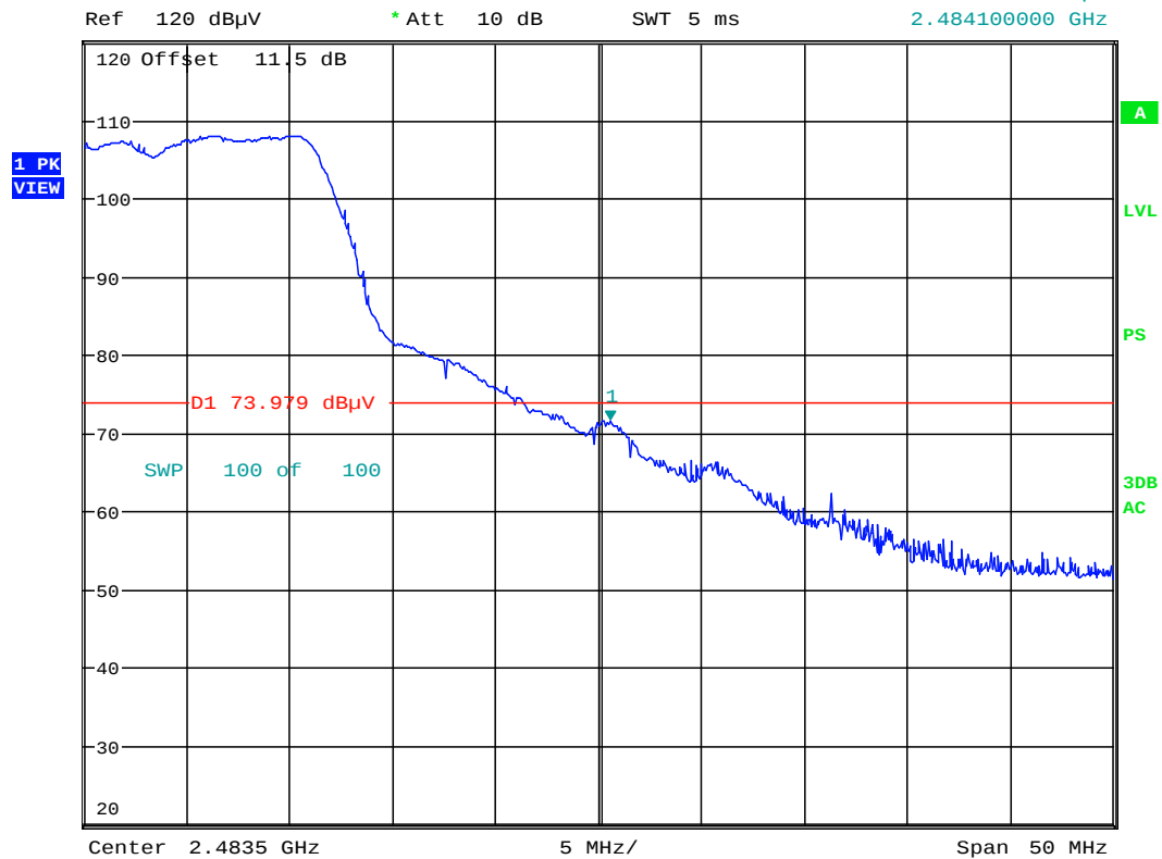
Plot 6-34. Radiated Restricted Upper Band Edge Measurement (Peak)
