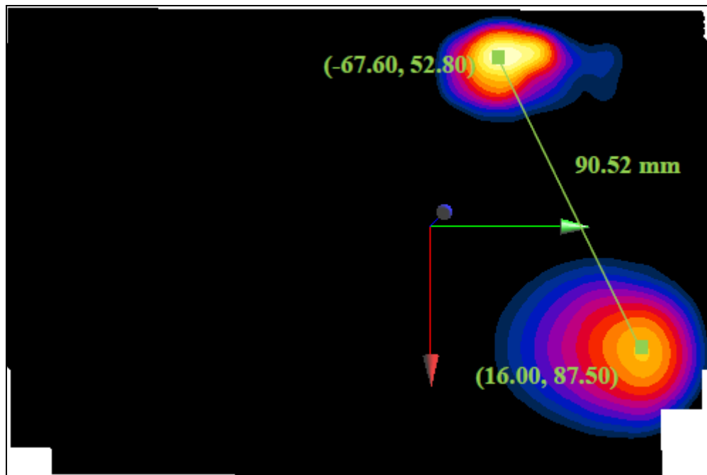
Figure 11-1 Peak SAR Locations of 2.4 GHz WLAN and GPRS 850 MHz
