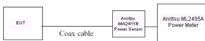
Figure 8-3 Power Measurement Setup
