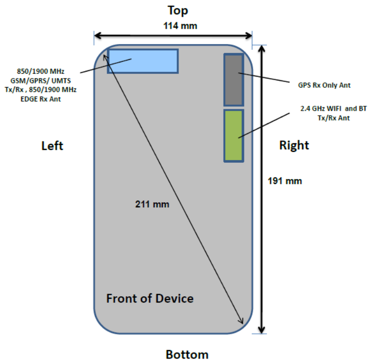
Figure 1-1 DUT Antenna Locations
