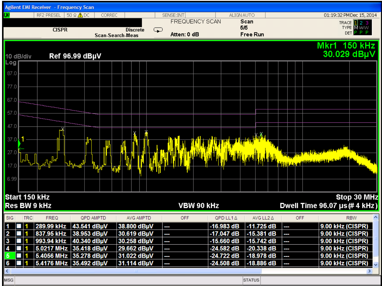
Plot 6-36. Line Conducted Plot and Data with 802.11b (N)
