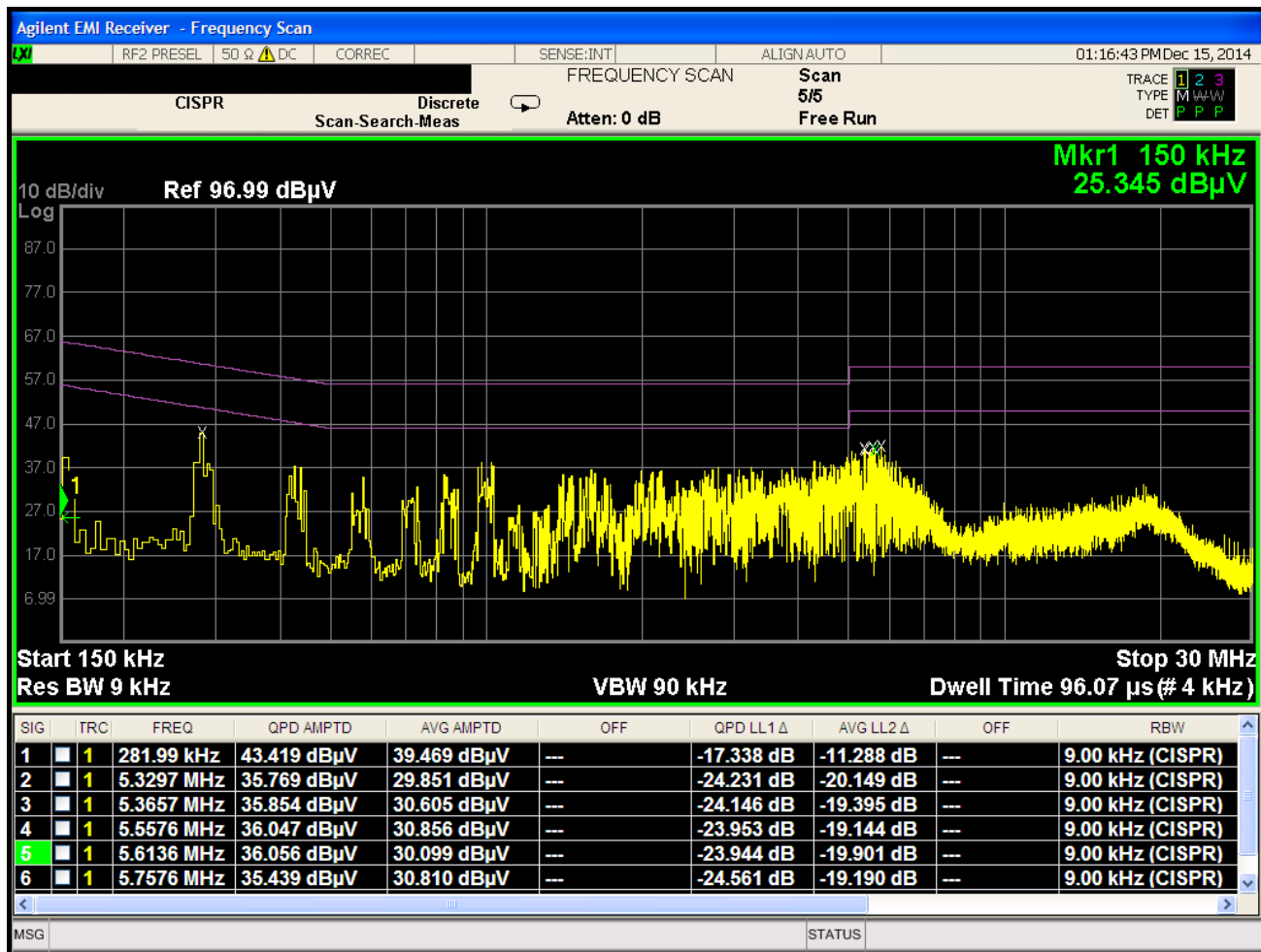
Plot 6-35. Line Conducted Plot and Data with 802.11b (L1)
