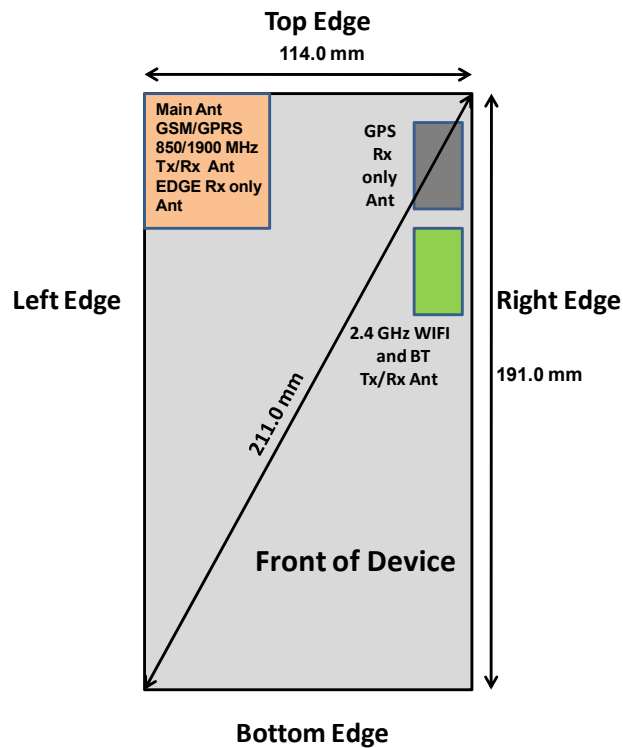
Figure 1 DUT Antenna Locations
