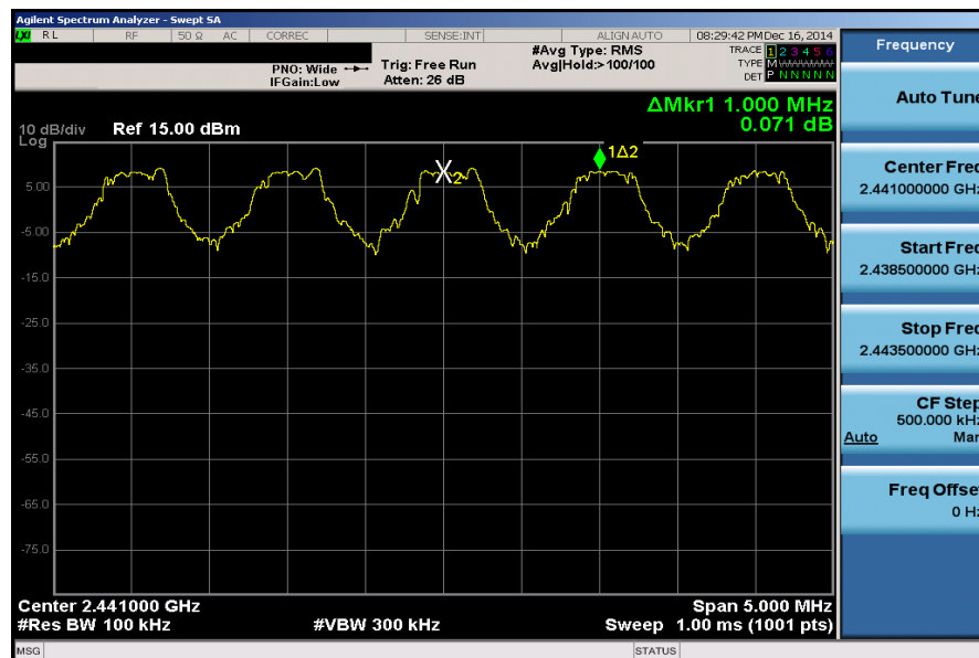
Plot 6-32. Channel Spacing Plot (Bluetooth)
