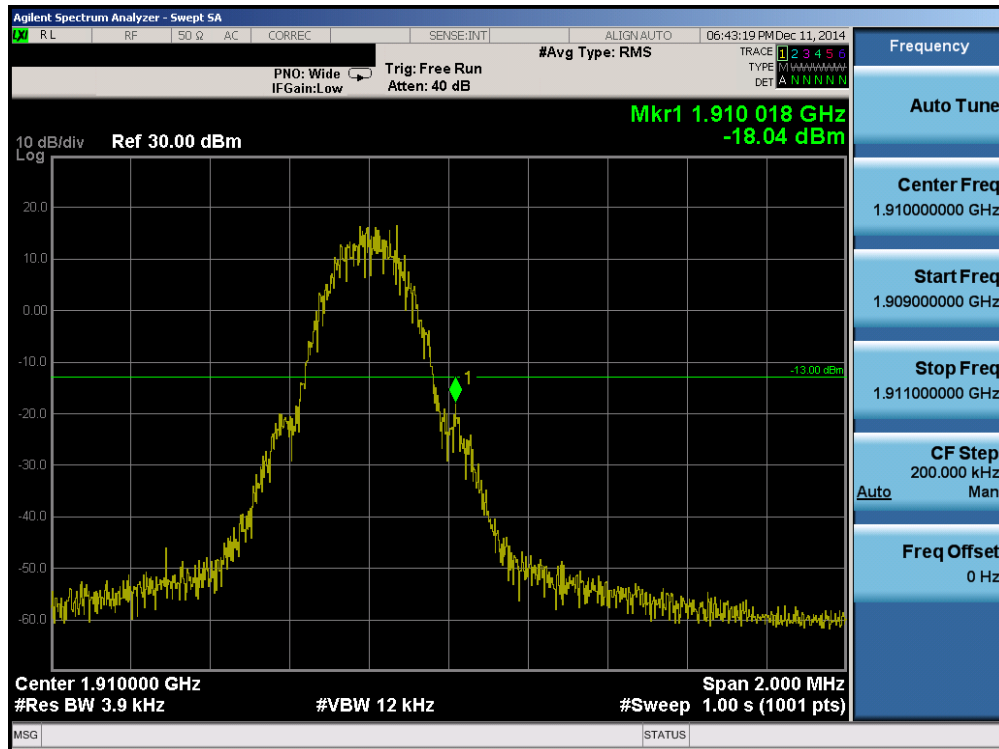
Plot 6-41. Band Edge Plot (PCS GPRS Mode – Ch. 810)
