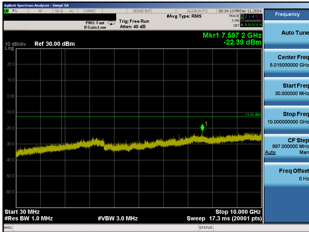
Plot 6-16. Conducted Spurious Plot (PCS GPRS Mode – Ch. 661)
