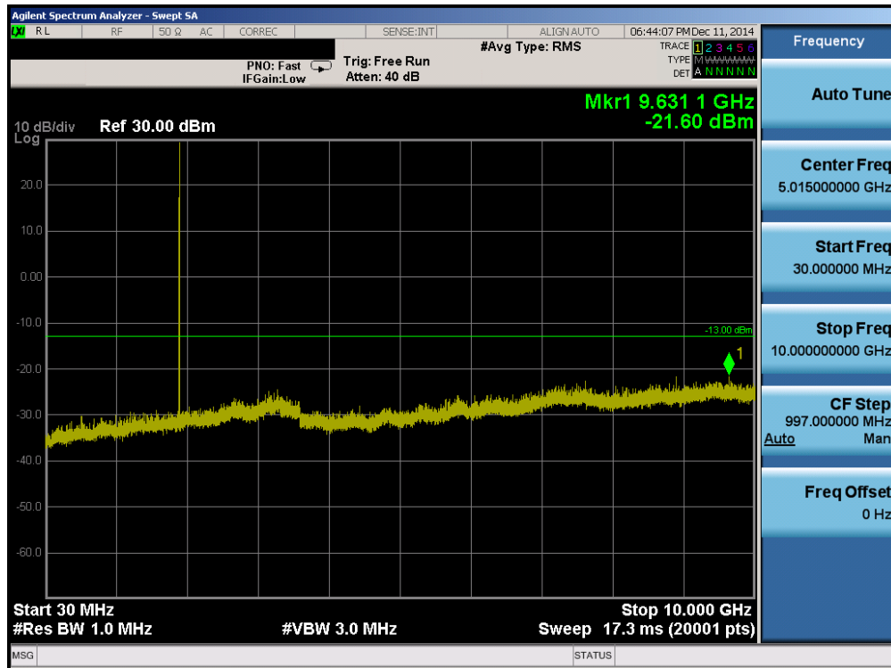
Plot 6-18. Conducted Spurious Plot (PCS GPRS Mode – Ch. 810)
