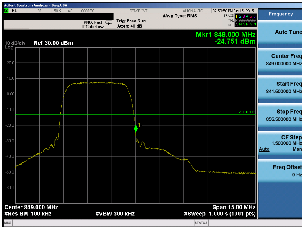
Plot 6-43. Band Edge Plot (Cellular WCDMA Mode – Ch. 4233)
