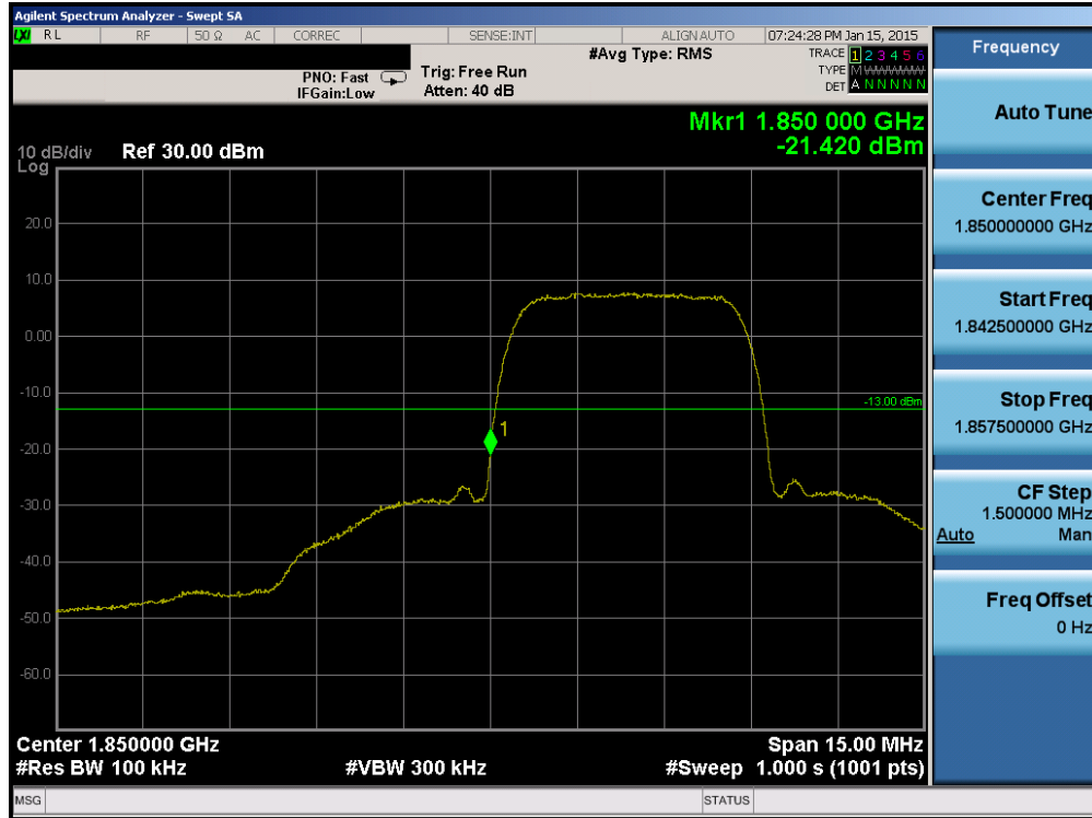
Plot 6-44. Band Edge Plot (PCS WCDMA Mode – Ch. 9262)
