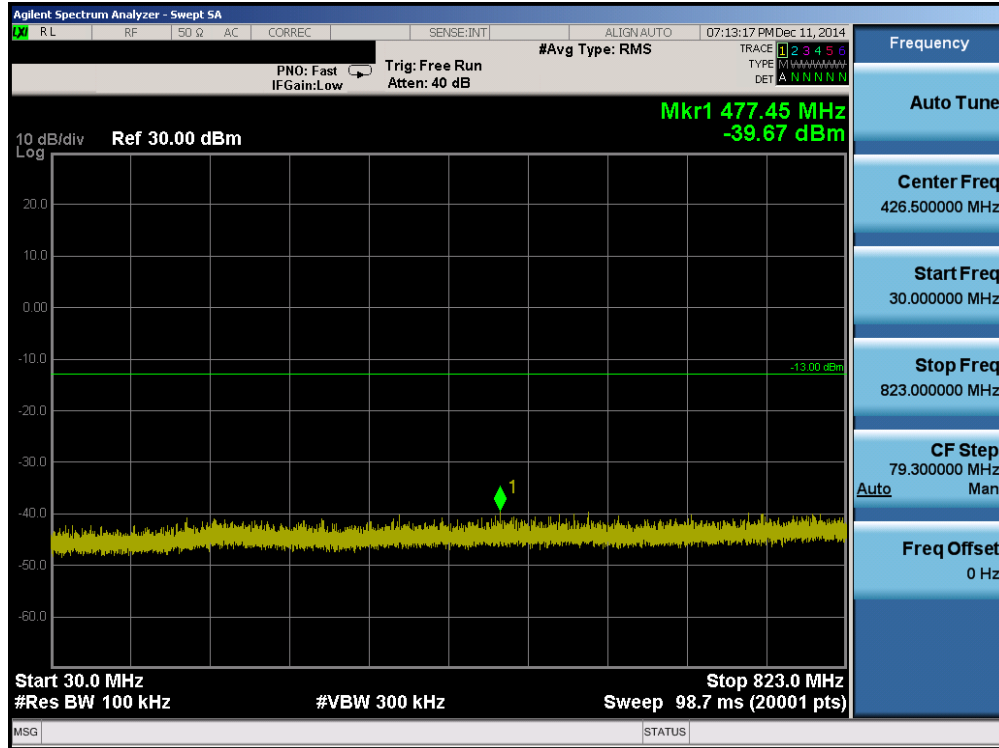
Plot 6-11. Conducted Spurious Plot (Cellular GPRS Mode – Ch. 251)
