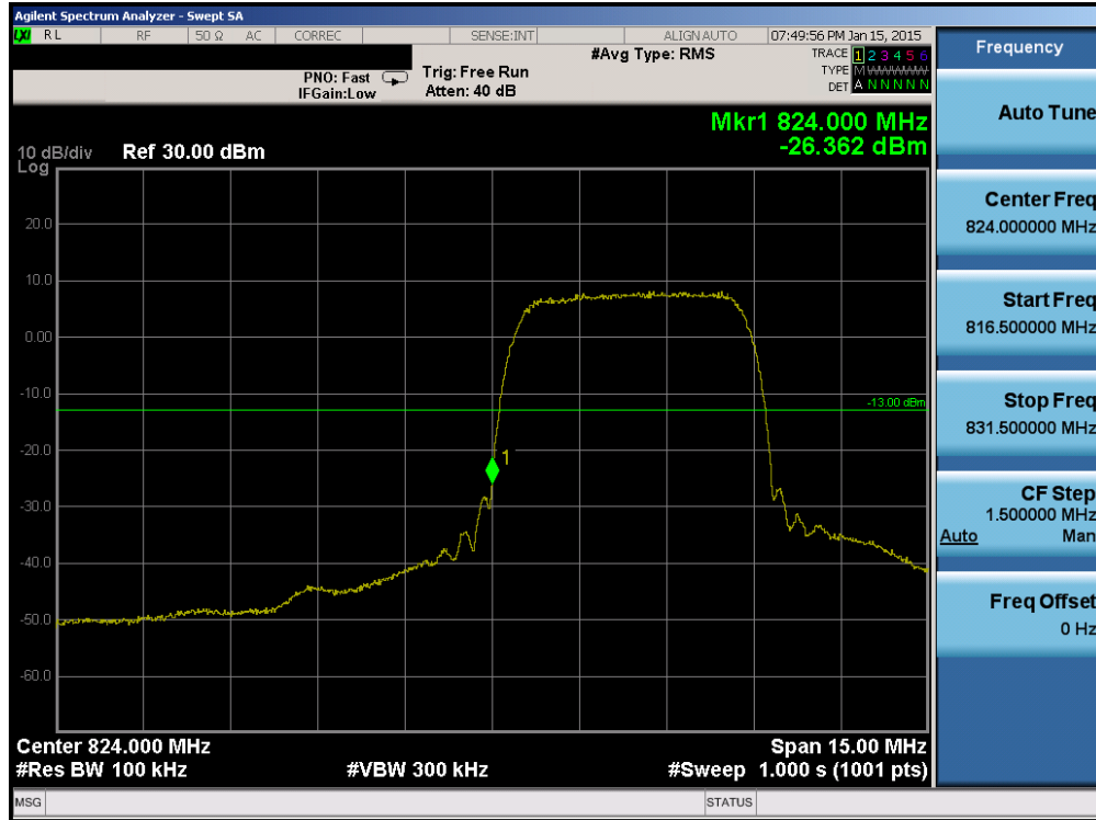
Plot 6-42. Band Edge Plot (Cellular WCDMA Mode – Ch. 4132)
