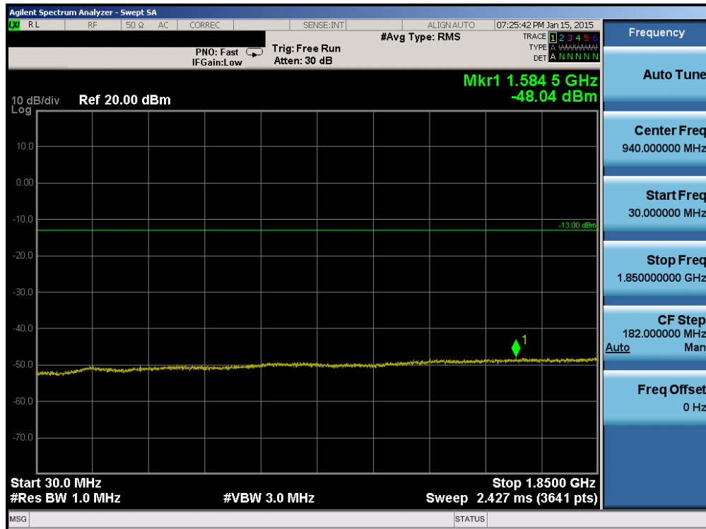
Plot 6-32. Conducted Spurious Plot (PCS WCDMA Mode - Ch. 9400)
