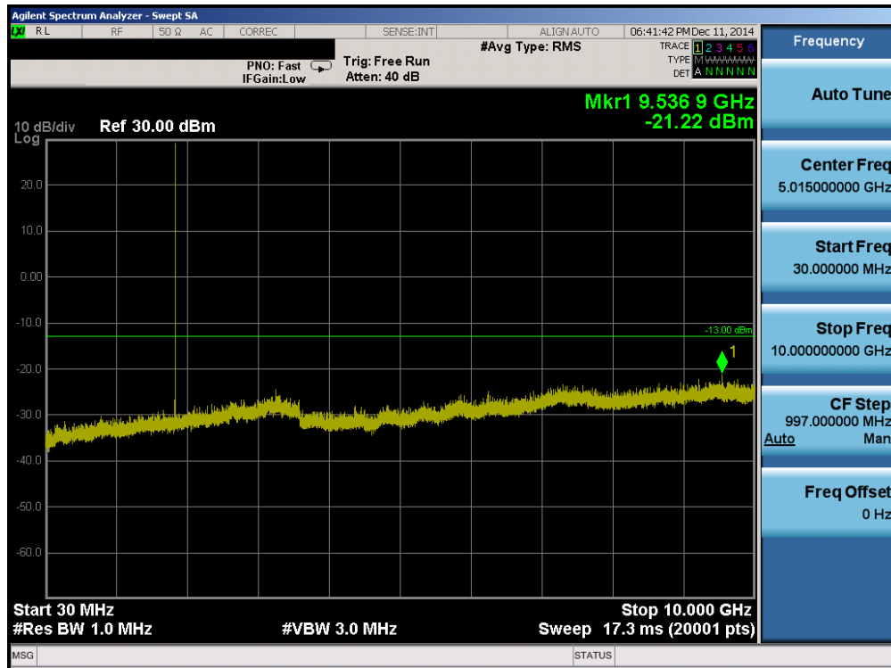
Plot 6-14. Conducted Spurious Plot (PCS GPRS Mode – Ch. 512)
