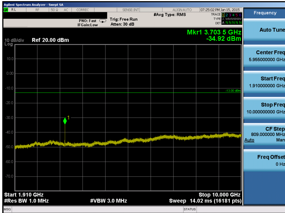
Plot 6-30. Conducted Spurious Plot (PCS WCDMA Mode – Ch. 9262)
