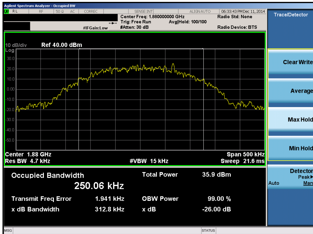
Plot 6-2. Occupied Bandwidth Plot (PCS GPRS Mode – Ch. 661)
