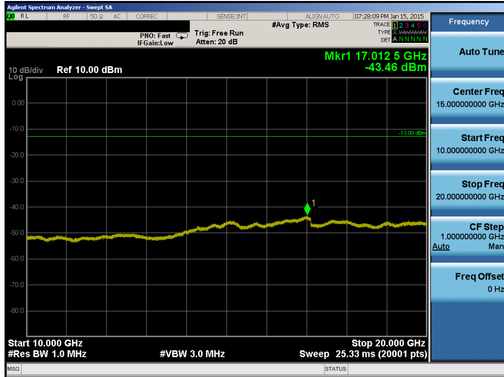
Plot 6-37. Conducted Spurious Plot (PCS WCDMA Mode – Ch. 9538)
