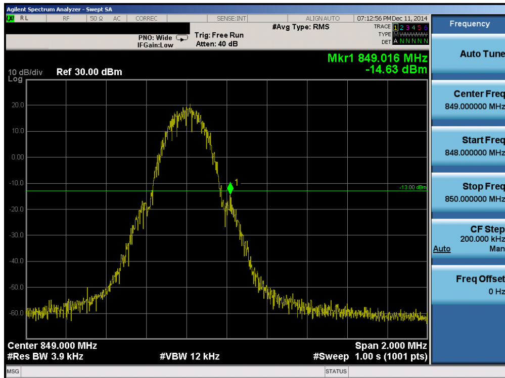
Plot 6-39. Band Edge Plot (Cellular GPRS Mode – Ch. 251)
