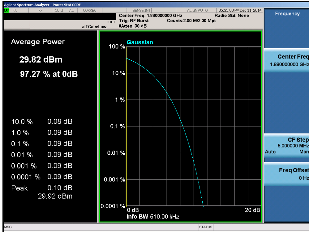
Plot 6-48. Peak-Average Ratio Plot (PCS GPRS Mode – Ch. 661)
