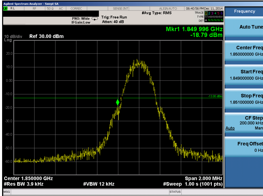
Plot 6-40. Band Edge Plot (PCS GPRS Mode – Ch. 512)
