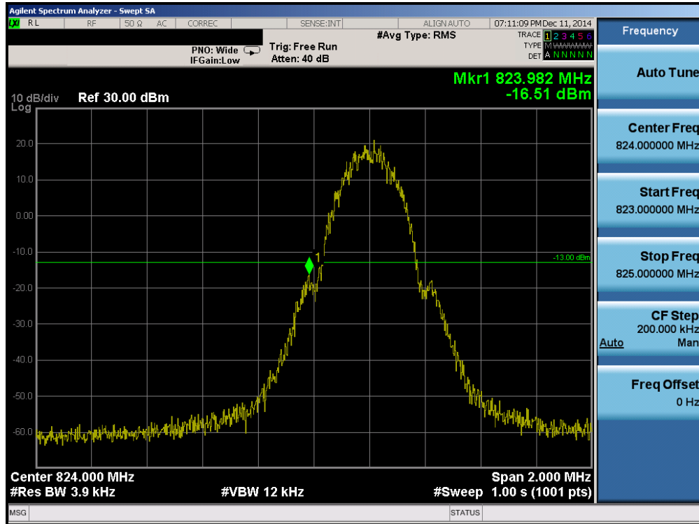
Plot 6-38. Band Edge Plot (Cellular GPRS Mode – Ch. 128)
