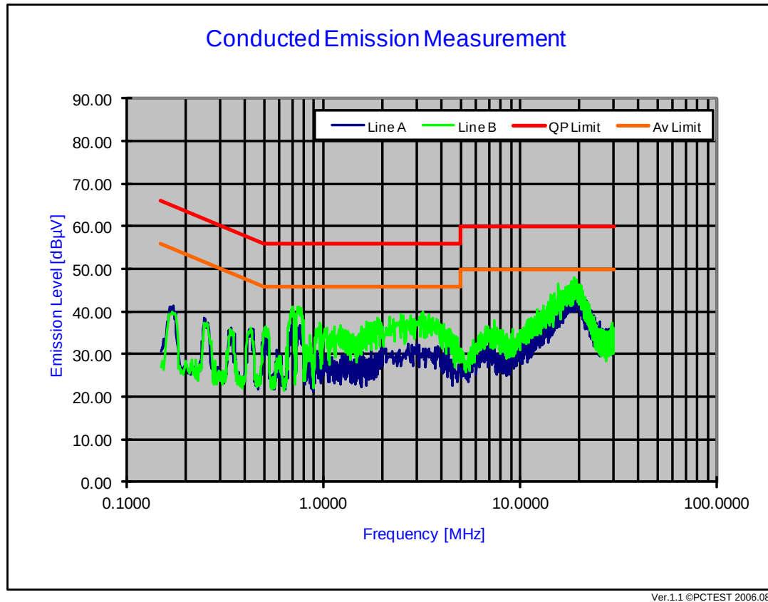
Plot 6-42. Line Conducted Plot with Bluetooth
