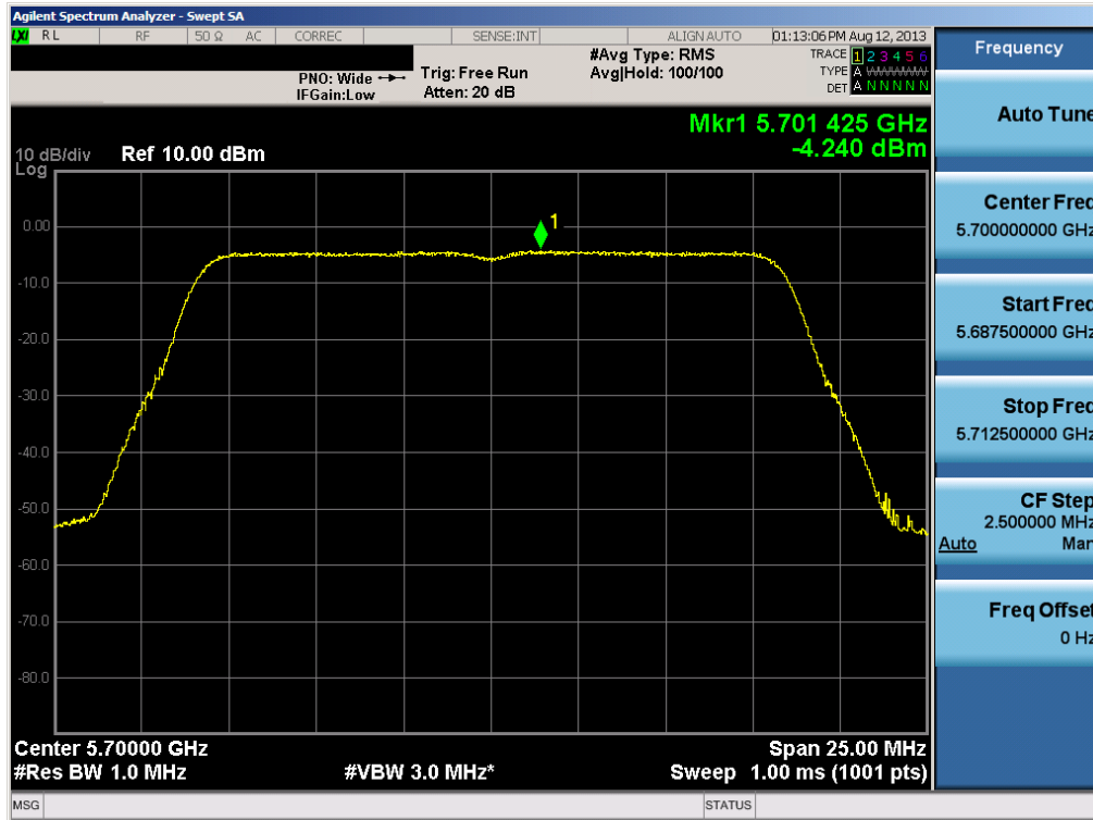
Plot 6-45. Peak Power Spectral Density Plot (802.11a (UNII Band 3) – Ch. 140)
