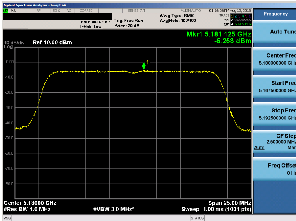
Plot 6-30. Peak Power Spectral Density Plot (20MHz BW 802.11n (UNII Band 1) – Ch. 36)
