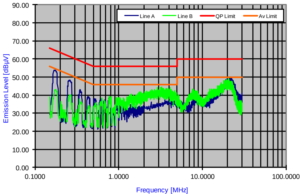
Plot 6-55. Line Conducted Plot with 802.11a (UNII Band 1)
