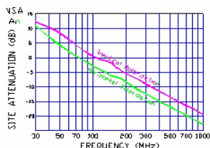
Figure 3-8. Normalized Site Attenuation Curves (H&V)
