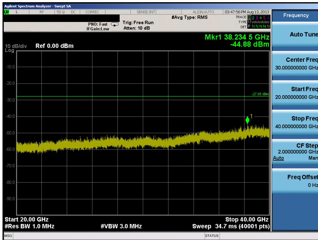
Plot 6-58. Conducted Spurious Plot (802.11a – Ch. 165)
