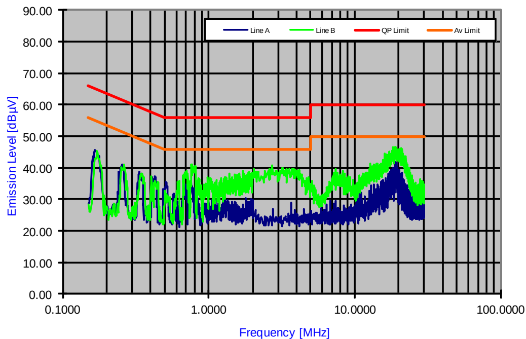
Plot 6-61. Line Conducted Plot with 802.11b
