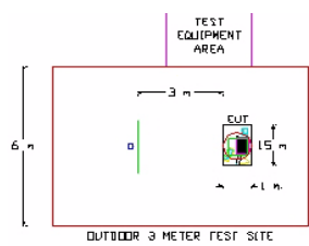
Figure 3-6. Dimensions of Outdoor Test Site
