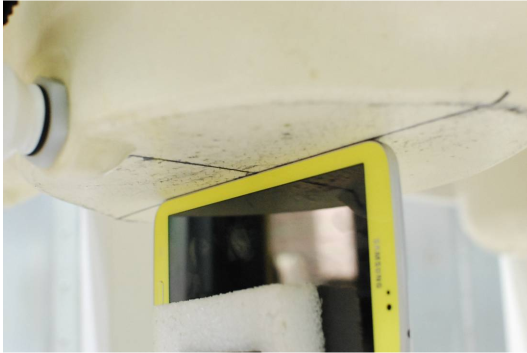
SAR Test Setup Photo 3 - Left Side at 0.0 cm
