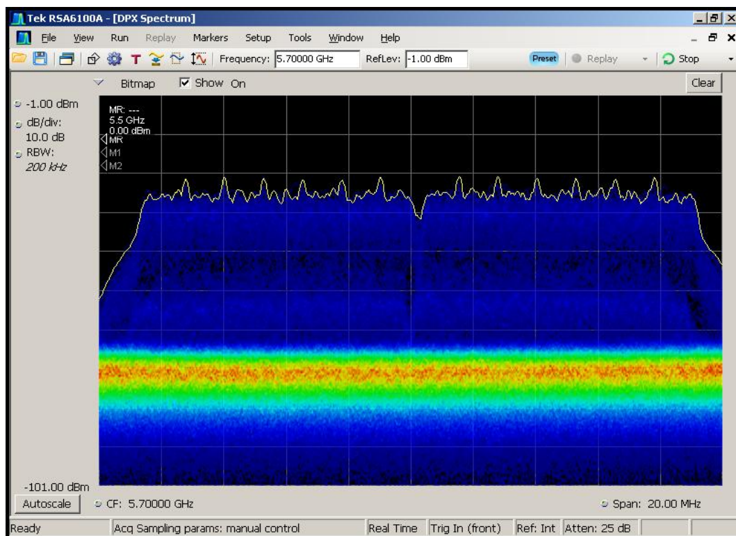
Figure 6-4. Real-Time Spectrum Display, WLAN Traffic (Streaming Video)
