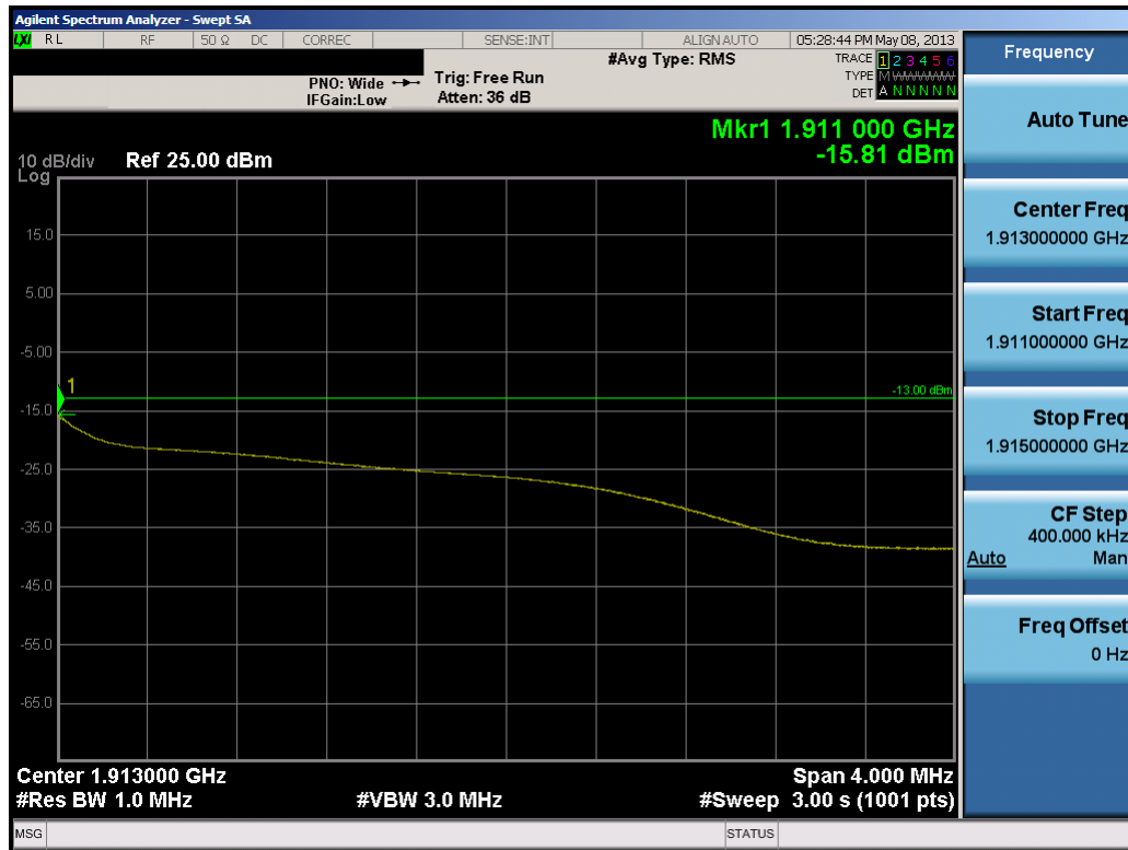
Plot 7-43. 4MHz Span Plot (PCS WCDMA Mode – Ch. 9538)
