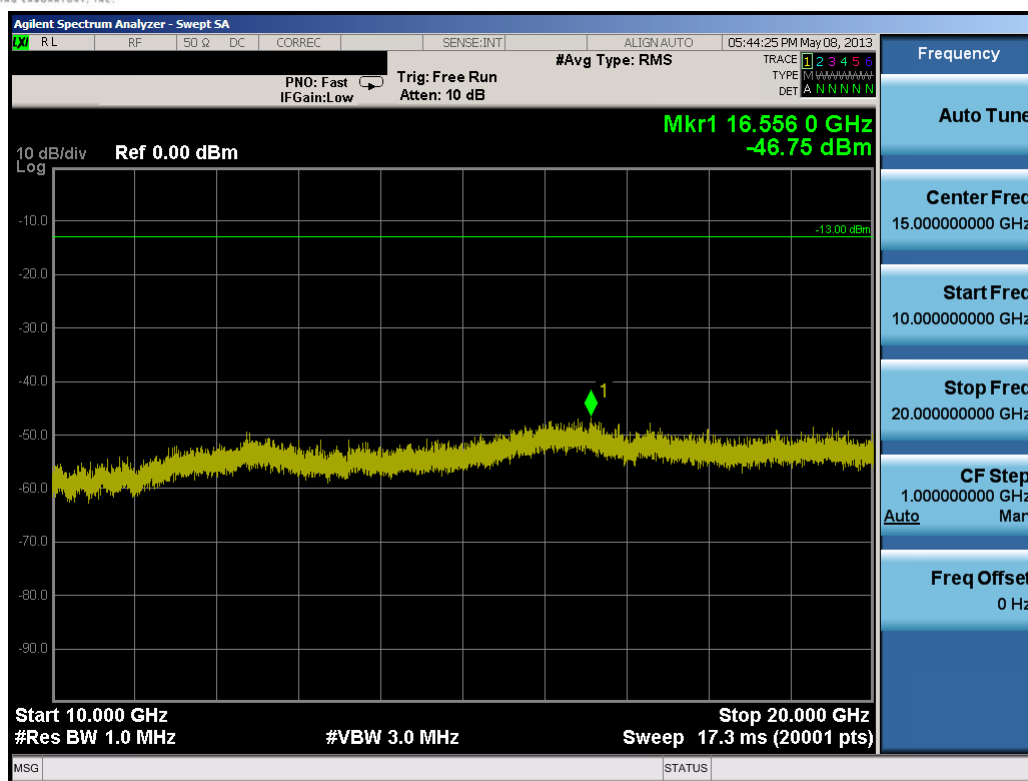
Plot 7-14. Conducted Spurious Plot (PCS GSM Mode – Ch. 512)
