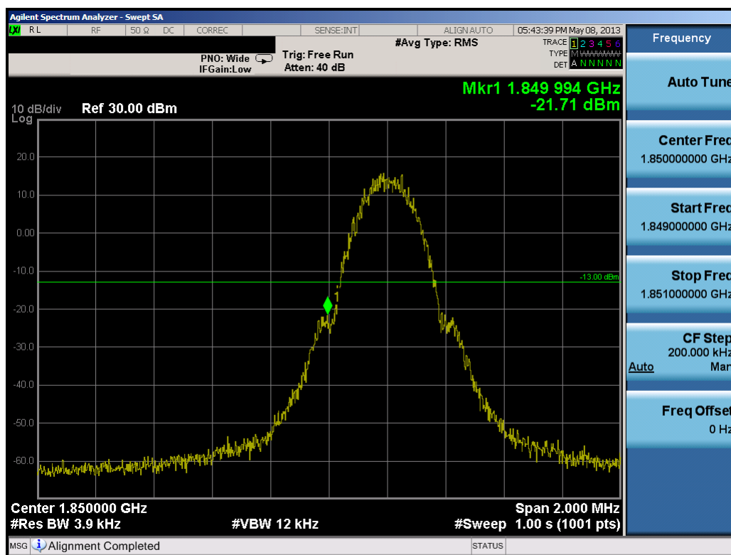
Plot 7-15. Band Edge Plot (PCS GSM Mode – Ch. 512)
