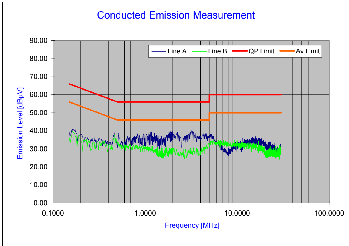
Plot 6-18. Line Conducted Plot with Bluetooth LE
