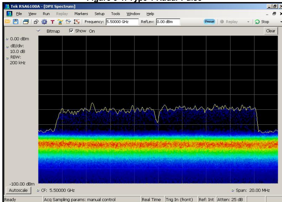
Figure 6-2. Real-Time Spectrum Display, No WLAN Traffic
