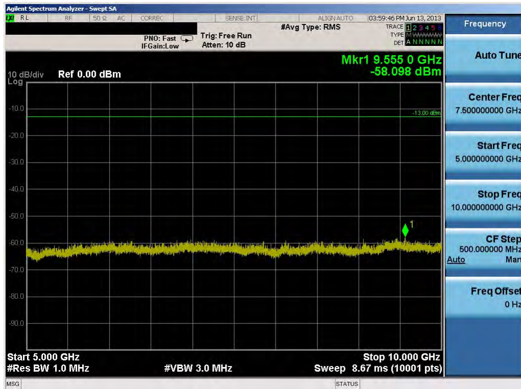
Plot 8-34. Conducted Spurious Plot (10.0MHz QPSK – RB Size 1, RB Offset 0 – High Channel)
