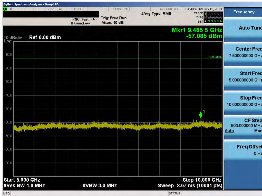
Plot 8-10. Conducted Spurious Plot (3.0MHz QPSK – RB Size 1, RB Offset 0 – High Channel)
