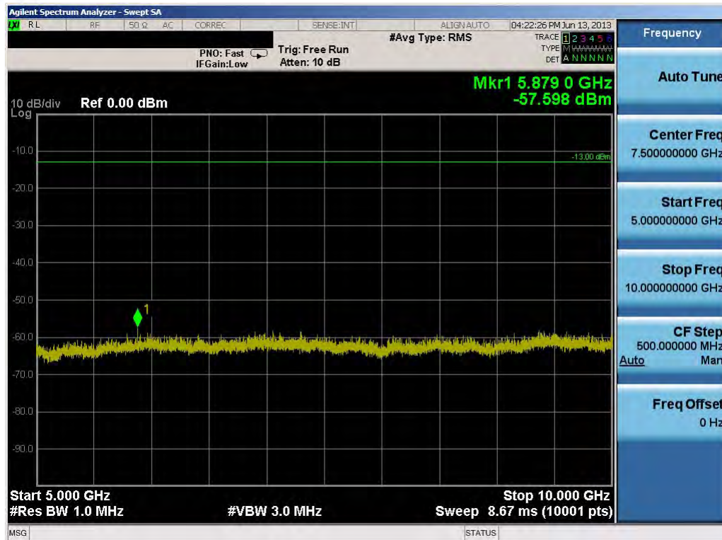
Plot 8-18. Conducted Spurious Plot (5.0MHz QPSK – RB Size 1, RB Offset 0 – Low Channel)
