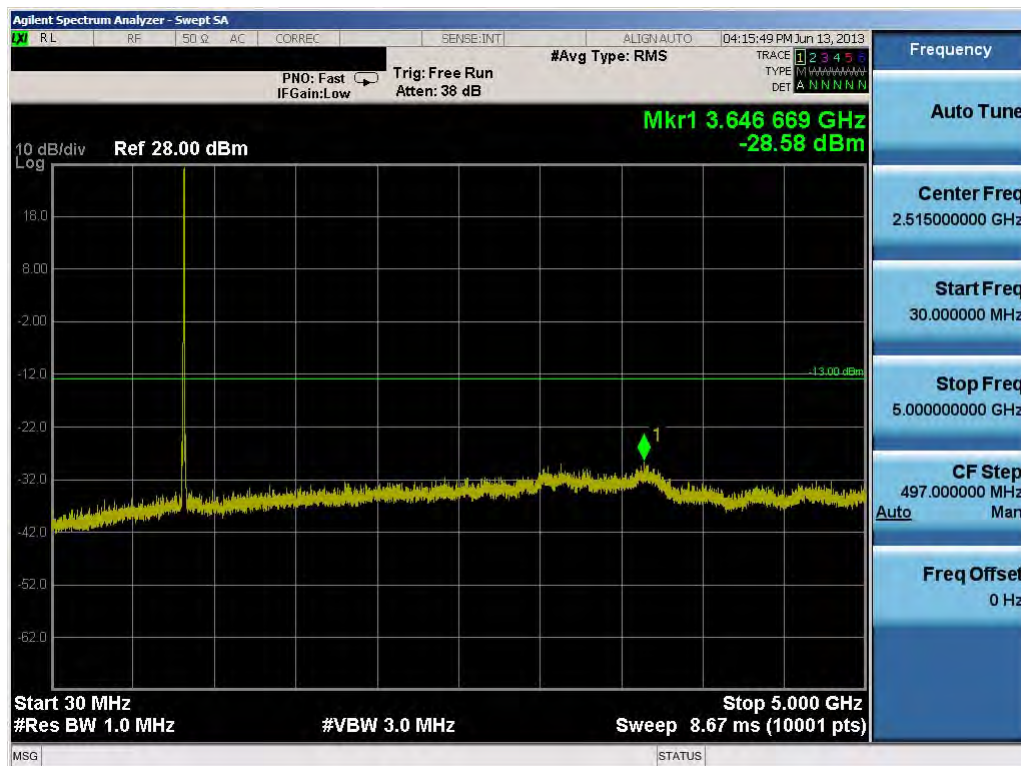
Plot 8-19. Conducted Spurious Plot (5.0MHz QPSK – RB Size 1, RB Offset 0 – Mid Channel)
