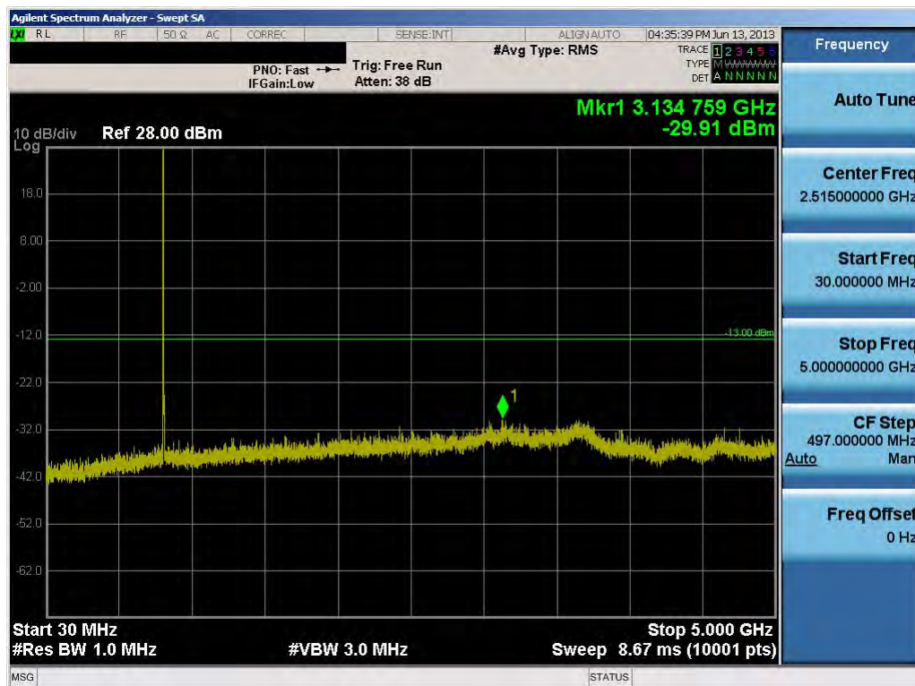
Plot 8-5. Conducted Spurious Plot (3.0MHz QPSK – RB Size 1, RB Offset 0 – Low Channel)
