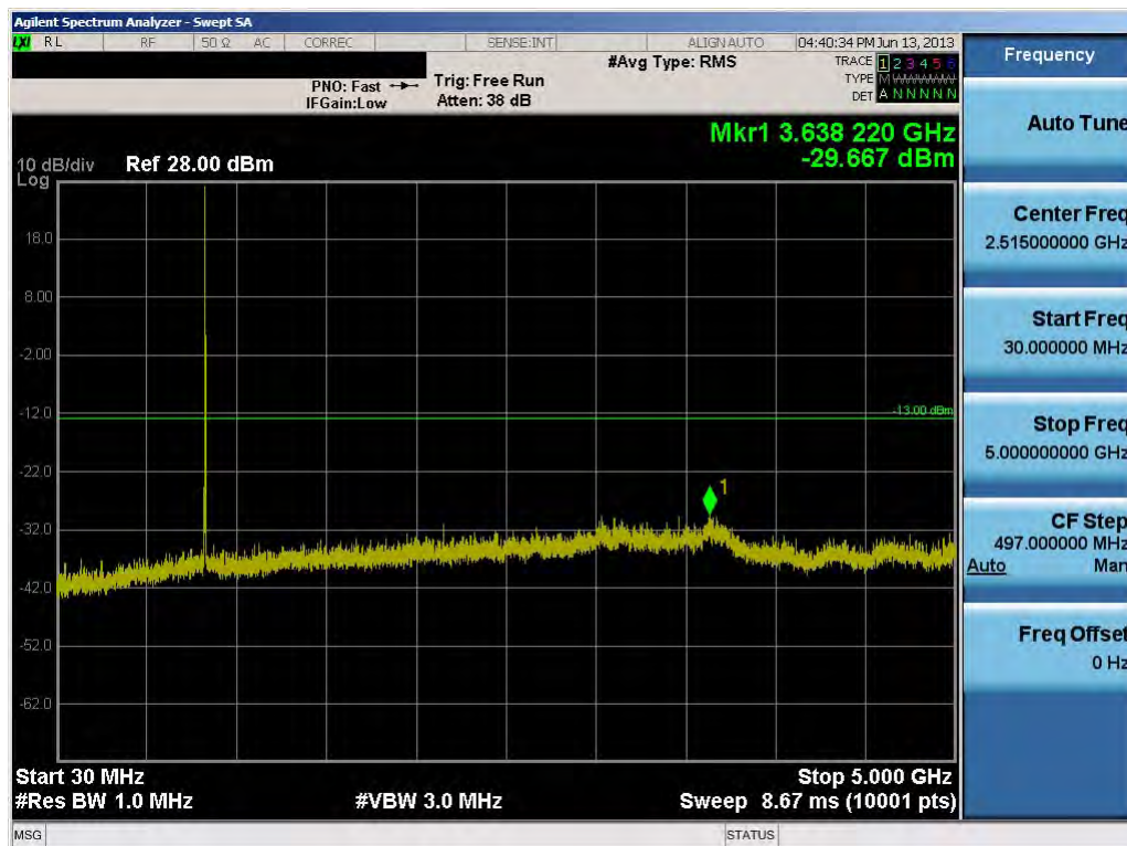
Plot 8-9. Conducted Spurious Plot (3.0MHz QPSK – RB Size 1, RB Offset 0 – High Channel)
