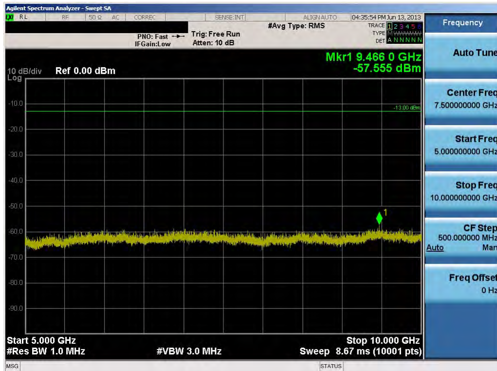
Plot 8-6. Conducted Spurious Plot (3.0MHz QPSK – RB Size 1, RB Offset 0 – Low Channel)
