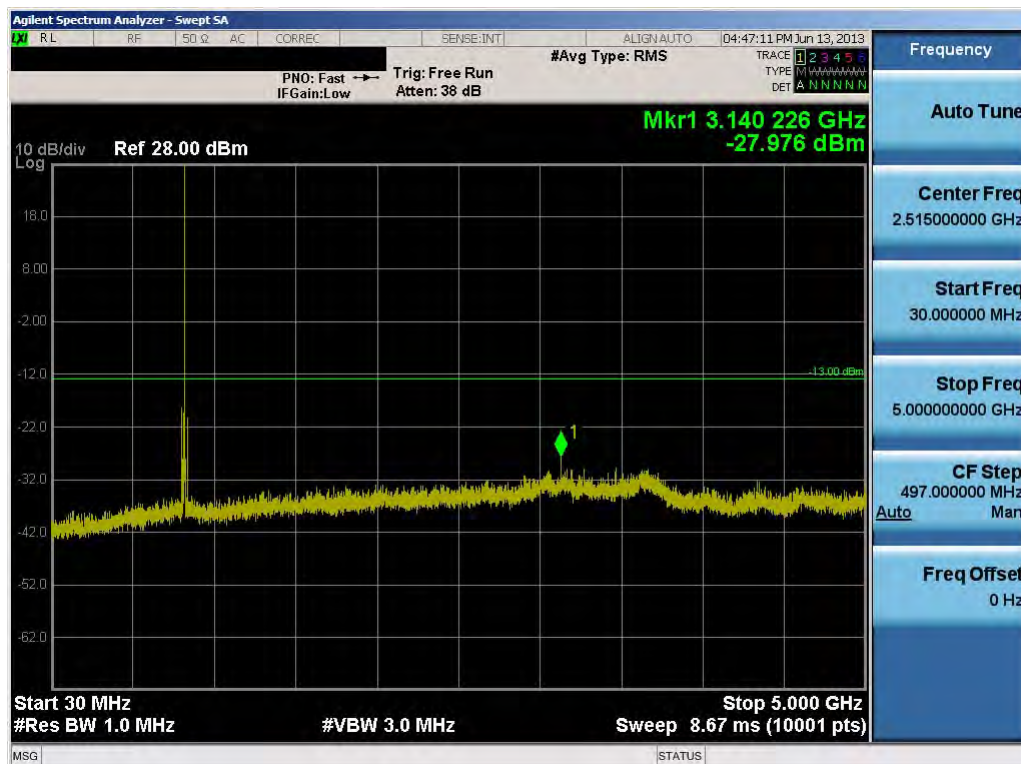
Plot 8-31. Conducted Spurious Plot (10.0MHz QPSK – RB Size 1, RB Offset 0 – Mid Channel)
