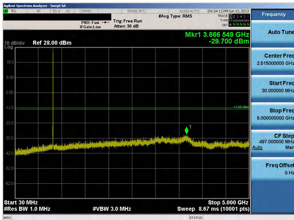
Plot 8-7. Conducted Spurious Plot (3.0MHz QPSK – RB Size 1, RB Offset 0 – Mid Channel)
