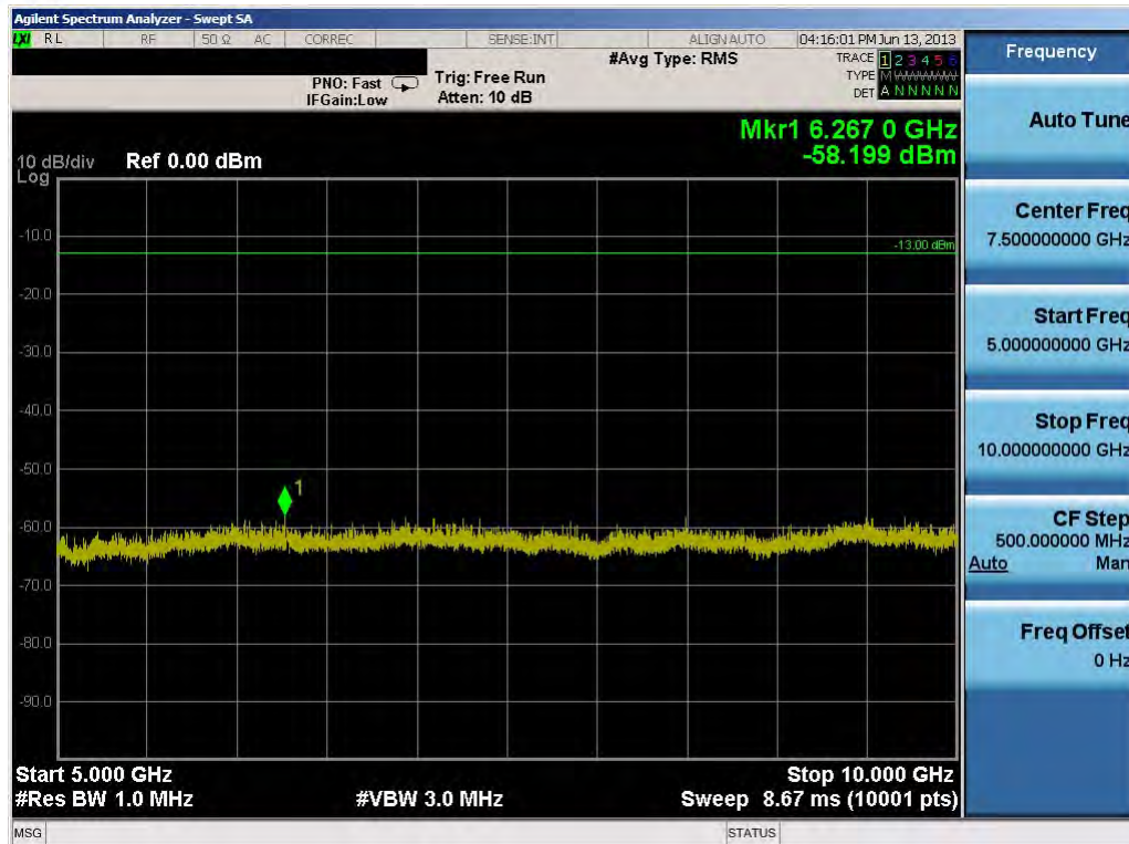
Plot 8-20. Conducted Spurious Plot (5.0MHz QPSK – RB Size 1, RB Offset 0 – Mid Channel)
