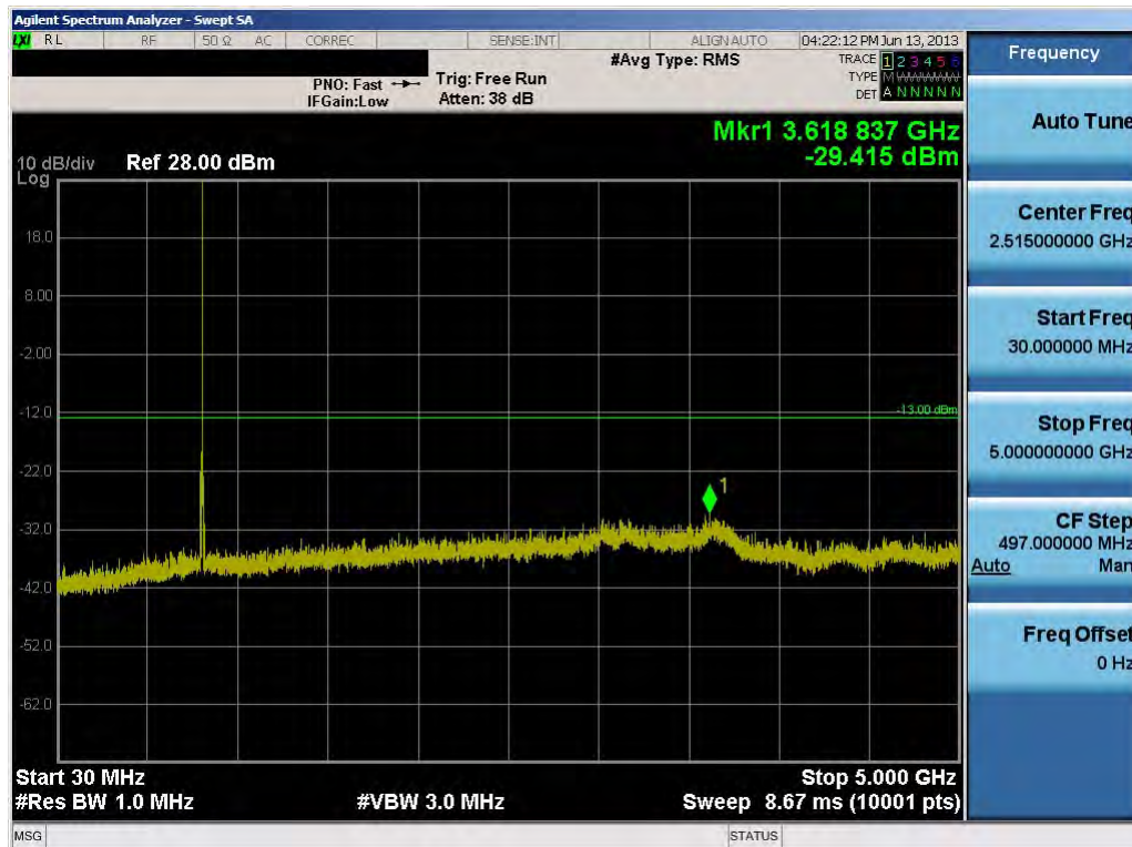
Plot 8-17. Conducted Spurious Plot (5.0MHz QPSK – RB Size 1, RB Offset 0 – Low Channel)
