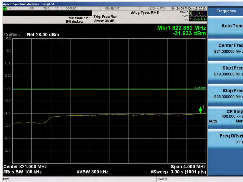
Plot 8-14. Lower Extended Band Edge Plot (5.0MHz QPSK – RB Size 25)
