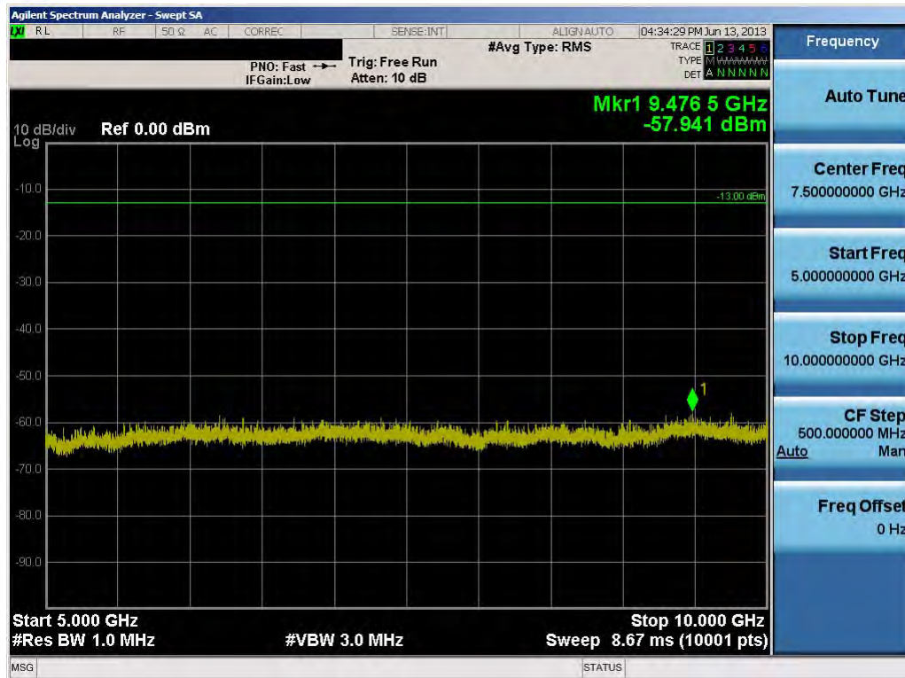
Plot 8-8. Conducted Spurious Plot (3.0MHz QPSK – RB Size 1, RB Offset 0 – Mid Channel)
