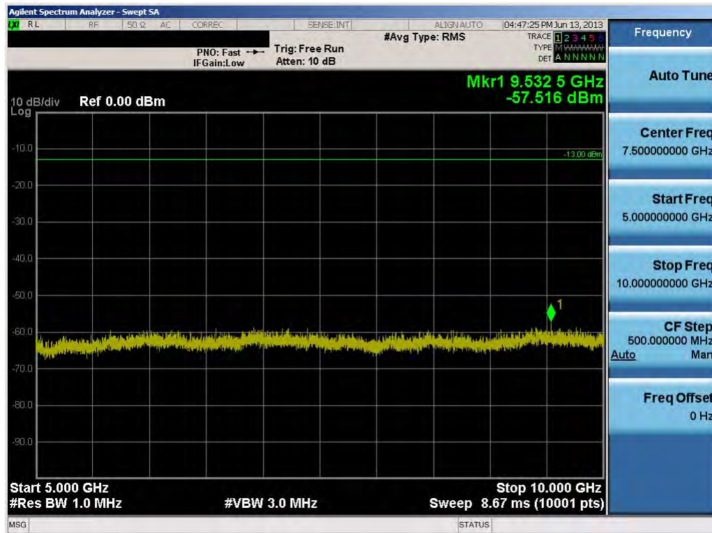
Plot 8-32. Conducted Spurious Plot (10.0MHz QPSK – RB Size 1, RB Offset 0 – Mid Channel)
