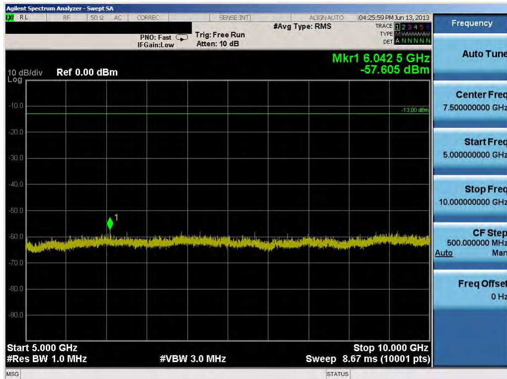
Plot 8-22. Conducted Spurious Plot (5.0MHz QPSK – RB Size 1, RB Offset 0 – High Channel)
