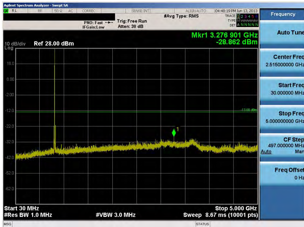
Plot 8-29. Conducted Spurious Plot (10.0MHz QPSK – RB Size 1, RB Offset 0– Low Channel)
