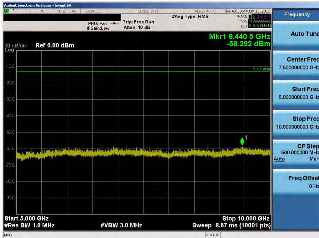
Plot 8-30. Conducted Spurious Plot (10.0MHz QPSK – RB Size 1, RB Offset 0 – Low Channel)
