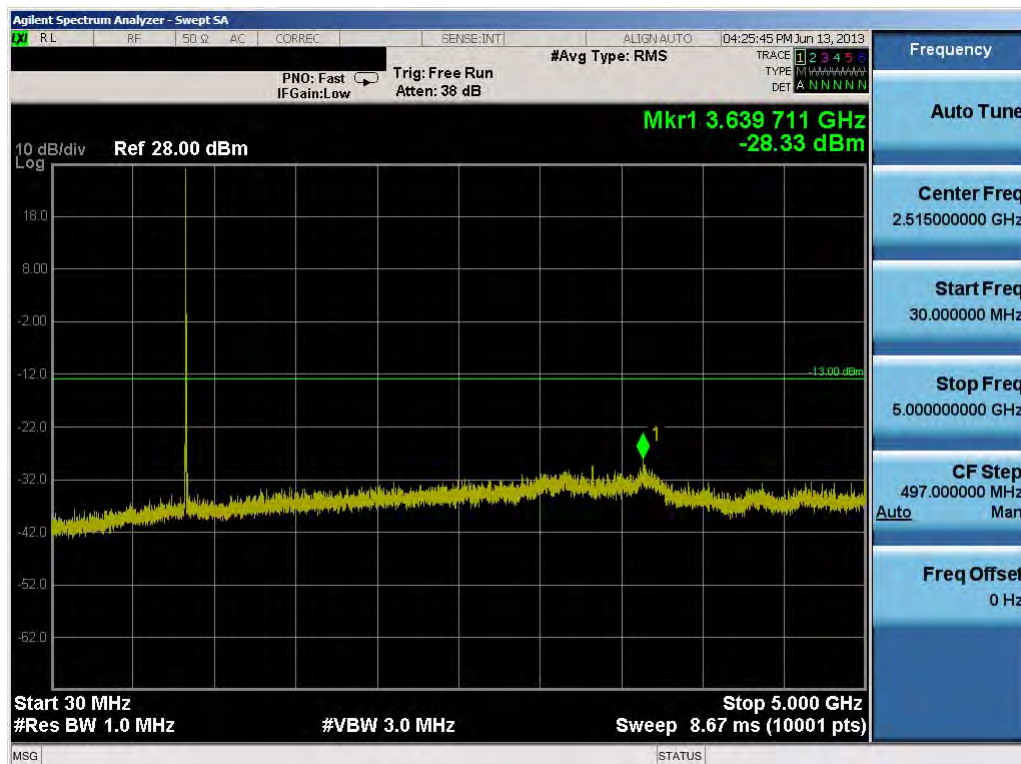
Plot 8-21. Conducted Spurious Plot (5.0MHz QPSK – RB Size 1, RB Offset 0 – High Channel)
