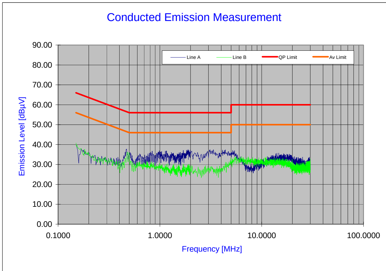
Plot 6-60. Line Conducted Plot with 802.11a
