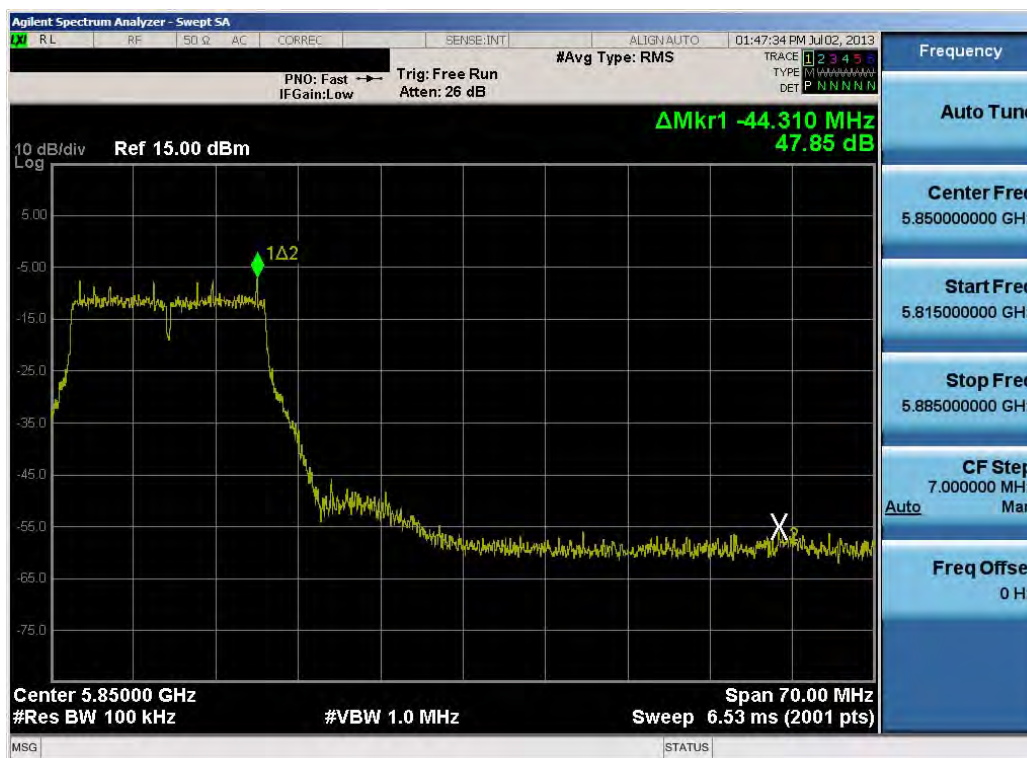
Plot 6-42. Band Edge Plot (802.11a – Ch. 165)
