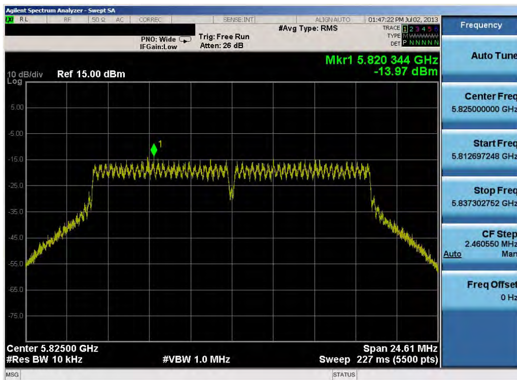
Plot 6-29. Power Spectral Density Plot (802.11a – Ch. 165)
