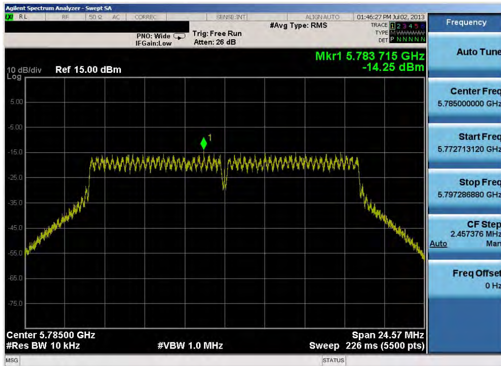
Plot 6-28. Power Spectral Density Plot (802.11a – Ch. 157)
