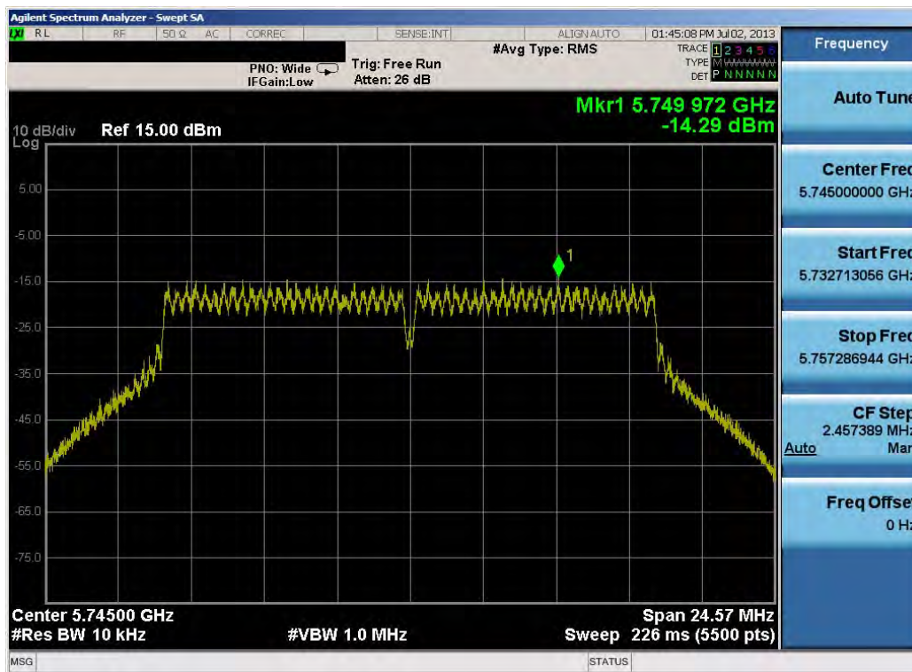
Plot 6-27. Power Spectral Density Plot (802.11a – Ch. 149)
