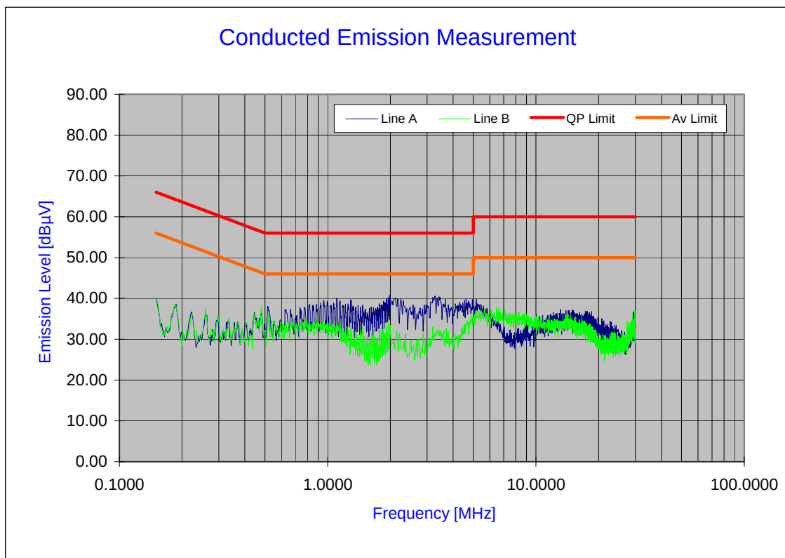
Plot 6-55. Line Conducted Plot with 802.11a UNII Band
