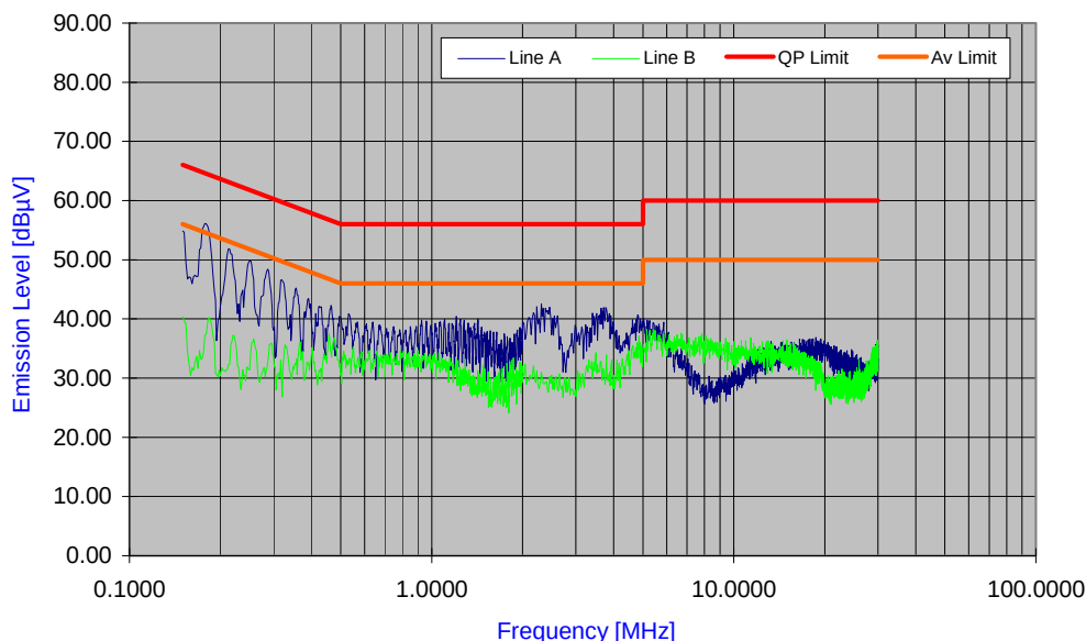
Plot 6-54. Line Conducted Plot with 802.11a UNII Band 1
