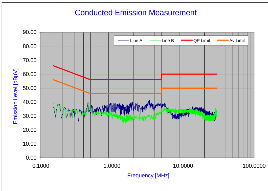
Plot 6-56. Line Conducted Plot with 802.11a UNII Band 3
