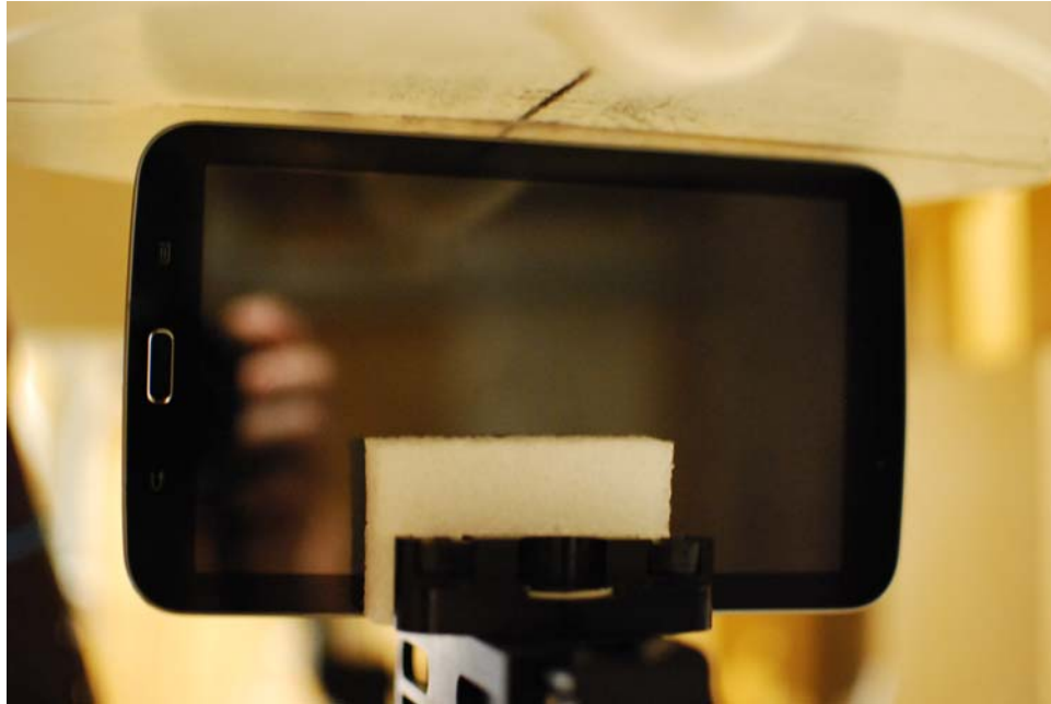
SAR Test Setup Photo 7: Left at 0.4 cm
