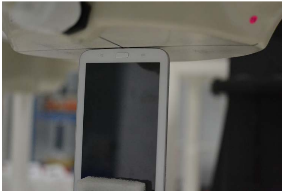
SAR Test Setup Photo 2 – Bottom Edge at 0.0 cm
