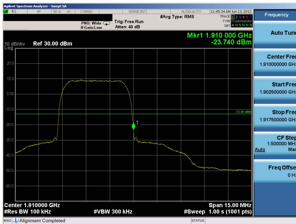
Plot 6-30. Band Edge Plot (PCS WCDMA Mode – Ch. 9538)
