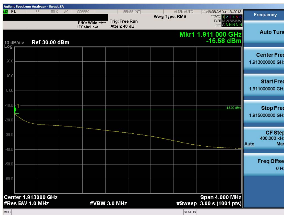
Plot 6-31. 4MHz Span Plot (PCS WCDMA Mode – Ch. 9538)
