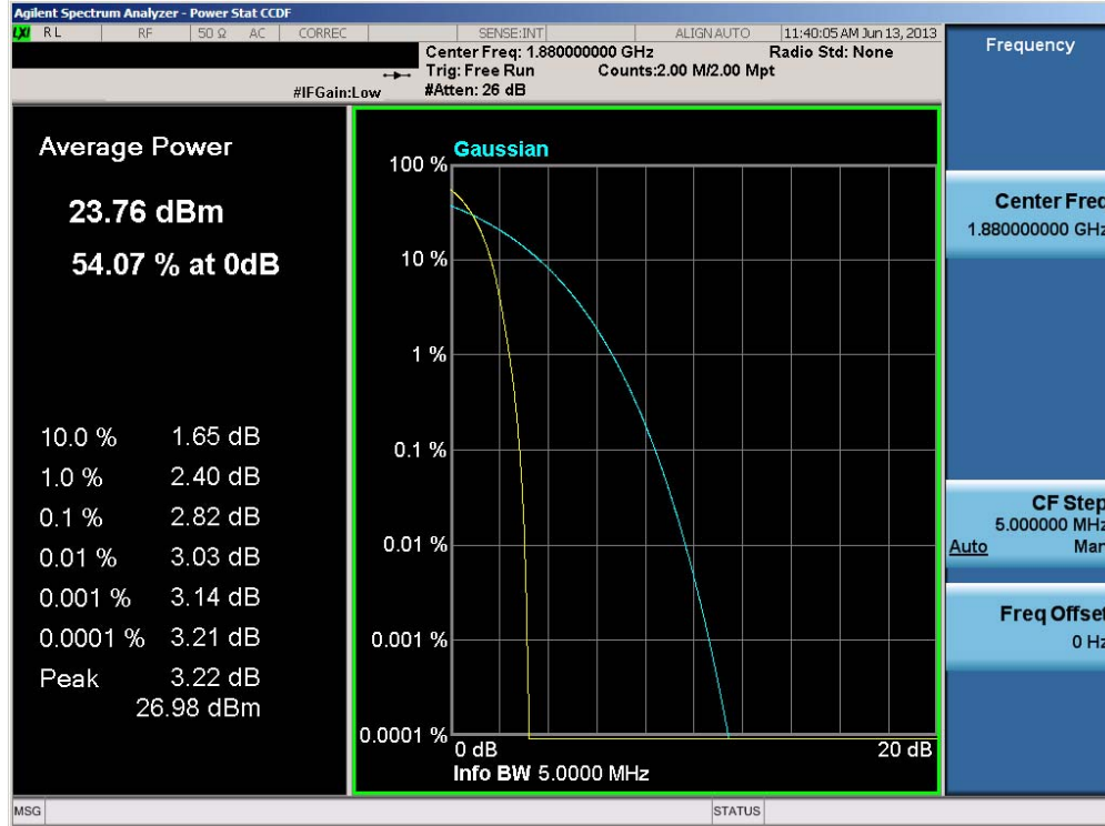
Plot 6-33. Peak-Average Ratio Plot (PCS WCDMA Mode – Ch. 9400)
