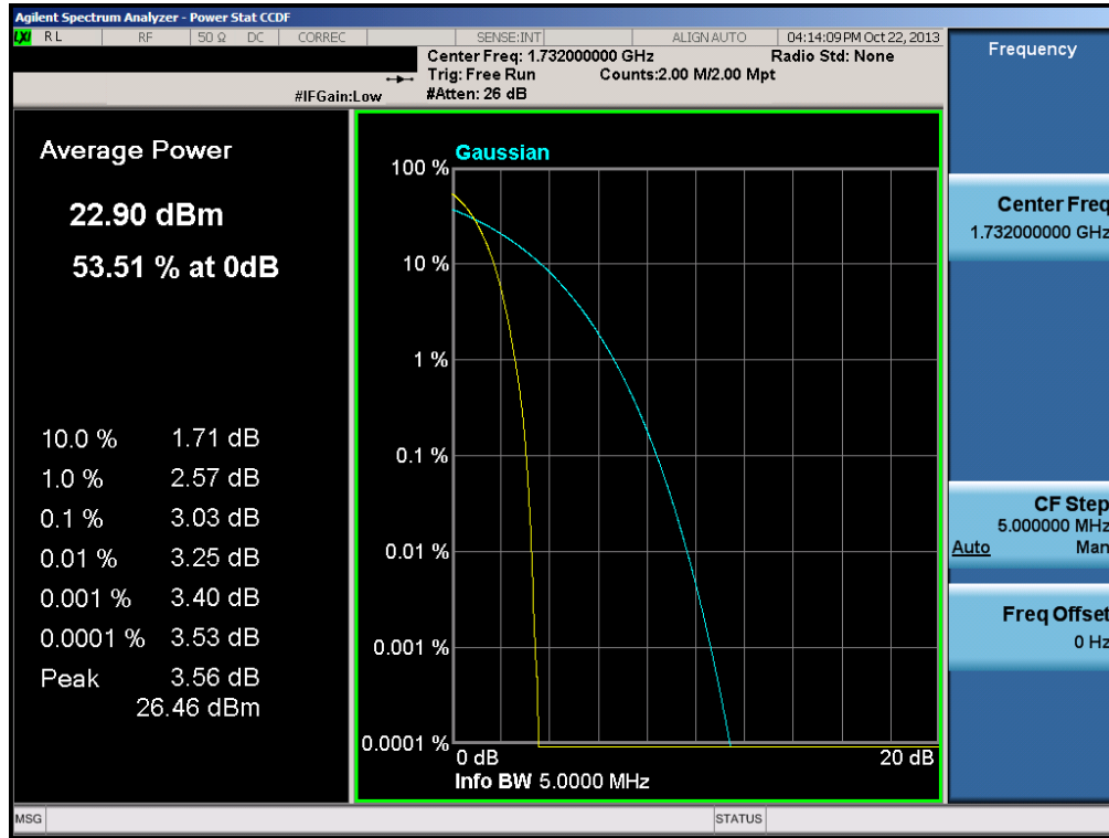
Plot 6-32. Peak-Average Ratio Plot (AWS WCDMA Mode – Ch. 1412)
