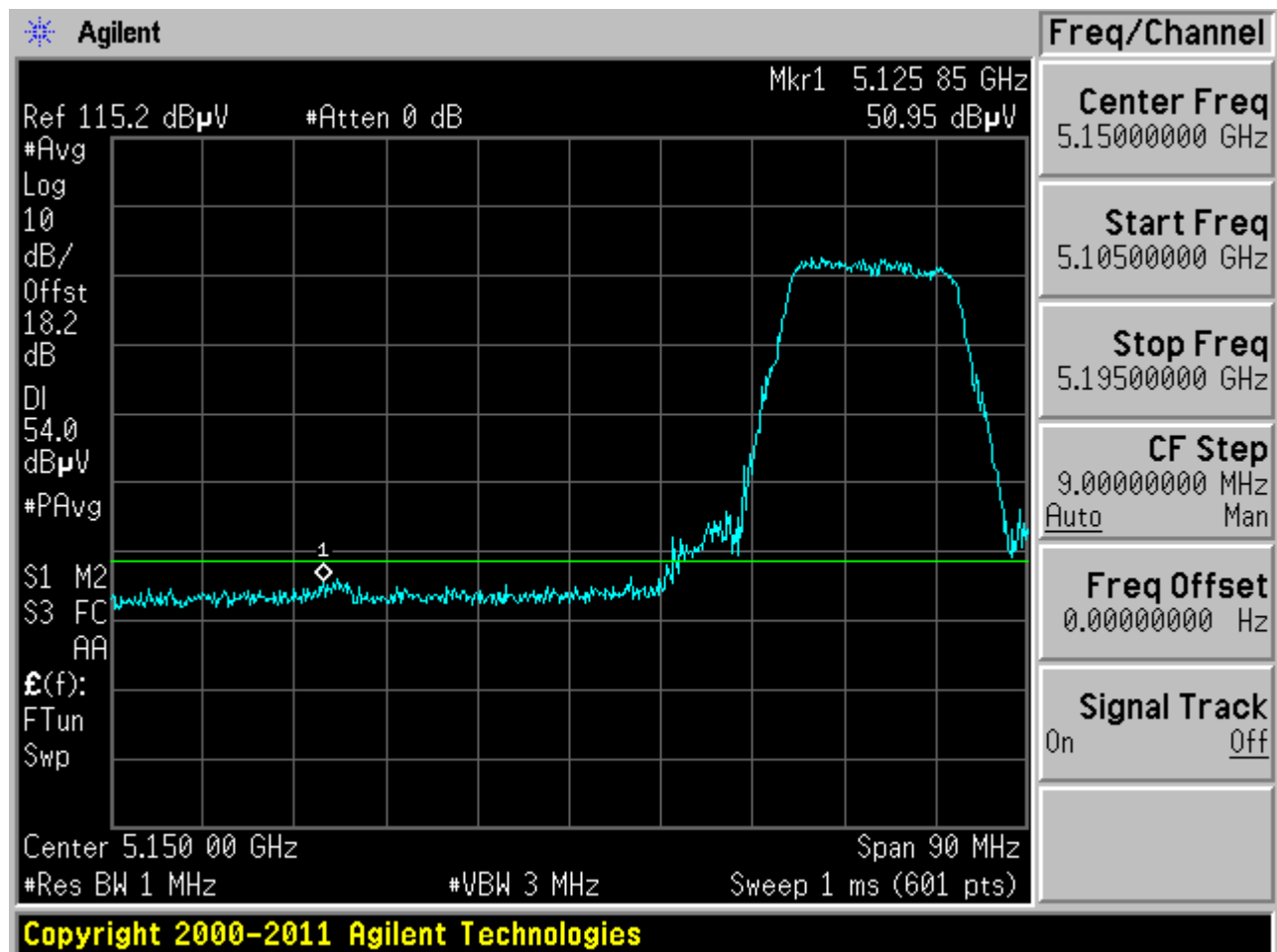
Plot 6-54. Radiated Restricted Lower Band Edge Plot (Average – UNII Band 1)
