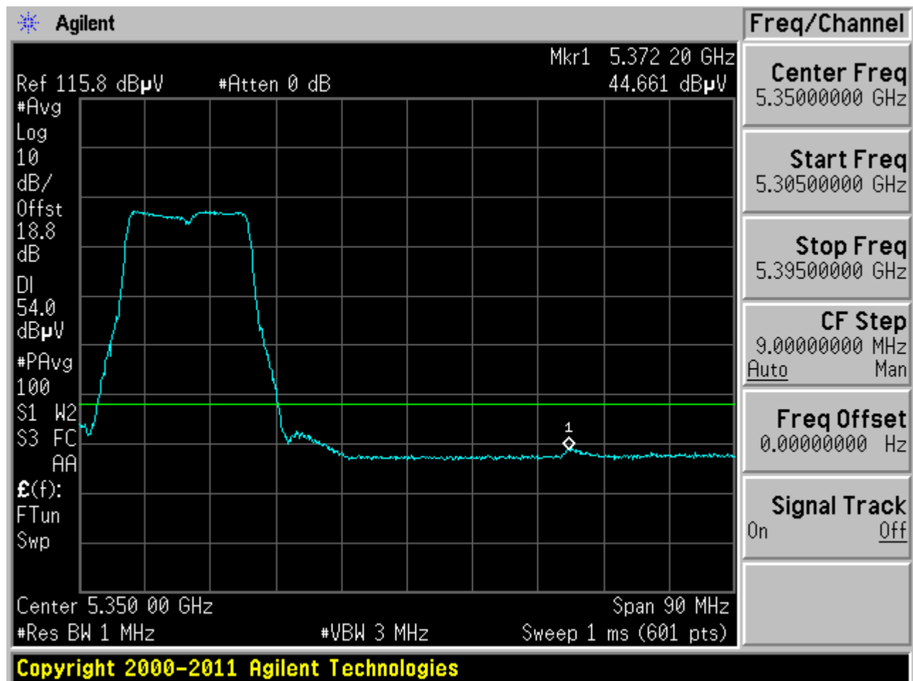
Plot 6-56. Radiated Restricted Upper Band Edge Plot (Average – UNII Band 2)
