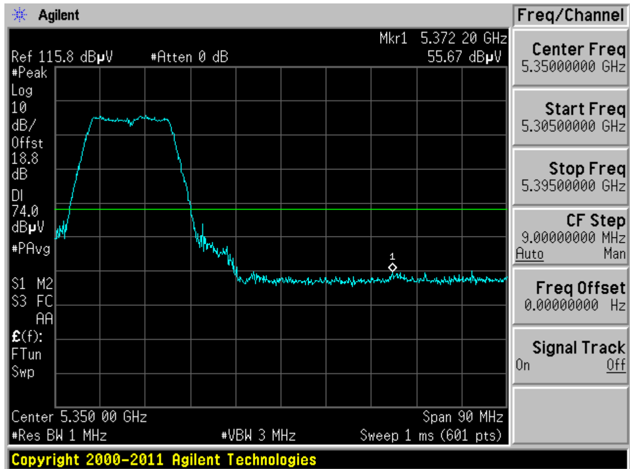
Plot 6-57. Radiated Restricted Upper Band Edge Plot (Peak – UNII Band 2)
