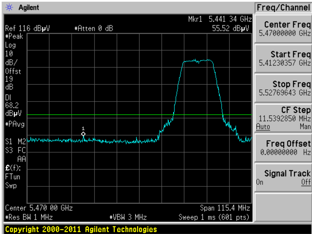
Plot 6-59. Radiated Restricted Lower Band Edge Plot (Peak – UNII Band 3)
