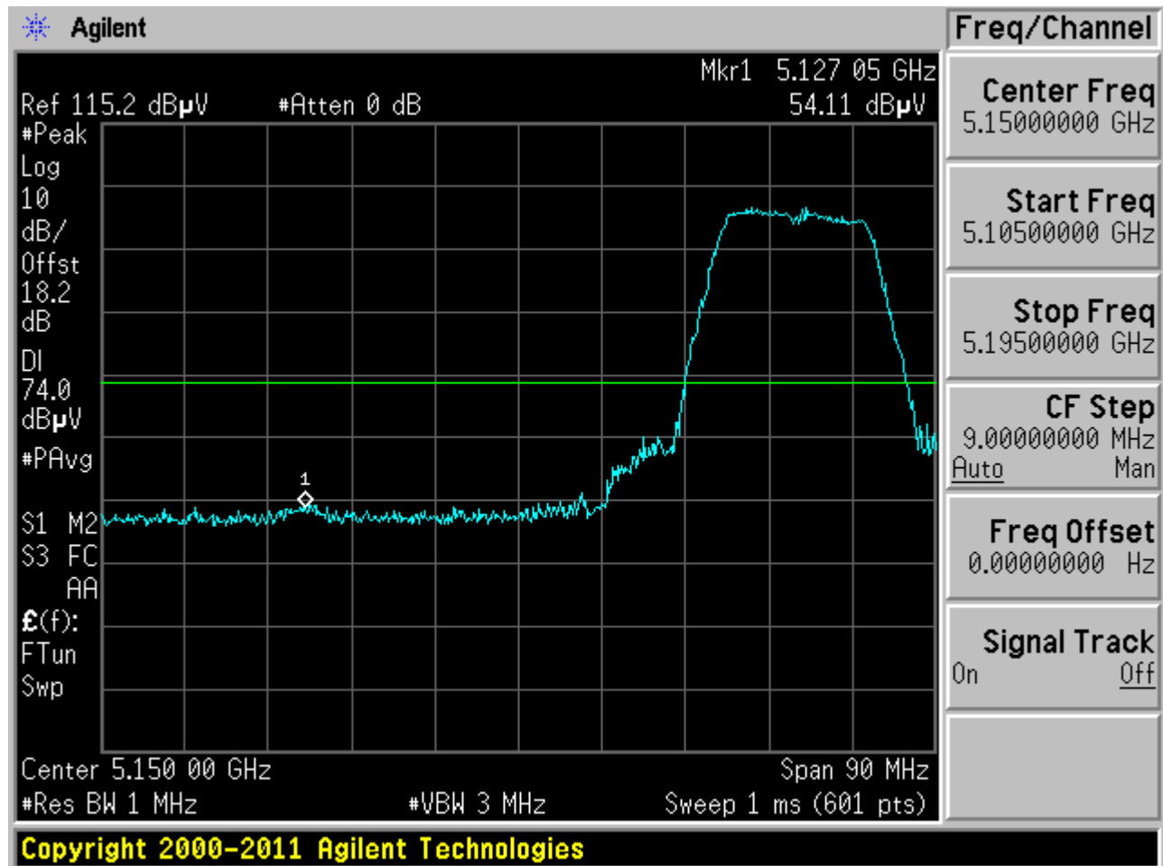
Plot 6-55. Radiated Restricted Lower Band Edge Plot (Peak – UNII Band 1)
