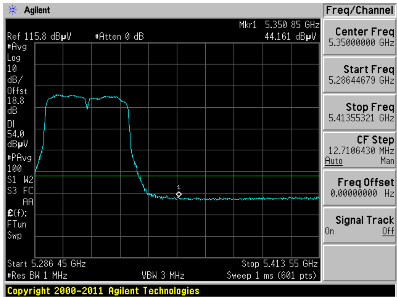
Plot 6-63. Radiated Restricted Upper Band Edge Plot (Average – UNII Band 2)
