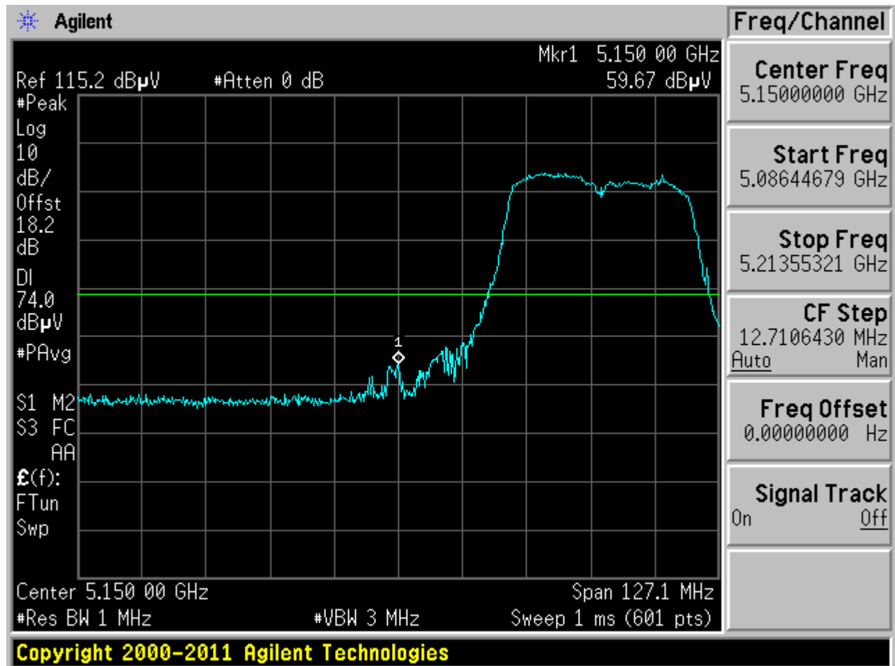
Plot 6-62. Radiated Restricted Lower Band Edge Plot (Peak – UNII Band 1)
