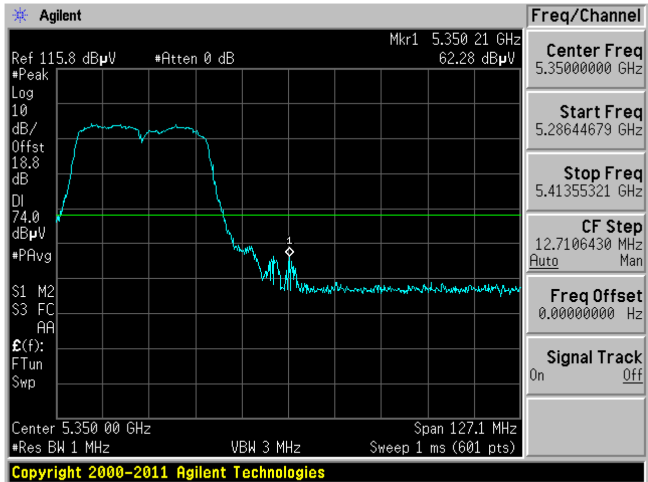
Plot 6-64. Radiated Restricted Upper Band Edge Plot (Peak – UNII Band 2)
