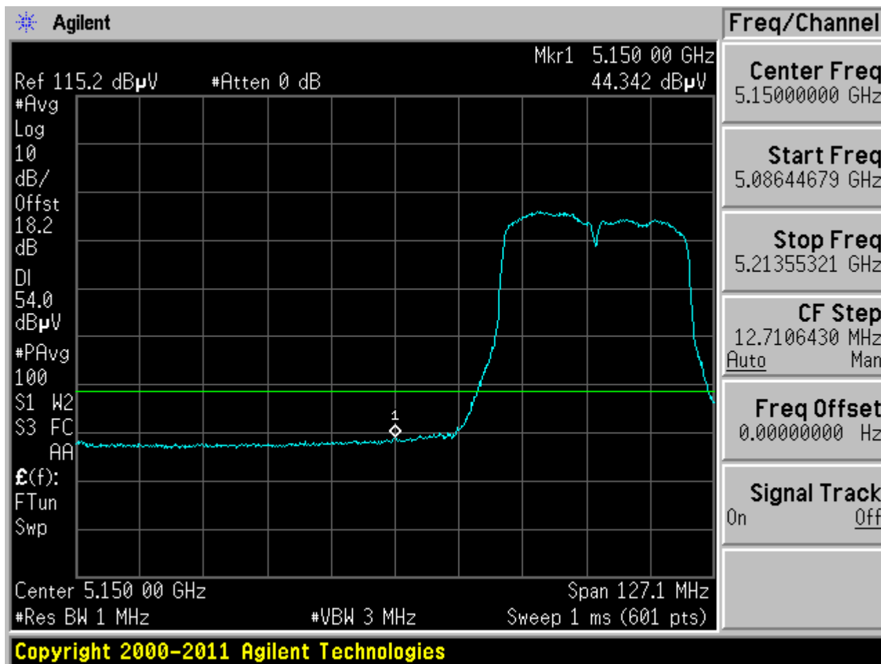
Plot 6-61. Radiated Restricted Lower Band Edge Plot (Average – UNII Band 1)
