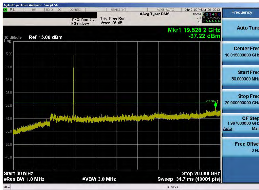
Plot 6-57. Conducted Spurious Plot (802.11a – Ch. 165)
