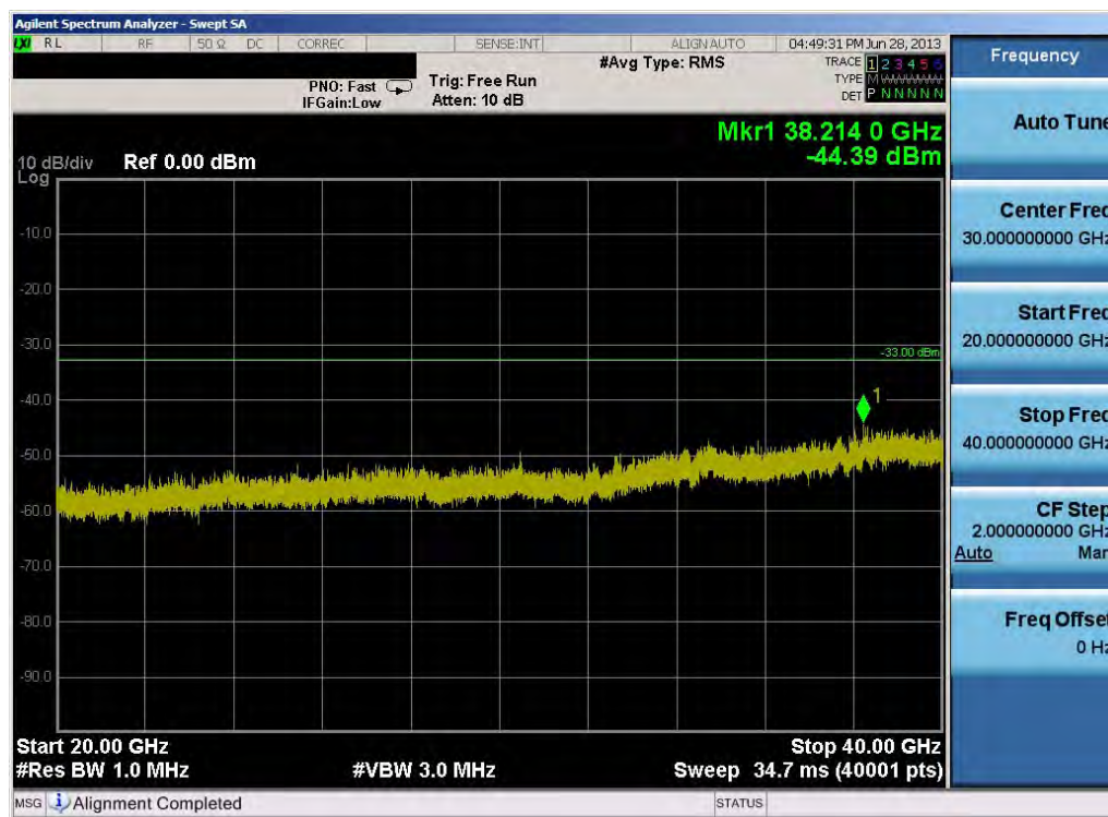
Plot 6-58. Conducted Spurious Plot (802.11a – Ch. 165)
