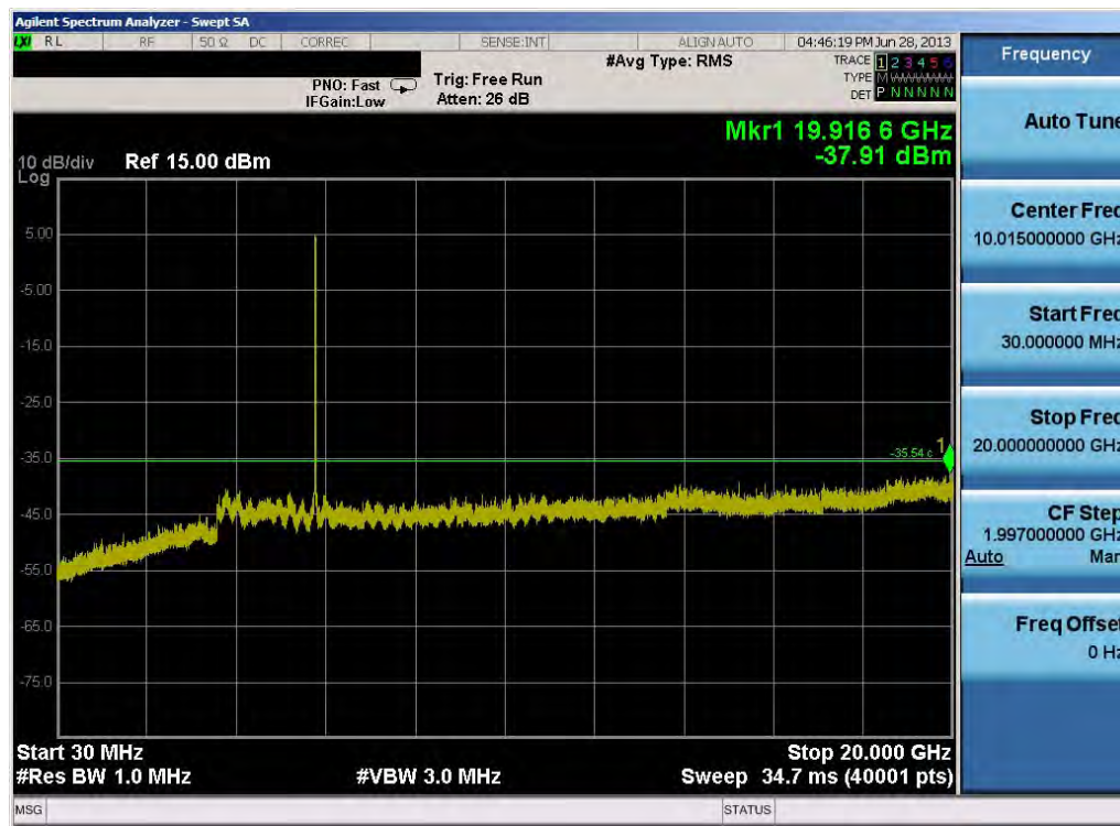
Plot 6-55. Conducted Spurious Plot (802.11a - Ch. 157)
