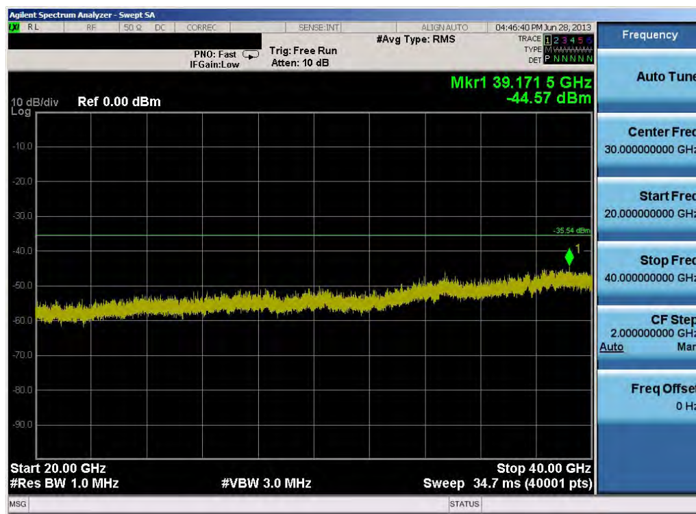
Plot 6-56. Conducted Spurious Plot (802.11a - Ch. 157)
