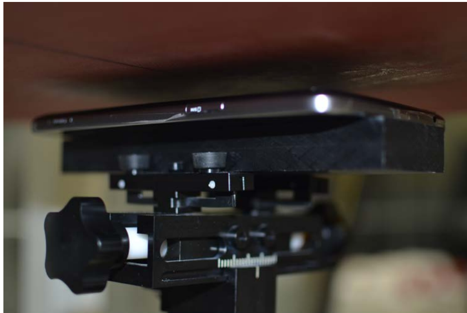
SAR Test Setup Photo 2: Back at 1.4 cm
