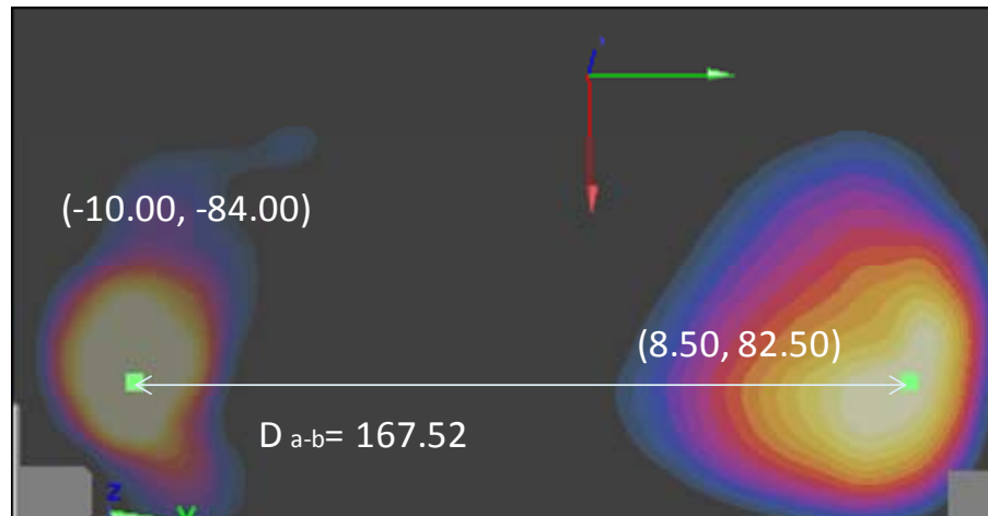
Figure 12-1 Peak SAR Locations of 2.4 GHz WLAN and GPRS 1900 MHz
