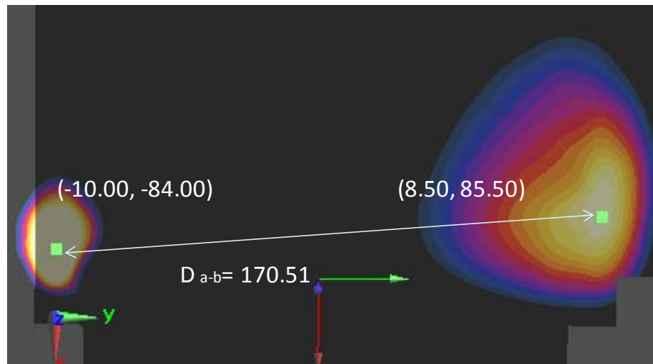
Figure 12-2 Peak SAR Locations of 2.4 GHz WLAN and UMTS 850 MHz
