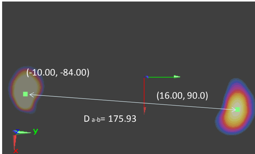
Figure 12-5 Peak SAR Locations of 2.4 GHz WLAN and GPRS 1900 MHz
