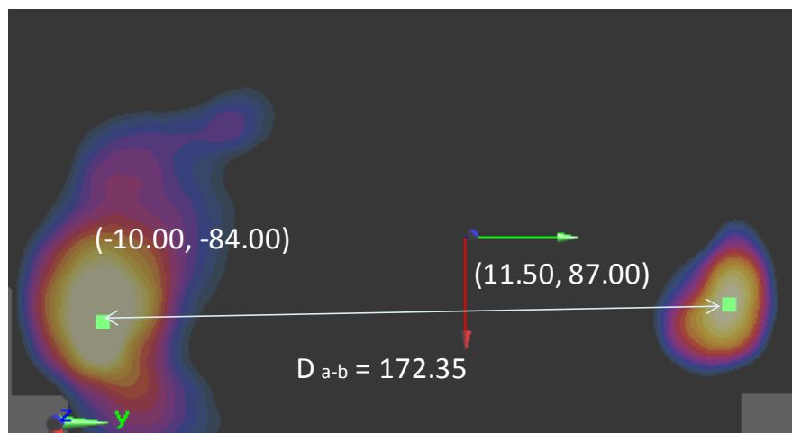
Figure 12-3 Peak SAR Locations of 2.4 GHz WLAN and UMTS 1900 MHz
