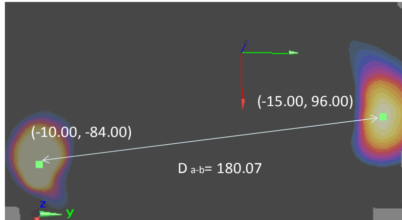
Figure 12-6 Peak SAR Locations of 2.4 GHz WLAN and UMTS 1900 MHz
