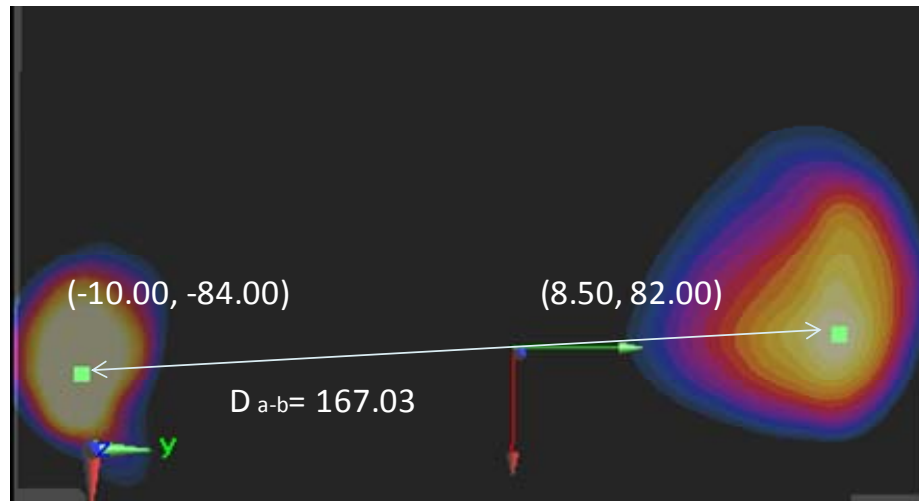
Figure 12-4 Peak SAR Locations of 2.4 GHz WLAN and LTE band 5
