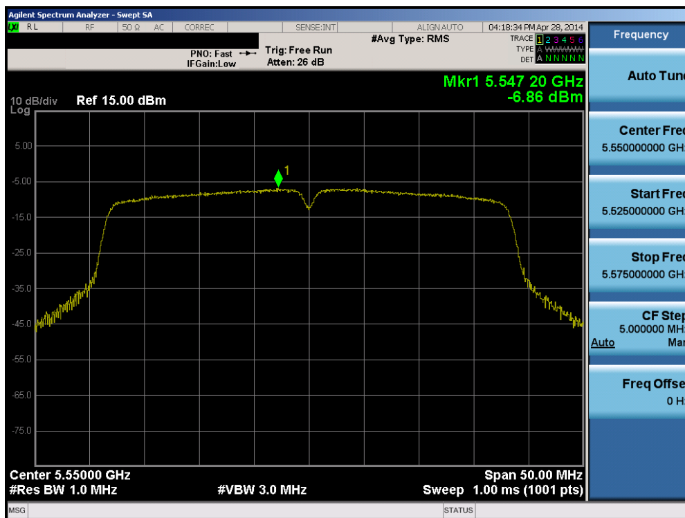
Plot 6-53. Peak Power Spectral Density Plot (40MHz BW 802.11a/n (UNII Band 2C) – Ch. 110)
