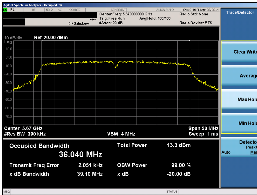
Plot 6-29. 20dB Bandwidth Plot (40MHz BW 802.11n (UNII Band 2C) – Ch. 134)
