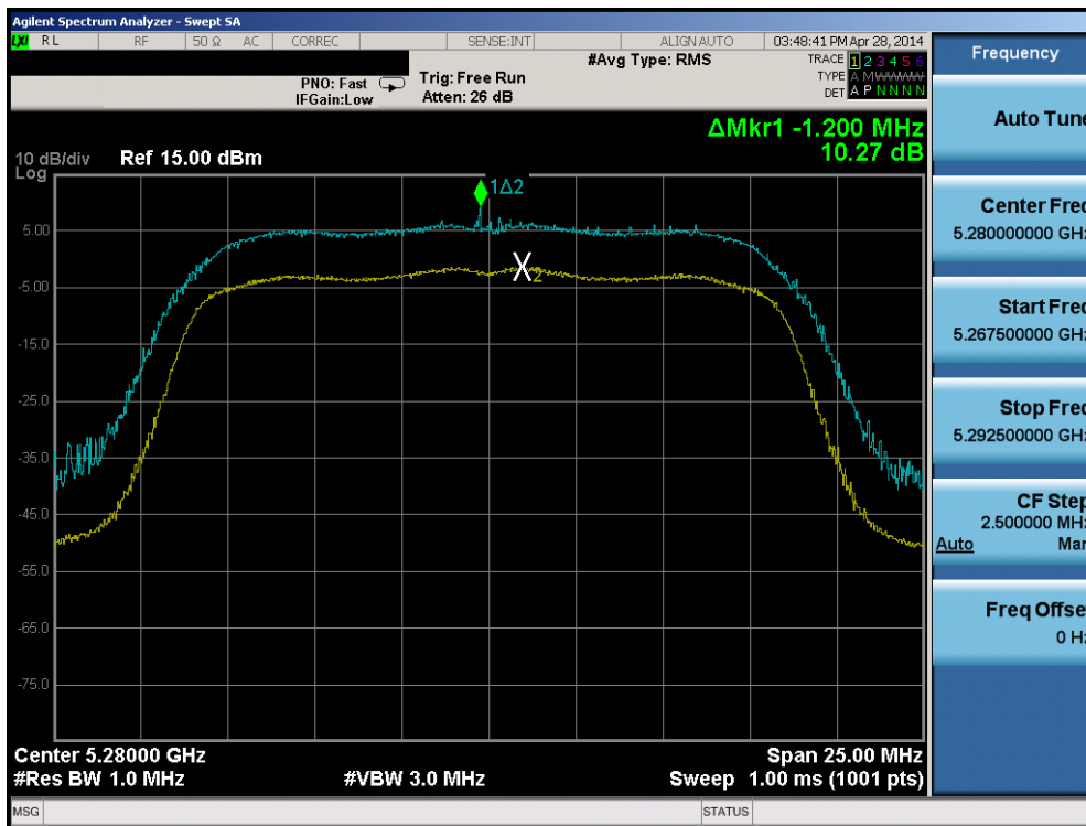
Plot 6-56. Peak Excursion Ratio Plot (802.11a (UNII Band 2A) – Ch. 56)
