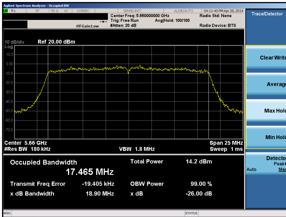
Plot 6-23. 26dB Bandwidth Plot (20MHz BW 802.11n (UNII Band 2C) – Ch. 132)
