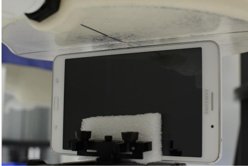
SAR Test Setup Photo 11: Left Edge at 4 mm
