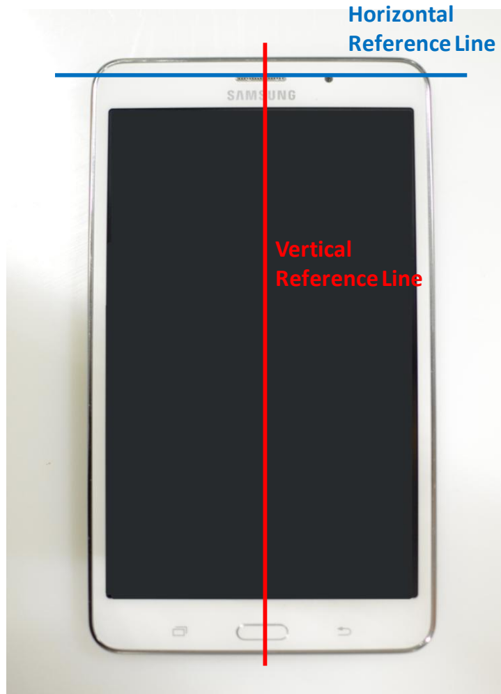
SAR Test Setup Photo 13: Vertical and Horizontal Reference Lines
