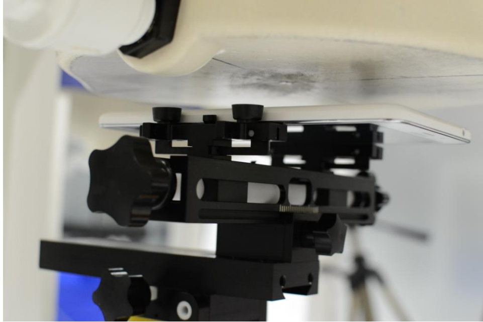
SAR Test Setup Photo 5: Back Side at 21 mm
