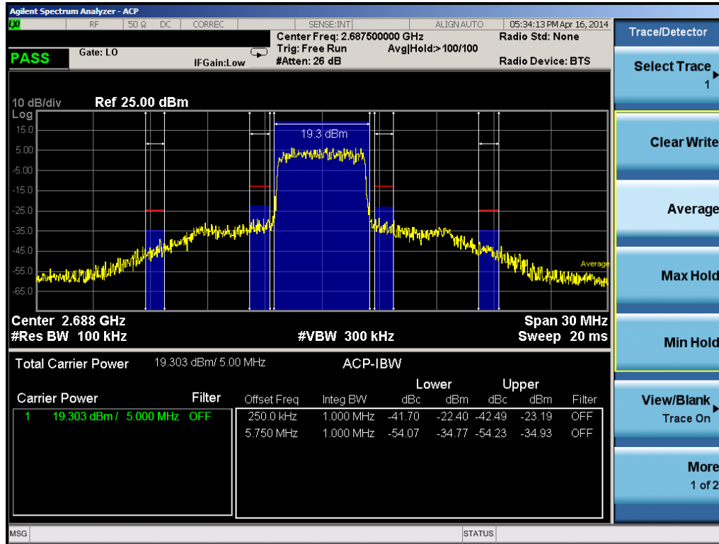
Plot 6-30. High Adjacent Channel Band Edge Plot (5.0 MHz QPSK – RB Size 25)
