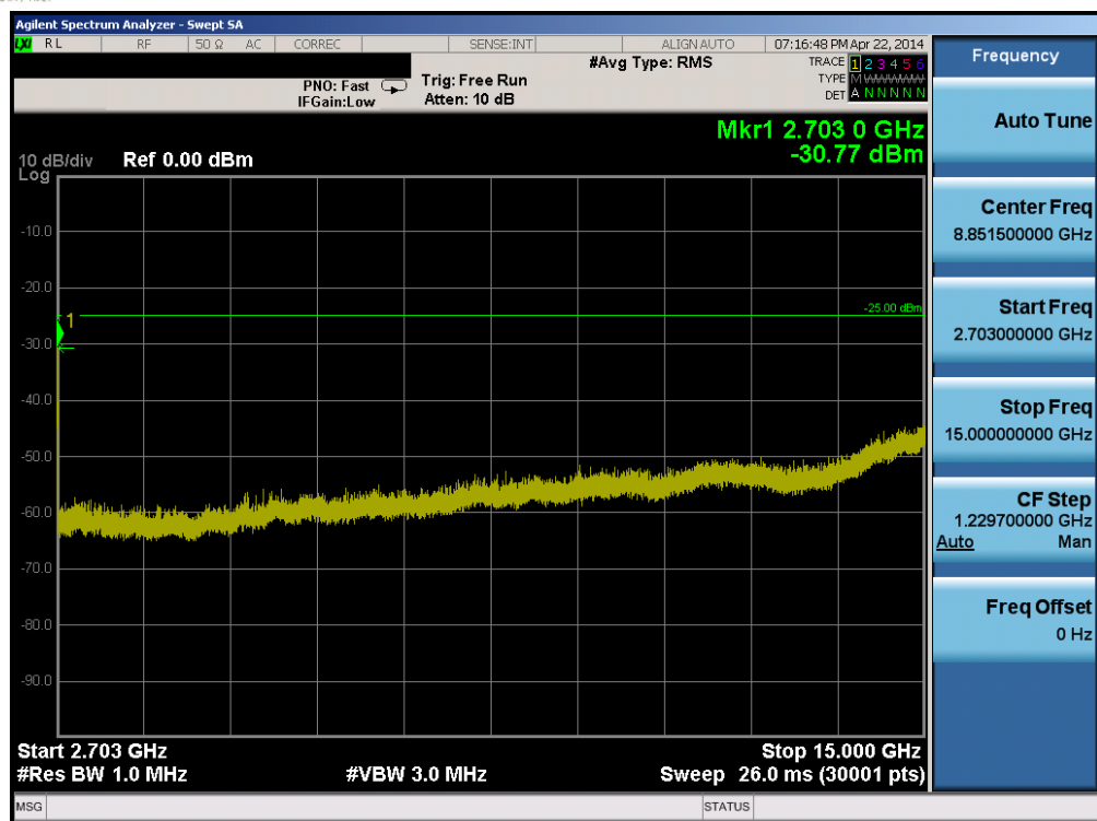
Plot 6-19. Conducted Spurious Plot (Band 41 – 10.0MHz QPSK – RB Size 49, RB Offset 0 – High Channel)
