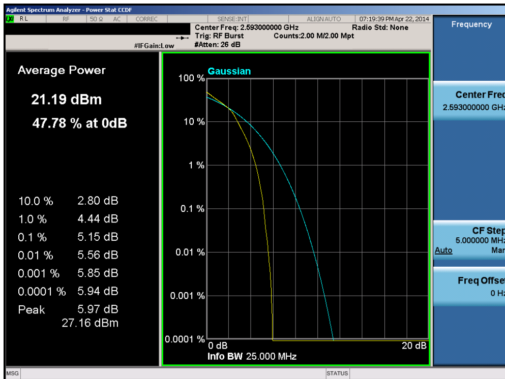
Plot 6-45. PAR Plot (Band 41 – 15.0MHz 16-QAM – RB Size 75)
