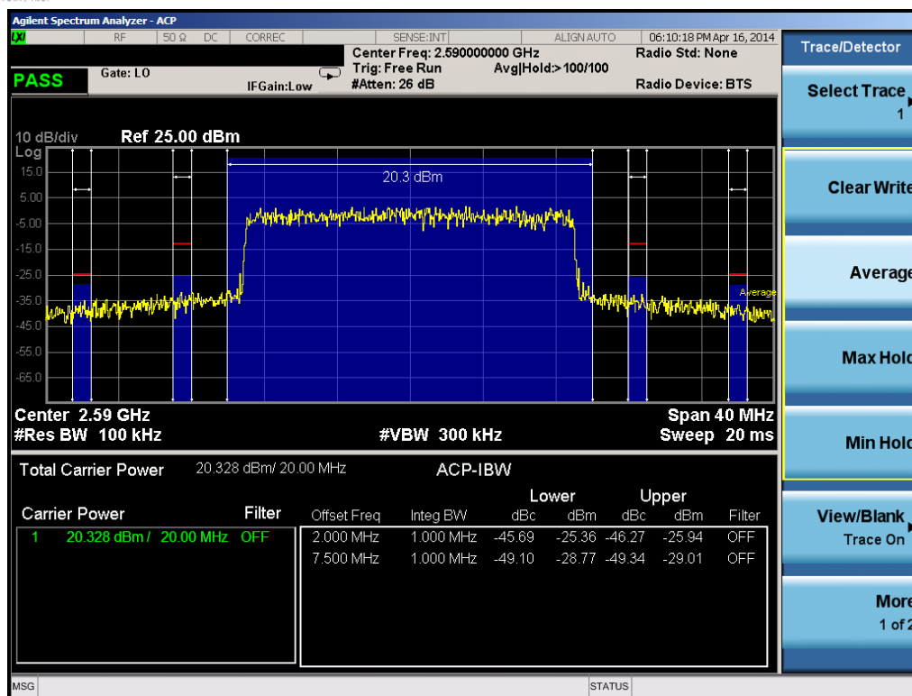
Plot 6-38. Mid Extended Band Edge Plot (Band 41 – 20.0MHz QPSK – RB Size 100)
