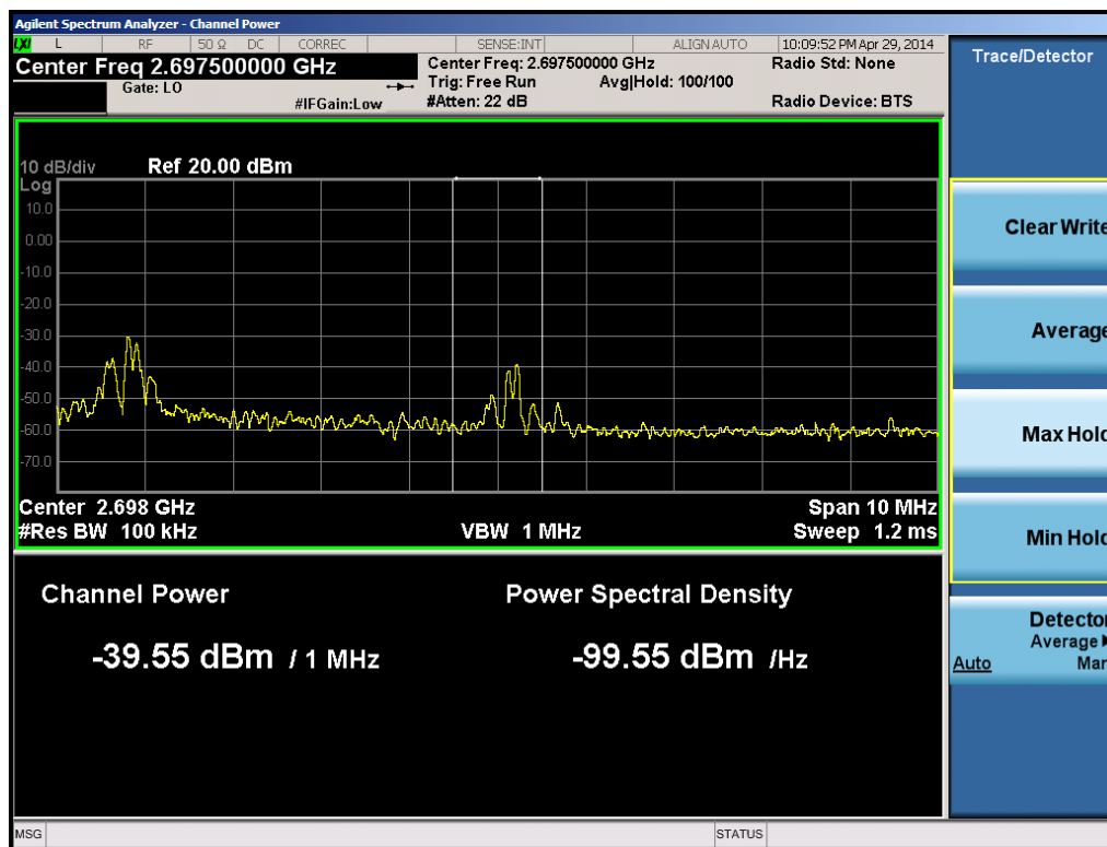
Plot 6-22. Upper Band Edge Plot 1MHz Integration (Band 41 – 10.0MHz QPSK – RB Size 1, Offset 49)
