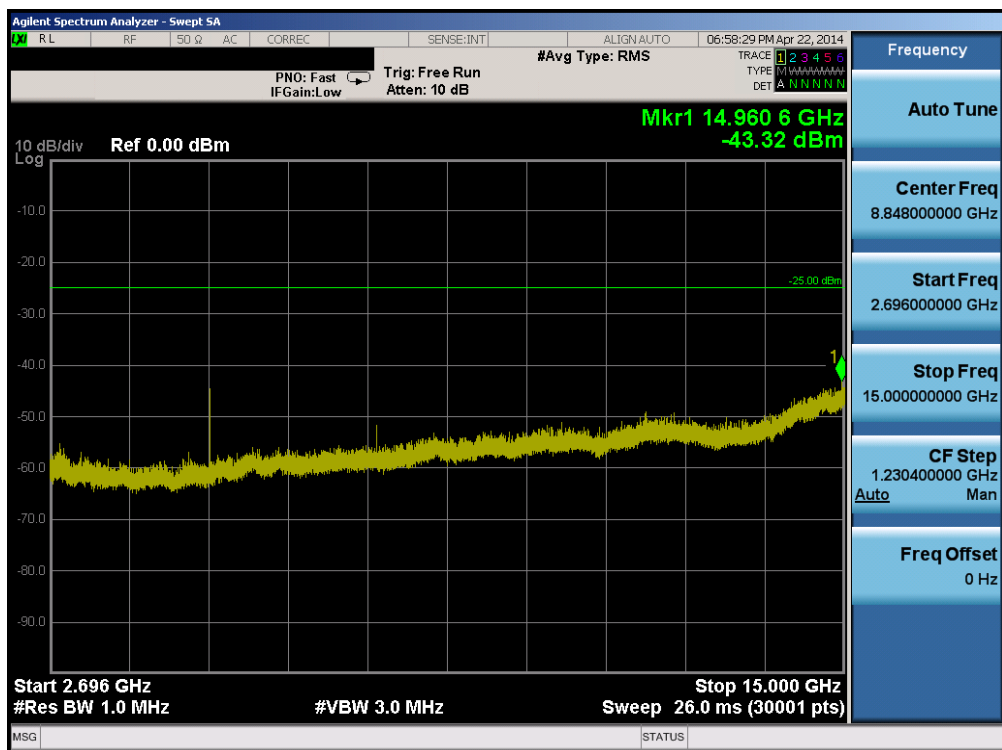
Plot 6-16. Conducted Spurious Plot (Band 41 – 10.0MHz QPSK – RB Size 1, RB Offset 0 – Mid Channel)
