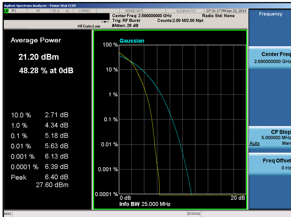
Plot 6-47. PAR Plot (Band 41 – 20.0MHz 16-QAM – RB Size 100)
