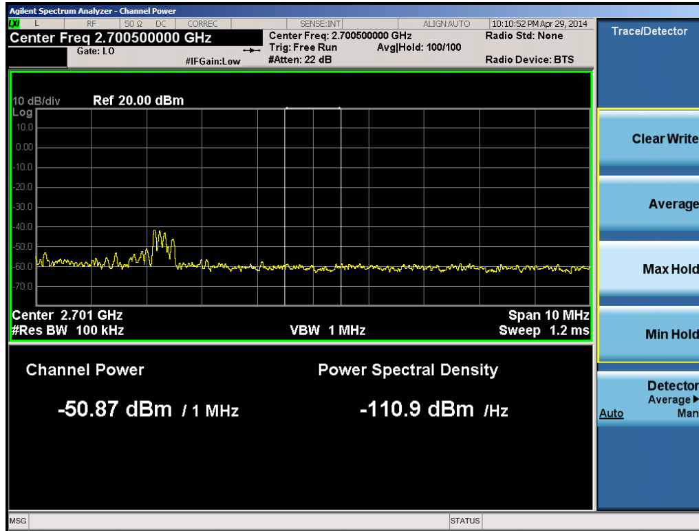
Plot 6-25. Upper Band Edge Plot 1MHz Integration (Band 41 – 10.0MHz QPSK – RB Size 1, Offset 49)
