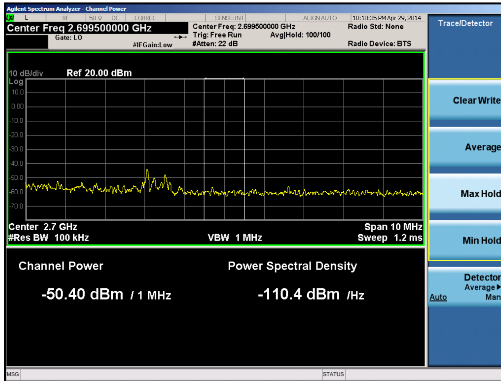
Plot 6-24. Upper Band Edge Plot 1MHz Integration (Band 41 – 10.0MHz QPSK – RB Size 1, Offset 49)
