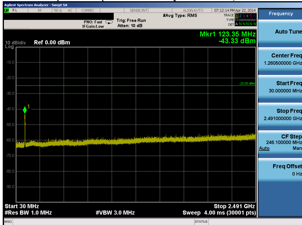
Plot 6-18. Conducted Spurious Plot (Band 41 – 10.0MHz QPSK – RB Size 49, RB Offset 0 – High Channel)
