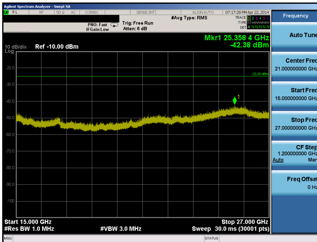
Plot 6-20. Conducted Spurious Plot (Band 41 – 10.0MHz QPSK – RB Size 50, RB Offset 49 – High Channel)
