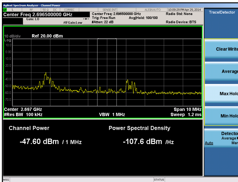
Plot 6-21. Upper Band Edge Plot 1MHz Integration (Band 41 – 10.0MHz QPSK – RB Size 1, Offset 49)
