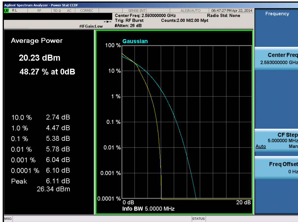
Plot 6-41. PAR Plot (Band 41 – 5.0MHz 16-QAM – RB Size 25)
