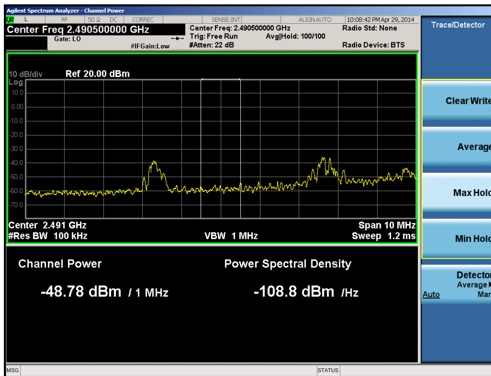
Plot 6-14. Lower Band Edge Plot 1MHz Integration (Band 41 – 10.0MHz QPSK – RB Size 1, Offset 0)
