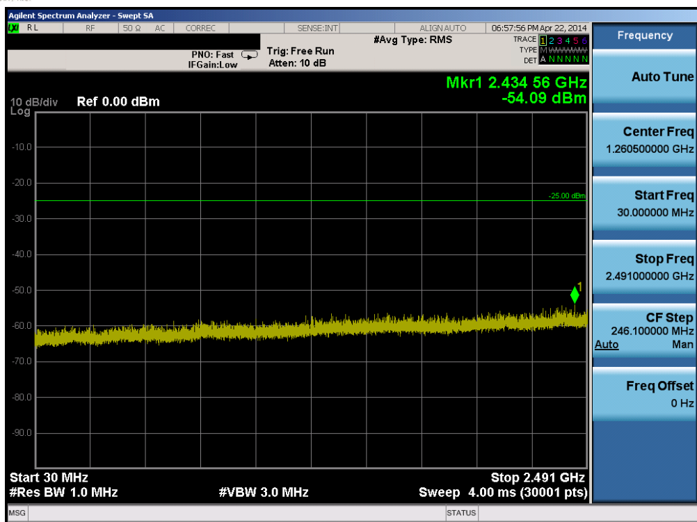
Plot 6-15. Conducted Spurious Plot (Band 41 – 10.0MHz QPSK – RB Size 1, RB Offset 0 – Mid Channel)
