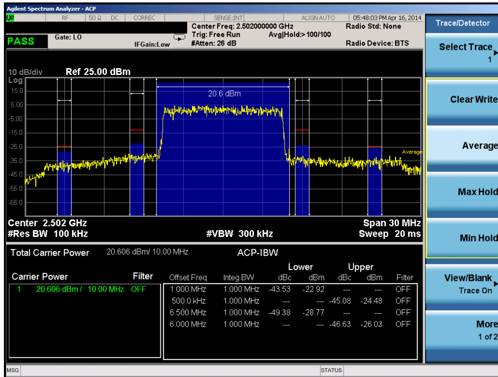
Plot 6-31. Low Adjacent Channel Band Edge Plot (10.0 MHz QPSK – RB Size 50)
