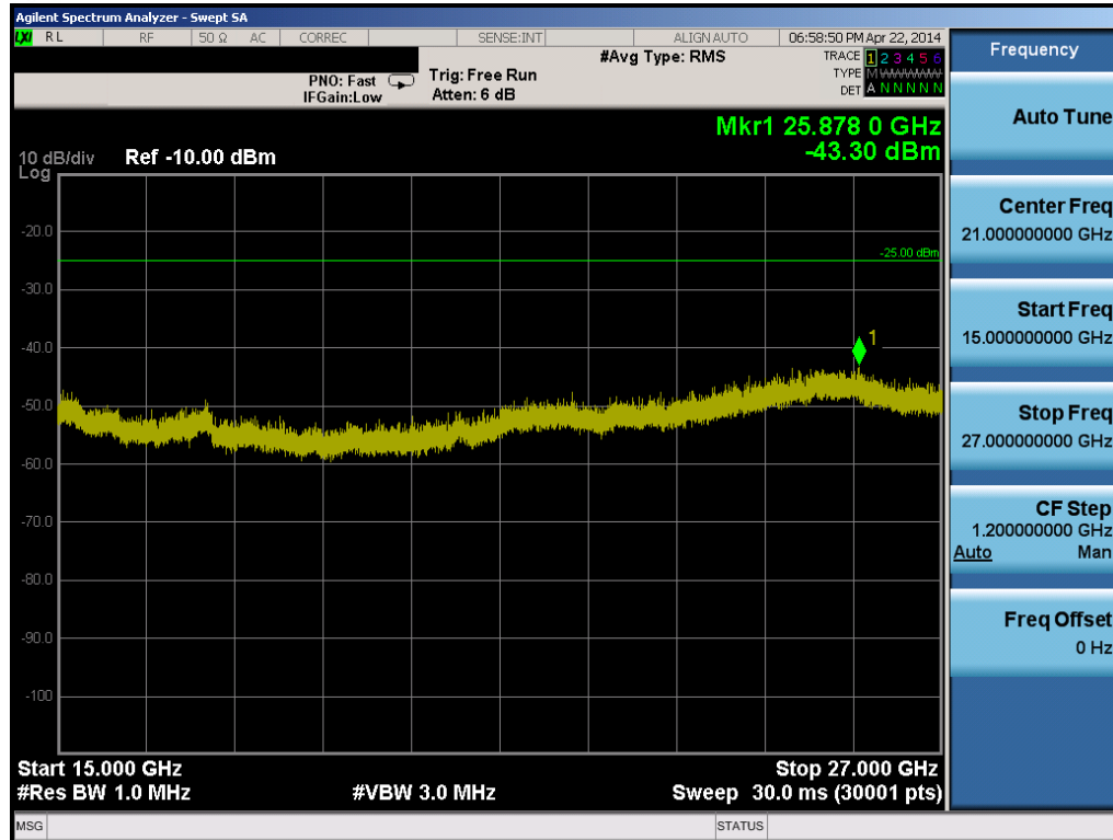
Plot 6-17. Conducted Spurious Plot (Band 41 – 10.0MHz QPSK – RB Size 1, RB Offset 0 – Mid Channel)
