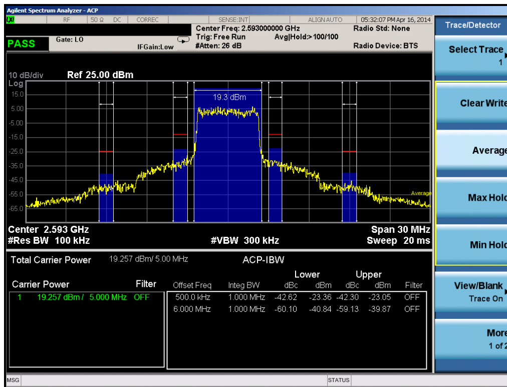
Plot 6-29. Mid Adjacent Channel Band Edge Plot (5.0 MHz QPSK – RB Size 25)
