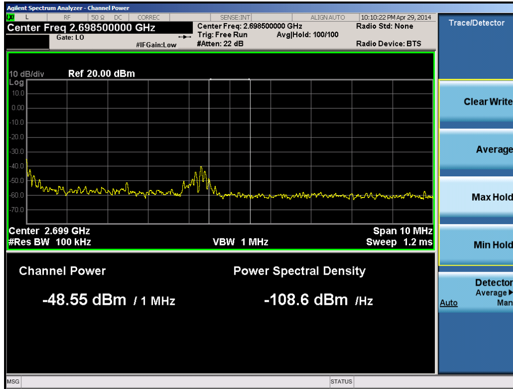
Plot 6-23. Upper Band Edge Plot 1MHz Integration (Band 41 – 10.0MHz QPSK – RB Size 1, Offset 49)
