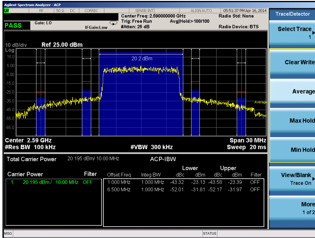
Plot 6-32. Mid Adjacent Channel Band Edge Plot (10.0 MHz QPSK – RB Size 50)
