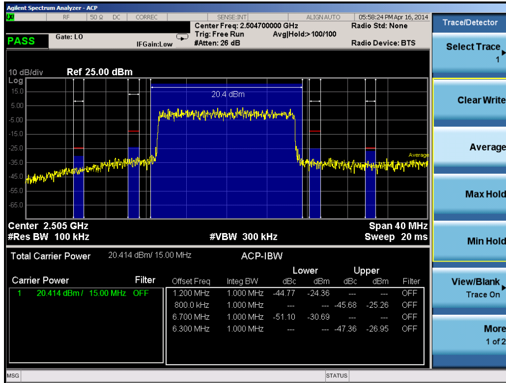
Plot 6-34. Low Adjacent Channel Band Edge Plot (15.0 MHz QPSK – RB Size 75)
