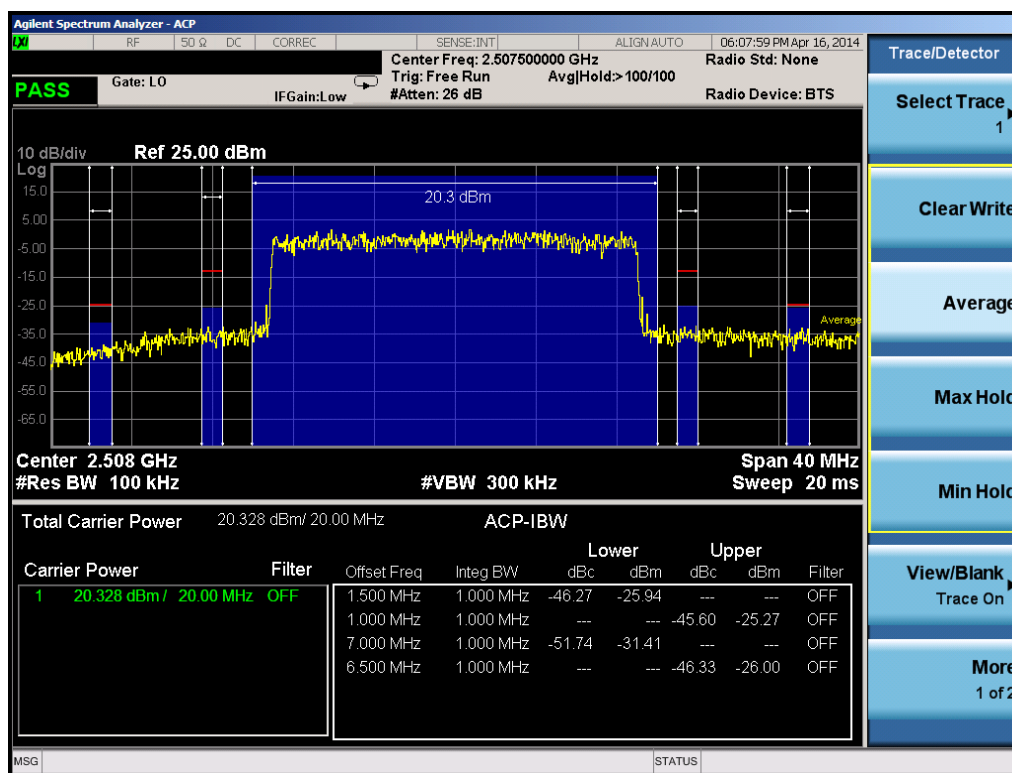
Plot 6-37. Low Extended Band Edge Plot (Band 41 – 20.0MHz QPSK – RB Size 100)
