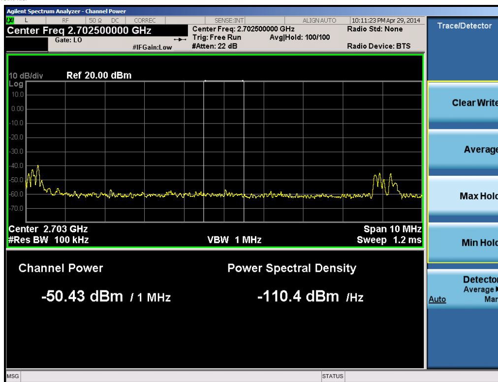
Plot 6-27. Upper Band Edge Plot 1MHz Integration (Band 41 – 10.0MHz QPSK – RB Size 1, Offset 49)
