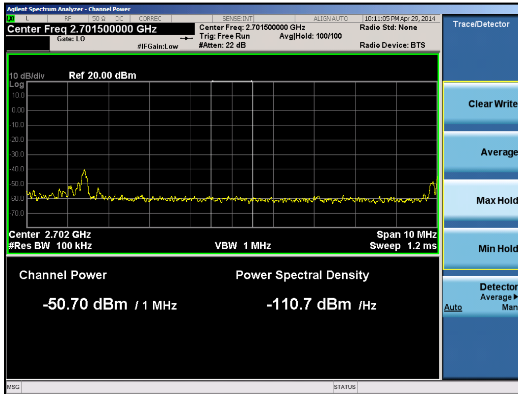
Plot 6-26. Upper Band Edge Plot 1MHz Integration (Band 41 – 10.0MHz QPSK – RB Size 1, Offset 49)
