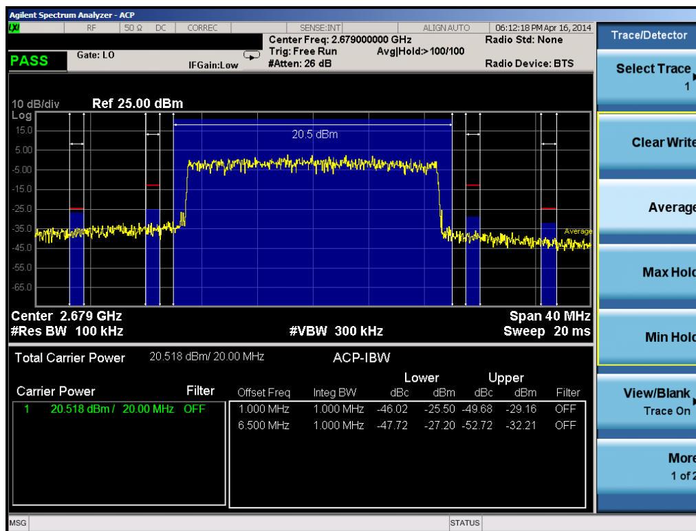
Plot 6-39. High Extended Band Edge Plot (Band 41 – 20.0MHz QPSK – RB Size 100)
