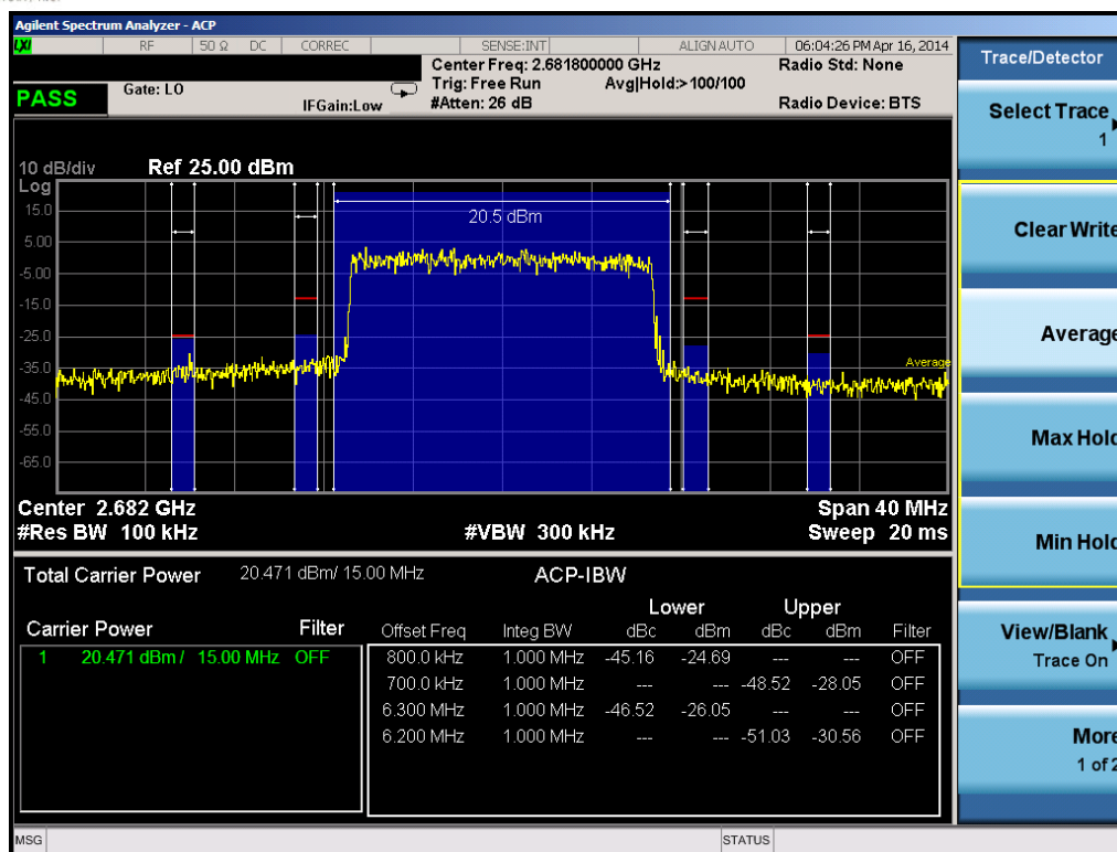
Plot 6-36. High Adjacent Channel Band Edge Plot (15.0 MHz QPSK – RB Size 75)
