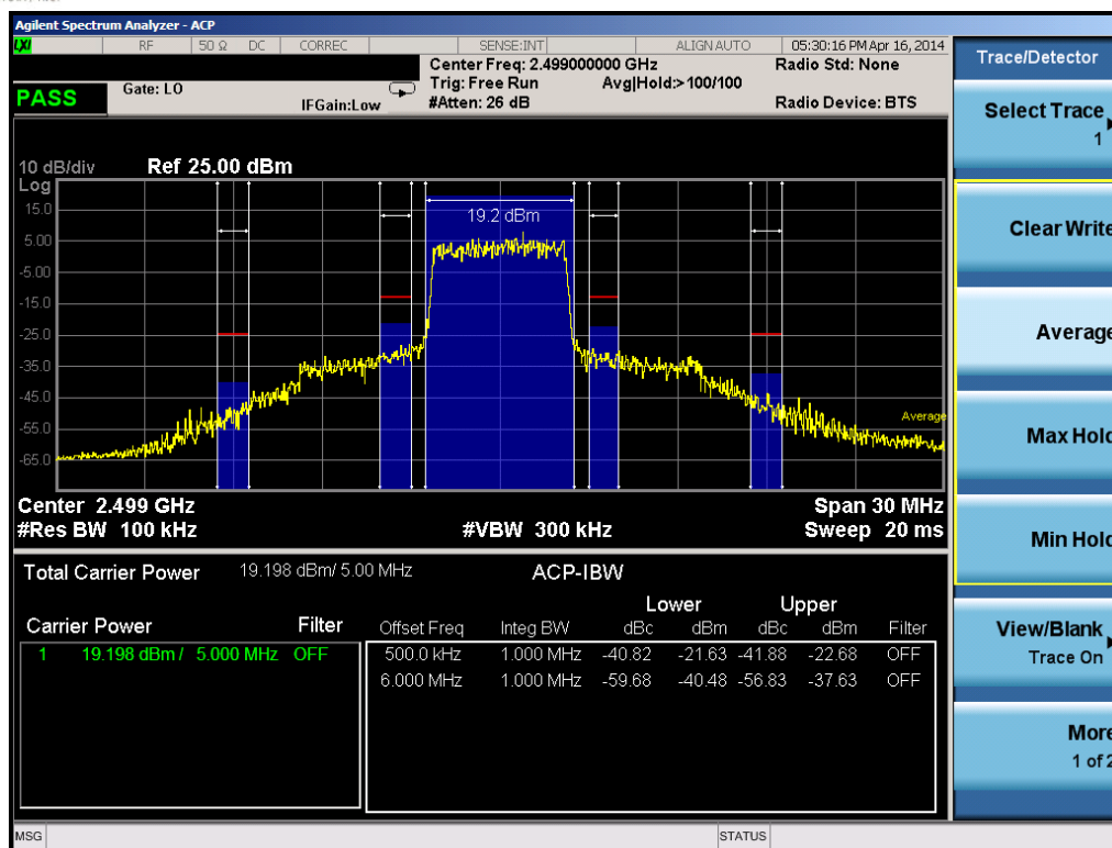
Plot 6-28. Low Adjacent Channel Band Edge Plot (5.0 MHz QPSK – RB Size 25)
