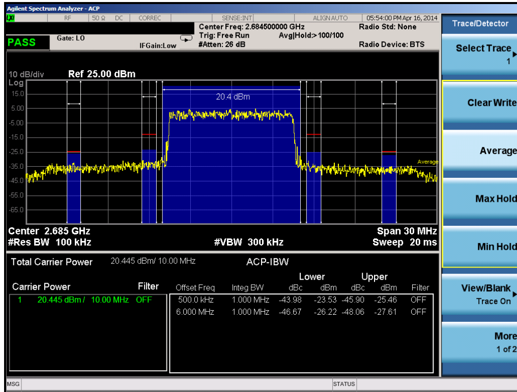
Plot 6-33. High Adjacent Channel Band Edge Plot (10.0 MHz QPSK – RB Size 50)
