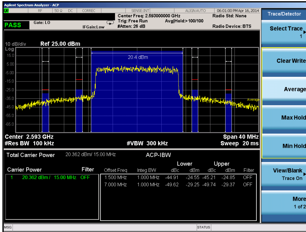
Plot 6-35. Mid Adjacent Channel Band Edge Plot (15.0 MHz QPSK – RB Size 75)
