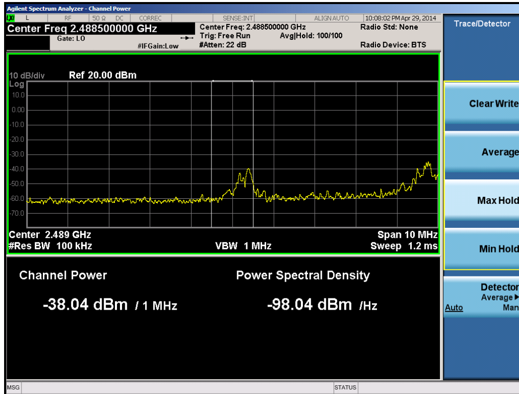
Plot 6-12. Lower Band Edge Plot 1MHz Integration (Band 41 – 10.0MHz QPSK – RB Size 1, Offset 0)
