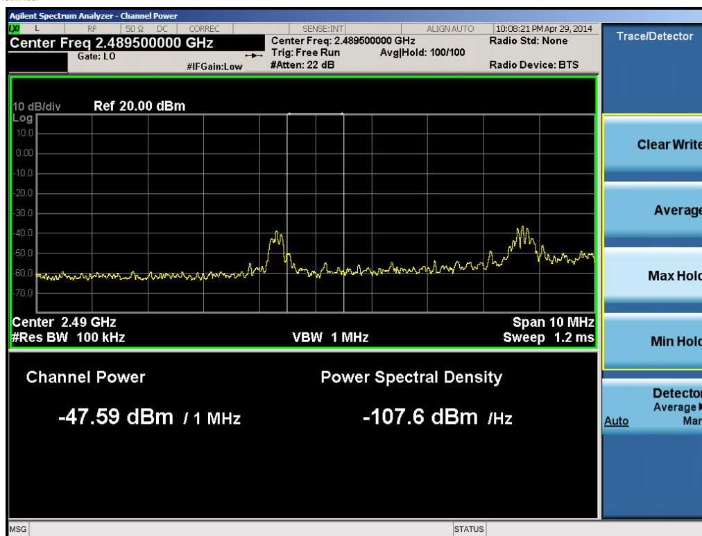
Plot 6-13. Lower Band Edge Plot 1MHz Integration (Band 41 – 10.0MHz QPSK – RB Size 1, Offset 0)
