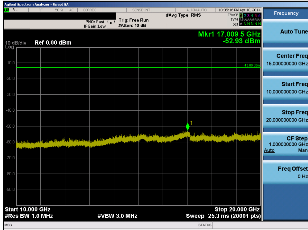
Plot 6-26. Conducted Spurious Plot (PCS WCDMA Mode – Ch. 9538)
