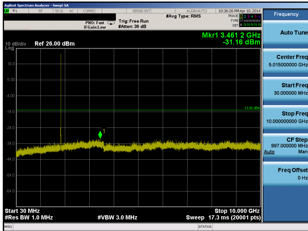
Plot 6-21. Conducted Spurious Plot (PCS WCDMA Mode – Ch. 9262)
