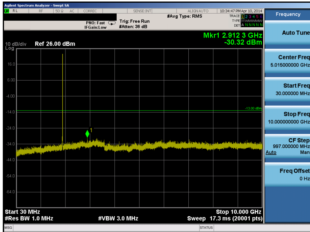
Plot 6-25. Conducted Spurious Plot (PCS WCDMA Mode – Ch. 9538)
