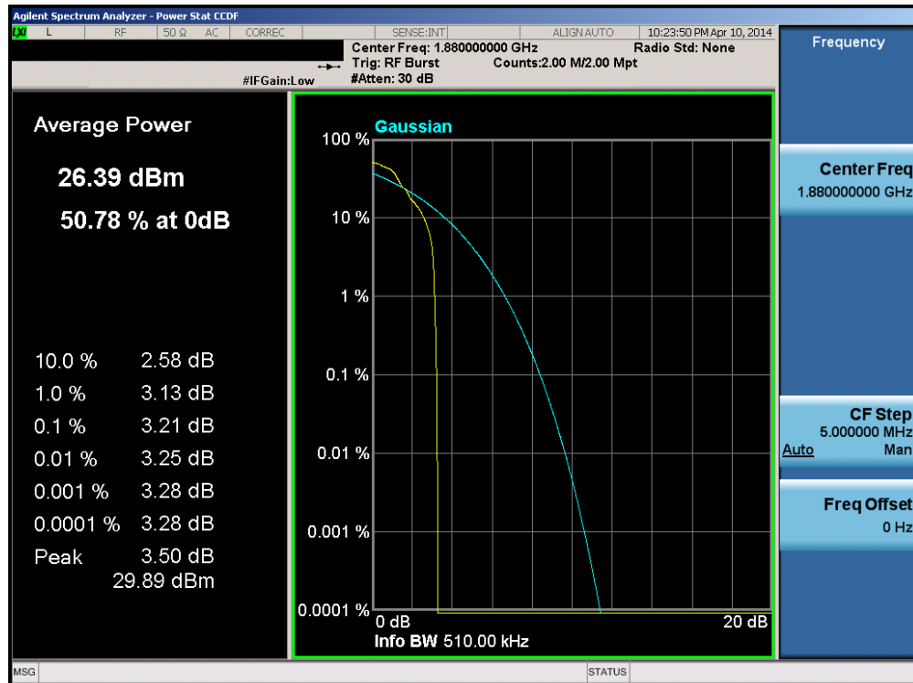
Plot 6-36. Peak-Average Ratio Plot (EDGE1900 Mode – Ch. 661)
