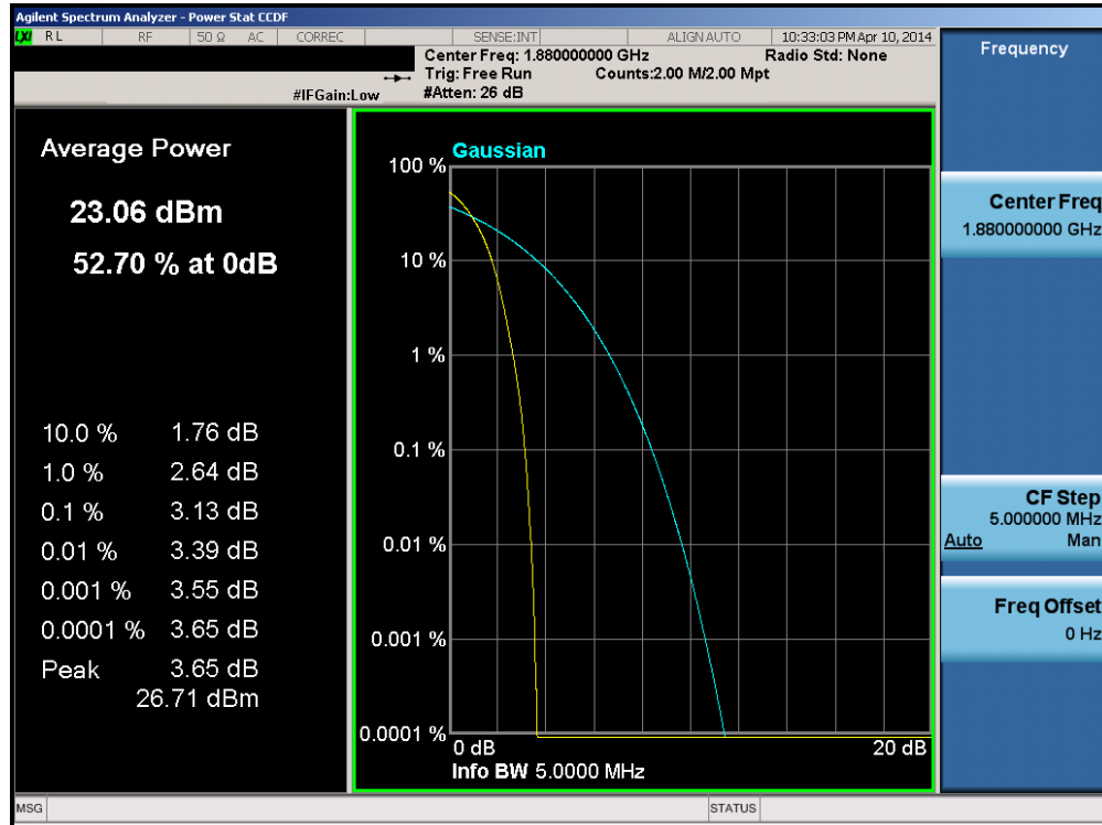
Plot 6-37. Peak-Average Ratio Plot (PCS WCDMA Mode – Ch. 9400)
