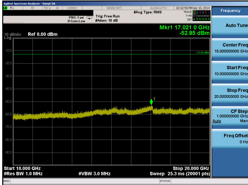
Plot 6-24. Conducted Spurious Plot (PCS WCDMA Mode – Ch. 9400)
