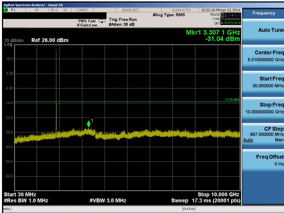
Plot 6-23. Conducted Spurious Plot (PCS WCDMA Mode – Ch. 9400)
