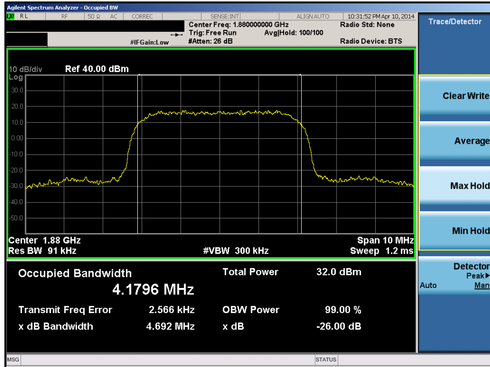
Plot 6-5. Occupied Bandwidth Plot (PCS WCDMA Mode – Ch. 9400)
