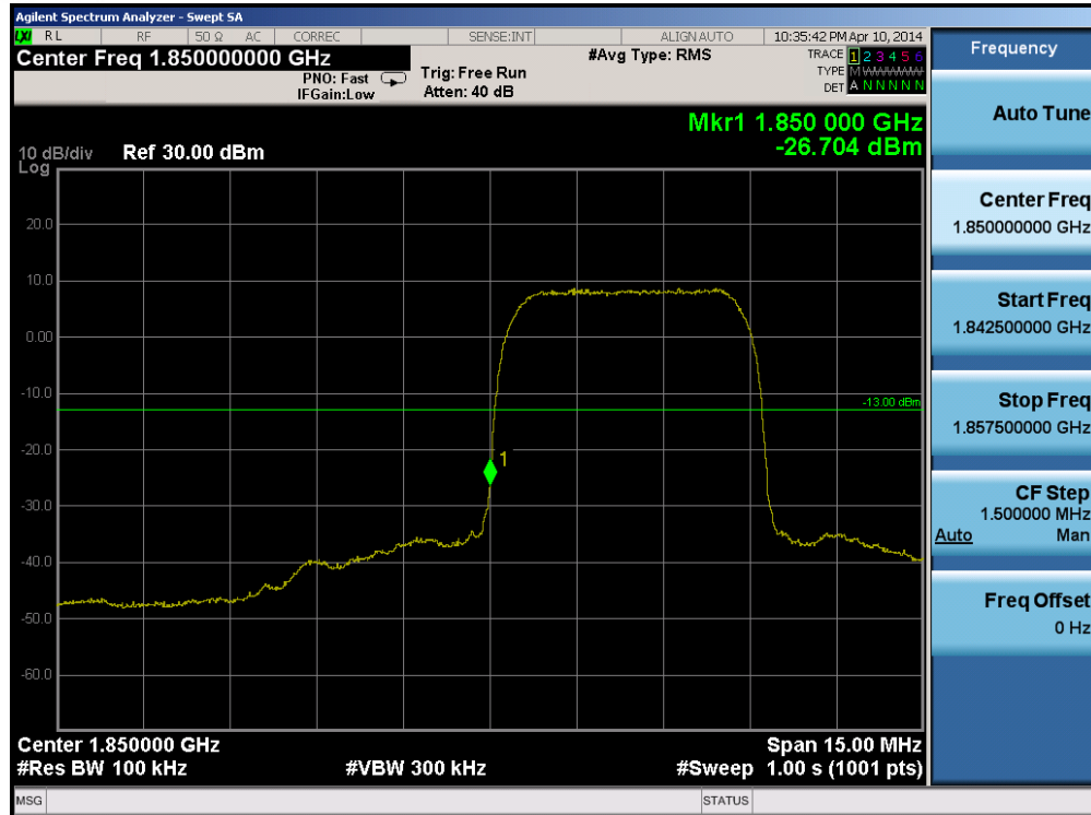
Plot 6-31. Band Edge Plot (PCS WCDMA Mode – Ch. 9262)
