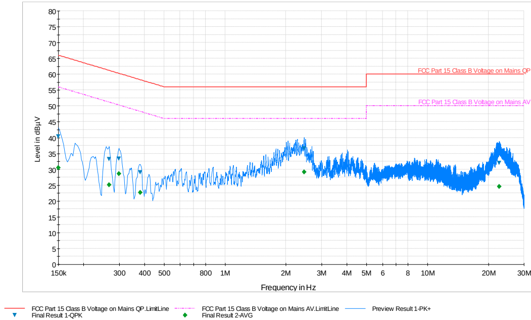
Plot 6-76. Line Conducted Plot with 802.11a UNII Band 2A (L1)
