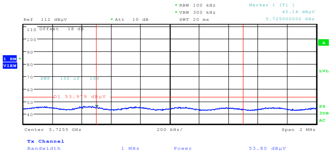
Plot 6-72. Radiated Upper Band Edge Plot (Average– UNII Band 2C)
