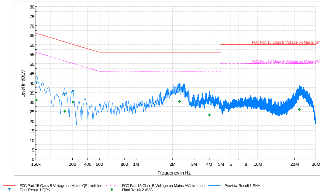
Plot 6-74. Line Conducted Plot with 802.11a UNII Band 1 (L1)
