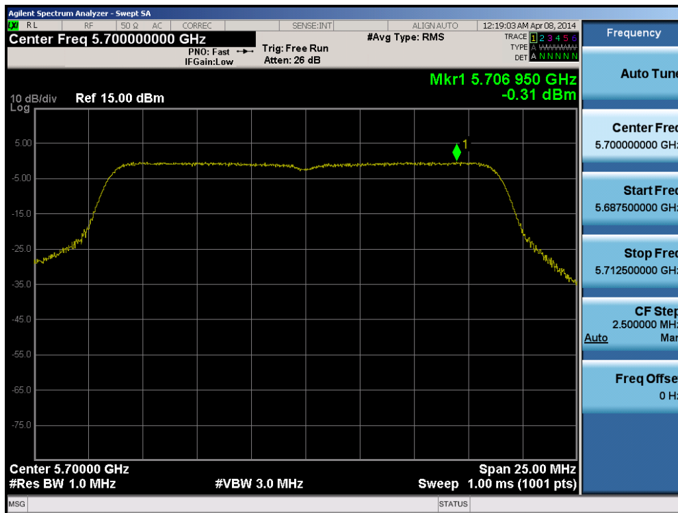
Plot 6-52. Peak Power Spectral Density Plot (20MHz BW 802.11a/n (UNII Band 2C) – Ch. 140)
