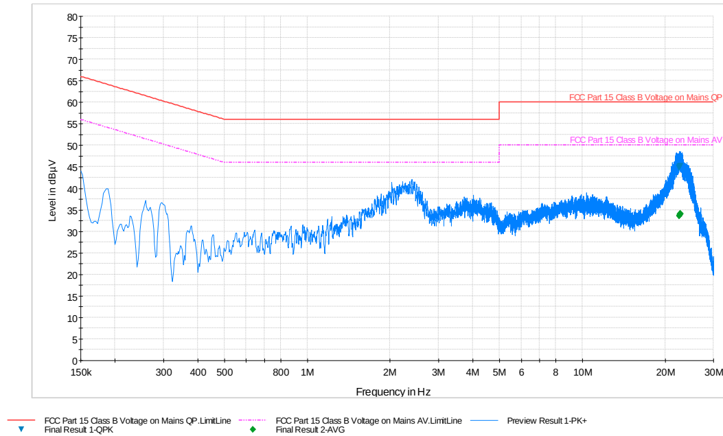
Plot 6-75. Line Conducted Plot with 802.11a UNII Band 1 (N)
