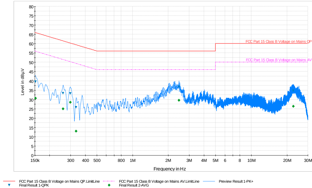
Plot 6-78. Line Conducted Plot with 802.11a UNII Band 2C (L1)
