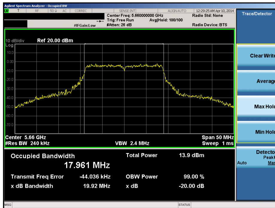
Plot 6-28. 20dB Bandwidth Plot (20MHz BW 802.11a/n (UNII Band 2C) – Ch. 132)
