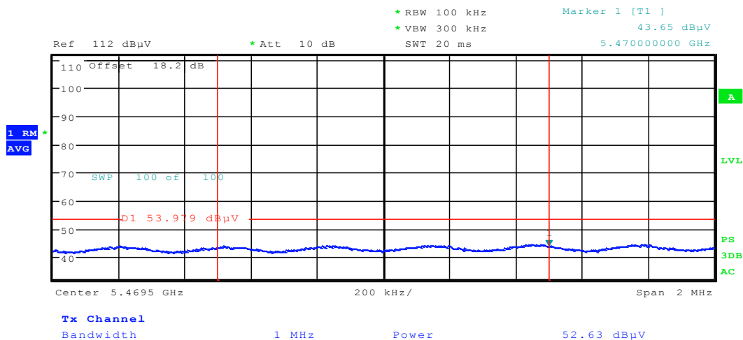
Plot 6-70. Radiated Restricted Lower Band Edge Plot (Average – UNII Band 2C)
