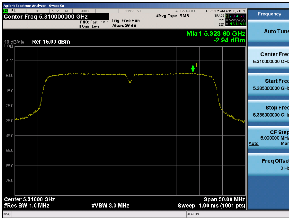
Plot 6-46. Peak Power Spectral Density Plot (40MHz BW 802.11a/n (UNII Band 2A) – Ch. 62)
