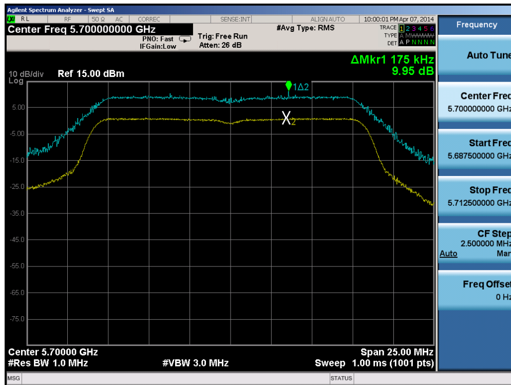
Plot 6-56. Peak Excursion Ratio Plot (802.11a (UNII Band 2C) – Ch. 140)
