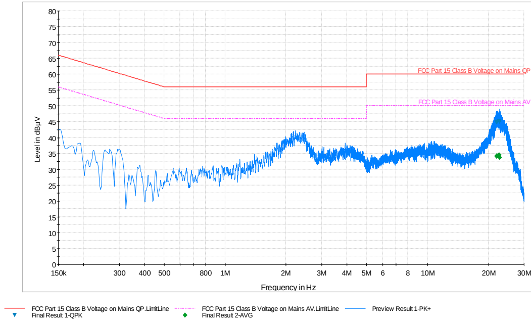
Plot 6-79. Line Conducted Plot with 802.11a UNII Band 2C (N)
