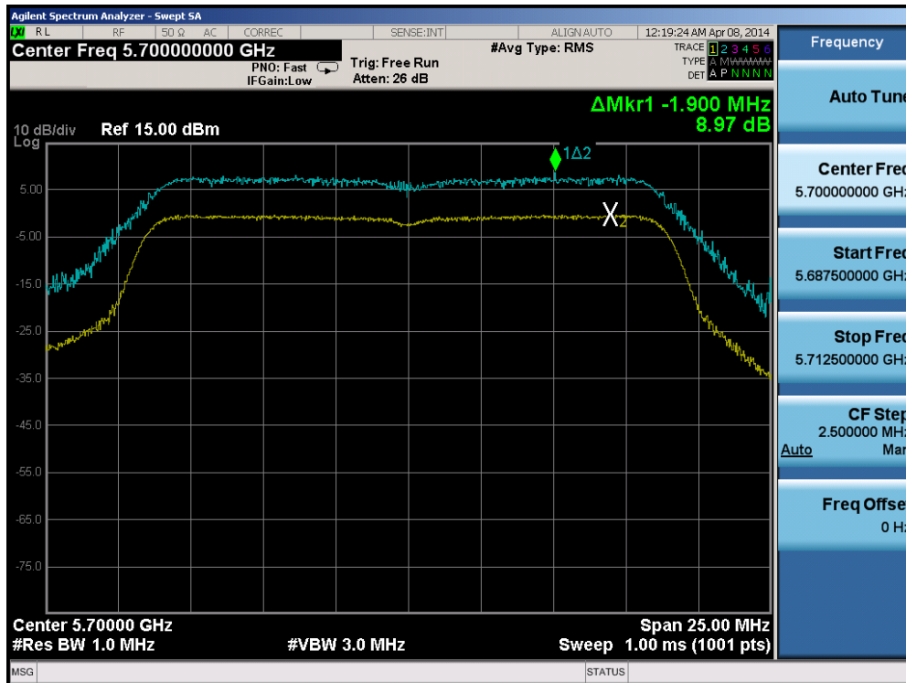
Plot 6-57. Peak Excursion Ratio Plot (20MHz BW 802.11n (UNII Band 2C) – Ch. 140)
