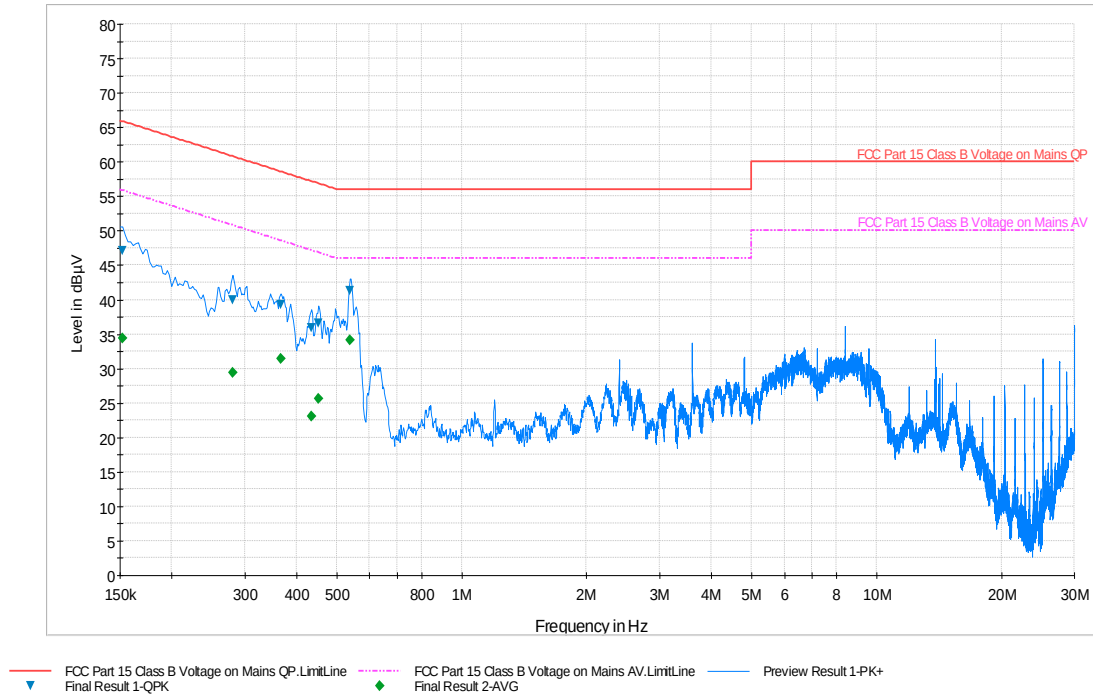
Plot 6-77. Line Conducted Plot with 802.11a UNII Band 2A (N)
