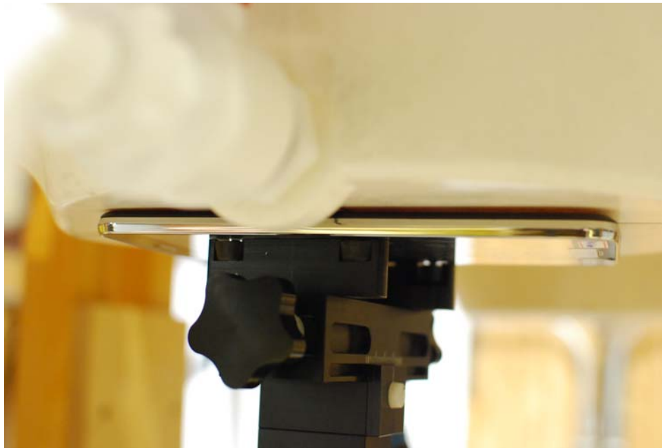
SAR Test Setup Photo 6: Back at 0 mm
