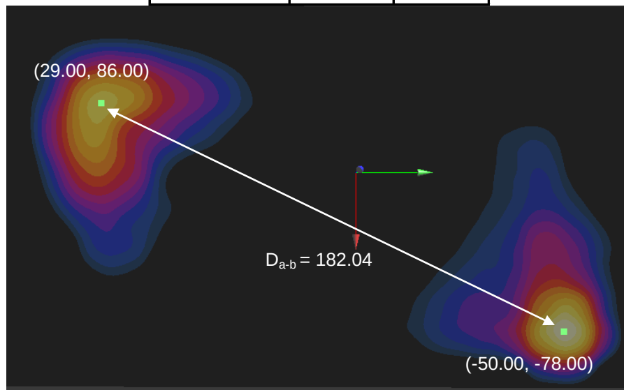
Figure 11-3 Peak SAR Locations for Body Back Side at 0 mm UMTS 1900 and 2.4 GHz WLAN Antenna
