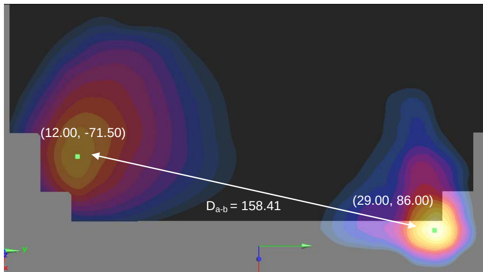
Figure 11-1 Peak SAR Locations for Body Back Side at 0 mm GPRS 850 and 2.4 GHz WLAN Antenna
